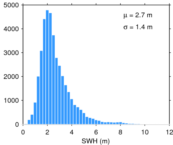
Figure 20. Histogram of science-valid SWH over oceans and lakes for 26/02/2017. The mean ( \mu ) and standard deviation ( \sigma ) are also shown. Note that values larger than 12 m are excluded from the histogram for the sake of readability but not from the computation of \mu and \sigma .
