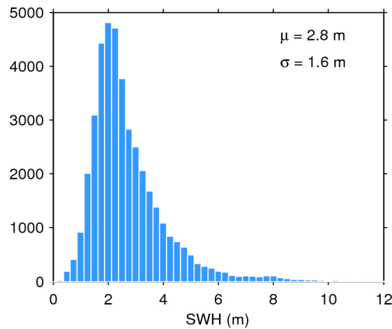
Figure 17. Histogram of flag-valid SWH over oceans and lakes for 26/02/2017. The mean ( \mu ) and standard deviation ( \sigma ) are also shown. Note that values larger than 12 m are excluded from the histogram for the sake of readability but not from the computation of \mu and \sigma .
