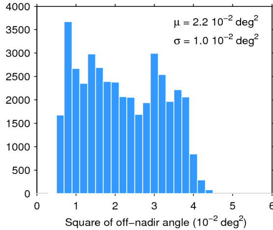
Figure 39. Histogram of flag-valid mispointing over oceans and lakes for 26/02/2017. The mean ( \mu ) and standard deviation ( \sigma ) are also shown. Note that values larger than 6 \cdot 10^{-2} \text{ deg}^2 are excluded from the histogram for the sake of readability but not from the computation of \mu and \sigma .
