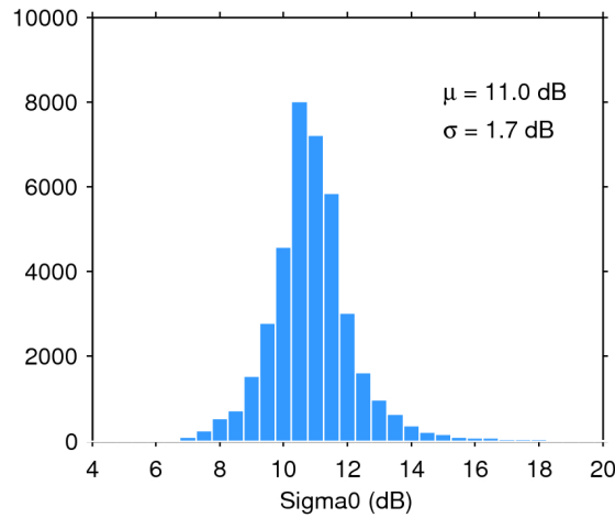
Figure 28. Histogram of science-valid sigma0 over oceans and lakes for 26/02/2017. The mean ( \mu ) and standard deviation ( \sigma ) are also shown. Note that values outside [4 20] dB are excluded from the histogram for the sake of readability but not from the computation of \mu and \sigma .
