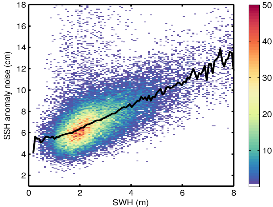
Figure 9. 2D histogram showing flag-valid SSH anomaly noise as a function of SWH for 26/02/2017. The black line denotes the median SSH anomaly noise as a function of SWH.
