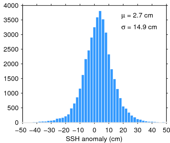
Figure 7. Histogram of flag-valid SSH anomaly over oceans and lakes for 26/02/2017. The mean ( \mu ) and standard deviation ( \sigma ) are also shown. Note that values outside [-50 50] cm are excluded from the histogram for the sake of readability but not from the computation of \mu and \sigma .
