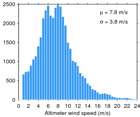
Figure 33. Histogram of flag-valid wind over oceans and lakes for 26/02/2017. The mean ( \mu ) and standard deviation ( \sigma ) are also shown. Note that values larger than 24 m/s are excluded from the histogram for the sake of readability but not from the computation of \mu and \sigma .
