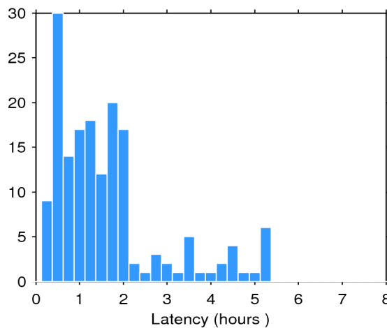
Figure 2. Histogram of the data latency for 26/02/2017. The y-axis denotes the number of files that are made available with a delay of x-hours with respect to the mean time of the records stored in the file.
