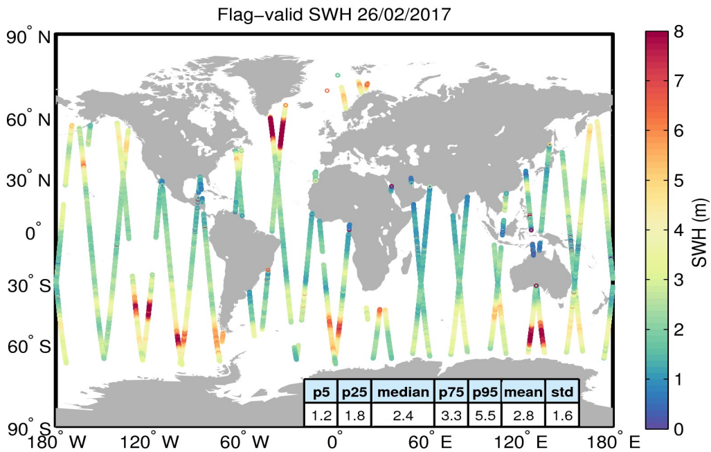
Figure 15. Geographical distribution of flag-valid SWH data over oceans and lakes for 26/02/2017. The statistical values shown in the table refer to the SWH in m and are calculated over all measurements shown in the figure.
