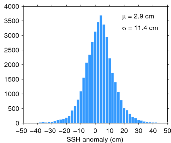
Figure 11. Histogram of science-valid SSH anomaly over oceans and lakes for 26/02/2017. The mean ( \mu ) and standard deviation ( \sigma ) are also shown. Note that values outside [-50 50] cm are excluded from the histogram for the sake of readability but not from the computation of \mu and \sigma .
