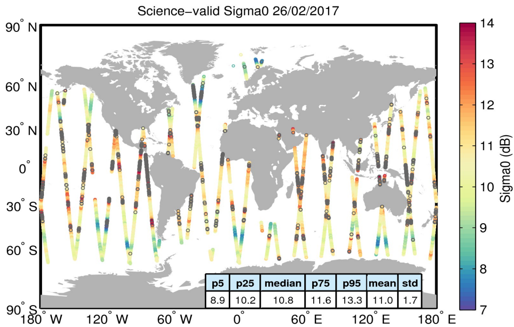
Figure 27. Geographical distribution of science-valid sigma0 data over oceans and lakes for 26/02/2017. The statistical values shown in the table refer to the sigma0 in dB and are calculated over all measurements shown in the figure. Gray circles denote records that have been rejected based on the editing criteria described in Table 4.
