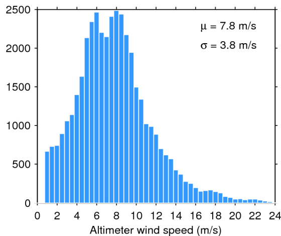
Figure 35. Histogram of science-valid wind over oceans and lakes for 26/02/2017. The mean ( \mu ) and standard deviation ( \sigma ) are also shown. Note that values larger than 24 m/s are excluded from the histogram for the sake of readability but not from the computation of \mu and \sigma .
