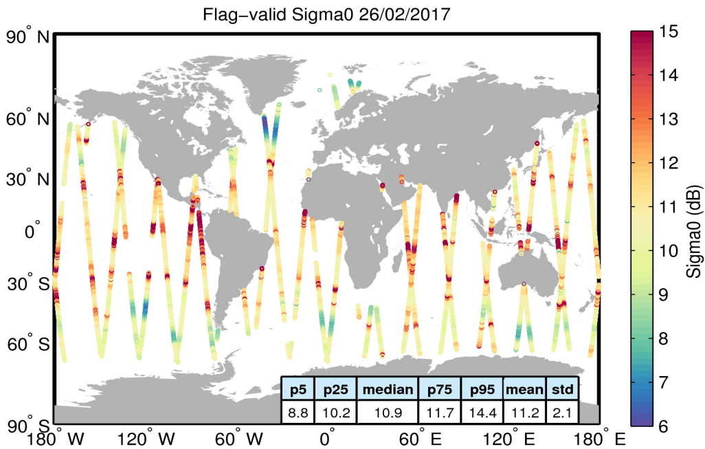
Figure 23. Geographical distribution of flag-valid sigma0 data over oceans and lakes for 26/02/2017. The statistical values shown in the table refer to the sigma0 in dB and are calculated over all measurements shown in the figure.
