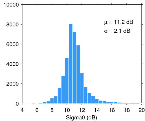
Figure 25. Histogram of flag-valid sigma0 over oceans and lakes for 26/02/2017. The mean ( \mu ) and standard deviation ( \sigma ) are also shown. Note that values outside [4 20] dB are excluded from the histogram for the sake of readability but not from the computation of \mu and \sigma .
