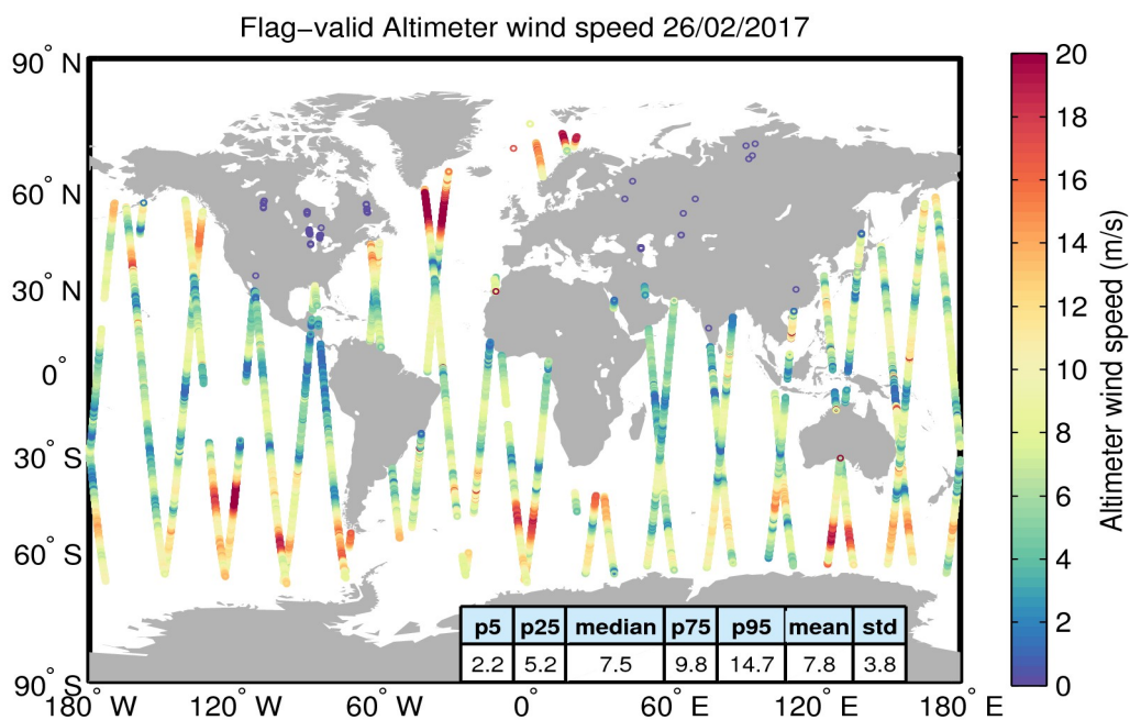
Figure 31. Geographical distribution of flag-valid wind data over oceans and lakes for 26/02/2017. The statistical values shown in the table refer to the wind in m/s and are calculated over all measurements shown in the figure.
