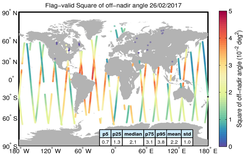
Figure 37. Geographical distribution of flag-valid mispointing data over oceans and lakes for 26/02/2017. The statistical values shown in the table refer to the mispointing in 10^{-2} \text{ deg}^2 and are calculated over all measurements shown in the figure.
