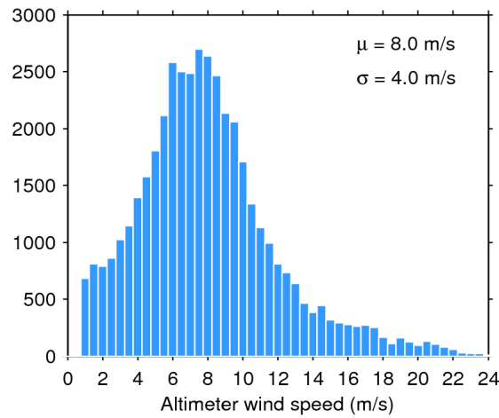
Figure 33. Histogram of flag-valid wind over oceans and lakes for 25/02/2017. The mean ( \mu ) and standard deviation ( \sigma ) are also shown. Note that values larger than 24 m/s are excluded from the histogram for the sake of readability but not from the computation of \mu and \sigma .
