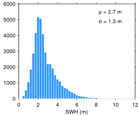
Figure 20. Histogram of science-valid SWH over oceans and lakes for 25/02/2017. The mean ( \mu ) and standard deviation ( \sigma ) are also shown. Note that values larger than 12 m are excluded from the histogram for the sake of readability but not from the computation of \mu and \sigma .
