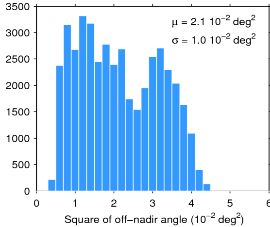
Figure 39. Histogram of flag-valid mispointing over oceans and lakes for 25/02/2017. The mean ( \mu ) and standard deviation ( \sigma ) are also shown. Note that values larger than 6 \cdot 10^{-2} \text{ deg}^2 are excluded from the histogram for the sake of readability but not from the computation of \mu and \sigma .
