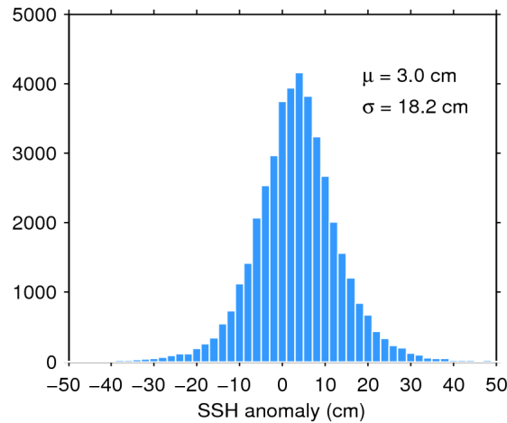
Figure 7. Histogram of flag-valid SSH anomaly over oceans and lakes for 25/02/2017. The mean ( \mu ) and standard deviation ( \sigma ) are also shown. Note that values outside [-50 50] cm are excluded from the histogram for the sake of readability but not from the computation of \mu and \sigma .
