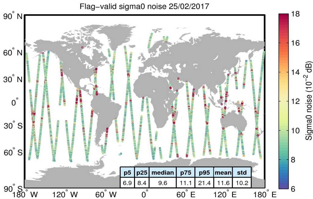
Figure 26. Geographical distribution of flag-valid 20-Hz sigma0 measurement noise over oceans and lakes for 25/02/2017. The statistical values shown in the table refer to the sigma0 noise and are calculated over all measurements shown in the figure.
