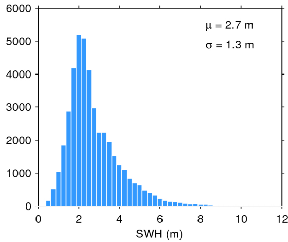
Figure 17. Histogram of flag-valid SWH over oceans and lakes for 25/02/2017. The mean ( \mu ) and standard deviation ( \sigma ) are also shown. Note that values larger than 12 m are excluded from the histogram for the sake of readability but not from the computation of \mu and \sigma .
