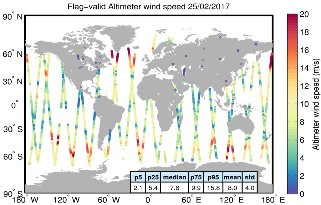
Figure 31. Geographical distribution of flag-valid wind data over oceans and lakes for 25/02/2017. The statistical values shown in the table refer to the wind in m/s and are calculated over all measurements shown in the figure.
