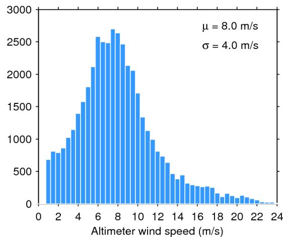
Figure 35. Histogram of science-valid wind over oceans and lakes for 25/02/2017. The mean ( \mu ) and standard deviation ( \sigma ) are also shown. Note that values larger than 24 m/s are excluded from the histogram for the sake of readability but not from the computation of \mu and \sigma .
