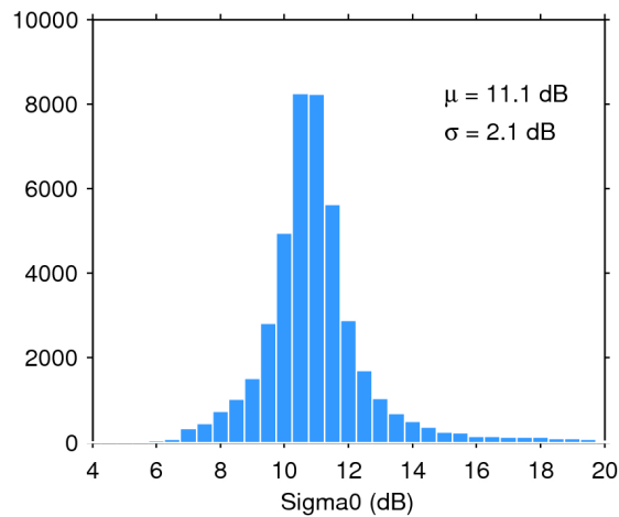
Figure 25. Histogram of flag-valid sigma0 over oceans and lakes for 25/02/2017. The mean ( \mu ) and standard deviation ( \sigma ) are also shown. Note that values outside [4 20] dB are excluded from the histogram for the sake of readability but not from the computation of \mu and \sigma .
