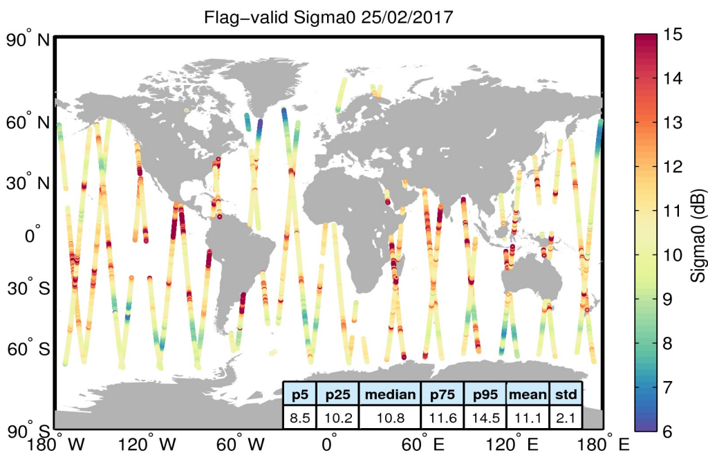
Figure 23. Geographical distribution of flag-valid sigma0 data over oceans and lakes for 25/02/2017. The statistical values shown in the table refer to the sigma0 in dB and are calculated over all measurements shown in the figure.
