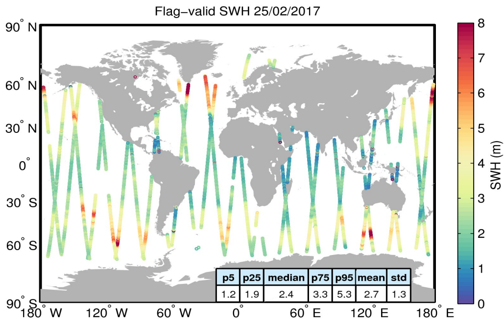
Figure 15. Geographical distribution of flag-valid SWH data over oceans and lakes for 25/02/2017. The statistical values shown in the table refer to the SWH in m and are calculated over all measurements shown in the figure.
