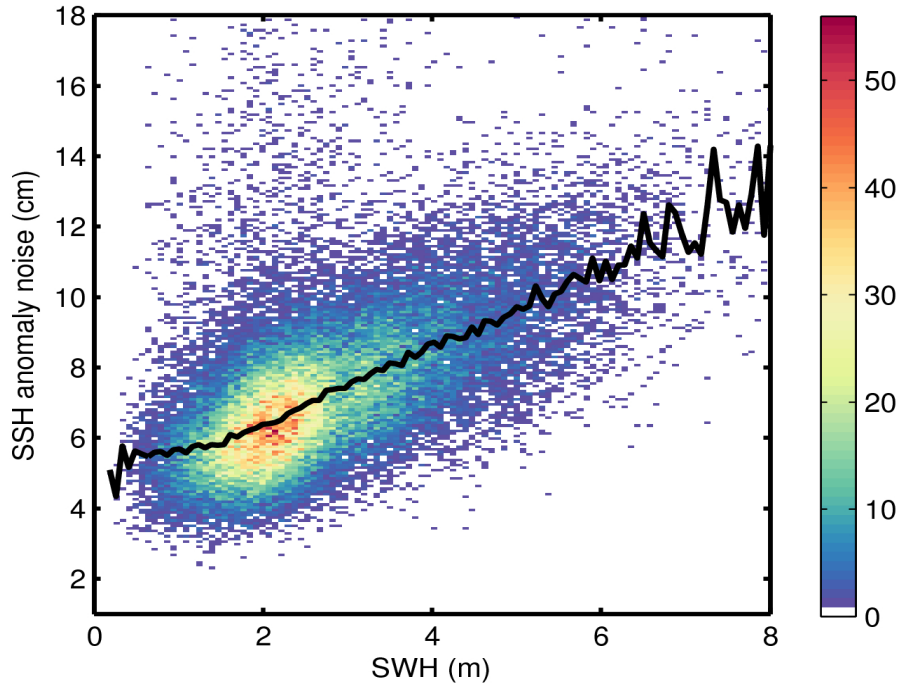
Figure 9. 2D histogram showing flag-valid SSH anomaly noise as a function of SWH for 25/02/2017. The black line denotes the median SSH anomaly noise as a function of SWH.
