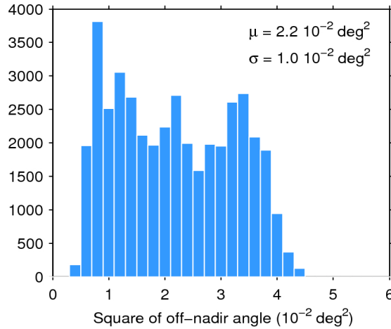
Figure 39. Histogram of flag-valid mispointing over oceans and lakes for 24/02/2017. The mean ( \mu ) and standard deviation ( \sigma ) are also shown. Note that values larger than 6 \cdot 10^{-2} \text{ deg}^2 are excluded from the histogram for the sake of readability but not from the computation of \mu and \sigma .
