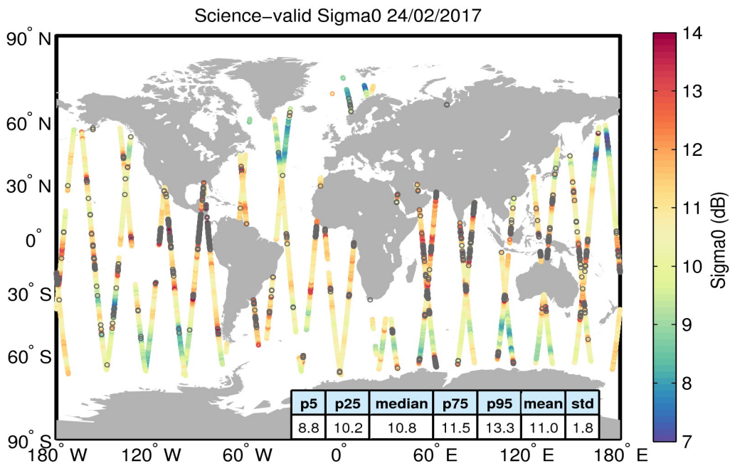
Figure 27. Geographical distribution of science-valid sigma0 data over oceans and lakes for 24/02/2017. The statistical values shown in the table refer to the sigma0 in dB and are calculated over all measurements shown in the figure. Gray circles denote records that have been rejected based on the editing criteria described in Table 4.
