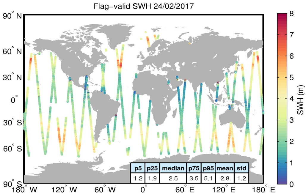
Figure 15. Geographical distribution of flag-valid SWH data over oceans and lakes for 24/02/2017. The statistical values shown in the table refer to the SWH in m and are calculated over all measurements shown in the figure.
