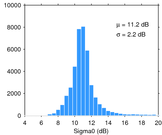
Figure 25. Histogram of flag-valid sigma0 over oceans and lakes for 24/02/2017. The mean ( \mu ) and standard deviation ( \sigma ) are also shown. Note that values outside [4 20] dB are excluded from the histogram for the sake of readability but not from the computation of \mu and \sigma .
