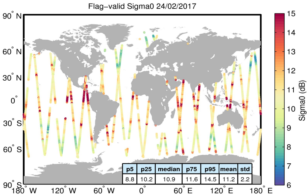
Figure 23. Geographical distribution of flag-valid sigma0 data over oceans and lakes for 24/02/2017. The statistical values shown in the table refer to the sigma0 in dB and are calculated over all measurements shown in the figure.
