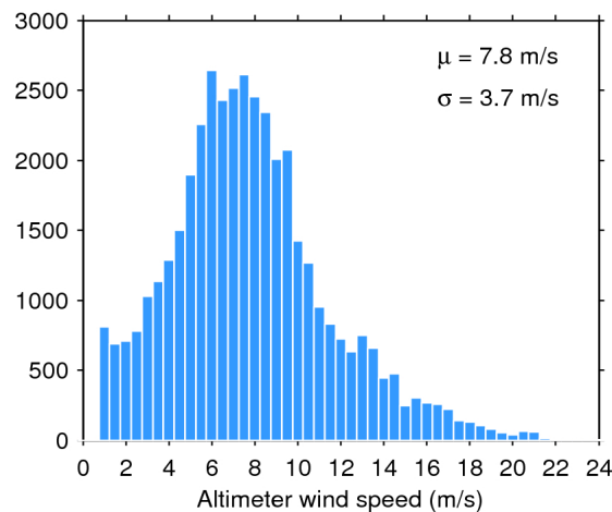
Figure 35. Histogram of science-valid wind over oceans and lakes for 24/02/2017. The mean ( \mu ) and standard deviation ( \sigma ) are also shown. Note that values larger than 24 m/s are excluded from the histogram for the sake of readability but not from the computation of \mu and \sigma .
