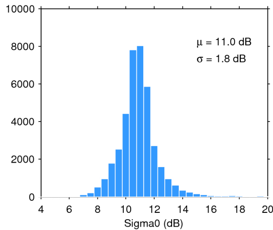
Figure 28. Histogram of science-valid sigma0 over oceans and lakes for 24/02/2017. The mean ( \mu ) and standard deviation ( \sigma ) are also shown. Note that values outside [4 20] dB are excluded from the histogram for the sake of readability but not from the computation of \mu and \sigma .
