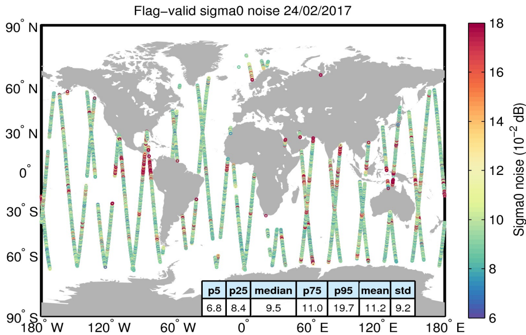
Figure 26. Geographical distribution of flag-valid 20-Hz sigma0 measurement noise over oceans and lakes for 24/02/2017. The statistical values shown in the table refer to the sigma0 noise and are calculated over all measurements shown in the figure.
