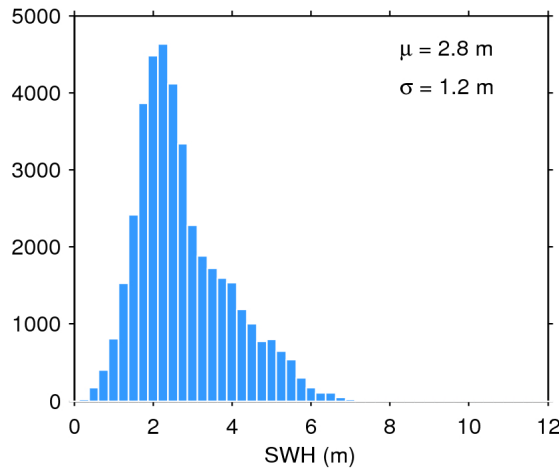
Figure 20. Histogram of science-valid SWH over oceans and lakes for 24/02/2017. The mean ( \mu ) and standard deviation ( \sigma ) are also shown. Note that values larger than 12 m are excluded from the histogram for the sake of readability but not from the computation of \mu and \sigma .
