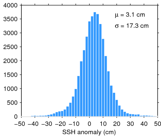
Figure 7. Histogram of flag-valid SSH anomaly over oceans and lakes for 24/02/2017. The mean ( \mu ) and standard deviation ( \sigma ) are also shown. Note that values outside [-50 50] cm are excluded from the histogram for the sake of readability but not from the computation of \mu and \sigma .
