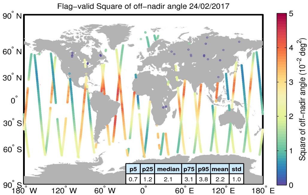
Figure 37. Geographical distribution of flag-valid mispointing data over oceans and lakes for 24/02/2017. The statistical values shown in the table refer to the mispointing in 10^{-2} deg 2 and are calculated over all measurements shown in the figure.
