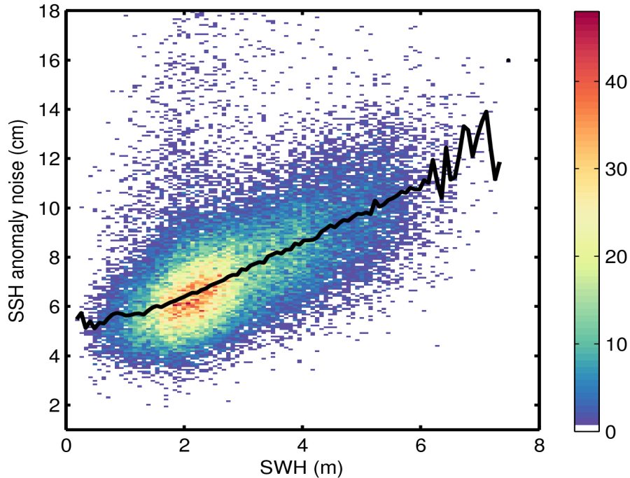
Figure 9. 2D histogram showing flag-valid SSH anomaly noise as a function of SWH for 24/02/2017. The black line denotes the median SSH anomaly noise as a function of SWH.
