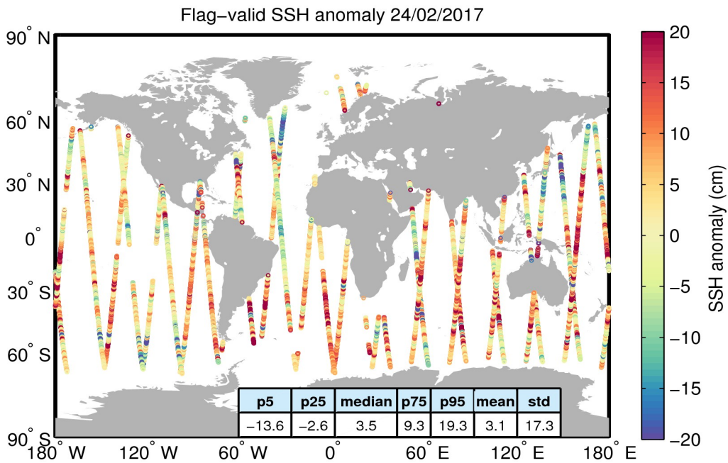
Figure 5. Geographical distribution of flag-valid 1-Hz SSH anomaly data over oceans and lakes for 24/02/2017. The statistical values shown in the table refer to the SSH anomaly in cm and are calculated over all measurements shown in the figure.
