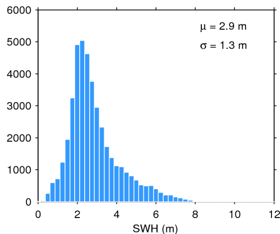
Figure 20. Histogram of science-valid SWH over oceans and lakes for 23/02/2017. The mean ( \mu ) and standard deviation ( \sigma ) are also shown. Note that values larger than 12 m are excluded from the histogram for the sake of readability but not from the computation of \mu and \sigma .
