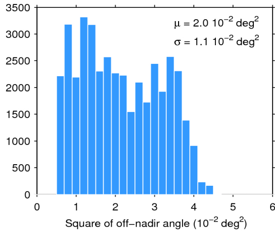
Figure 39. Histogram of flag-valid mispointing over oceans and lakes for 23/02/2017. The mean ( \mu ) and standard deviation ( \sigma ) are also shown. Note that values larger than 6 \cdot 10^{-2} \text{ deg}^2 are excluded from the histogram for the sake of readability but not from the computation of \mu and \sigma .
