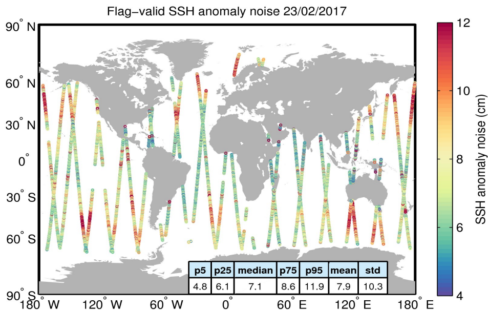
Figure 8. Geographical distribution of flag-valid 20-Hz SSH anomaly measurement noise over oceans and lakes for 23/02/2017. The statistical values shown in the table refer to the SSH anomaly noise and are calculated over all measurements shown in the figure.
