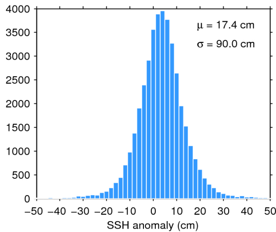
Figure 7. Histogram of flag-valid SSH anomaly over oceans and lakes for 23/02/2017. The mean ( \mu ) and standard deviation ( \sigma ) are also shown. Note that values outside [-50 50] cm are excluded from the histogram for the sake of readability but not from the computation of \mu and \sigma .
