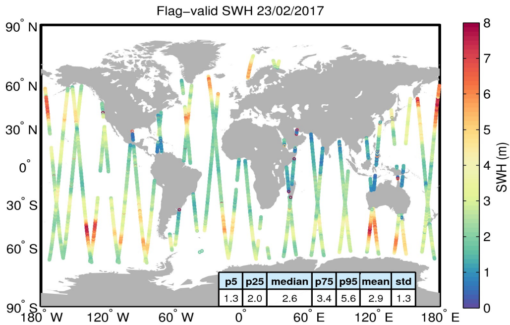
Figure 15. Geographical distribution of flag-valid SWH data over oceans and lakes for 23/02/2017. The statistical values shown in the table refer to the SWH in m and are calculated over all measurements shown in the figure.
