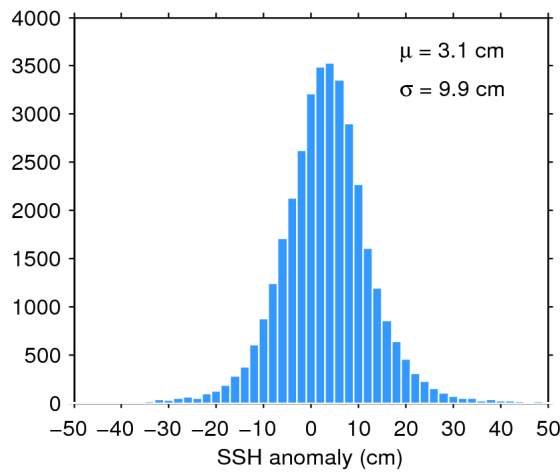
Figure 11. Histogram of science-valid SSH anomaly over oceans and lakes for 23/02/2017. The mean ( \mu ) and standard deviation ( \sigma ) are also shown. Note that values outside [-50 50] cm are excluded from the histogram for the sake of readability but not from the computation of \mu and \sigma .
