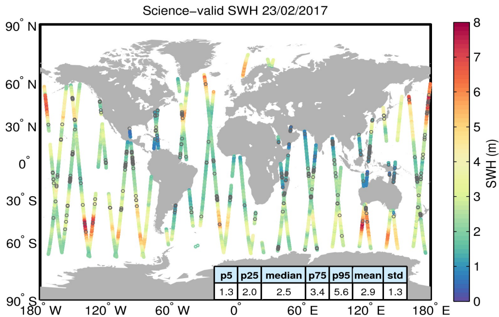
Figure 19. Geographical distribution of science-valid SWH data over oceans and lakes for 23/02/2017. The statistical values shown in the table refer to the SWH in m and are calculated over all measurements shown in the figure. Gray circles denote records that have been rejected based on the editing criteria described in Table 3.
