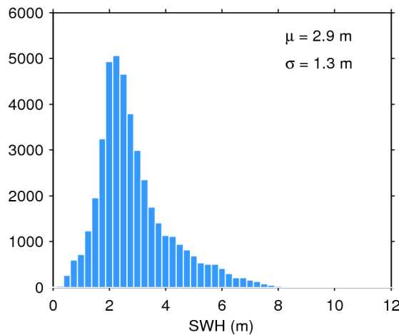
Figure 17. Histogram of flag-valid SWH over oceans and lakes for 23/02/2017. The mean ( \mu ) and standard deviation ( \sigma ) are also shown. Note that values larger than 12 m are excluded from the histogram for the sake of readability but not from the computation of \mu and \sigma .
