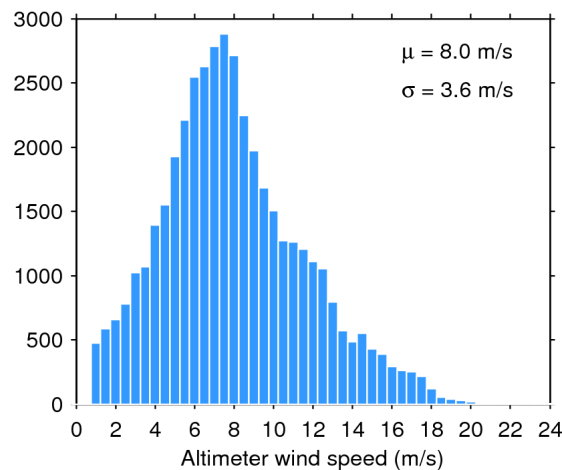
Figure 35. Histogram of science-valid wind over oceans and lakes for 23/02/2017. The mean ( \mu ) and standard deviation ( \sigma ) are also shown. Note that values larger than 24 m/s are excluded from the histogram for the sake of readability but not from the computation of \mu and \sigma .
