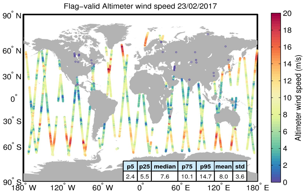
Figure 31. Geographical distribution of flag-valid wind data over oceans and lakes for 23/02/2017. The statistical values shown in the table refer to the wind in m/s and are calculated over all measurements shown in the figure.
