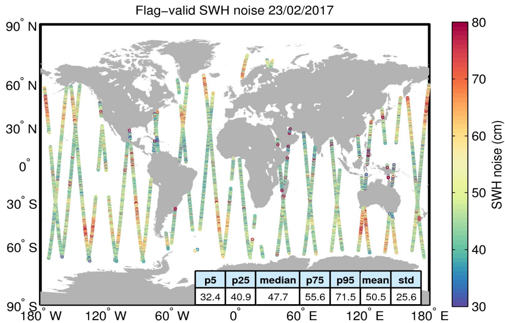
Figure 18. Geographical distribution of flag-valid 20-Hz SWH measurement noise over oceans and lakes for 23/02/2017. The statistical values shown in the table refer to the SWH noise and are calculated over all measurements shown in the figure.
