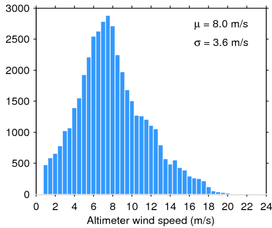
Figure 33. Histogram of flag-valid wind over oceans and lakes for 23/02/2017. The mean ( \mu ) and standard deviation ( \sigma ) are also shown. Note that values larger than 24 m/s are excluded from the histogram for the sake of readability but not from the computation of \mu and \sigma .
