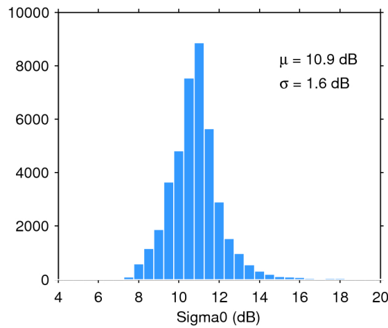
Figure 28. Histogram of science-valid sigma0 over oceans and lakes for 23/02/2017. The mean ( \mu ) and standard deviation ( \sigma ) are also shown. Note that values outside [4 20] dB are excluded from the histogram for the sake of readability but not from the computation of \mu and \sigma .
