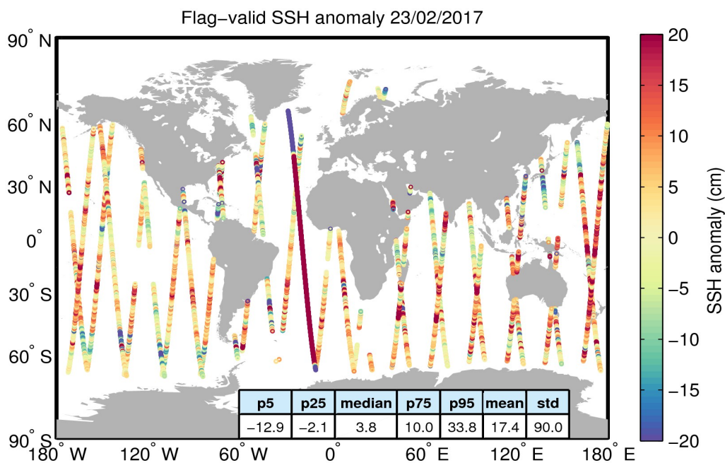
Figure 5. Geographical distribution of flag-valid 1-Hz SSH anomaly data over oceans and lakes for 23/02/2017. The statistical values shown in the table refer to the SSH anomaly in cm and are calculated over all measurements shown in the figure.
