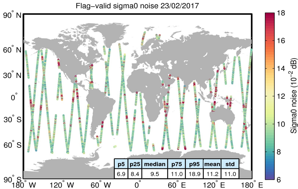
Figure 26. Geographical distribution of flag-valid 20-Hz sigma0 measurement noise over oceans and lakes for 23/02/2017. The statistical values shown in the table refer to the sigma0 noise and are calculated over all measurements shown in the figure.
