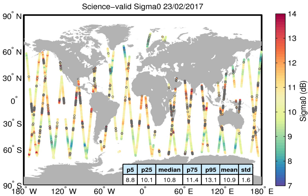
Figure 27. Geographical distribution of science-valid sigma0 data over oceans and lakes for 23/02/2017. The statistical values shown in the table refer to the sigma0 in dB and are calculated over all measurements shown in the figure. Gray circles denote records that have been rejected based on the editing criteria described in Table 4.
