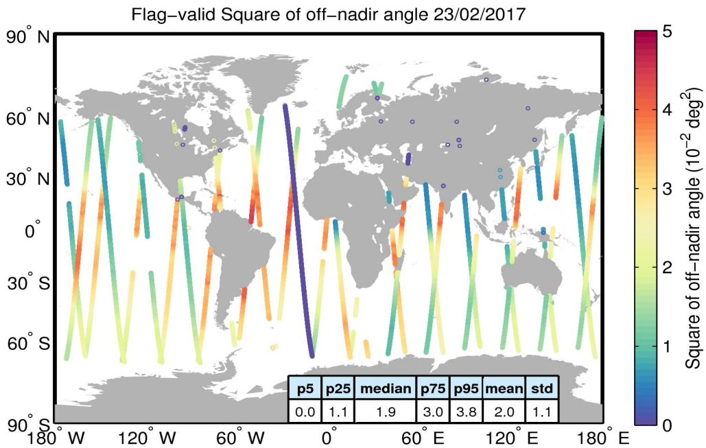
Figure 37. Geographical distribution of flag-valid mispointing data over oceans and lakes for 23/02/2017. The statistical values shown in the table refer to the mispointing in 10^{-2} deg 2 and are calculated over all measurements shown in the figure.
