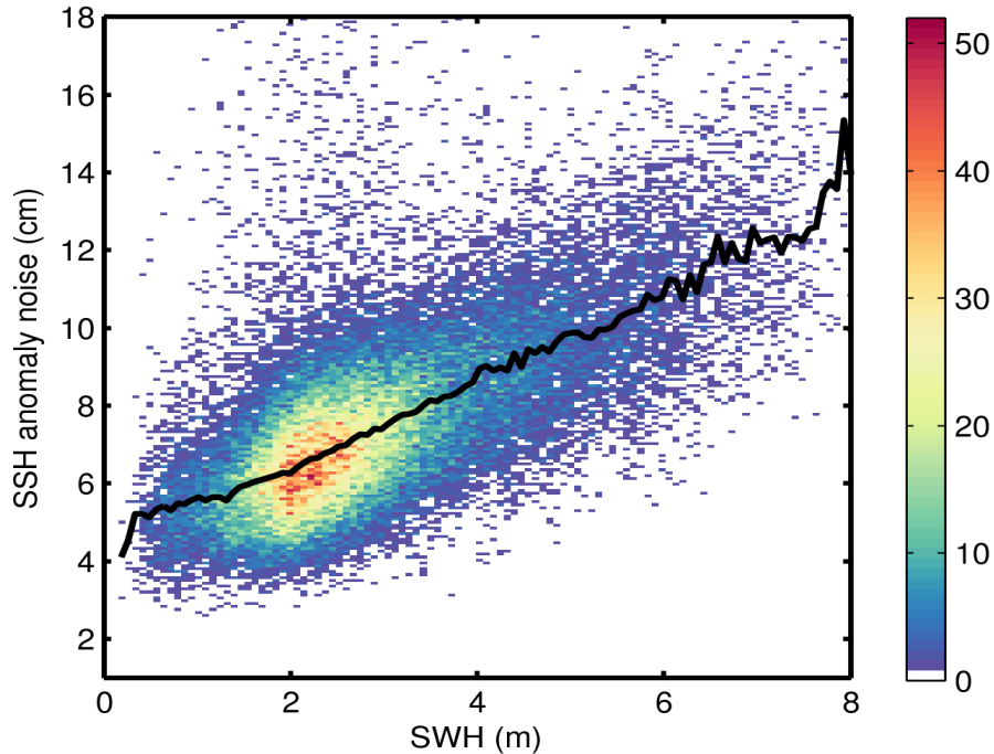
Figure 9. 2D histogram showing flag-valid SSH anomaly noise as a function of SWH for 23/02/2017. The black line denotes the median SSH anomaly noise as a function of SWH.
