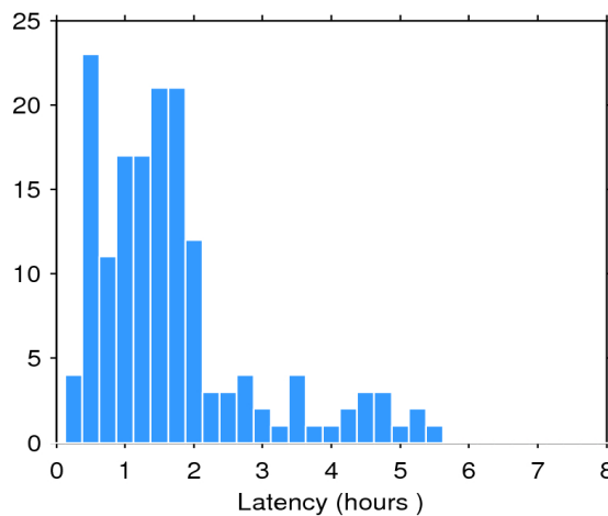
Figure 2. Histogram of the data latency for 23/02/2017. The y-axis denotes the number of files that are made available with a delay of x-hours with respect to the mean time of the records stored in the file.
