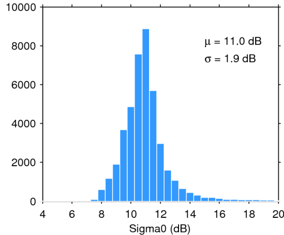
Figure 25. Histogram of flag-valid sigma0 over oceans and lakes for 23/02/2017. The mean ( \mu ) and standard deviation ( \sigma ) are also shown. Note that values outside [4 20] dB are excluded from the histogram for the sake of readability but not from the computation of \mu and \sigma .
