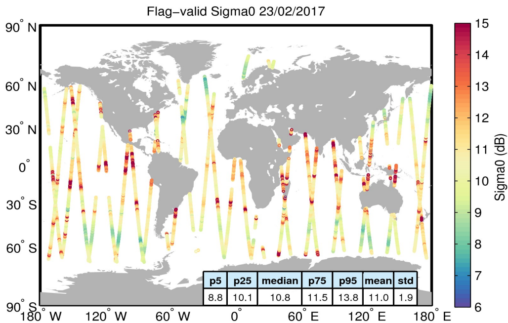
Figure 23. Geographical distribution of flag-valid sigma0 data over oceans and lakes for 23/02/2017. The statistical values shown in the table refer to the sigma0 in dB and are calculated over all measurements shown in the figure.
