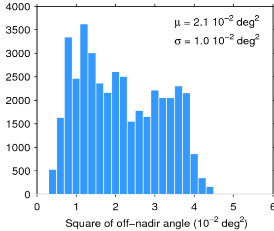
Figure 39. Histogram of flag-valid mispointing over oceans and lakes for 22/02/2017. The mean ( \mu ) and standard deviation ( \sigma ) are also shown. Note that values larger than 6 \cdot 10^{-2} \text{ deg}^2 are excluded from the histogram for the sake of readability but not from the computation of \mu and \sigma .
