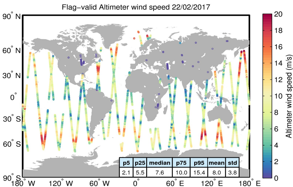
Figure 31. Geographical distribution of flag-valid wind data over oceans and lakes for 22/02/2017. The statistical values shown in the table refer to the wind in m/s and are calculated over all measurements shown in the figure.
