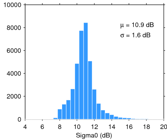
Figure 28. Histogram of science-valid sigma0 over oceans and lakes for 22/02/2017. The mean ( \mu ) and standard deviation ( \sigma ) are also shown. Note that values outside [4 20] dB are excluded from the histogram for the sake of readability but not from the computation of \mu and \sigma .
