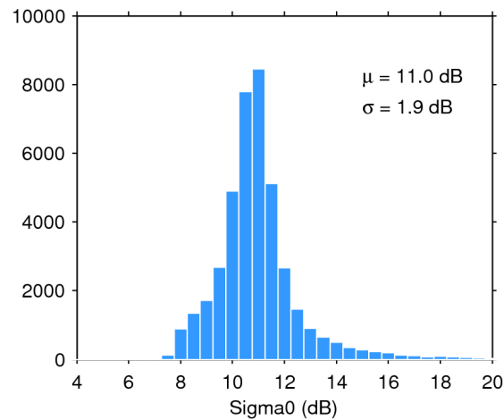
Figure 25. Histogram of flag-valid sigma0 over oceans and lakes for 22/02/2017. The mean ( \mu ) and standard deviation ( \sigma ) are also shown. Note that values outside [4 20] dB are excluded from the histogram for the sake of readability but not from the computation of \mu and \sigma .
