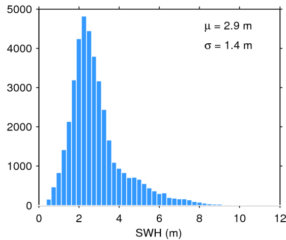
Figure 17. Histogram of flag-valid SWH over oceans and lakes for 22/02/2017. The mean ( \mu ) and standard deviation ( \sigma ) are also shown. Note that values larger than 12 m are excluded from the histogram for the sake of readability but not from the computation of \mu and \sigma .
