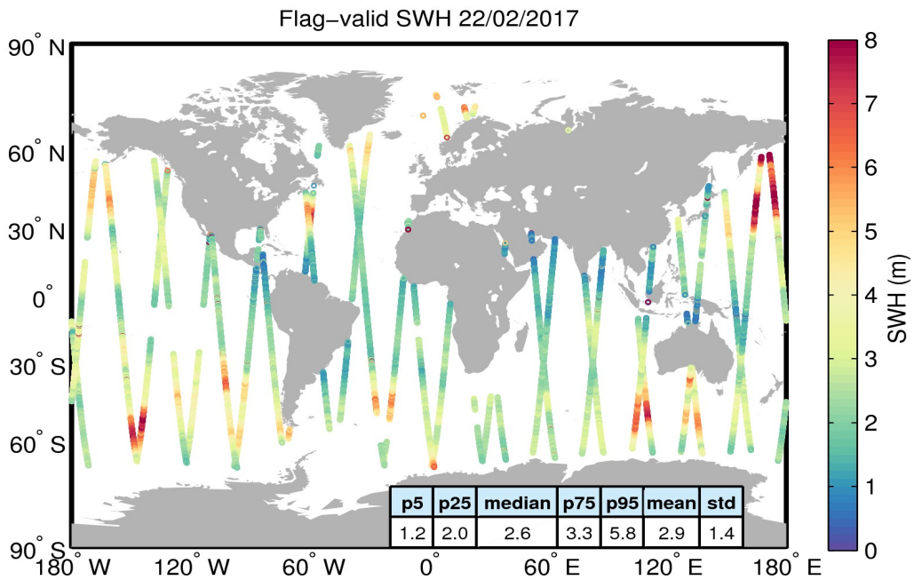
Figure 15. Geographical distribution of flag-valid SWH data over oceans and lakes for 22/02/2017. The statistical values shown in the table refer to the SWH in m and are calculated over all measurements shown in the figure.
