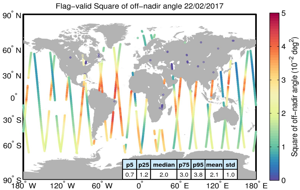
Figure 37. Geographical distribution of flag-valid mispointing data over oceans and lakes for 22/02/2017. The statistical values shown in the table refer to the mispointing in 10^{-2} deg 2 and are calculated over all measurements shown in the figure.
