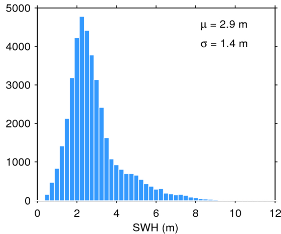
Figure 20. Histogram of science-valid SWH over oceans and lakes for 22/02/2017. The mean ( \mu ) and standard deviation ( \sigma ) are also shown. Note that values larger than 12 m are excluded from the histogram for the sake of readability but not from the computation of \mu and \sigma .
