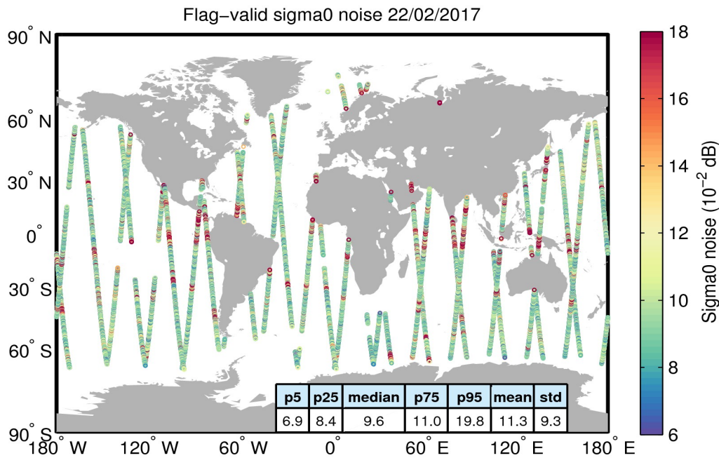
Figure 26. Geographical distribution of flag-valid 20-Hz sigma0 measurement noise over oceans and lakes for 22/02/2017. The statistical values shown in the table refer to the sigma0 noise and are calculated over all measurements shown in the figure.
