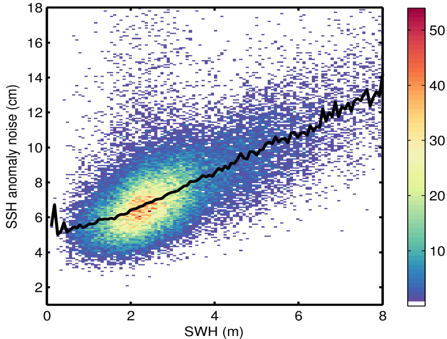
Figure 9. 2D histogram showing flag-valid SSH anomaly noise as a function of SWH for 22/02/2017. The black line denotes the median SSH anomaly noise as a function of SWH.
