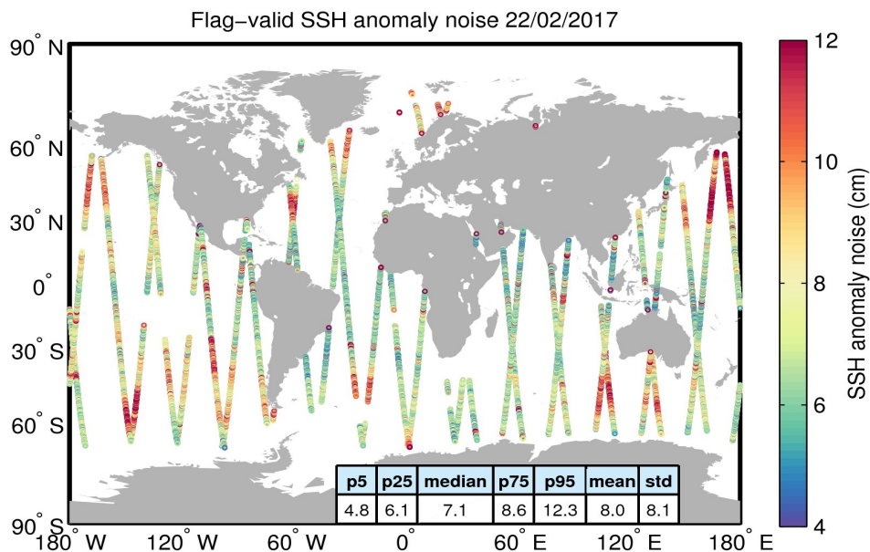
Figure 8. Geographical distribution of flag-valid 20-Hz SSH anomaly measurement noise over oceans and lakes for 22/02/2017. The statistical values shown in the table refer to the SSH anomaly noise and are calculated over all measurements shown in the figure.
