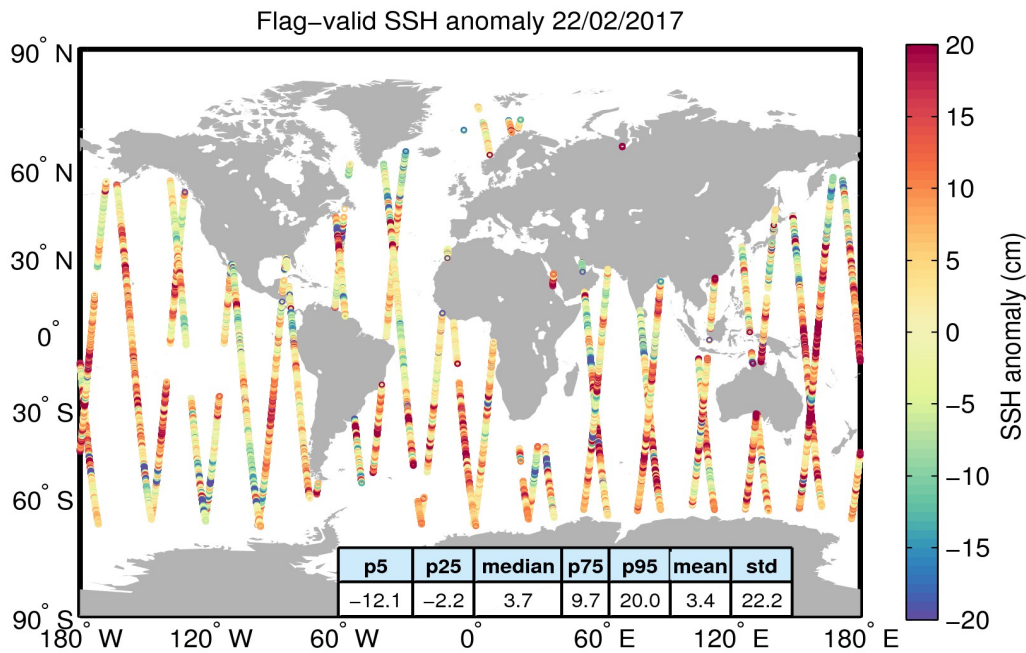
Figure 5. Geographical distribution of flag-valid 1-Hz SSH anomaly data over oceans and lakes for 22/02/2017. The statistical values shown in the table refer to the SSH anomaly in cm and are calculated over all measurements shown in the figure.
