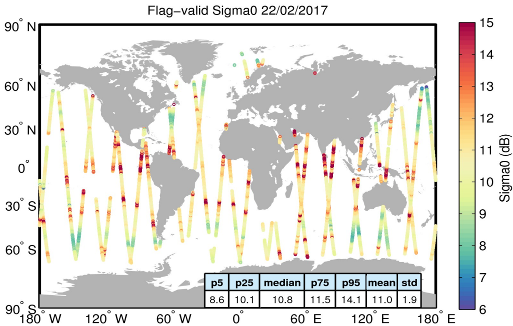
Figure 23. Geographical distribution of flag-valid sigma0 data over oceans and lakes for 22/02/2017. The statistical values shown in the table refer to the sigma0 in dB and are calculated over all measurements shown in the figure.
