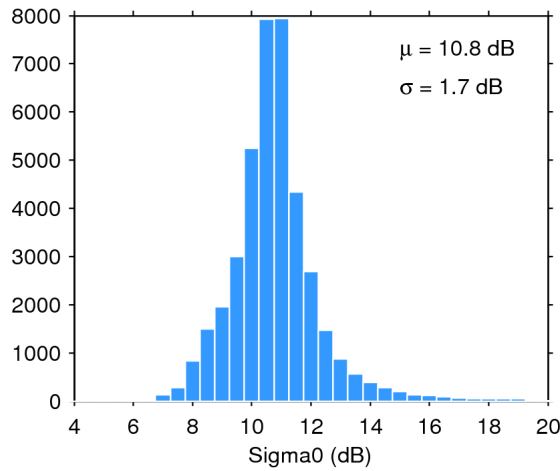
Figure 28. Histogram of science-valid sigma0 over oceans and lakes for 21/02/2017. The mean ( \mu ) and standard deviation ( \sigma ) are also shown. Note that values outside [4 20] dB are excluded from the histogram for the sake of readability but not from the computation of \mu and \sigma .
