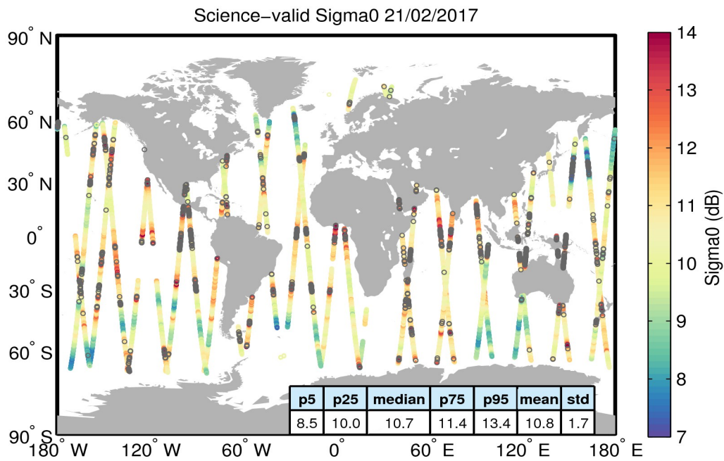
Figure 27. Geographical distribution of science-valid sigma0 data over oceans and lakes for 21/02/2017. The statistical values shown in the table refer to the sigma0 in dB and are calculated over all measurements shown in the figure. Gray circles denote records that have been rejected based on the editing criteria described in Table 4.
