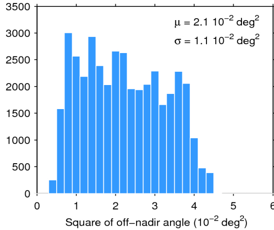
Figure 39. Histogram of flag-valid mispointing over oceans and lakes for 21/02/2017. The mean ( \mu ) and standard deviation ( \sigma ) are also shown. Note that values larger than 6 \cdot 10^{-2} \text{ deg}^2 are excluded from the histogram for the sake of readability but not from the computation of \mu and \sigma .
