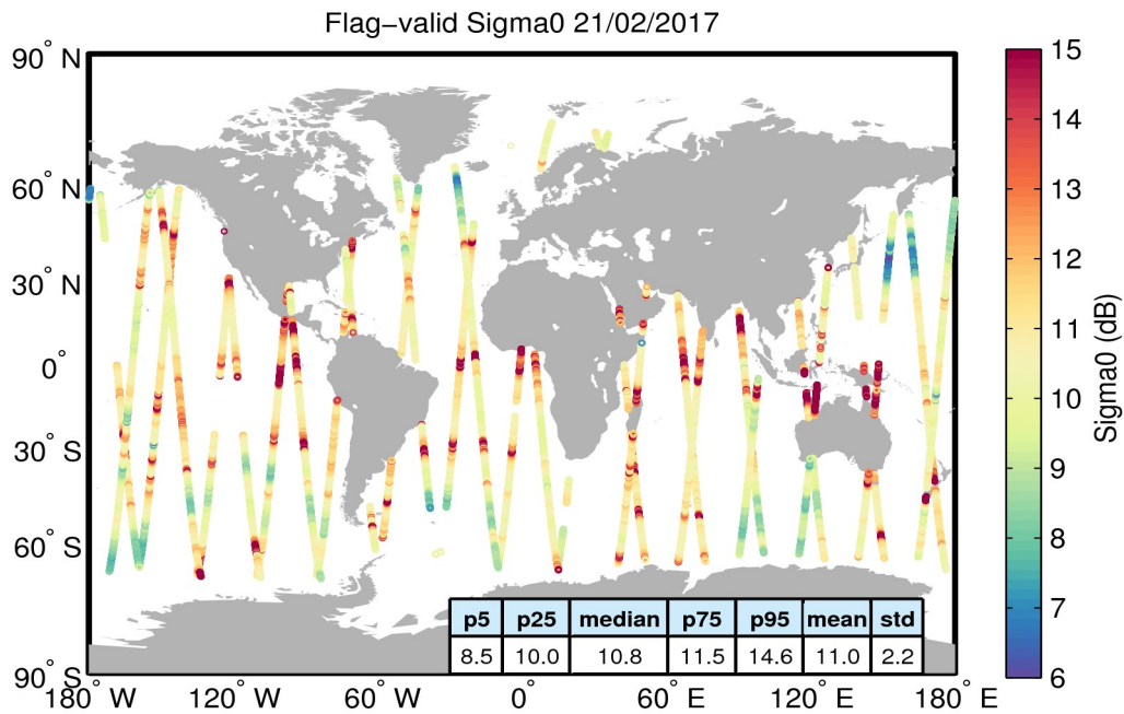
Figure 23. Geographical distribution of flag-valid sigma0 data over oceans and lakes for 21/02/2017. The statistical values shown in the table refer to the sigma0 in dB and are calculated over all measurements shown in the figure.
