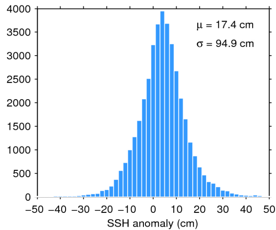
Figure 7. Histogram of flag-valid SSH anomaly over oceans and lakes for 21/02/2017. The mean ( \mu ) and standard deviation ( \sigma ) are also shown. Note that values outside [-50 50] cm are excluded from the histogram for the sake of readability but not from the computation of \mu and \sigma .
