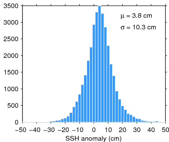
Figure 11. Histogram of science-valid SSH anomaly over oceans and lakes for 21/02/2017. The mean ( \mu ) and standard deviation ( \sigma ) are also shown. Note that values outside [-50 50] cm are excluded from the histogram for the sake of readability but not from the computation of \mu and \sigma .
