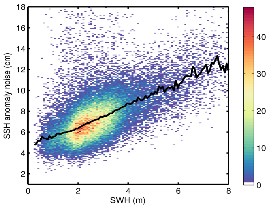
Figure 9. 2D histogram showing flag-valid SSH anomaly noise as a function of SWH for 21/02/2017. The black line denotes the median SSH anomaly noise as a function of SWH.
