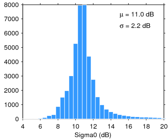
Figure 25. Histogram of flag-valid sigma0 over oceans and lakes for 21/02/2017. The mean ( \mu ) and standard deviation ( \sigma ) are also shown. Note that values outside [4 20] dB are excluded from the histogram for the sake of readability but not from the computation of \mu and \sigma .
