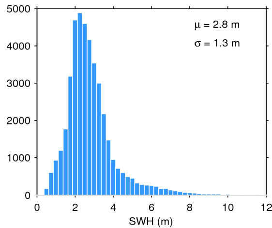
Figure 17. Histogram of flag-valid SWH over oceans and lakes for 21/02/2017. The mean ( \mu ) and standard deviation ( \sigma ) are also shown. Note that values larger than 12 m are excluded from the histogram for the sake of readability but not from the computation of \mu and \sigma .
