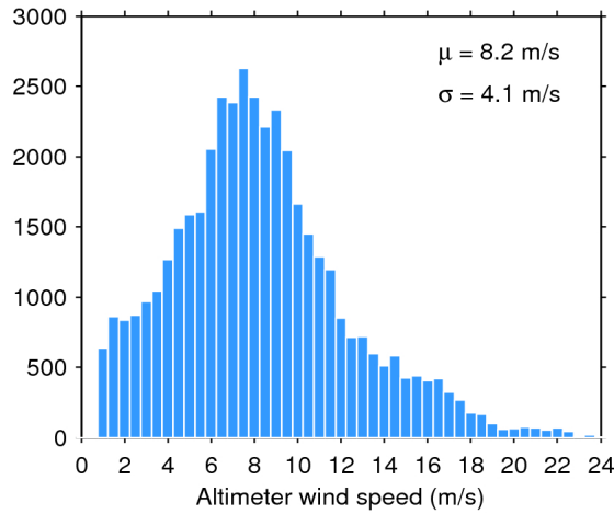
Figure 33. Histogram of flag-valid wind over oceans and lakes for 21/02/2017. The mean ( \mu ) and standard deviation ( \sigma ) are also shown. Note that values larger than 24 m/s are excluded from the histogram for the sake of readability but not from the computation of \mu and \sigma .
