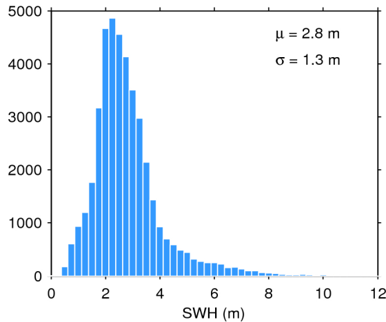
Figure 20. Histogram of science-valid SWH over oceans and lakes for 21/02/2017. The mean ( \mu ) and standard deviation ( \sigma ) are also shown. Note that values larger than 12 m are excluded from the histogram for the sake of readability but not from the computation of \mu and \sigma .
