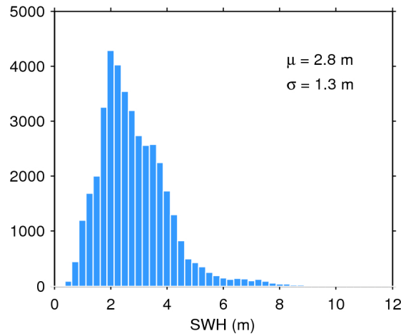
Figure 17. Histogram of flag-valid SWH over oceans and lakes for 20/02/2017. The mean ( \mu ) and standard deviation ( \sigma ) are also shown. Note that values larger than 12 m are excluded from the histogram for the sake of readability but not from the computation of \mu and \sigma .
