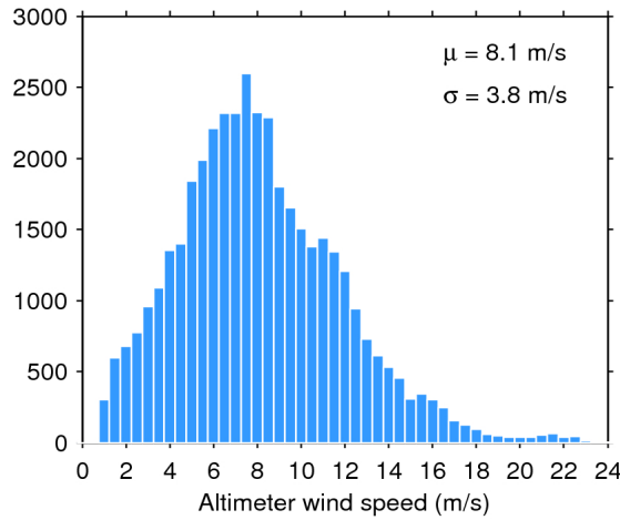
Figure 33. Histogram of flag-valid wind over oceans and lakes for 20/02/2017. The mean ( \mu ) and standard deviation ( \sigma ) are also shown. Note that values larger than 24 m/s are excluded from the histogram for the sake of readability but not from the computation of \mu and \sigma .
