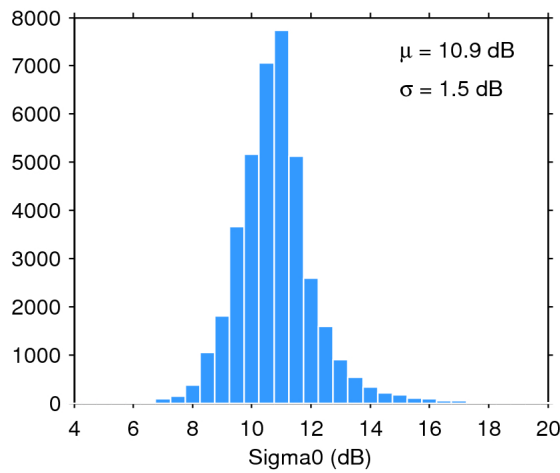
Figure 28. Histogram of science-valid sigma0 over oceans and lakes for 20/02/2017. The mean ( \mu ) and standard deviation ( \sigma ) are also shown. Note that values outside [4 20] dB are excluded from the histogram for the sake of readability but not from the computation of \mu and \sigma .
