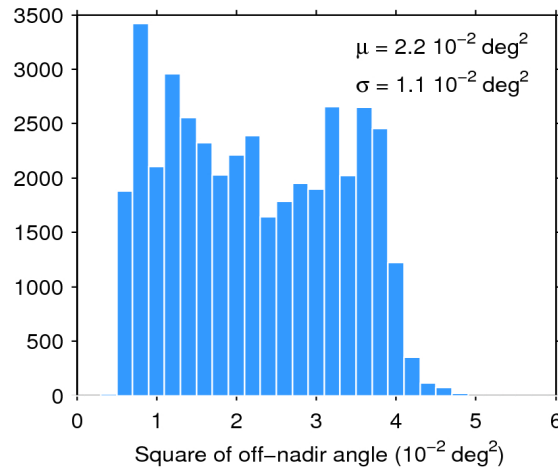
Figure 39. Histogram of flag-valid mispointing over oceans and lakes for 20/02/2017. The mean ( \mu ) and standard deviation ( \sigma ) are also shown. Note that values larger than 6 \cdot 10^{-2} \text{ deg}^2 are excluded from the histogram for the sake of readability but not from the computation of \mu and \sigma .
