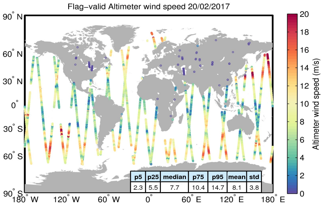
Figure 31. Geographical distribution of flag-valid wind data over oceans and lakes for 20/02/2017. The statistical values shown in the table refer to the wind in m/s and are calculated over all measurements shown in the figure.
