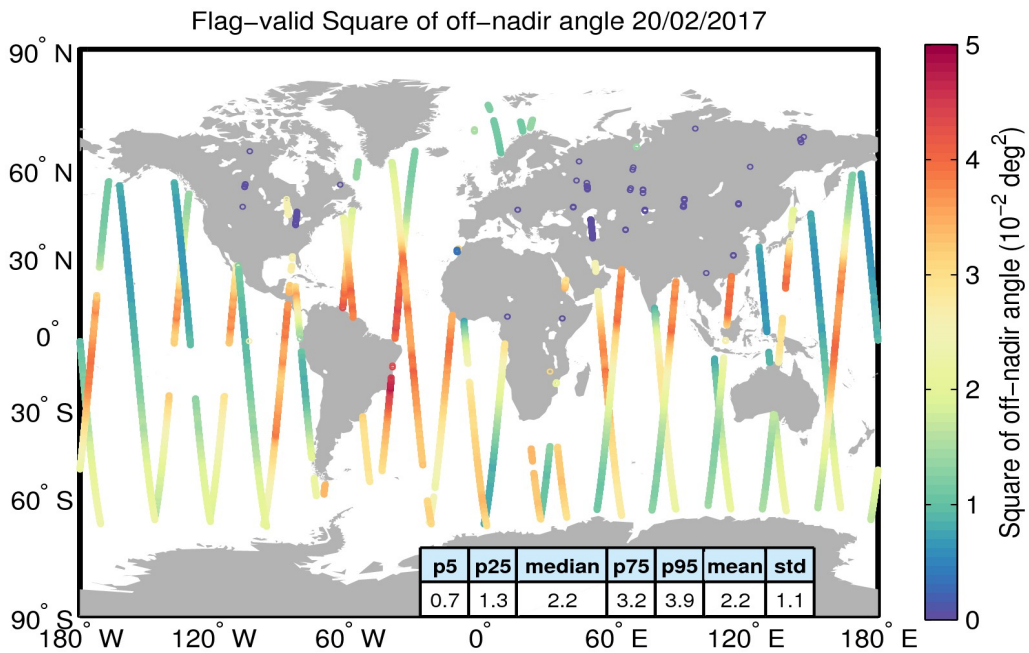
Figure 37. Geographical distribution of flag-valid mispointing data over oceans and lakes for 20/02/2017. The statistical values shown in the table refer to the mispointing in 10^{-2} deg 2 and are calculated over all measurements shown in the figure.
