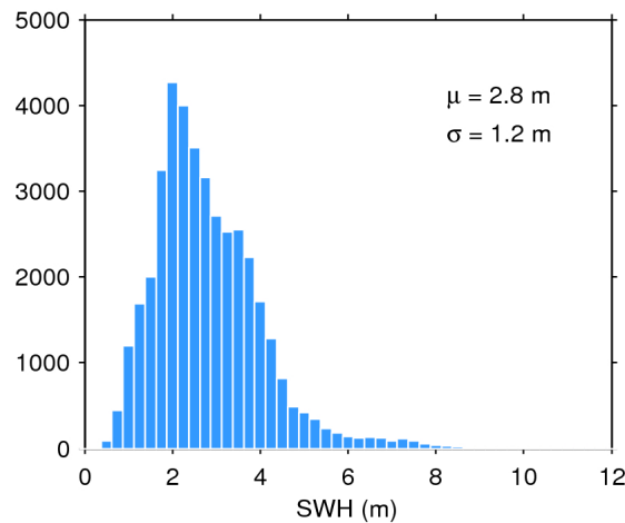
Figure 20. Histogram of science-valid SWH over oceans and lakes for 20/02/2017. The mean ( \mu ) and standard deviation ( \sigma ) are also shown. Note that values larger than 12 m are excluded from the histogram for the sake of readability but not from the computation of \mu and \sigma .
