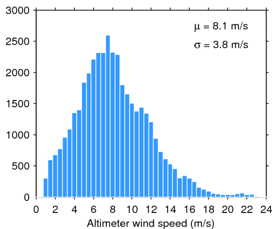
Figure 35. Histogram of science-valid wind over oceans and lakes for 20/02/2017. The mean ( \mu ) and standard deviation ( \sigma ) are also shown. Note that values larger than 24 m/s are excluded from the histogram for the sake of readability but not from the computation of \mu and \sigma .
