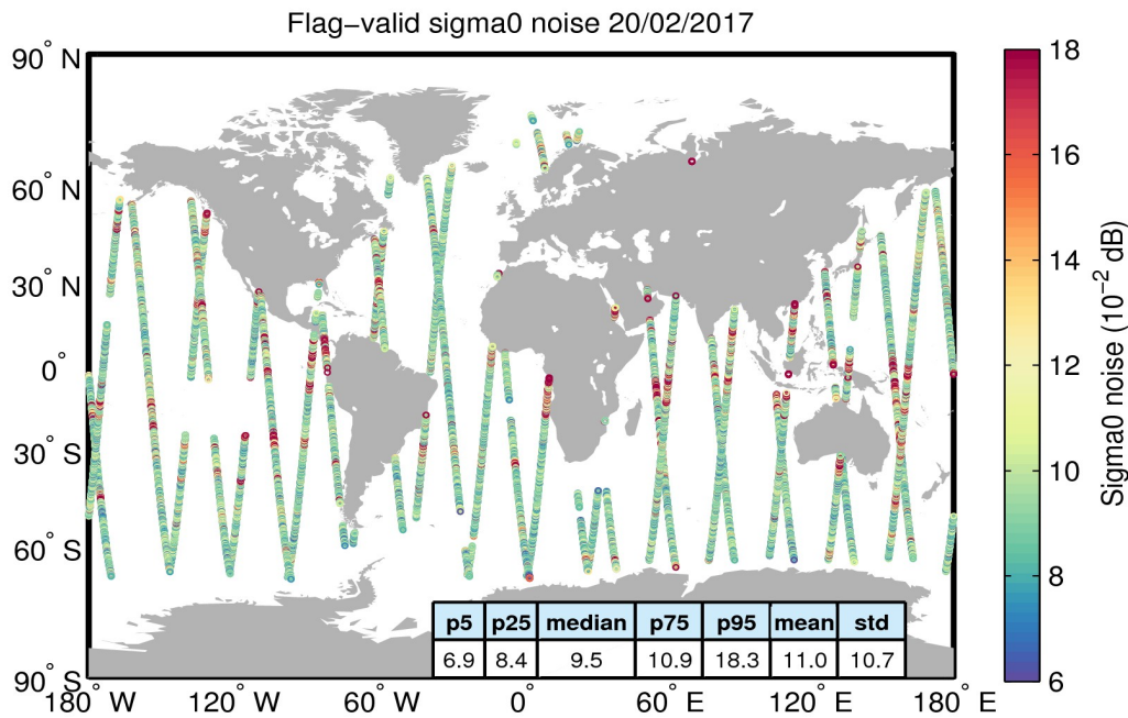
Figure 26. Geographical distribution of flag-valid 20-Hz sigma0 measurement noise over oceans and lakes for 20/02/2017. The statistical values shown in the table refer to the sigma0 noise and are calculated over all measurements shown in the figure.
