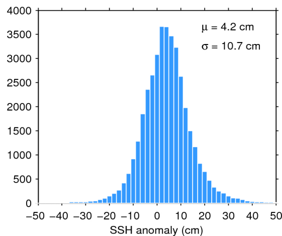
Figure 11. Histogram of science-valid SSH anomaly over oceans and lakes for 20/02/2017. The mean ( \mu ) and standard deviation ( \sigma ) are also shown. Note that values outside [-50 50] cm are excluded from the histogram for the sake of readability but not from the computation of \mu and \sigma .
