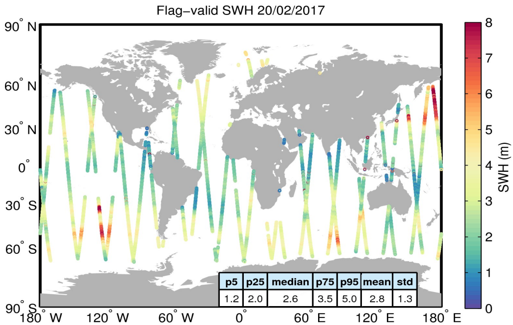
Figure 15. Geographical distribution of flag-valid SWH data over oceans and lakes for 20/02/2017. The statistical values shown in the table refer to the SWH in m and are calculated over all measurements shown in the figure.
