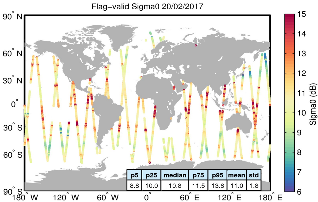
Figure 23. Geographical distribution of flag-valid sigma0 data over oceans and lakes for 20/02/2017. The statistical values shown in the table refer to the sigma0 in dB and are calculated over all measurements shown in the figure.
