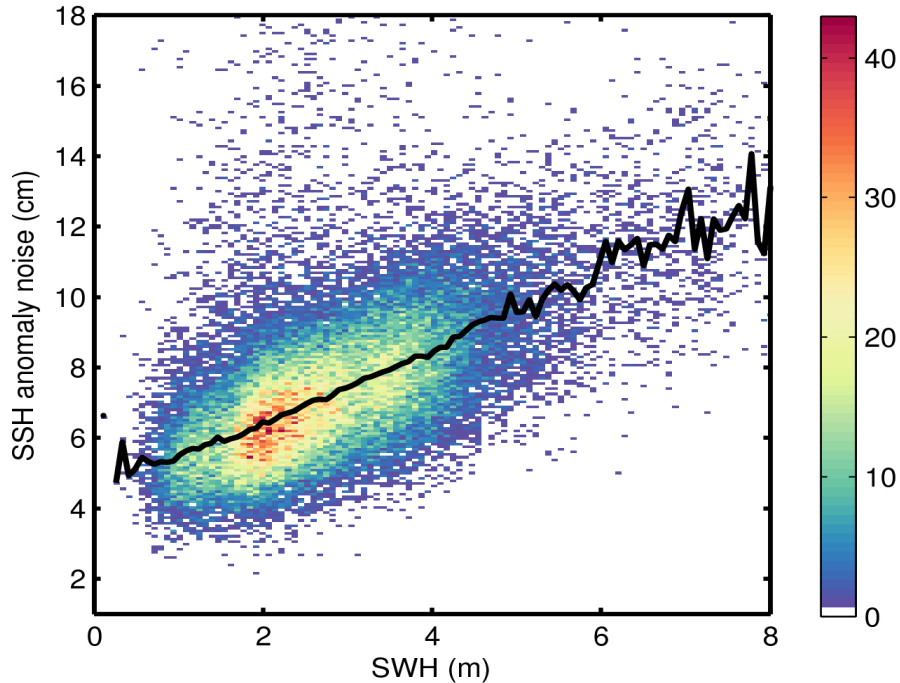
Figure 9. 2D histogram showing flag-valid SSH anomaly noise as a function of SWH for 20/02/2017. The black line denotes the median SSH anomaly noise as a function of SWH.
