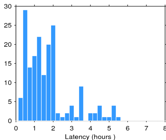
Figure 2. Histogram of the data latency for 20/02/2017. The y-axis denotes the number of files that are made available with a delay of x-hours with respect to the mean time of the records stored in the file.
