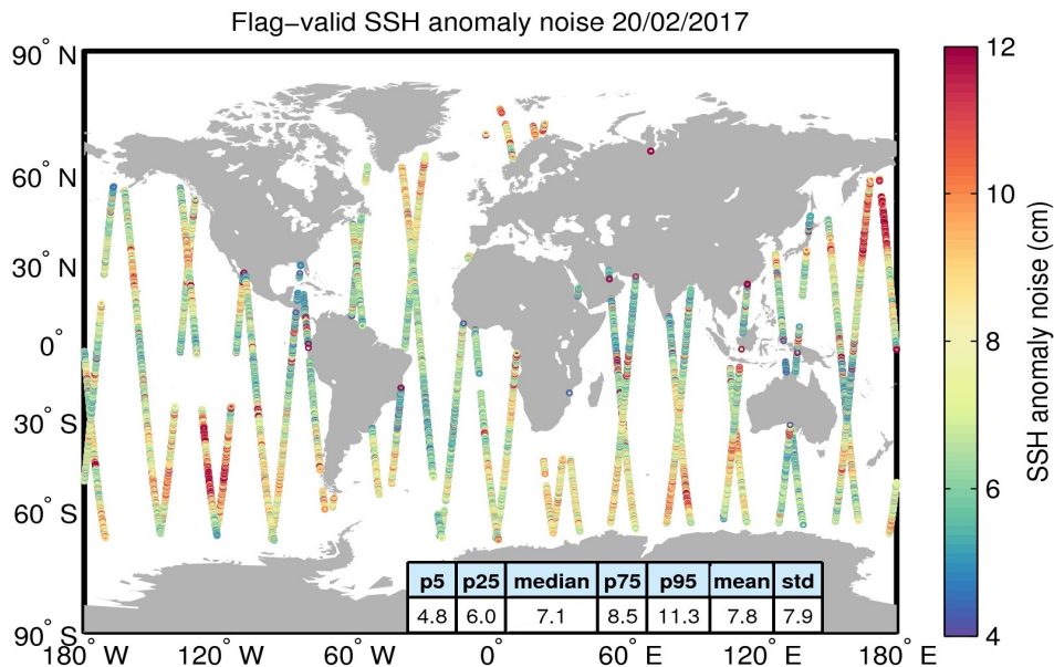
Figure 8. Geographical distribution of flag-valid 20-Hz SSH anomaly measurement noise over oceans and lakes for 20/02/2017. The statistical values shown in the table refer to the SSH anomaly noise and are calculated over all measurements shown in the figure.
