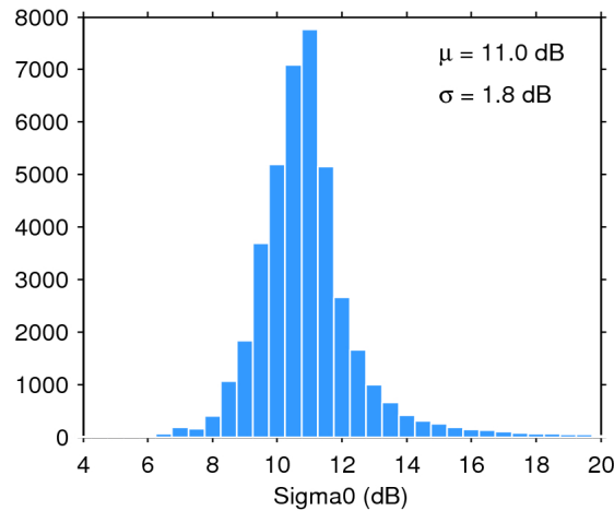
Figure 25. Histogram of flag-valid sigma0 over oceans and lakes for 20/02/2017. The mean ( \mu ) and standard deviation ( \sigma ) are also shown. Note that values outside [4 20] dB are excluded from the histogram for the sake of readability but not from the computation of \mu and \sigma .
