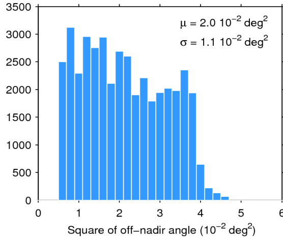
Figure 39. Histogram of flag-valid mispointing over oceans and lakes for 19/02/2017. The mean ( \mu ) and standard deviation ( \sigma ) are also shown. Note that values larger than 6 \cdot 10^{-2} \text{ deg}^2 are excluded from the histogram for the sake of readability but not from the computation of \mu and \sigma .
