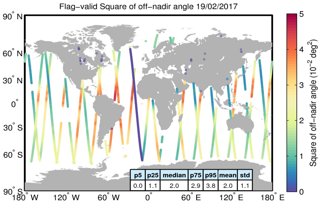
Figure 37. Geographical distribution of flag-valid mispointing data over oceans and lakes for 19/02/2017. The statistical values shown in the table refer to the mispointing in 10^{-2} deg 2 and are calculated over all measurements shown in the figure.
