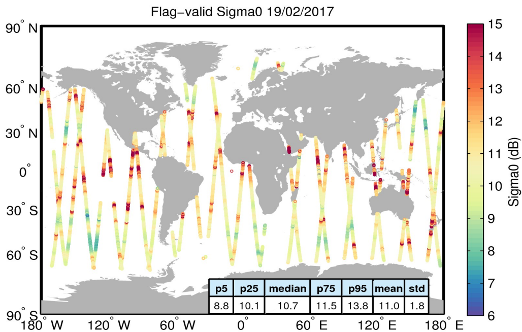
Figure 23. Geographical distribution of flag-valid sigma0 data over oceans and lakes for 19/02/2017. The statistical values shown in the table refer to the sigma0 in dB and are calculated over all measurements shown in the figure.
