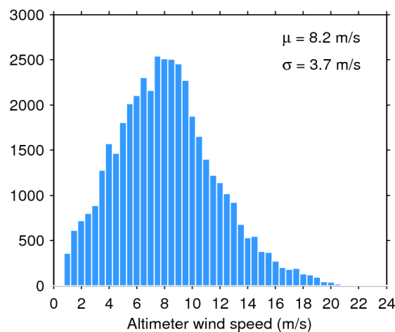
Figure 35. Histogram of science-valid wind over oceans and lakes for 19/02/2017. The mean ( \mu ) and standard deviation ( \sigma ) are also shown. Note that values larger than 24 m/s are excluded from the histogram for the sake of readability but not from the computation of \mu and \sigma .
