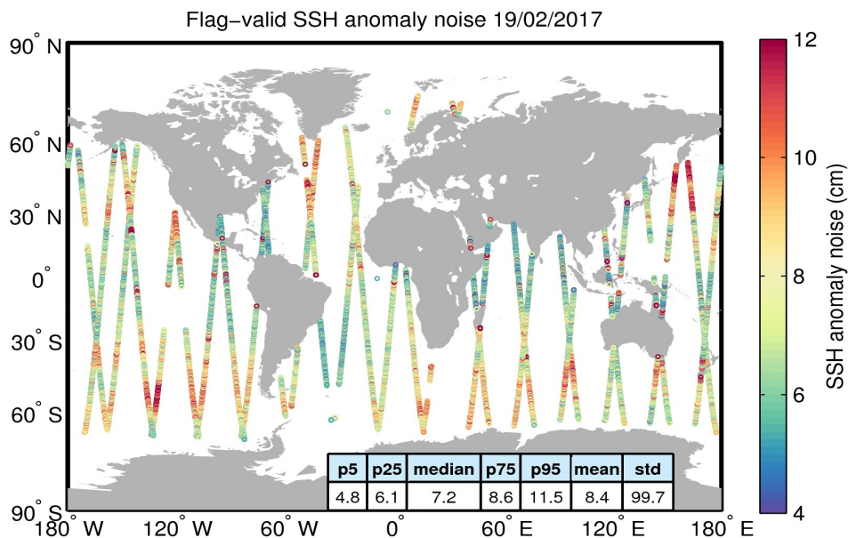
Figure 8. Geographical distribution of flag-valid 20-Hz SSH anomaly measurement noise over oceans and lakes for 19/02/2017. The statistical values shown in the table refer to the SSH anomaly noise and are calculated over all measurements shown in the figure.
