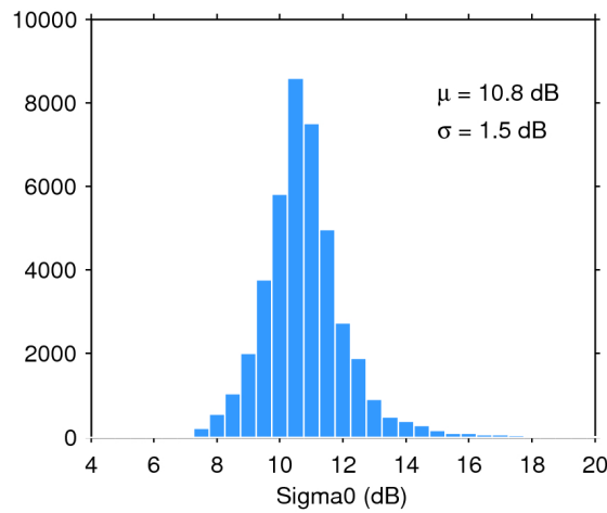
Figure 28. Histogram of science-valid sigma0 over oceans and lakes for 19/02/2017. The mean ( \mu ) and standard deviation ( \sigma ) are also shown. Note that values outside [4 20] dB are excluded from the histogram for the sake of readability but not from the computation of \mu and \sigma .
