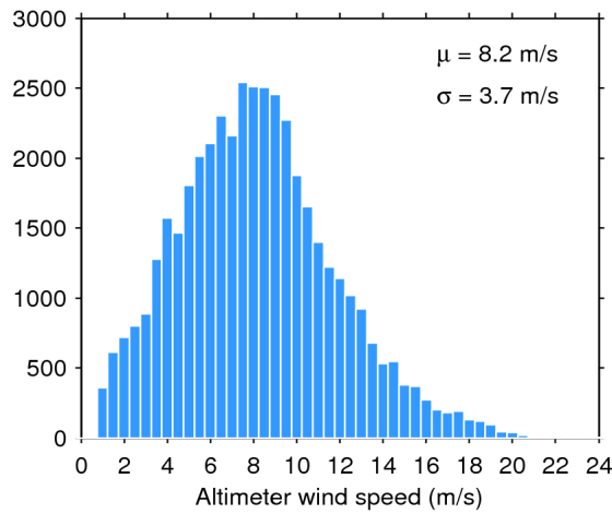
Figure 33. Histogram of flag-valid wind over oceans and lakes for 19/02/2017. The mean ( \mu ) and standard deviation ( \sigma ) are also shown. Note that values larger than 24 m/s are excluded from the histogram for the sake of readability but not from the computation of \mu and \sigma .
