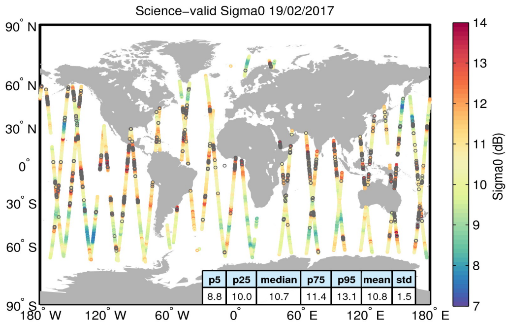
Figure 27. Geographical distribution of science-valid sigma0 data over oceans and lakes for 19/02/2017. The statistical values shown in the table refer to the sigma0 in dB and are calculated over all measurements shown in the figure. Gray circles denote records that have been rejected based on the editing criteria described in Table 4.
