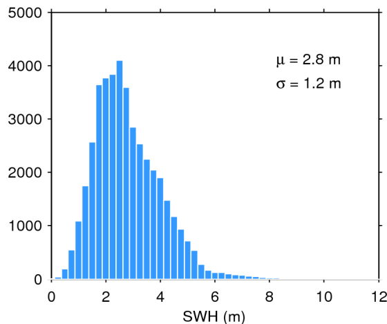
Figure 20. Histogram of science-valid SWH over oceans and lakes for 19/02/2017. The mean ( \mu ) and standard deviation ( \sigma ) are also shown. Note that values larger than 12 m are excluded from the histogram for the sake of readability but not from the computation of \mu and \sigma .
