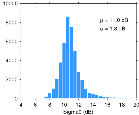
Figure 25. Histogram of flag-valid sigma0 over oceans and lakes for 19/02/2017. The mean ( \mu ) and standard deviation ( \sigma ) are also shown. Note that values outside [4 20] dB are excluded from the histogram for the sake of readability but not from the computation of \mu and \sigma .
