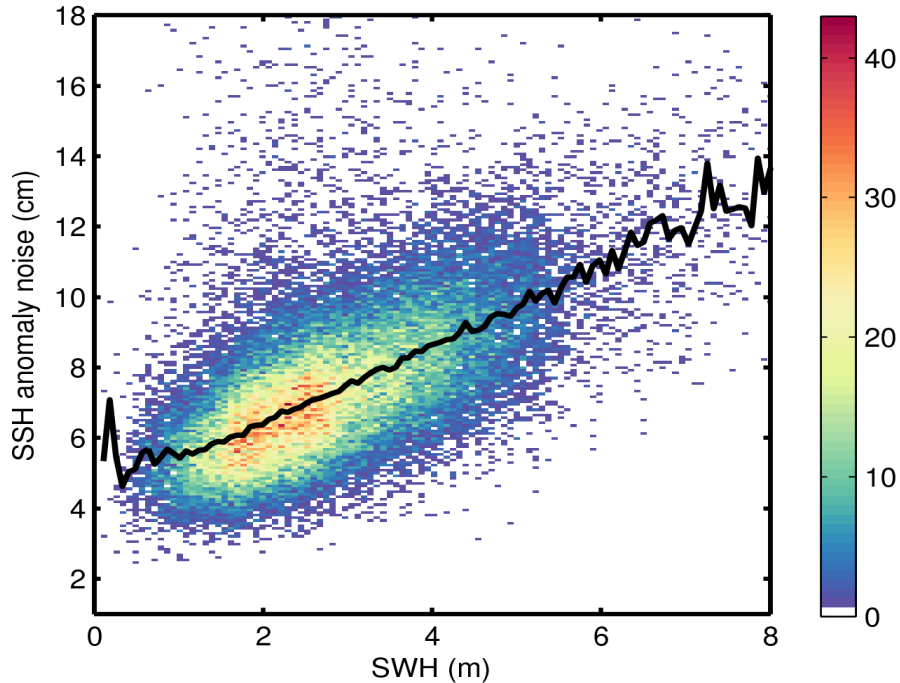
Figure 9. 2D histogram showing flag-valid SSH anomaly noise as a function of SWH for 19/02/2017. The black line denotes the median SSH anomaly noise as a function of SWH.
