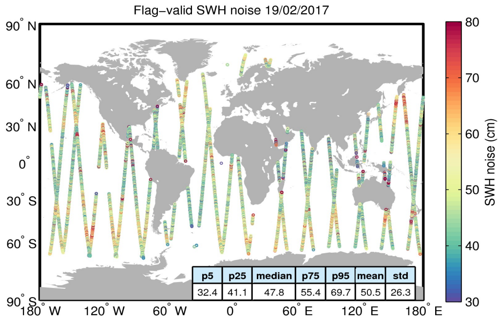
Figure 18. Geographical distribution of flag-valid 20-Hz SWH measurement noise over oceans and lakes for 19/02/2017. The statistical values shown in the table refer to the SWH noise and are calculated over all measurements shown in the figure.
