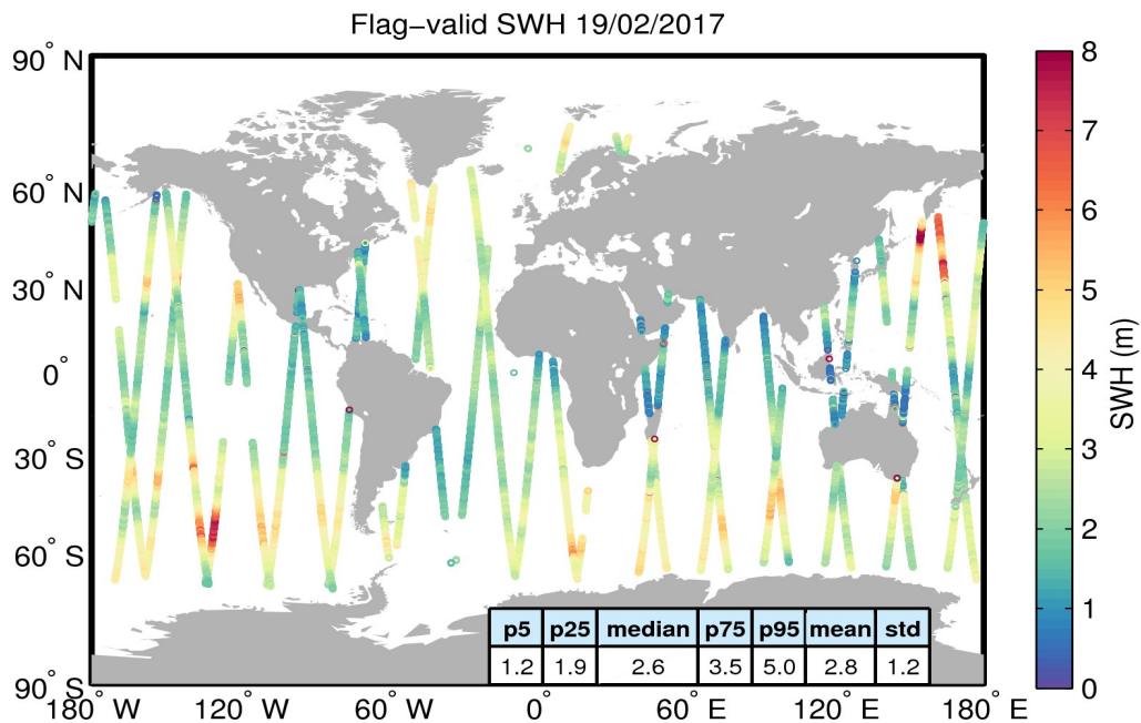
Figure 15. Geographical distribution of flag-valid SWH data over oceans and lakes for 19/02/2017. The statistical values shown in the table refer to the SWH in m and are calculated over all measurements shown in the figure.
