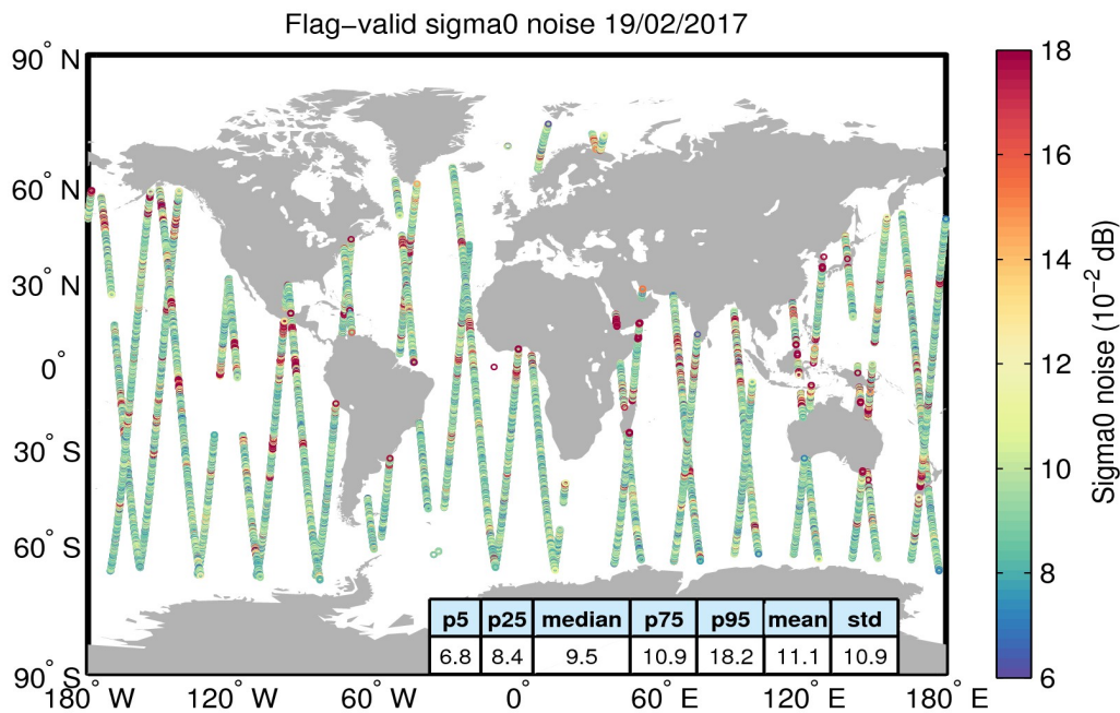
Figure 26. Geographical distribution of flag-valid 20-Hz sigma0 measurement noise over oceans and lakes for 19/02/2017. The statistical values shown in the table refer to the sigma0 noise and are calculated over all measurements shown in the figure.
