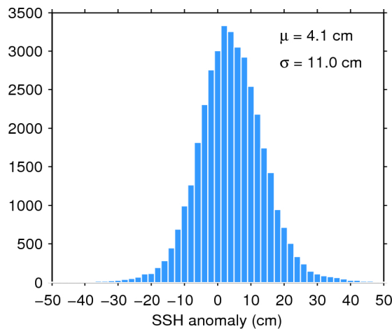
Figure 11. Histogram of science-valid SSH anomaly over oceans and lakes for 18/02/2017. The mean ( \mu ) and standard deviation ( \sigma ) are also shown. Note that values outside [-50 50] cm are excluded from the histogram for the sake of readability but not from the computation of \mu and \sigma .
