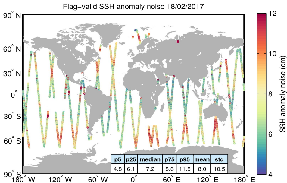
Figure 8. Geographical distribution of flag-valid 20-Hz SSH anomaly measurement noise over oceans and lakes for 18/02/2017. The statistical values shown in the table refer to the SSH anomaly noise and are calculated over all measurements shown in the figure.
