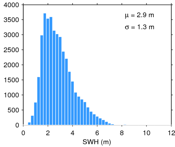
Figure 17. Histogram of flag-valid SWH over oceans and lakes for 18/02/2017. The mean ( \mu ) and standard deviation ( \sigma ) are also shown. Note that values larger than 12 m are excluded from the histogram for the sake of readability but not from the computation of \mu and \sigma .
