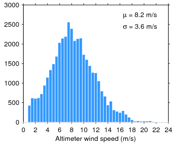
Figure 33. Histogram of flag-valid wind over oceans and lakes for 18/02/2017. The mean ( \mu ) and standard deviation ( \sigma ) are also shown. Note that values larger than 24 m/s are excluded from the histogram for the sake of readability but not from the computation of \mu and \sigma .
