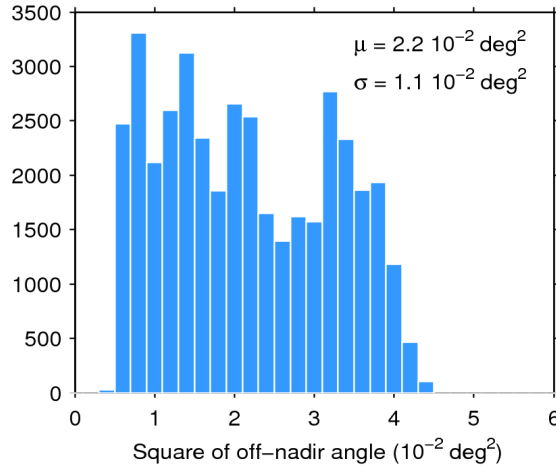
Figure 39. Histogram of flag-valid mispointing over oceans and lakes for 18/02/2017. The mean ( \mu ) and standard deviation ( \sigma ) are also shown. Note that values larger than 6 \cdot 10^{-2} \text{ deg}^2 are excluded from the histogram for the sake of readability but not from the computation of \mu and \sigma .
