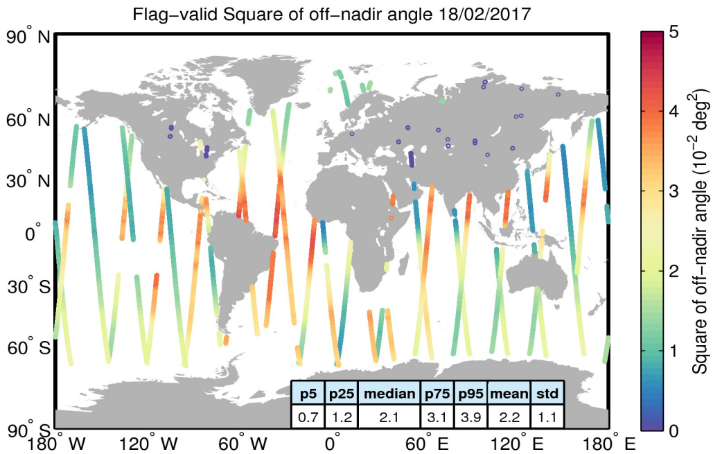
Figure 37. Geographical distribution of flag-valid mispointing data over oceans and lakes for 18/02/2017. The statistical values shown in the table refer to the mispointing in 10^{-2} deg 2 and are calculated over all measurements shown in the figure.
