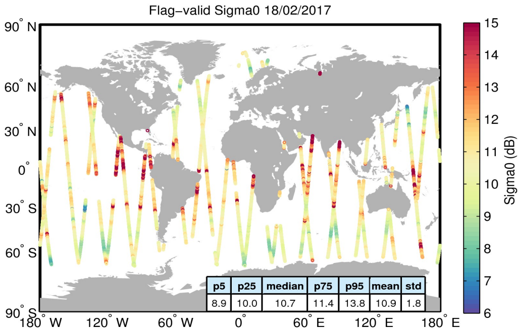
Figure 23. Geographical distribution of flag-valid sigma0 data over oceans and lakes for 18/02/2017. The statistical values shown in the table refer to the sigma0 in dB and are calculated over all measurements shown in the figure.
