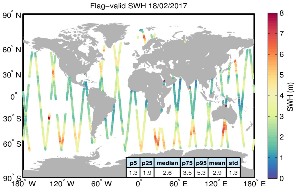
Figure 15. Geographical distribution of flag-valid SWH data over oceans and lakes for 18/02/2017. The statistical values shown in the table refer to the SWH in m and are calculated over all measurements shown in the figure.
