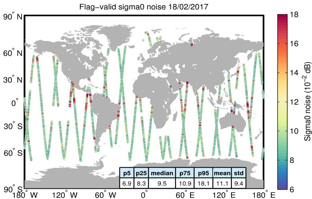
Figure 26. Geographical distribution of flag-valid 20-Hz sigma0 measurement noise over oceans and lakes for 18/02/2017. The statistical values shown in the table refer to the sigma0 noise and are calculated over all measurements shown in the figure.
