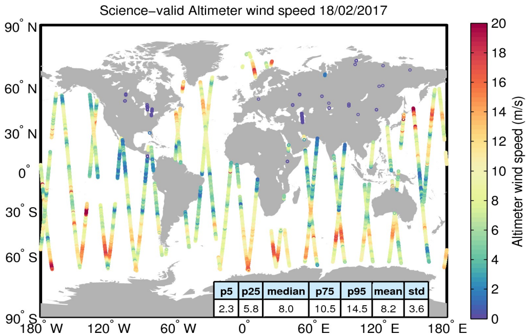
Figure 34. Geographical distribution of science-valid wind data over oceans and lakes for 18/02/2017. The statistical values shown in the table refer to the wind in m/s and are calculated over all measurements shown in the figure. Gray circles denote records that have been rejected based on the editing criteria described in Table 5.
