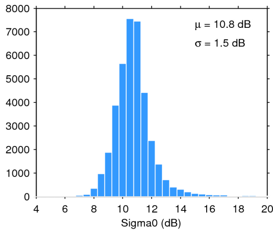
Figure 28. Histogram of science-valid sigma0 over oceans and lakes for 18/02/2017. The mean ( \mu ) and standard deviation ( \sigma ) are also shown. Note that values outside [4 20] dB are excluded from the histogram for the sake of readability but not from the computation of \mu and \sigma .
