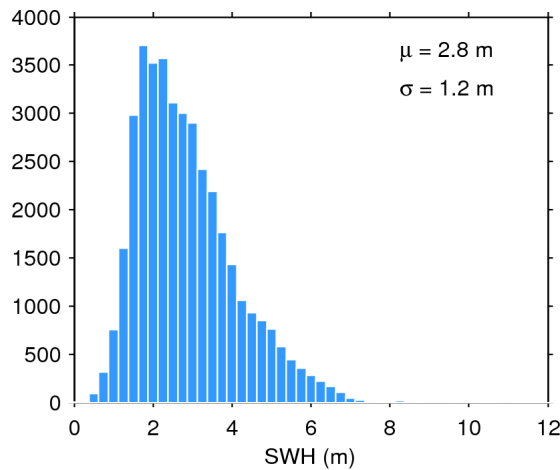
Figure 20. Histogram of science-valid SWH over oceans and lakes for 18/02/2017. The mean ( \mu ) and standard deviation ( \sigma ) are also shown. Note that values larger than 12 m are excluded from the histogram for the sake of readability but not from the computation of \mu and \sigma .
