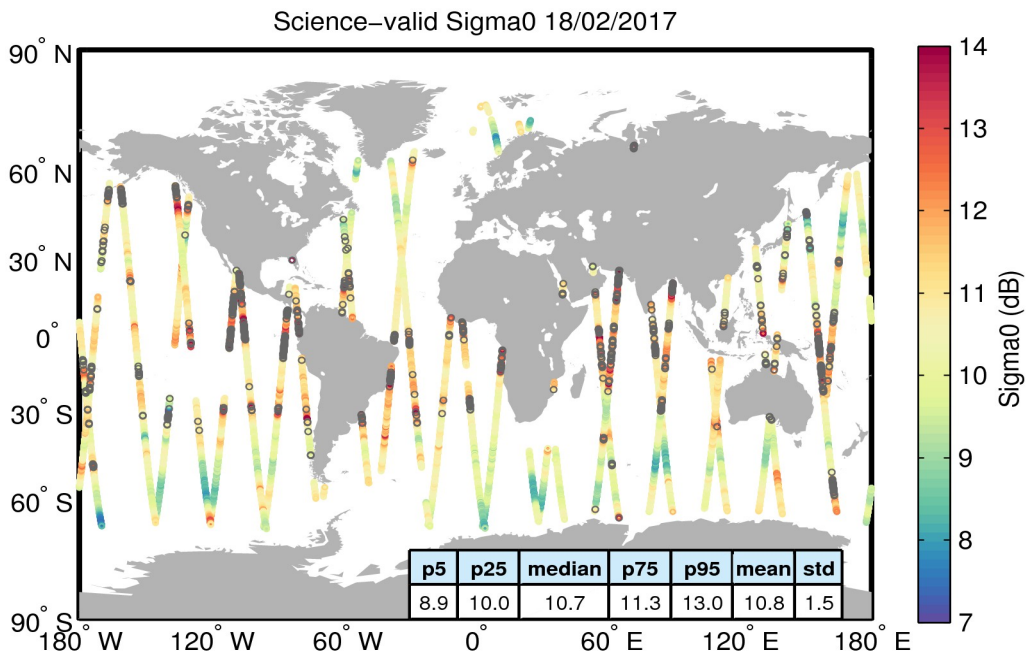
Figure 27. Geographical distribution of science-valid sigma0 data over oceans and lakes for 18/02/2017. The statistical values shown in the table refer to the sigma0 in dB and are calculated over all measurements shown in the figure. Gray circles denote records that have been rejected based on the editing criteria described in Table 4.
