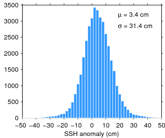
Figure 7. Histogram of flag-valid SSH anomaly over oceans and lakes for 18/02/2017. The mean ( \mu ) and standard deviation ( \sigma ) are also shown. Note that values outside [-50 50] cm are excluded from the histogram for the sake of readability but not from the computation of \mu and \sigma .
