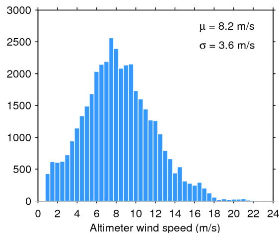
Figure 35. Histogram of science-valid wind over oceans and lakes for 18/02/2017. The mean ( \mu ) and standard deviation ( \sigma ) are also shown. Note that values larger than 24 m/s are excluded from the histogram for the sake of readability but not from the computation of \mu and \sigma .
