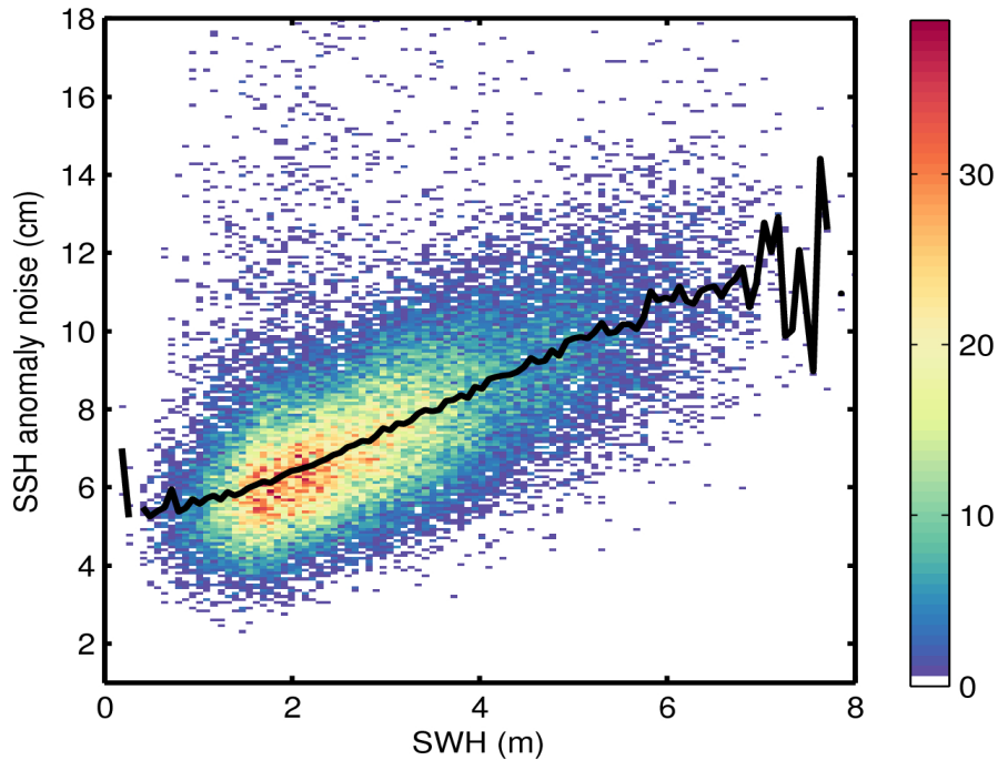
Figure 9. 2D histogram showing flag-valid SSH anomaly noise as a function of SWH for 18/02/2017. The black line denotes the median SSH anomaly noise as a function of SWH.
