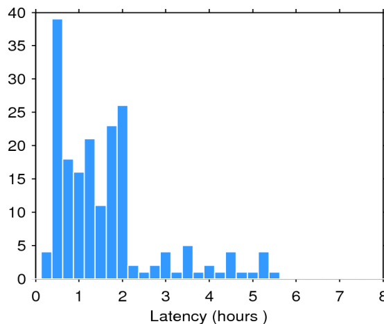
Figure 2. Histogram of the data latency for 18/02/2017. The y-axis denotes the number of files that are made available with a delay of x-hours with respect to the mean time of the records stored in the file.
