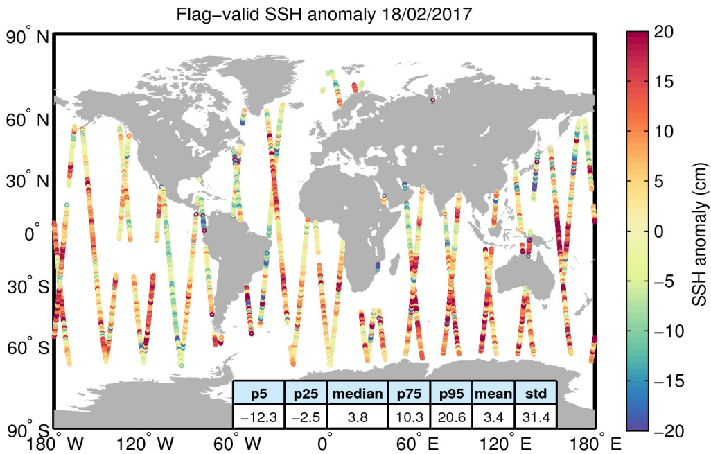
Figure 5. Geographical distribution of flag-valid 1-Hz SSH anomaly data over oceans and lakes for 18/02/2017. The statistical values shown in the table refer to the SSH anomaly in cm and are calculated over all measurements shown in the figure.
