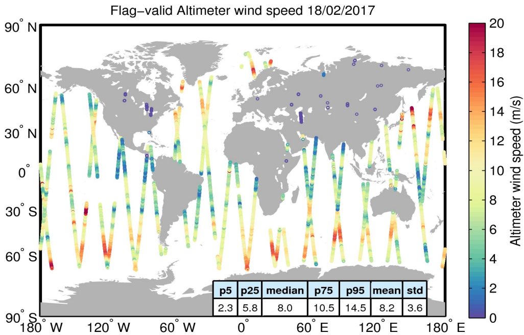
Figure 31. Geographical distribution of flag-valid wind data over oceans and lakes for 18/02/2017. The statistical values shown in the table refer to the wind in m/s and are calculated over all measurements shown in the figure.
