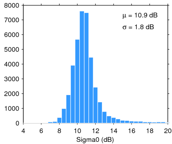
Figure 25. Histogram of flag-valid sigma0 over oceans and lakes for 18/02/2017. The mean ( \mu ) and standard deviation ( \sigma ) are also shown. Note that values outside [4 20] dB are excluded from the histogram for the sake of readability but not from the computation of \mu and \sigma .
