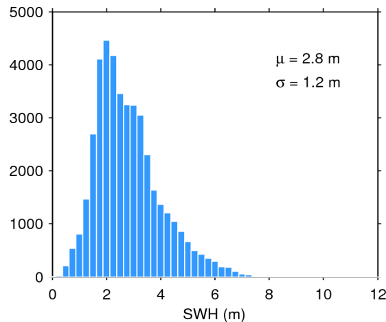
Figure 20. Histogram of science-valid SWH over oceans and lakes for 17/02/2017. The mean ( \mu ) and standard deviation ( \sigma ) are also shown. Note that values larger than 12 m are excluded from the histogram for the sake of readability but not from the computation of \mu and \sigma .
