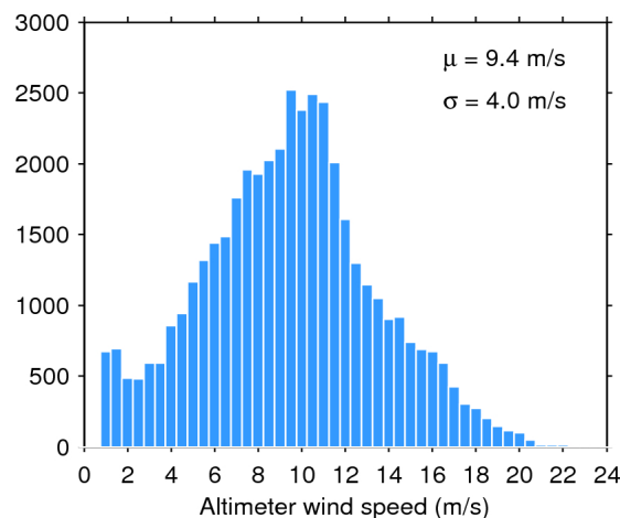
Figure 35. Histogram of science-valid wind over oceans and lakes for 17/02/2017. The mean ( \mu ) and standard deviation ( \sigma ) are also shown. Note that values larger than 24 m/s are excluded from the histogram for the sake of readability but not from the computation of \mu and \sigma .
