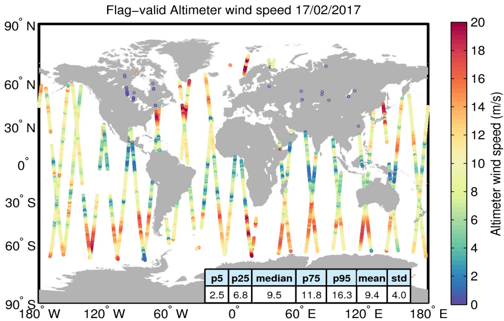
Figure 31. Geographical distribution of flag-valid wind data over oceans and lakes for 17/02/2017. The statistical values shown in the table refer to the wind in m/s and are calculated over all measurements shown in the figure.
