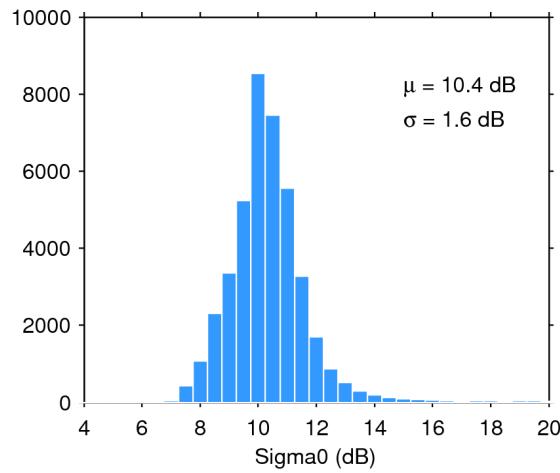
Figure 28. Histogram of science-valid sigma0 over oceans and lakes for 17/02/2017. The mean ( \mu ) and standard deviation ( \sigma ) are also shown. Note that values outside [4 20] dB are excluded from the histogram for the sake of readability but not from the computation of \mu and \sigma .
