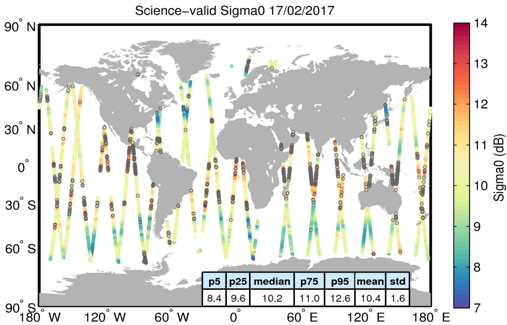
Figure 27. Geographical distribution of science-valid sigma0 data over oceans and lakes for 17/02/2017. The statistical values shown in the table refer to the sigma0 in dB and are calculated over all measurements shown in the figure. Gray circles denote records that have been rejected based on the editing criteria described in Table 4.
