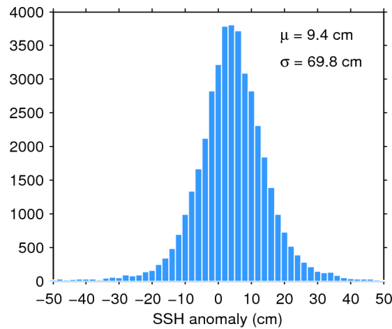
Figure 7. Histogram of flag-valid SSH anomaly over oceans and lakes for 17/02/2017. The mean ( \mu ) and standard deviation ( \sigma ) are also shown. Note that values outside [-50 50] cm are excluded from the histogram for the sake of readability but not from the computation of \mu and \sigma .
