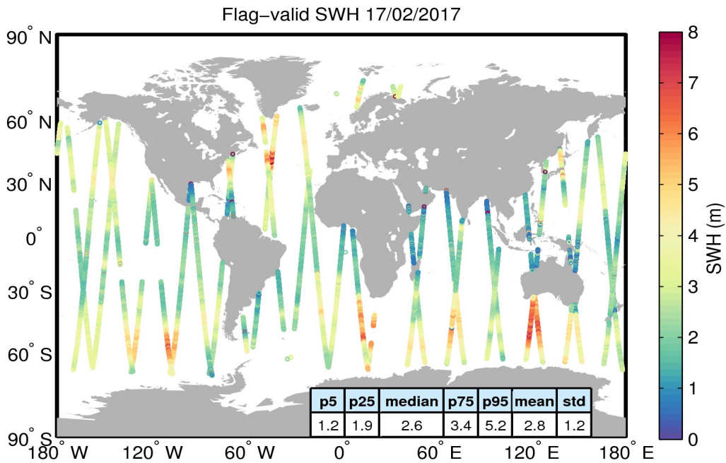
Figure 15. Geographical distribution of flag-valid SWH data over oceans and lakes for 17/02/2017. The statistical values shown in the table refer to the SWH in m and are calculated over all measurements shown in the figure.
