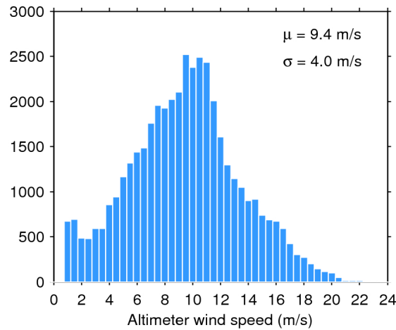
Figure 33. Histogram of flag-valid wind over oceans and lakes for 17/02/2017. The mean ( \mu ) and standard deviation ( \sigma ) are also shown. Note that values larger than 24 m/s are excluded from the histogram for the sake of readability but not from the computation of \mu and \sigma .
