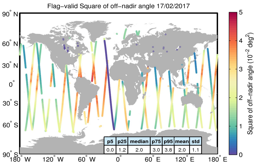
Figure 37. Geographical distribution of flag-valid mispointing data over oceans and lakes for 17/02/2017. The statistical values shown in the table refer to the mispointing in 10^{-2} deg 2 and are calculated over all measurements shown in the figure.
