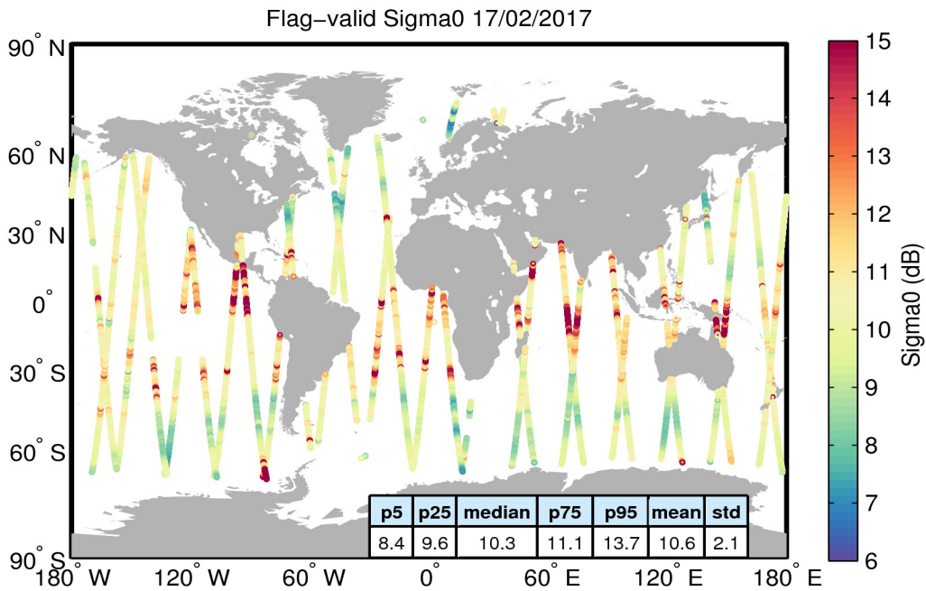
Figure 23. Geographical distribution of flag-valid sigma0 data over oceans and lakes for 17/02/2017. The statistical values shown in the table refer to the sigma0 in dB and are calculated over all measurements shown in the figure.
