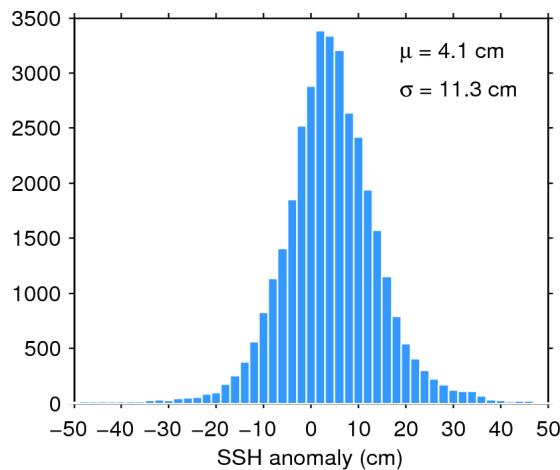
Figure 11. Histogram of science-valid SSH anomaly over oceans and lakes for 17/02/2017. The mean ( \mu ) and standard deviation ( \sigma ) are also shown. Note that values outside [-50 50] cm are excluded from the histogram for the sake of readability but not from the computation of \mu and \sigma .
