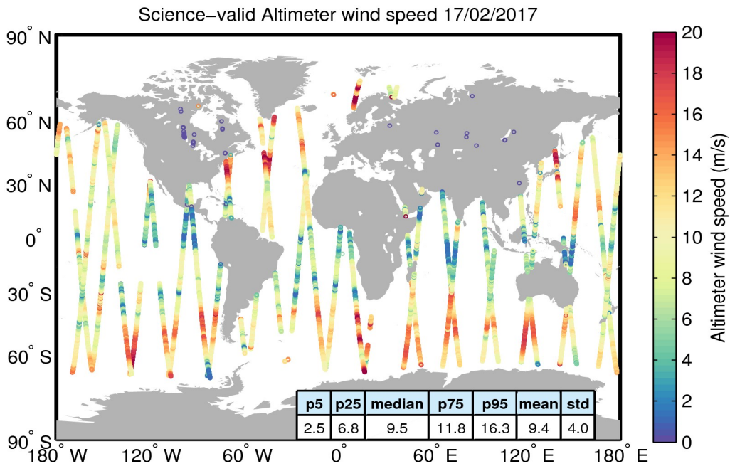
Figure 34. Geographical distribution of science-valid wind data over oceans and lakes for 17/02/2017. The statistical values shown in the table refer to the wind in m/s and are calculated over all measurements shown in the figure. Gray circles denote records that have been rejected based on the editing criteria described in Table 5.
