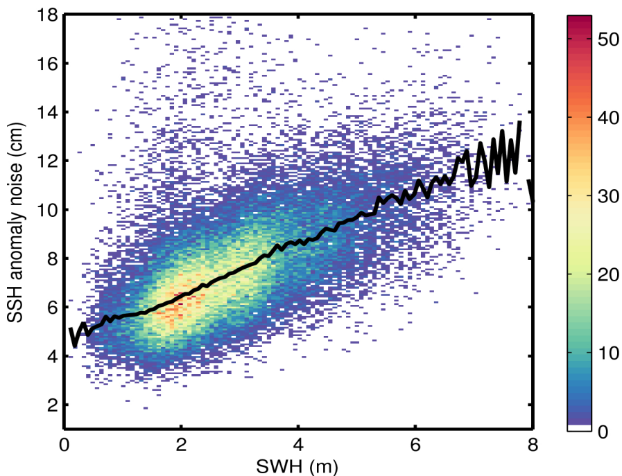
Figure 9. 2D histogram showing flag-valid SSH anomaly noise as a function of SWH for 17/02/2017. The black line denotes the median SSH anomaly noise as a function of SWH.
