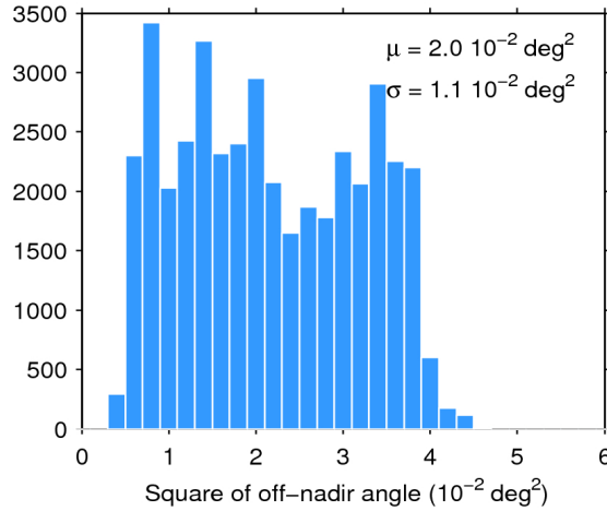
Figure 39. Histogram of flag-valid mispointing over oceans and lakes for 17/02/2017. The mean ( \mu ) and standard deviation ( \sigma ) are also shown. Note that values larger than 6 \cdot 10^{-2} \text{ deg}^2 are excluded from the histogram for the sake of readability but not from the computation of \mu and \sigma .
