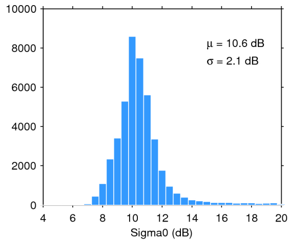
Figure 25. Histogram of flag-valid sigma0 over oceans and lakes for 17/02/2017. The mean ( \mu ) and standard deviation ( \sigma ) are also shown. Note that values outside [4 20] dB are excluded from the histogram for the sake of readability but not from the computation of \mu and \sigma .
