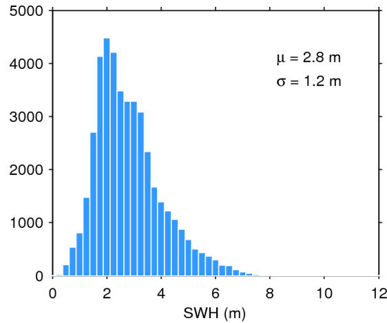
Figure 17. Histogram of flag-valid SWH over oceans and lakes for 17/02/2017. The mean ( \mu ) and standard deviation ( \sigma ) are also shown. Note that values larger than 12 m are excluded from the histogram for the sake of readability but not from the computation of \mu and \sigma .
