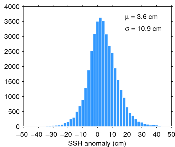
Figure 11. Histogram of science-valid SSH anomaly over oceans and lakes for 16/02/2017. The mean ( \mu ) and standard deviation ( \sigma ) are also shown. Note that values outside [-50 50] cm are excluded from the histogram for the sake of readability but not from the computation of \mu and \sigma .
