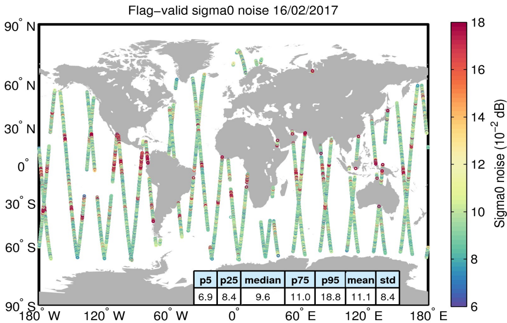
Figure 26. Geographical distribution of flag-valid 20-Hz sigma0 measurement noise over oceans and lakes for 16/02/2017. The statistical values shown in the table refer to the sigma0 noise and are calculated over all measurements shown in the figure.
