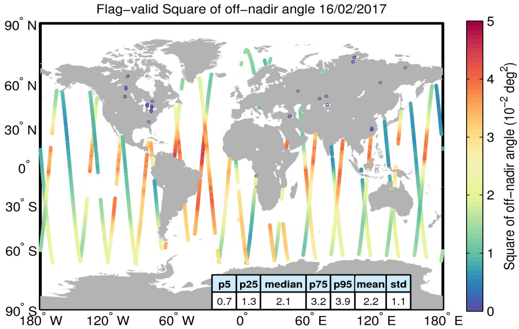
Figure 37. Geographical distribution of flag-valid mispointing data over oceans and lakes for 16/02/2017. The statistical values shown in the table refer to the mispointing in 10^{-2} deg 2 and are calculated over all measurements shown in the figure.
