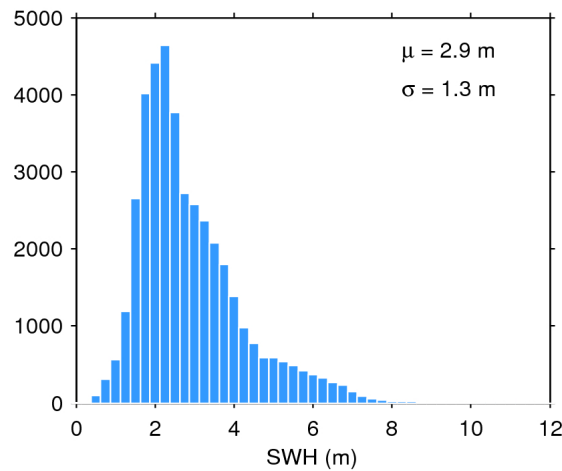
Figure 17. Histogram of flag-valid SWH over oceans and lakes for 16/02/2017. The mean ( \mu ) and standard deviation ( \sigma ) are also shown. Note that values larger than 12 m are excluded from the histogram for the sake of readability but not from the computation of \mu and \sigma .
