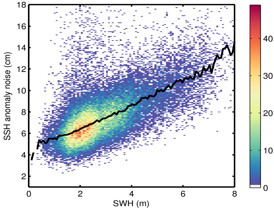
Figure 9. 2D histogram showing flag-valid SSH anomaly noise as a function of SWH for 16/02/2017. The black line denotes the median SSH anomaly noise as a function of SWH.
