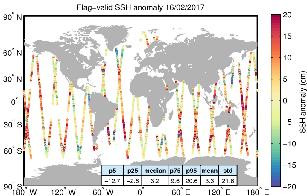
Figure 5. Geographical distribution of flag-valid 1-Hz SSH anomaly data over oceans and lakes for 16/02/2017. The statistical values shown in the table refer to the SSH anomaly in cm and are calculated over all measurements shown in the figure.
