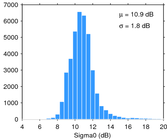
Figure 28. Histogram of science-valid sigma0 over oceans and lakes for 16/02/2017. The mean ( \mu ) and standard deviation ( \sigma ) are also shown. Note that values outside [4 20] dB are excluded from the histogram for the sake of readability but not from the computation of \mu and \sigma .
