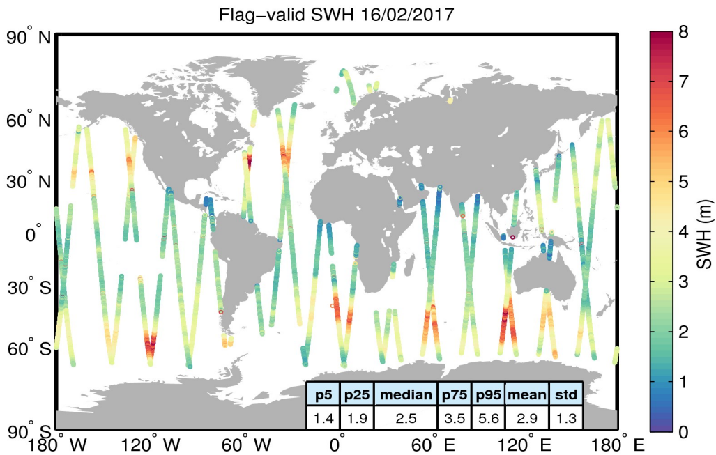
Figure 15. Geographical distribution of flag-valid SWH data over oceans and lakes for 16/02/2017. The statistical values shown in the table refer to the SWH in m and are calculated over all measurements shown in the figure.
