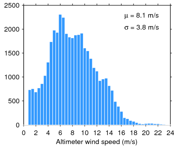
Figure 33. Histogram of flag-valid wind over oceans and lakes for 16/02/2017. The mean ( \mu ) and standard deviation ( \sigma ) are also shown. Note that values larger than 24 m/s are excluded from the histogram for the sake of readability but not from the computation of \mu and \sigma .
