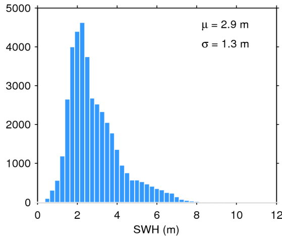
Figure 20. Histogram of science-valid SWH over oceans and lakes for 16/02/2017. The mean ( \mu ) and standard deviation ( \sigma ) are also shown. Note that values larger than 12 m are excluded from the histogram for the sake of readability but not from the computation of \mu and \sigma .
