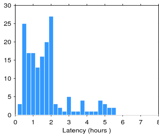
Figure 2. Histogram of the data latency for 16/02/2017. The y-axis denotes the number of files that are made available with a delay of x-hours with respect to the mean time of the records stored in the file.
