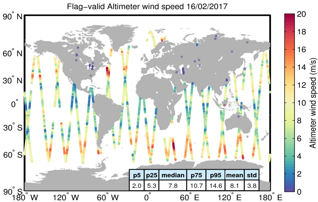
Figure 31. Geographical distribution of flag-valid wind data over oceans and lakes for 16/02/2017. The statistical values shown in the table refer to the wind in m/s and are calculated over all measurements shown in the figure.
