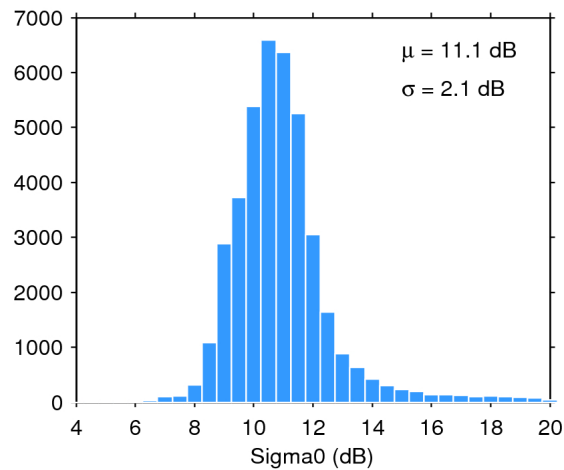
Figure 25. Histogram of flag-valid sigma0 over oceans and lakes for 16/02/2017. The mean ( \mu ) and standard deviation ( \sigma ) are also shown. Note that values outside [4 20] dB are excluded from the histogram for the sake of readability but not from the computation of \mu and \sigma .
