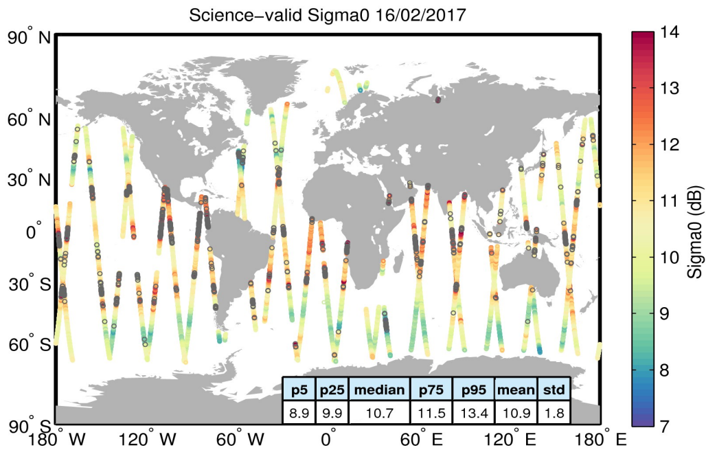
Figure 27. Geographical distribution of science-valid sigma0 data over oceans and lakes for 16/02/2017. The statistical values shown in the table refer to the sigma0 in dB and are calculated over all measurements shown in the figure. Gray circles denote records that have been rejected based on the editing criteria described in Table 4.
