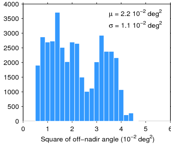
Figure 39. Histogram of flag-valid mispointing over oceans and lakes for 16/02/2017. The mean ( \mu ) and standard deviation ( \sigma ) are also shown. Note that values larger than 6 \cdot 10^{-2} \text{ deg}^2 are excluded from the histogram for the sake of readability but not from the computation of \mu and \sigma .
