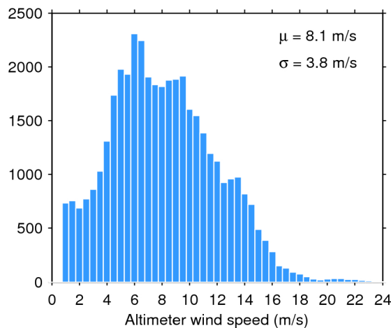
Figure 35. Histogram of science-valid wind over oceans and lakes for 16/02/2017. The mean ( \mu ) and standard deviation ( \sigma ) are also shown. Note that values larger than 24 m/s are excluded from the histogram for the sake of readability but not from the computation of \mu and \sigma .
