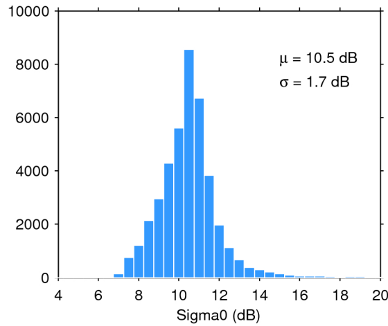
Figure 28. Histogram of science-valid sigma0 over oceans and lakes for 15/02/2017. The mean ( \mu ) and standard deviation ( \sigma ) are also shown. Note that values outside [4 20] dB are excluded from the histogram for the sake of readability but not from the computation of \mu and \sigma .
