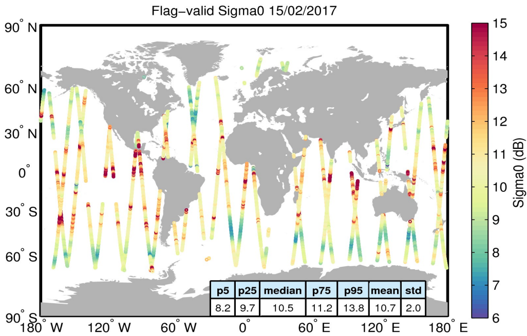
Figure 23. Geographical distribution of flag-valid sigma0 data over oceans and lakes for 15/02/2017. The statistical values shown in the table refer to the sigma0 in dB and are calculated over all measurements shown in the figure.
