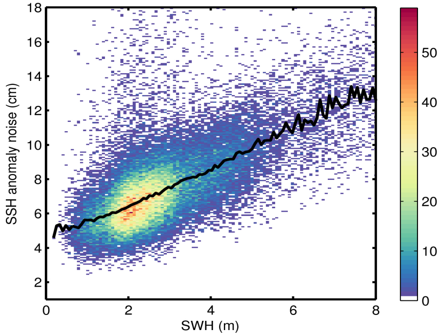
Figure 9. 2D histogram showing flag-valid SSH anomaly noise as a function of SWH for 15/02/2017. The black line denotes the median SSH anomaly noise as a function of SWH.
