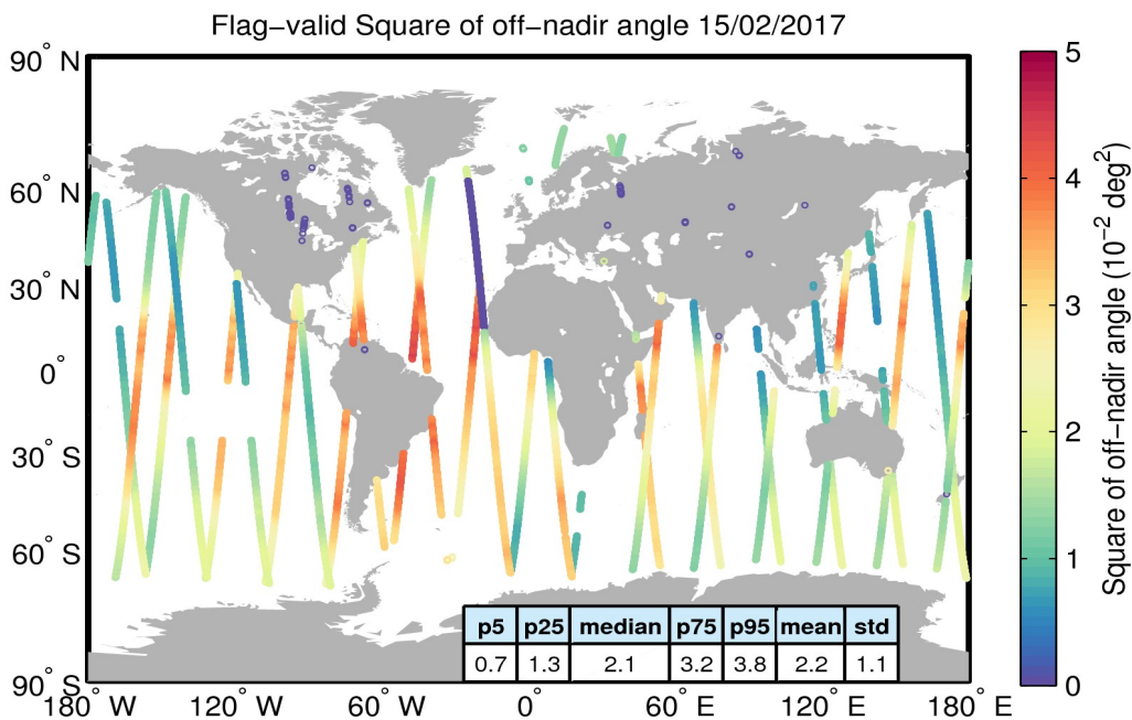
Figure 37. Geographical distribution of flag-valid mispointing data over oceans and lakes for 15/02/2017. The statistical values shown in the table refer to the mispointing in 10^{-2} deg 2 and are calculated over all measurements shown in the figure.
