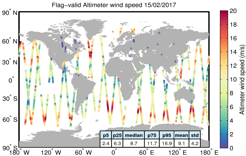
Figure 31. Geographical distribution of flag-valid wind data over oceans and lakes for 15/02/2017. The statistical values shown in the table refer to the wind in m/s and are calculated over all measurements shown in the figure.
