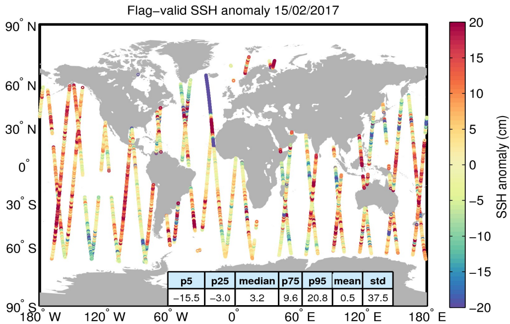
Figure 5. Geographical distribution of flag-valid 1-Hz SSH anomaly data over oceans and lakes for 15/02/2017. The statistical values shown in the table refer to the SSH anomaly in cm and are calculated over all measurements shown in the figure.
