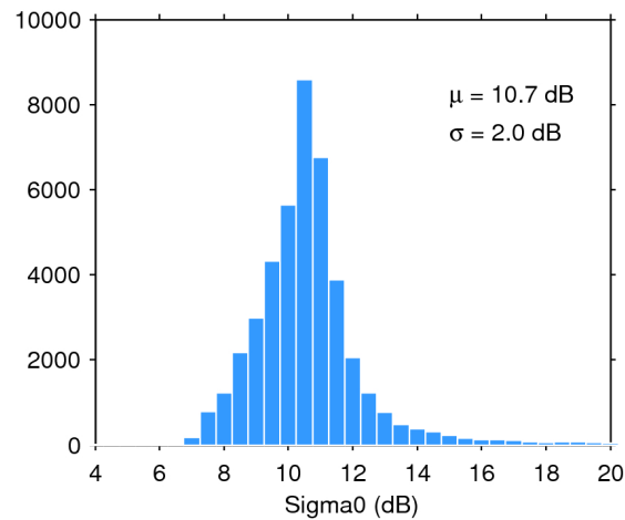
Figure 25. Histogram of flag-valid sigma0 over oceans and lakes for 15/02/2017. The mean ( \mu ) and standard deviation ( \sigma ) are also shown. Note that values outside [4 20] dB are excluded from the histogram for the sake of readability but not from the computation of \mu and \sigma .
