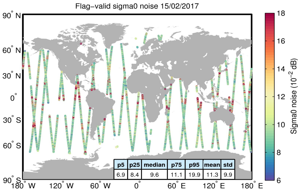
Figure 26. Geographical distribution of flag-valid 20-Hz sigma0 measurement noise over oceans and lakes for 15/02/2017. The statistical values shown in the table refer to the sigma0 noise and are calculated over all measurements shown in the figure.
