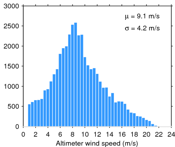
Figure 35. Histogram of science-valid wind over oceans and lakes for 15/02/2017. The mean ( \mu ) and standard deviation ( \sigma ) are also shown. Note that values larger than 24 m/s are excluded from the histogram for the sake of readability but not from the computation of \mu and \sigma .
