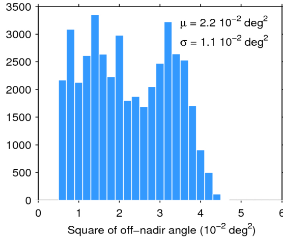
Figure 39. Histogram of flag-valid mispointing over oceans and lakes for 15/02/2017. The mean ( \mu ) and standard deviation ( \sigma ) are also shown. Note that values larger than 6 \cdot 10^{-2} \text{ deg}^2 are excluded from the histogram for the sake of readability but not from the computation of \mu and \sigma .
