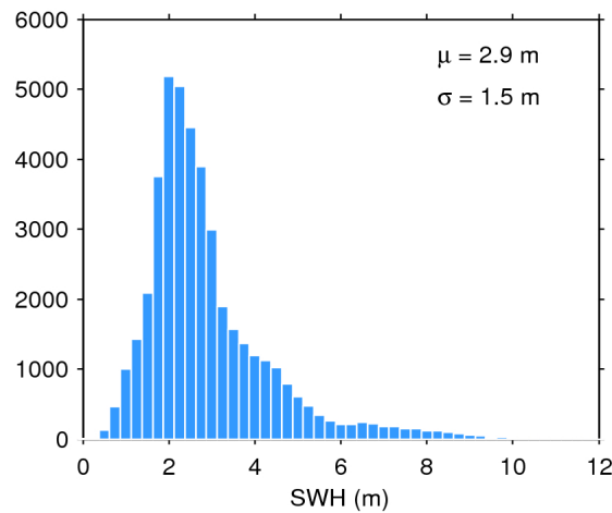
Figure 17. Histogram of flag-valid SWH over oceans and lakes for 15/02/2017. The mean ( \mu ) and standard deviation ( \sigma ) are also shown. Note that values larger than 12 m are excluded from the histogram for the sake of readability but not from the computation of \mu and \sigma .
