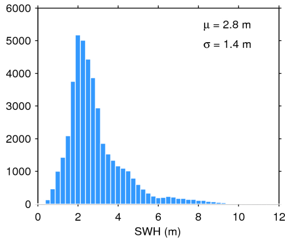
Figure 20. Histogram of science-valid SWH over oceans and lakes for 15/02/2017. The mean ( \mu ) and standard deviation ( \sigma ) are also shown. Note that values larger than 12 m are excluded from the histogram for the sake of readability but not from the computation of \mu and \sigma .
