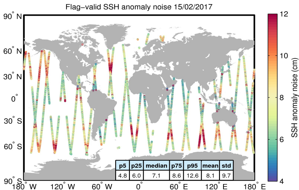
Figure 8. Geographical distribution of flag-valid 20-Hz SSH anomaly measurement noise over oceans and lakes for 15/02/2017. The statistical values shown in the table refer to the SSH anomaly noise and are calculated over all measurements shown in the figure.
