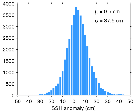
Figure 7. Histogram of flag-valid SSH anomaly over oceans and lakes for 15/02/2017. The mean ( \mu ) and standard deviation ( \sigma ) are also shown. Note that values outside [-50 50] cm are excluded from the histogram for the sake of readability but not from the computation of \mu and \sigma .
