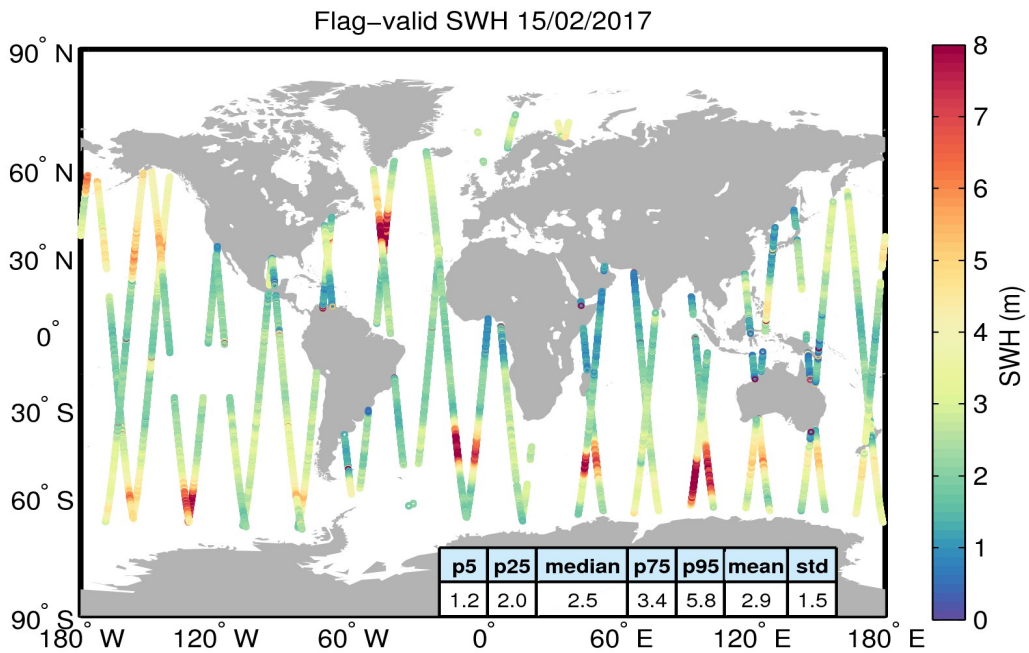
Figure 15. Geographical distribution of flag-valid SWH data over oceans and lakes for 15/02/2017. The statistical values shown in the table refer to the SWH in m and are calculated over all measurements shown in the figure.
