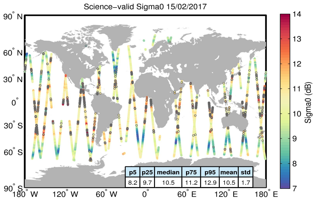
Figure 27. Geographical distribution of science-valid sigma0 data over oceans and lakes for 15/02/2017. The statistical values shown in the table refer to the sigma0 in dB and are calculated over all measurements shown in the figure. Gray circles denote records that have been rejected based on the editing criteria described in Table 4.
