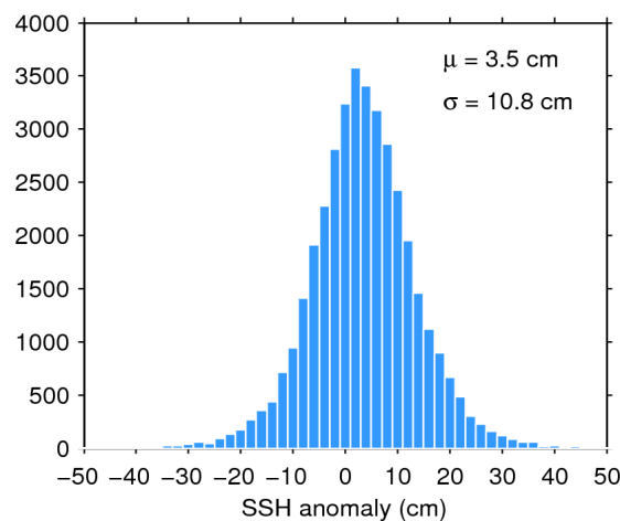
Figure 11. Histogram of science-valid SSH anomaly over oceans and lakes for 15/02/2017. The mean ( \mu ) and standard deviation ( \sigma ) are also shown. Note that values outside [-50 50] cm are excluded from the histogram for the sake of readability but not from the computation of \mu and \sigma .
