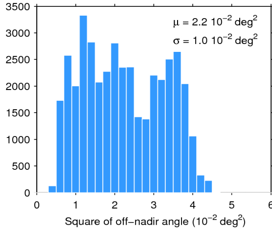
Figure 39. Histogram of flag-valid mispointing over oceans and lakes for 14/02/2017. The mean ( \mu ) and standard deviation ( \sigma ) are also shown. Note that values larger than 6 \cdot 10^{-2} \text{ deg}^2 are excluded from the histogram for the sake of readability but not from the computation of \mu and \sigma .
