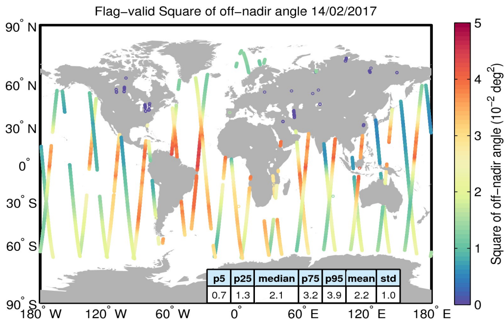
Figure 37. Geographical distribution of flag-valid mispointing data over oceans and lakes for 14/02/2017. The statistical values shown in the table refer to the mispointing in 10^{-2} deg 2 and are calculated over all measurements shown in the figure.
