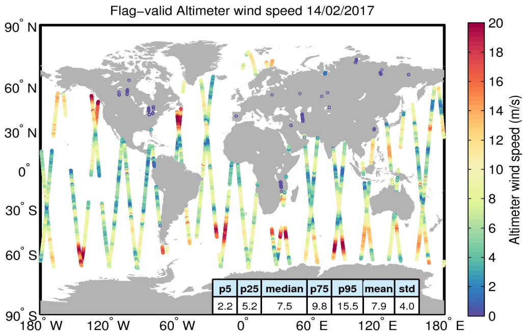
Figure 31. Geographical distribution of flag-valid wind data over oceans and lakes for 14/02/2017. The statistical values shown in the table refer to the wind in m/s and are calculated over all measurements shown in the figure.
