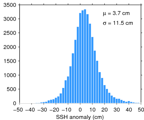
Figure 11. Histogram of science-valid SSH anomaly over oceans and lakes for 14/02/2017. The mean ( \mu ) and standard deviation ( \sigma ) are also shown. Note that values outside [-50 50] cm are excluded from the histogram for the sake of readability but not from the computation of \mu and \sigma .
