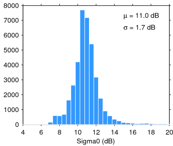
Figure 28. Histogram of science-valid sigma0 over oceans and lakes for 14/02/2017. The mean ( \mu ) and standard deviation ( \sigma ) are also shown. Note that values outside [4 20] dB are excluded from the histogram for the sake of readability but not from the computation of \mu and \sigma .
