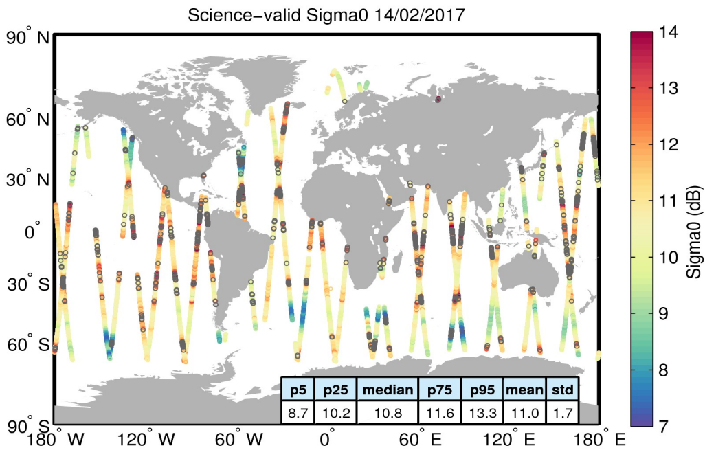
Figure 27. Geographical distribution of science-valid sigma0 data over oceans and lakes for 14/02/2017. The statistical values shown in the table refer to the sigma0 in dB and are calculated over all measurements shown in the figure. Gray circles denote records that have been rejected based on the editing criteria described in Table 4.
