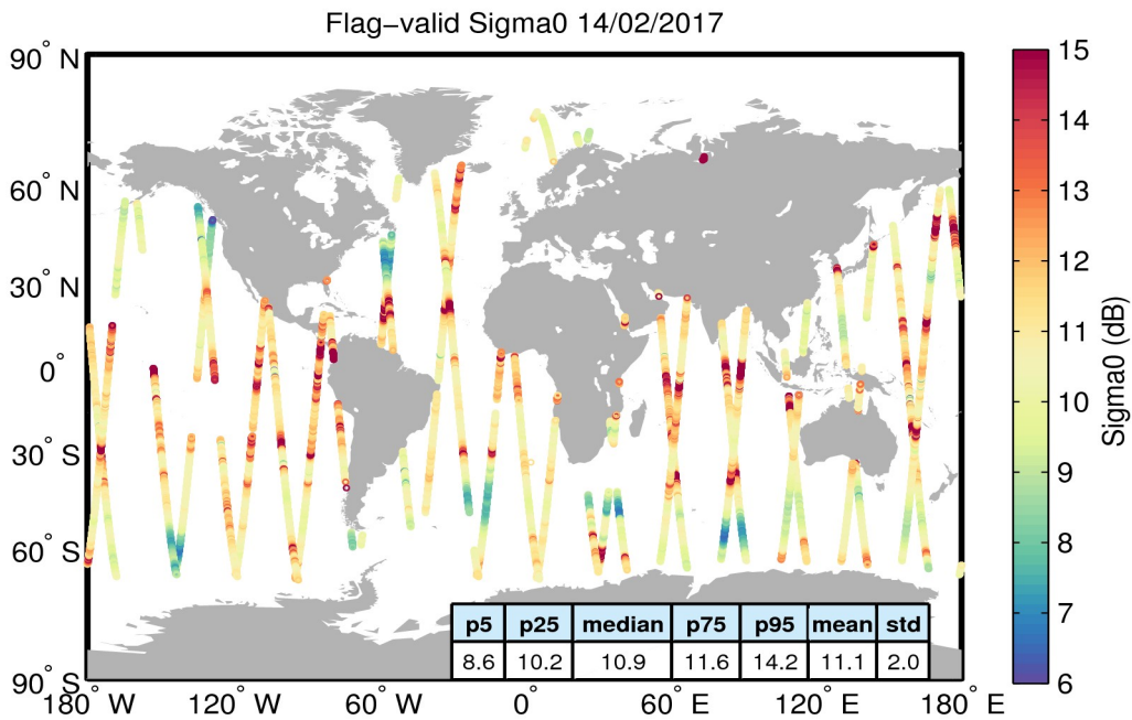
Figure 23. Geographical distribution of flag-valid sigma0 data over oceans and lakes for 14/02/2017. The statistical values shown in the table refer to the sigma0 in dB and are calculated over all measurements shown in the figure.
