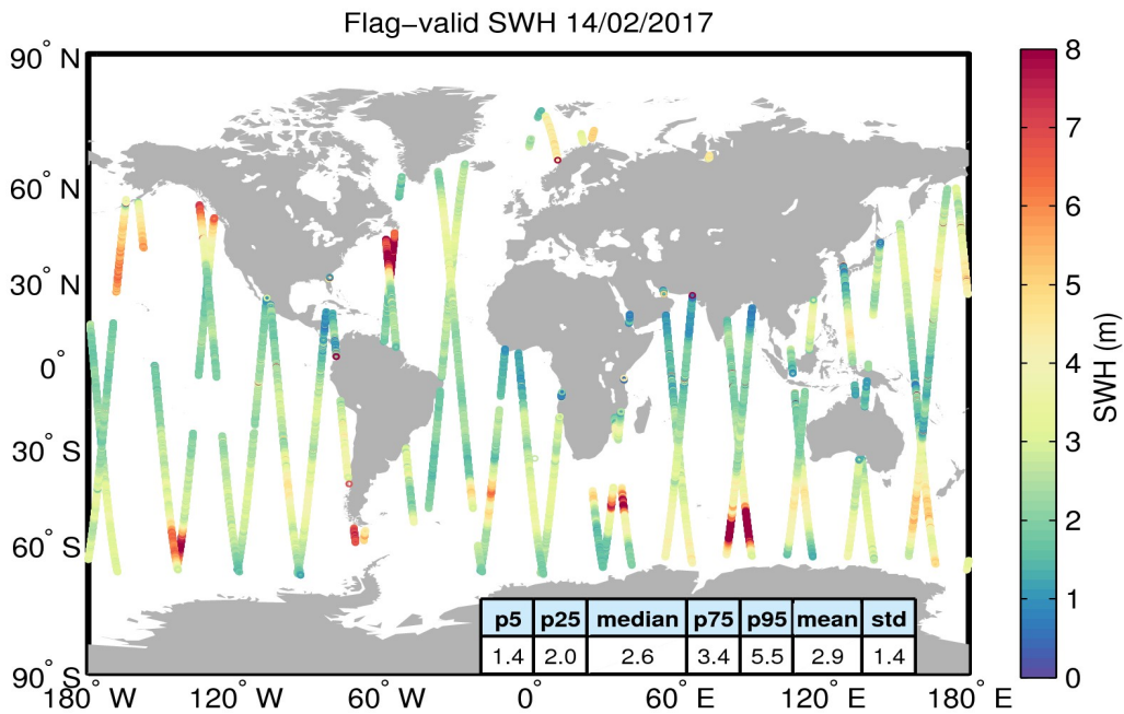
Figure 15. Geographical distribution of flag-valid SWH data over oceans and lakes for 14/02/2017. The statistical values shown in the table refer to the SWH in m and are calculated over all measurements shown in the figure.
