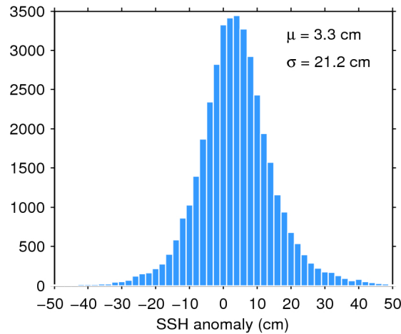
Figure 7. Histogram of flag-valid SSH anomaly over oceans and lakes for 14/02/2017. The mean ( \mu ) and standard deviation ( \sigma ) are also shown. Note that values outside [-50 50] cm are excluded from the histogram for the sake of readability but not from the computation of \mu and \sigma .
