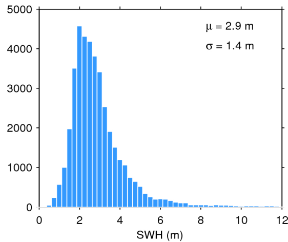
Figure 17. Histogram of flag-valid SWH over oceans and lakes for 14/02/2017. The mean ( \mu ) and standard deviation ( \sigma ) are also shown. Note that values larger than 12 m are excluded from the histogram for the sake of readability but not from the computation of \mu and \sigma .
