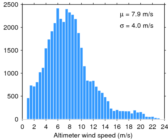
Figure 33. Histogram of flag-valid wind over oceans and lakes for 14/02/2017. The mean ( \mu ) and standard deviation ( \sigma ) are also shown. Note that values larger than 24 m/s are excluded from the histogram for the sake of readability but not from the computation of \mu and \sigma .
