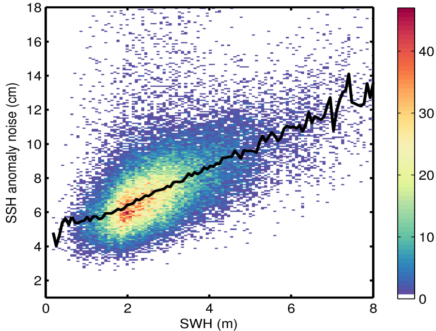
Figure 9. 2D histogram showing flag-valid SSH anomaly noise as a function of SWH for 14/02/2017. The black line denotes the median SSH anomaly noise as a function of SWH.
