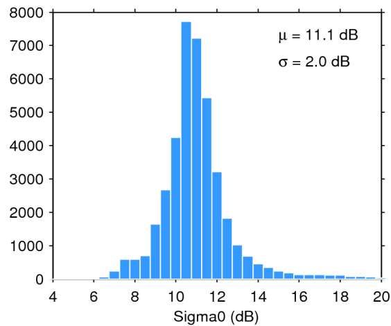
Figure 25. Histogram of flag-valid sigma0 over oceans and lakes for 14/02/2017. The mean ( \mu ) and standard deviation ( \sigma ) are also shown. Note that values outside [4 20] dB are excluded from the histogram for the sake of readability but not from the computation of \mu and \sigma .
