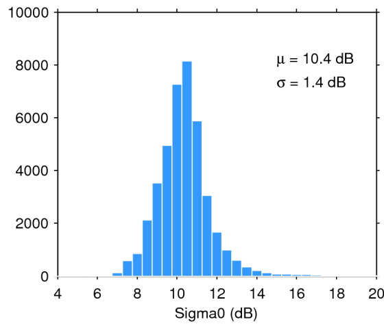
Figure 28. Histogram of science-valid sigma0 over oceans and lakes for 13/02/2017. The mean ( \mu ) and standard deviation ( \sigma ) are also shown. Note that values outside [4 20] dB are excluded from the histogram for the sake of readability but not from the computation of \mu and \sigma .
