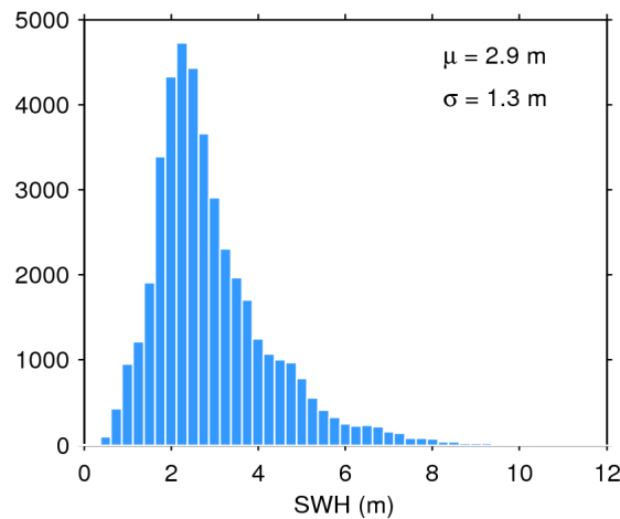
Figure 20. Histogram of science-valid SWH over oceans and lakes for 13/02/2017. The mean ( \mu ) and standard deviation ( \sigma ) are also shown. Note that values larger than 12 m are excluded from the histogram for the sake of readability but not from the computation of \mu and \sigma .
