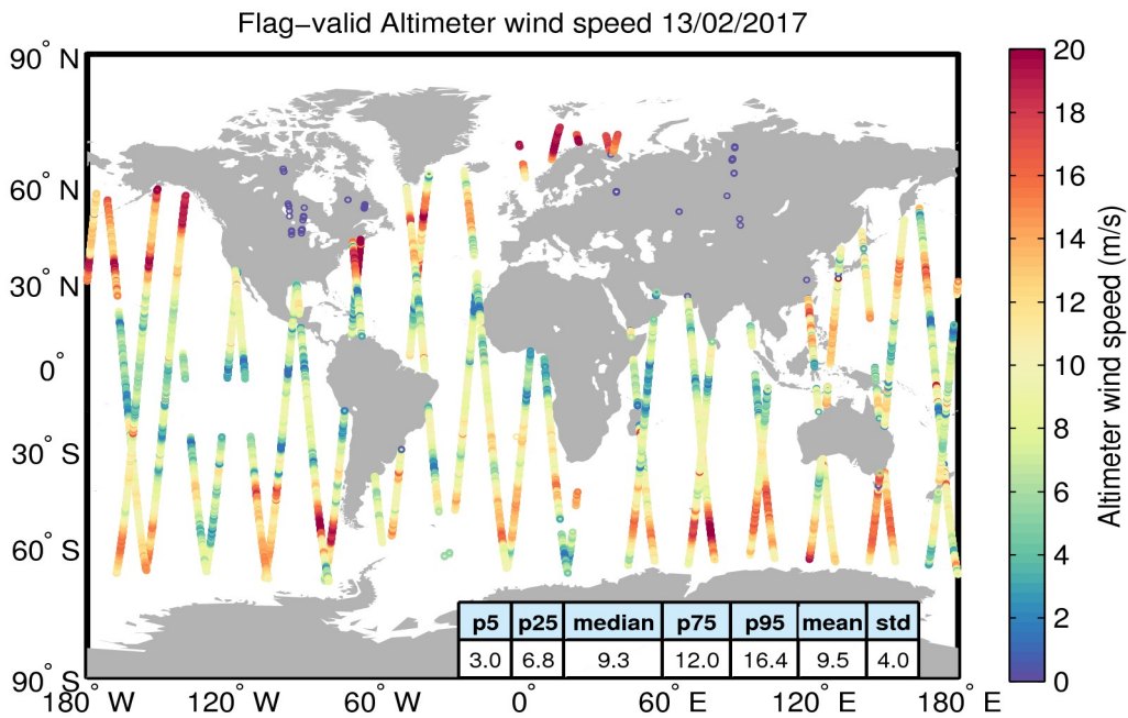
Figure 31. Geographical distribution of flag-valid wind data over oceans and lakes for 13/02/2017. The statistical values shown in the table refer to the wind in m/s and are calculated over all measurements shown in the figure.
