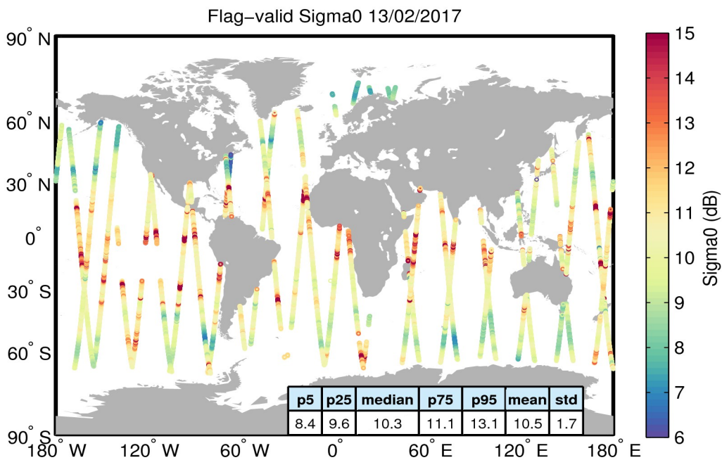
Figure 23. Geographical distribution of flag-valid sigma0 data over oceans and lakes for 13/02/2017. The statistical values shown in the table refer to the sigma0 in dB and are calculated over all measurements shown in the figure.
