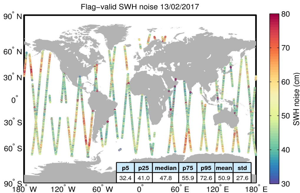
Figure 18. Geographical distribution of flag-valid 20-Hz SWH measurement noise over oceans and lakes for 13/02/2017. The statistical values shown in the table refer to the SWH noise and are calculated over all measurements shown in the figure.
