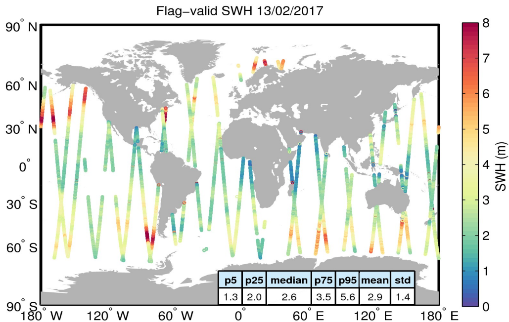
Figure 15. Geographical distribution of flag-valid SWH data over oceans and lakes for 13/02/2017. The statistical values shown in the table refer to the SWH in m and are calculated over all measurements shown in the figure.
