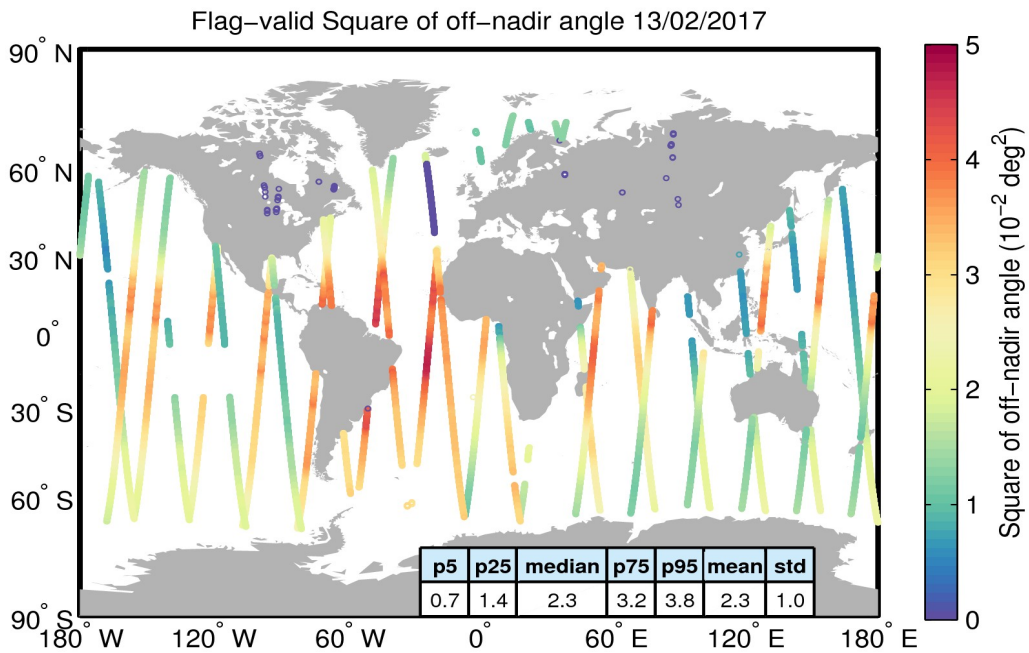
Figure 37. Geographical distribution of flag-valid mispointing data over oceans and lakes for 13/02/2017. The statistical values shown in the table refer to the mispointing in 10^{-2} deg 2 and are calculated over all measurements shown in the figure.
