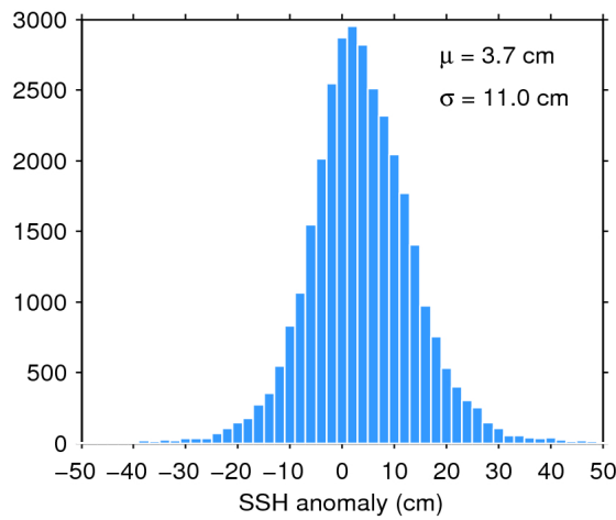
Figure 11. Histogram of science-valid SSH anomaly over oceans and lakes for 13/02/2017. The mean ( \mu ) and standard deviation ( \sigma ) are also shown. Note that values outside [-50 50] cm are excluded from the histogram for the sake of readability but not from the computation of \mu and \sigma .
