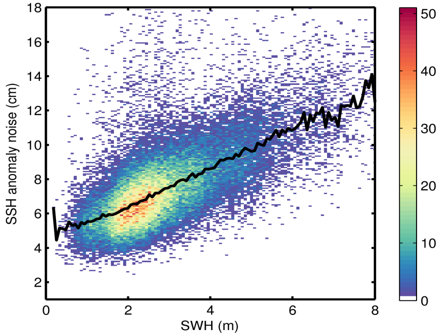
Figure 9. 2D histogram showing flag-valid SSH anomaly noise as a function of SWH for 13/02/2017. The black line denotes the median SSH anomaly noise as a function of SWH.
