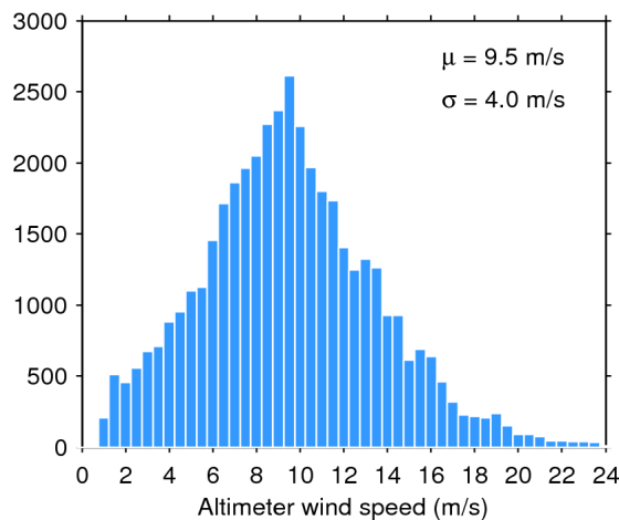
Figure 35. Histogram of science-valid wind over oceans and lakes for 13/02/2017. The mean ( \mu ) and standard deviation ( \sigma ) are also shown. Note that values larger than 24 m/s are excluded from the histogram for the sake of readability but not from the computation of \mu and \sigma .
