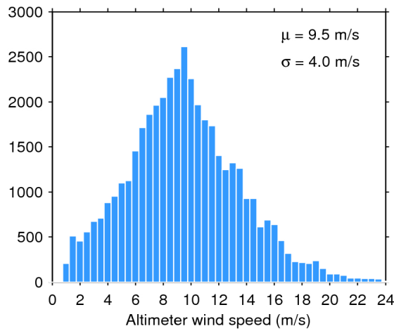
Figure 33. Histogram of flag-valid wind over oceans and lakes for 13/02/2017. The mean ( \mu ) and standard deviation ( \sigma ) are also shown. Note that values larger than 24 m/s are excluded from the histogram for the sake of readability but not from the computation of \mu and \sigma .
