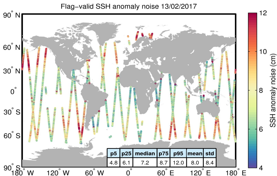
Figure 8. Geographical distribution of flag-valid 20-Hz SSH anomaly measurement noise over oceans and lakes for 13/02/2017. The statistical values shown in the table refer to the SSH anomaly noise and are calculated over all measurements shown in the figure.
