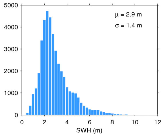
Figure 17. Histogram of flag-valid SWH over oceans and lakes for 13/02/2017. The mean ( \mu ) and standard deviation ( \sigma ) are also shown. Note that values larger than 12 m are excluded from the histogram for the sake of readability but not from the computation of \mu and \sigma .
