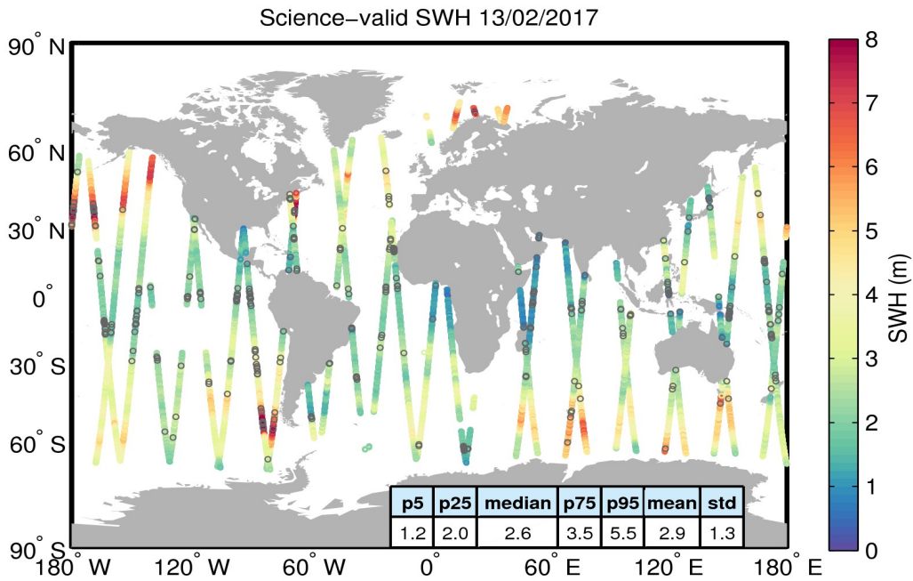
Figure 19. Geographical distribution of science-valid SWH data over oceans and lakes for 13/02/2017. The statistical values shown in the table refer to the SWH in m and are calculated over all measurements shown in the figure. Gray circles denote records that have been rejected based on the editing criteria described in Table 3.
