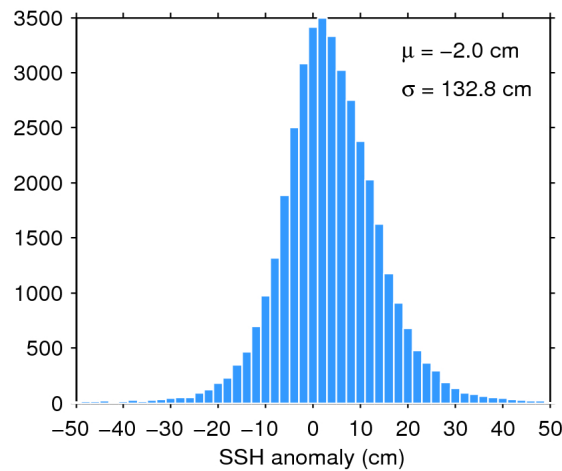
Figure 7. Histogram of flag-valid SSH anomaly over oceans and lakes for 13/02/2017. The mean ( \mu ) and standard deviation ( \sigma ) are also shown. Note that values outside [-50 50] cm are excluded from the histogram for the sake of readability but not from the computation of \mu and \sigma .
