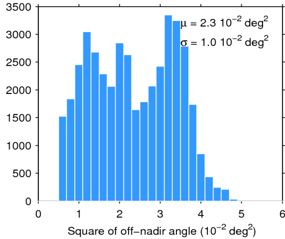
Figure 39. Histogram of flag-valid mispointing over oceans and lakes for 13/02/2017. The mean ( \mu ) and standard deviation ( \sigma ) are also shown. Note that values larger than 6 \cdot 10^{-2} \text{ deg}^2 are excluded from the histogram for the sake of readability but not from the computation of \mu and \sigma .
