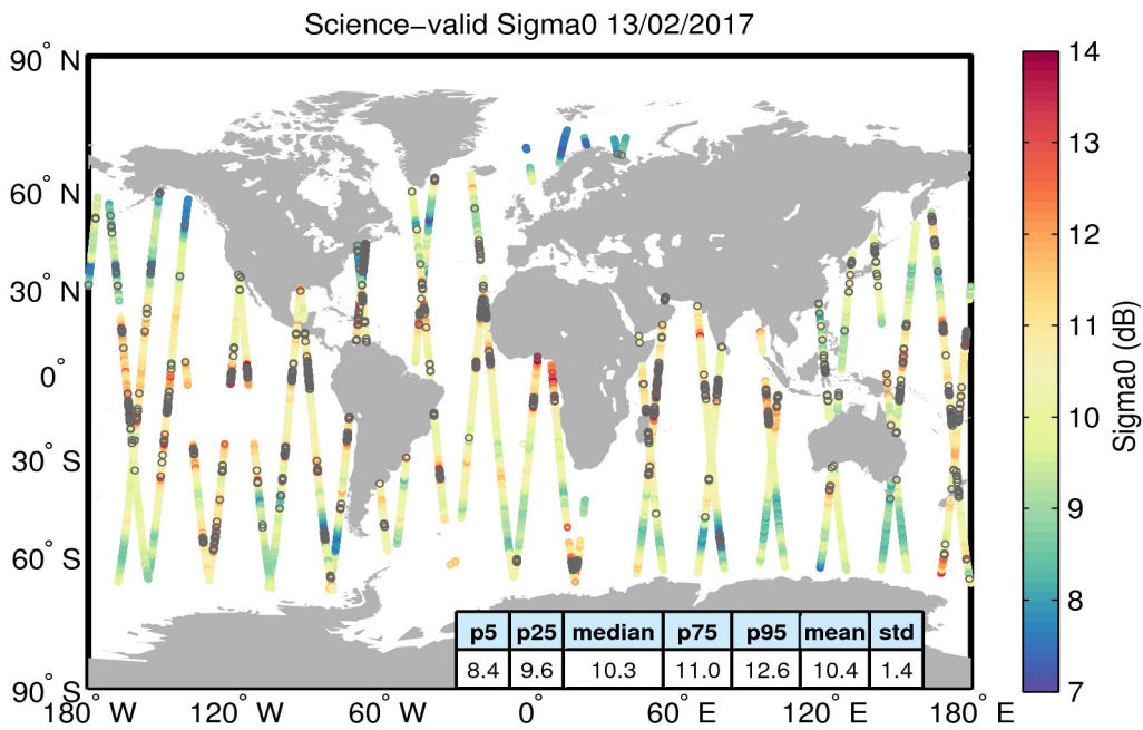
Figure 27. Geographical distribution of science-valid sigma0 data over oceans and lakes for 13/02/2017. The statistical values shown in the table refer to the sigma0 in dB and are calculated over all measurements shown in the figure. Gray circles denote records that have been rejected based on the editing criteria described in Table 4.
