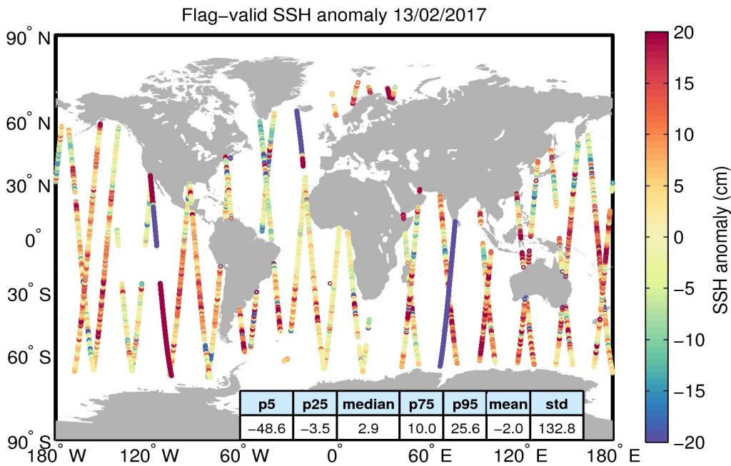
Figure 5. Geographical distribution of flag-valid 1-Hz SSH anomaly data over oceans and lakes for 13/02/2017. The statistical values shown in the table refer to the SSH anomaly in cm and are calculated over all measurements shown in the figure.
