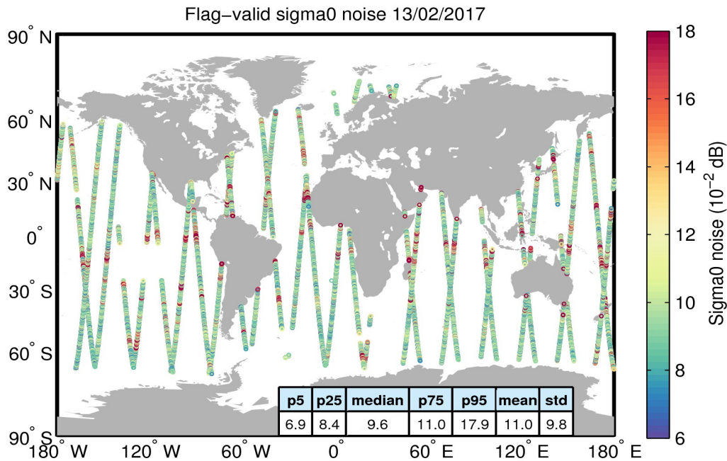
Figure 26. Geographical distribution of flag-valid 20-Hz sigma0 measurement noise over oceans and lakes for 13/02/2017. The statistical values shown in the table refer to the sigma0 noise and are calculated over all measurements shown in the figure.
