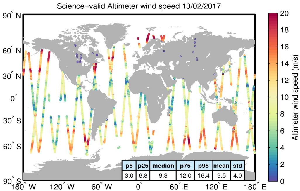
Figure 34. Geographical distribution of science-valid wind data over oceans and lakes for 13/02/2017. The statistical values shown in the table refer to the wind in m/s and are calculated over all measurements shown in the figure. Gray circles denote records that have been rejected based on the editing criteria described in Table 5.
