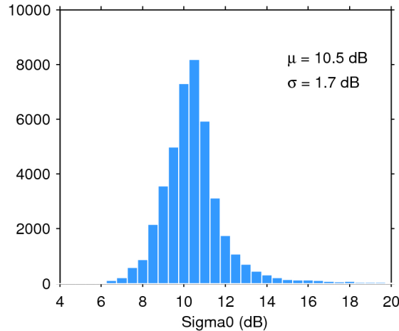
Figure 25. Histogram of flag-valid sigma0 over oceans and lakes for 13/02/2017. The mean ( \mu ) and standard deviation ( \sigma ) are also shown. Note that values outside [4 20] dB are excluded from the histogram for the sake of readability but not from the computation of \mu and \sigma .
