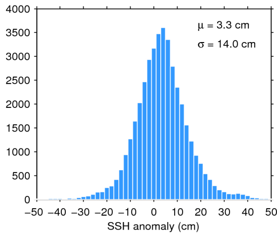
Figure 7. Histogram of flag-valid SSH anomaly over oceans and lakes for 12/02/2017. The mean ( \mu ) and standard deviation ( \sigma ) are also shown. Note that values outside [-50 50] cm are excluded from the histogram for the sake of readability but not from the computation of \mu and \sigma .
