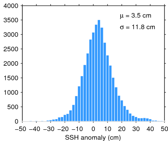
Figure 11. Histogram of science-valid SSH anomaly over oceans and lakes for 12/02/2017. The mean ( \mu ) and standard deviation ( \sigma ) are also shown. Note that values outside [-50 50] cm are excluded from the histogram for the sake of readability but not from the computation of \mu and \sigma .
