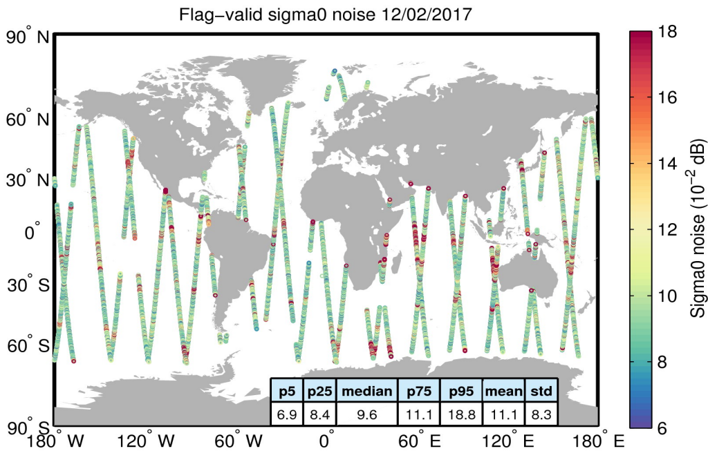
Figure 26. Geographical distribution of flag-valid 20-Hz sigma0 measurement noise over oceans and lakes for 12/02/2017. The statistical values shown in the table refer to the sigma0 noise and are calculated over all measurements shown in the figure.
