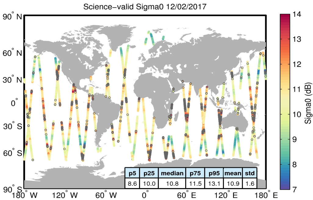
Figure 27. Geographical distribution of science-valid sigma0 data over oceans and lakes for 12/02/2017. The statistical values shown in the table refer to the sigma0 in dB and are calculated over all measurements shown in the figure. Gray circles denote records that have been rejected based on the editing criteria described in Table 4.
