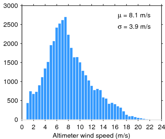
Figure 35. Histogram of science-valid wind over oceans and lakes for 12/02/2017. The mean ( \mu ) and standard deviation ( \sigma ) are also shown. Note that values larger than 24 m/s are excluded from the histogram for the sake of readability but not from the computation of \mu and \sigma .
