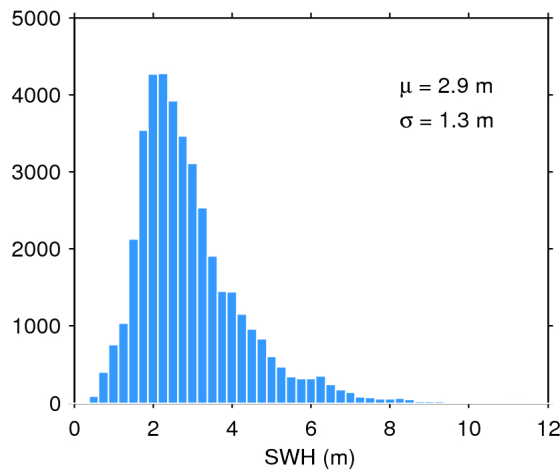
Figure 20. Histogram of science-valid SWH over oceans and lakes for 12/02/2017. The mean ( \mu ) and standard deviation ( \sigma ) are also shown. Note that values larger than 12 m are excluded from the histogram for the sake of readability but not from the computation of \mu and \sigma .
