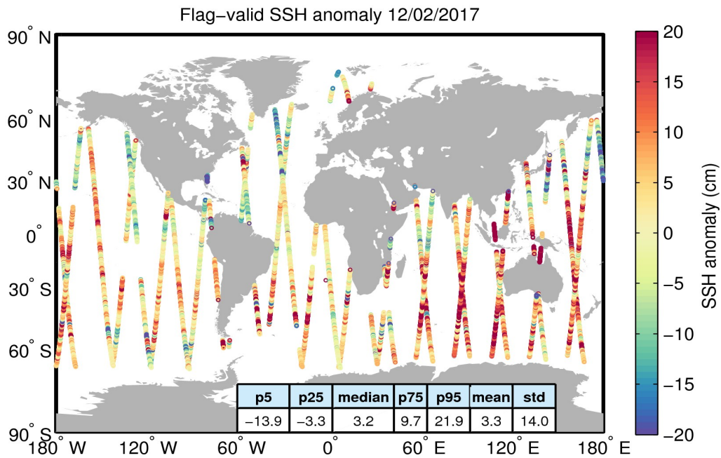
Figure 5. Geographical distribution of flag-valid 1-Hz SSH anomaly data over oceans and lakes for 12/02/2017. The statistical values shown in the table refer to the SSH anomaly in cm and are calculated over all measurements shown in the figure.
