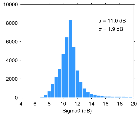
Figure 25. Histogram of flag-valid sigma0 over oceans and lakes for 12/02/2017. The mean ( \mu ) and standard deviation ( \sigma ) are also shown. Note that values outside [4 20] dB are excluded from the histogram for the sake of readability but not from the computation of \mu and \sigma .
