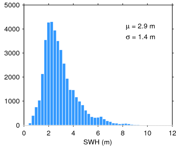
Figure 17. Histogram of flag-valid SWH over oceans and lakes for 12/02/2017. The mean ( \mu ) and standard deviation ( \sigma ) are also shown. Note that values larger than 12 m are excluded from the histogram for the sake of readability but not from the computation of \mu and \sigma .
