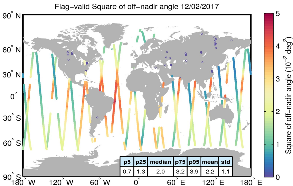
Figure 37. Geographical distribution of flag-valid mispointing data over oceans and lakes for 12/02/2017. The statistical values shown in the table refer to the mispointing in 10^{-2} deg 2 and are calculated over all measurements shown in the figure.
