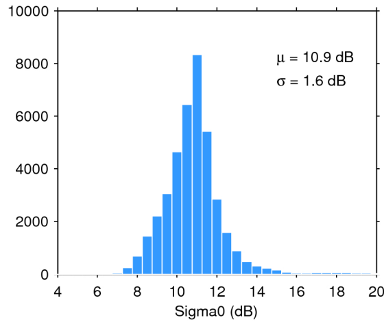
Figure 28. Histogram of science-valid sigma0 over oceans and lakes for 12/02/2017. The mean ( \mu ) and standard deviation ( \sigma ) are also shown. Note that values outside [4 20] dB are excluded from the histogram for the sake of readability but not from the computation of \mu and \sigma .
