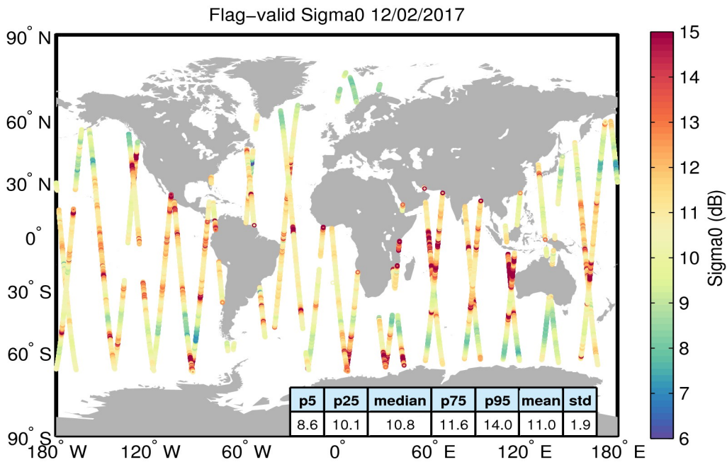
Figure 23. Geographical distribution of flag-valid sigma0 data over oceans and lakes for 12/02/2017. The statistical values shown in the table refer to the sigma0 in dB and are calculated over all measurements shown in the figure.
