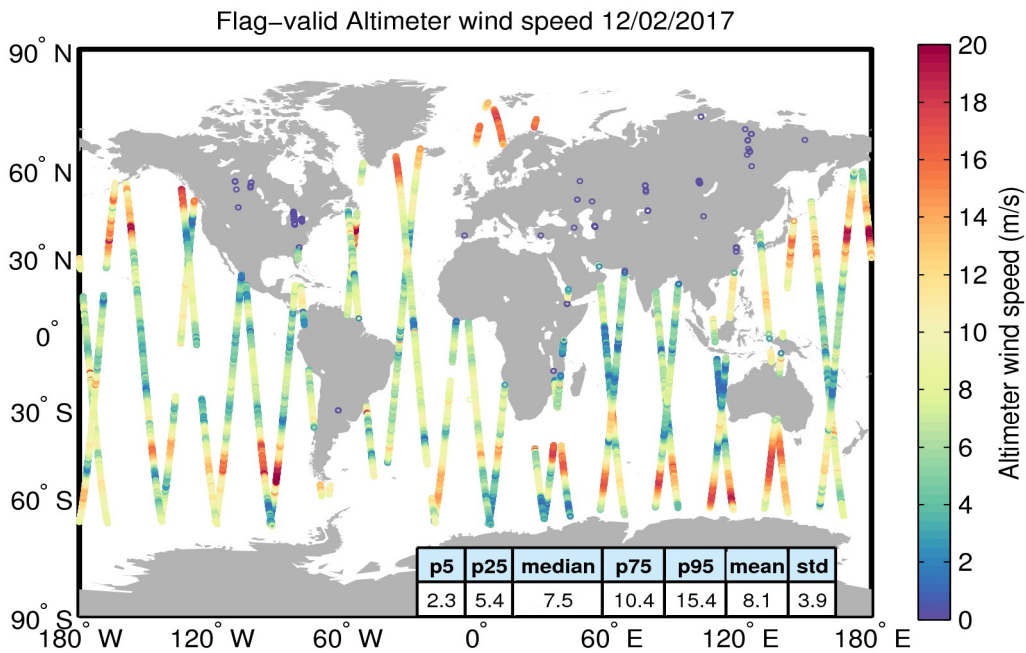
Figure 31. Geographical distribution of flag-valid wind data over oceans and lakes for 12/02/2017. The statistical values shown in the table refer to the wind in m/s and are calculated over all measurements shown in the figure.
