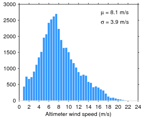
Figure 33. Histogram of flag-valid wind over oceans and lakes for 12/02/2017. The mean ( \mu ) and standard deviation ( \sigma ) are also shown. Note that values larger than 24 m/s are excluded from the histogram for the sake of readability but not from the computation of \mu and \sigma .
