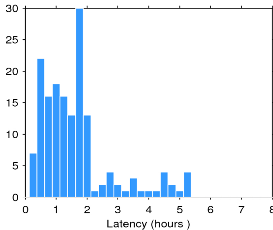
Figure 2. Histogram of the data latency for 12/02/2017. The y-axis denotes the number of files that are made available with a delay of x-hours with respect to the mean time of the records stored in the file.
