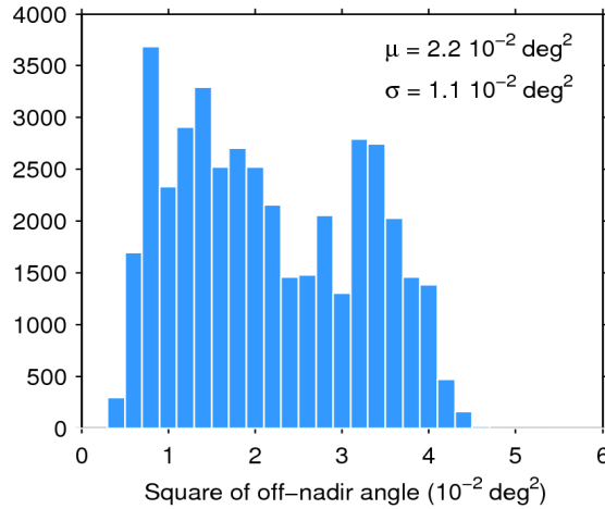
Figure 39. Histogram of flag-valid mispointing over oceans and lakes for 12/02/2017. The mean ( \mu ) and standard deviation ( \sigma ) are also shown. Note that values larger than 6 \cdot 10^{-2} \text{ deg}^2 are excluded from the histogram for the sake of readability but not from the computation of \mu and \sigma .
