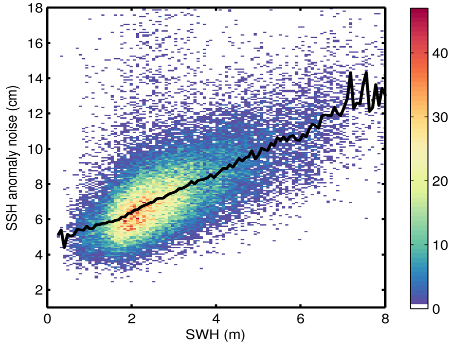
Figure 9. 2D histogram showing flag-valid SSH anomaly noise as a function of SWH for 12/02/2017. The black line denotes the median SSH anomaly noise as a function of SWH.
