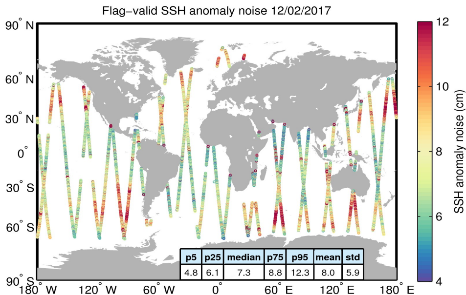
Figure 8. Geographical distribution of flag-valid 20-Hz SSH anomaly measurement noise over oceans and lakes for 12/02/2017. The statistical values shown in the table refer to the SSH anomaly noise and are calculated over all measurements shown in the figure.
