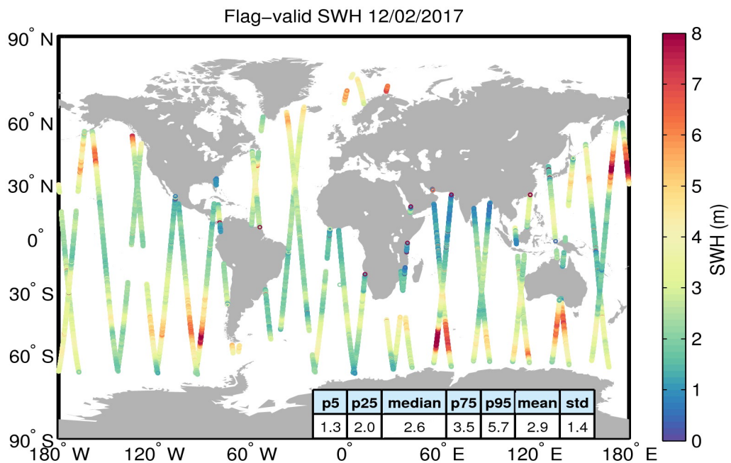
Figure 15. Geographical distribution of flag-valid SWH data over oceans and lakes for 12/02/2017. The statistical values shown in the table refer to the SWH in m and are calculated over all measurements shown in the figure.
