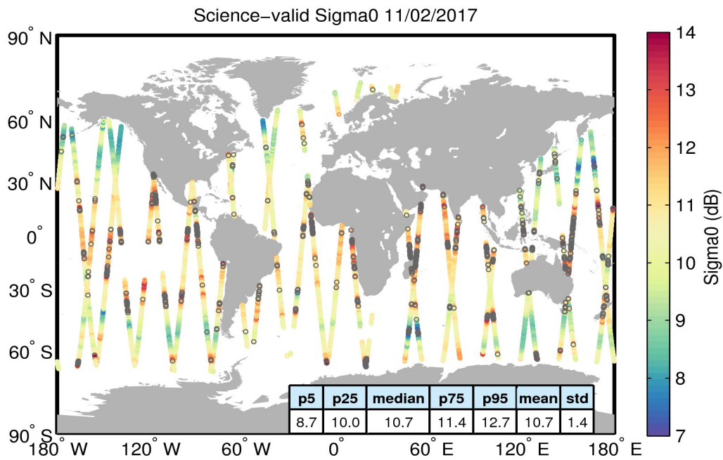
Figure 27. Geographical distribution of science-valid sigma0 data over oceans and lakes for 11/02/2017. The statistical values shown in the table refer to the sigma0 in dB and are calculated over all measurements shown in the figure. Gray circles denote records that have been rejected based on the editing criteria described in Table 4.
