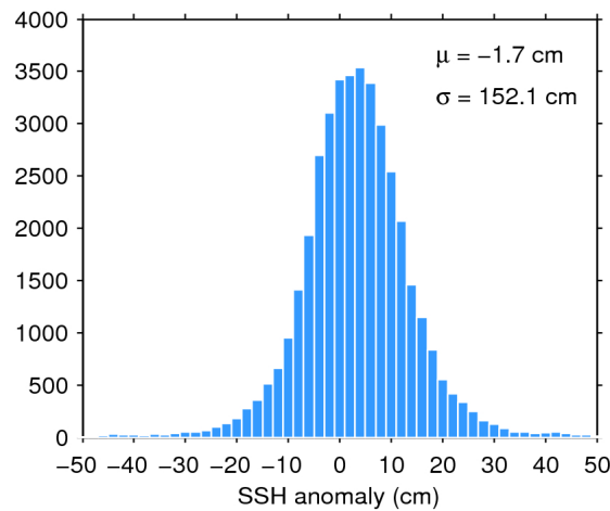
Figure 7. Histogram of flag-valid SSH anomaly over oceans and lakes for 11/02/2017. The mean ( \mu ) and standard deviation ( \sigma ) are also shown. Note that values outside [-50 50] cm are excluded from the histogram for the sake of readability but not from the computation of \mu and \sigma .
