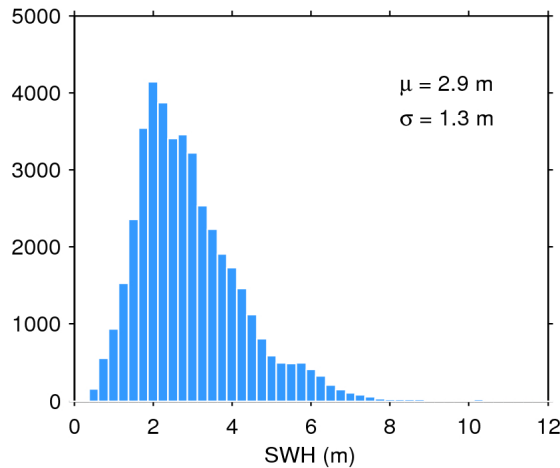
Figure 20. Histogram of science-valid SWH over oceans and lakes for 11/02/2017. The mean ( \mu ) and standard deviation ( \sigma ) are also shown. Note that values larger than 12 m are excluded from the histogram for the sake of readability but not from the computation of \mu and \sigma .
