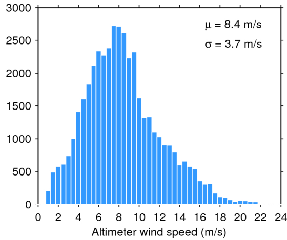
Figure 33. Histogram of flag-valid wind over oceans and lakes for 11/02/2017. The mean ( \mu ) and standard deviation ( \sigma ) are also shown. Note that values larger than 24 m/s are excluded from the histogram for the sake of readability but not from the computation of \mu and \sigma .
