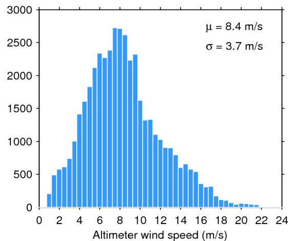
Figure 35. Histogram of science-valid wind over oceans and lakes for 11/02/2017. The mean ( \mu ) and standard deviation ( \sigma ) are also shown. Note that values larger than 24 m/s are excluded from the histogram for the sake of readability but not from the computation of \mu and \sigma .
