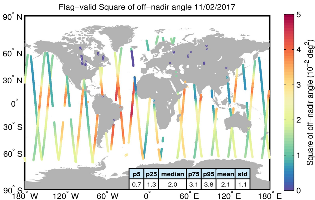
Figure 37. Geographical distribution of flag-valid mispointing data over oceans and lakes for 11/02/2017. The statistical values shown in the table refer to the mispointing in 10^{-2} deg 2 and are calculated over all measurements shown in the figure.
