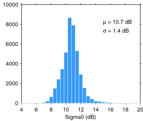
Figure 28. Histogram of science-valid sigma0 over oceans and lakes for 11/02/2017. The mean ( \mu ) and standard deviation ( \sigma ) are also shown. Note that values outside [4 20] dB are excluded from the histogram for the sake of readability but not from the computation of \mu and \sigma .
