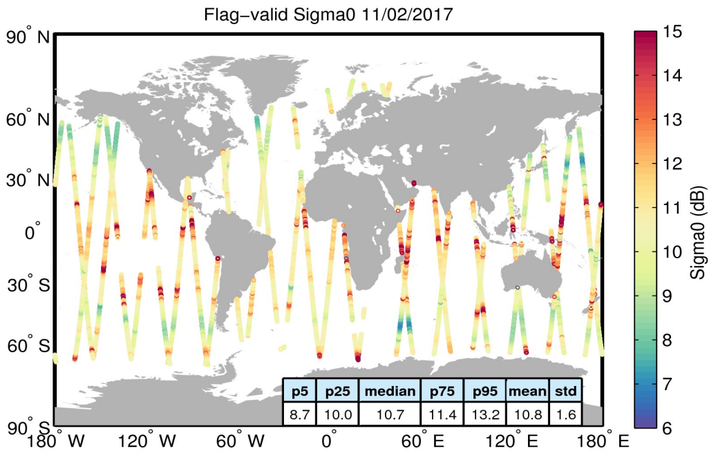
Figure 23. Geographical distribution of flag-valid sigma0 data over oceans and lakes for 11/02/2017. The statistical values shown in the table refer to the sigma0 in dB and are calculated over all measurements shown in the figure.
