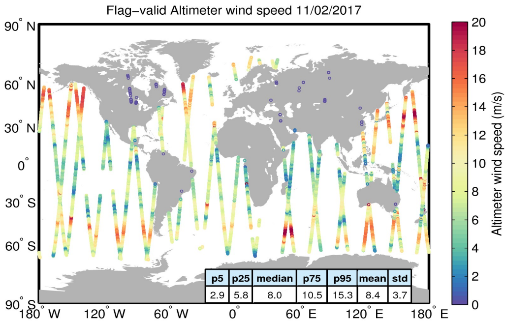
Figure 31. Geographical distribution of flag-valid wind data over oceans and lakes for 11/02/2017. The statistical values shown in the table refer to the wind in m/s and are calculated over all measurements shown in the figure.
