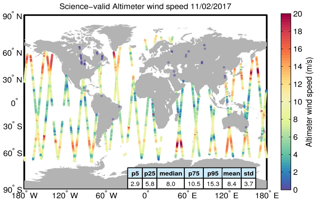
Figure 34. Geographical distribution of science-valid wind data over oceans and lakes for 11/02/2017. The statistical values shown in the table refer to the wind in m/s and are calculated over all measurements shown in the figure. Gray circles denote records that have been rejected based on the editing criteria described in Table 5.
