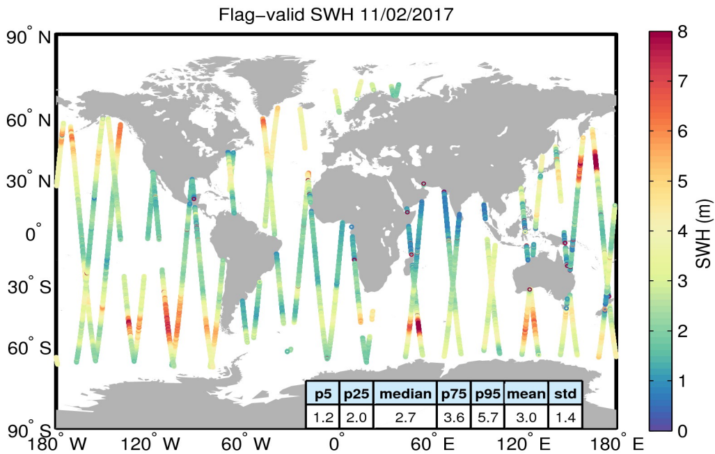
Figure 15. Geographical distribution of flag-valid SWH data over oceans and lakes for 11/02/2017. The statistical values shown in the table refer to the SWH in m and are calculated over all measurements shown in the figure.
