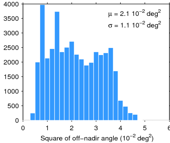
Figure 39. Histogram of flag-valid mispointing over oceans and lakes for 11/02/2017. The mean ( \mu ) and standard deviation ( \sigma ) are also shown. Note that values larger than 6 \cdot 10^{-2} \text{ deg}^2 are excluded from the histogram for the sake of readability but not from the computation of \mu and \sigma .
