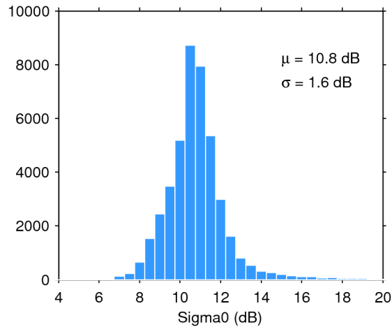
Figure 25. Histogram of flag-valid sigma0 over oceans and lakes for 11/02/2017. The mean ( \mu ) and standard deviation ( \sigma ) are also shown. Note that values outside [4 20] dB are excluded from the histogram for the sake of readability but not from the computation of \mu and \sigma .
