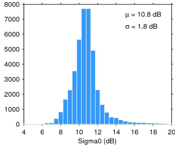
Figure 25. Histogram of flag-valid sigma0 over oceans and lakes for 10/02/2017. The mean ( \mu ) and standard deviation ( \sigma ) are also shown. Note that values outside [4 20] dB are excluded from the histogram for the sake of readability but not from the computation of \mu and \sigma .
