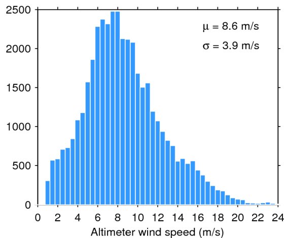
Figure 35. Histogram of science-valid wind over oceans and lakes for 10/02/2017. The mean ( \mu ) and standard deviation ( \sigma ) are also shown. Note that values larger than 24 m/s are excluded from the histogram for the sake of readability but not from the computation of \mu and \sigma .
