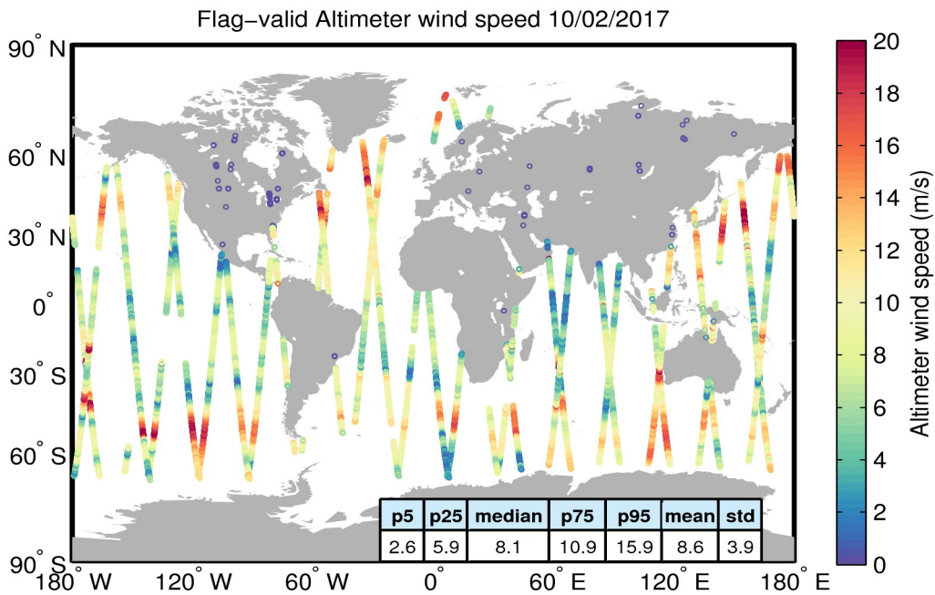
Figure 31. Geographical distribution of flag-valid wind data over oceans and lakes for 10/02/2017. The statistical values shown in the table refer to the wind in m/s and are calculated over all measurements shown in the figure.
