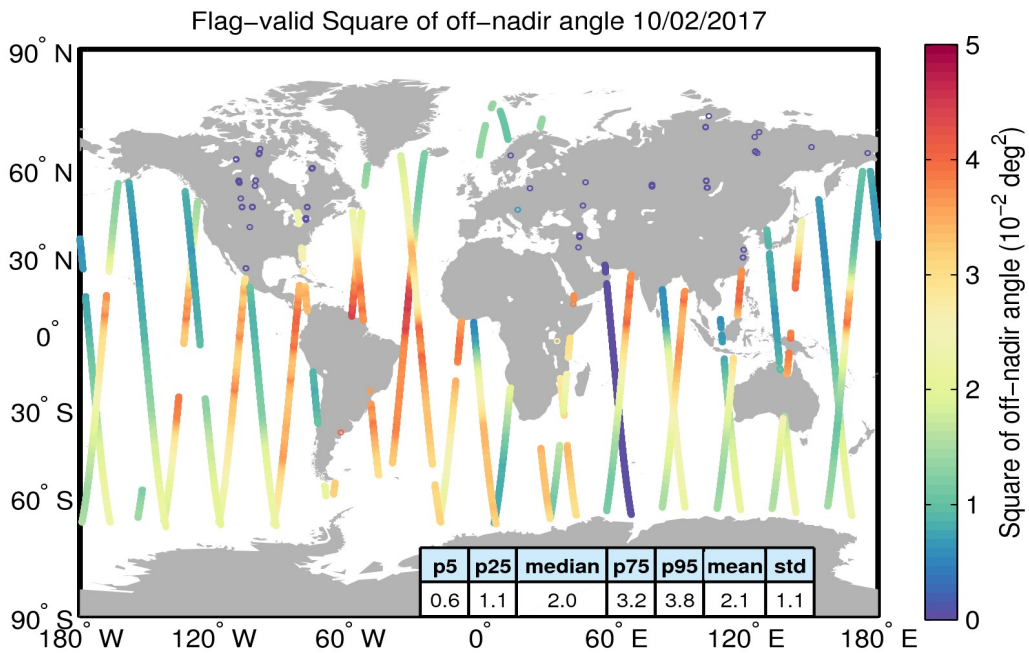
Figure 37. Geographical distribution of flag-valid mispointing data over oceans and lakes for 10/02/2017. The statistical values shown in the table refer to the mispointing in 10^{-2} deg 2 and are calculated over all measurements shown in the figure.
