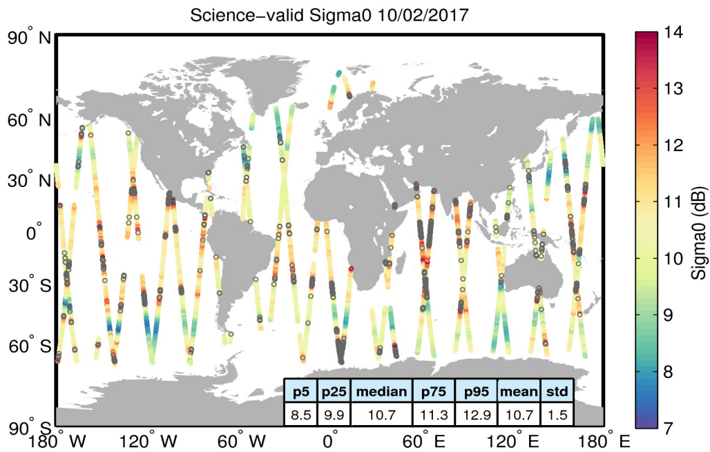
Figure 27. Geographical distribution of science-valid sigma0 data over oceans and lakes for 10/02/2017. The statistical values shown in the table refer to the sigma0 in dB and are calculated over all measurements shown in the figure. Gray circles denote records that have been rejected based on the editing criteria described in Table 4.
