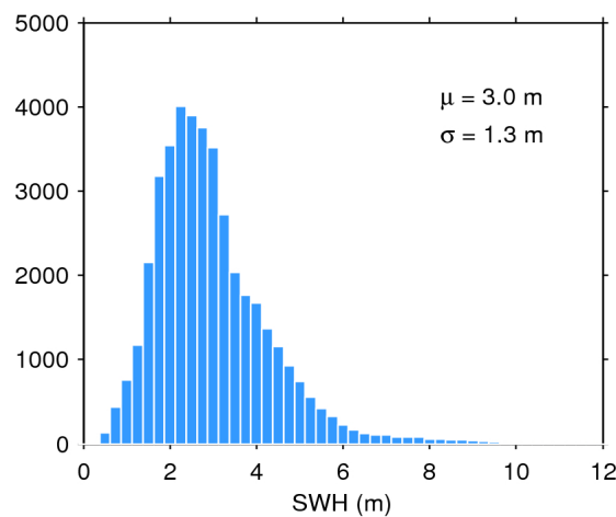
Figure 17. Histogram of flag-valid SWH over oceans and lakes for 10/02/2017. The mean ( \mu ) and standard deviation ( \sigma ) are also shown. Note that values larger than 12 m are excluded from the histogram for the sake of readability but not from the computation of \mu and \sigma .
