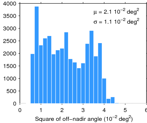
Figure 39. Histogram of flag-valid mispointing over oceans and lakes for 10/02/2017. The mean ( \mu ) and standard deviation ( \sigma ) are also shown. Note that values larger than 6 \cdot 10^{-2} \text{ deg}^2 are excluded from the histogram for the sake of readability but not from the computation of \mu and \sigma .
