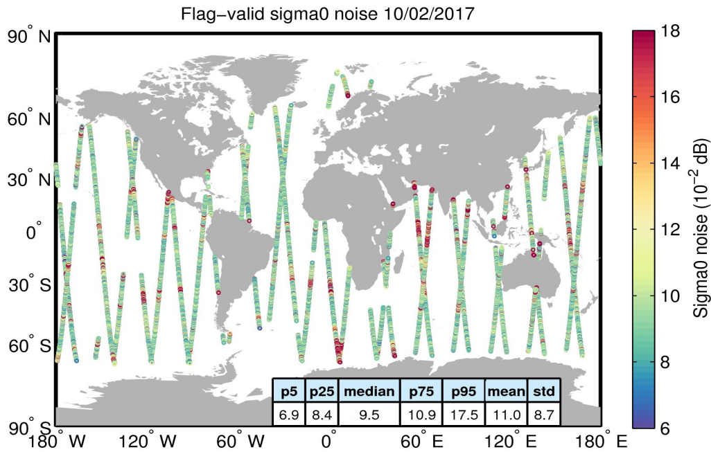
Figure 26. Geographical distribution of flag-valid 20-Hz sigma0 measurement noise over oceans and lakes for 10/02/2017. The statistical values shown in the table refer to the sigma0 noise and are calculated over all measurements shown in the figure.
