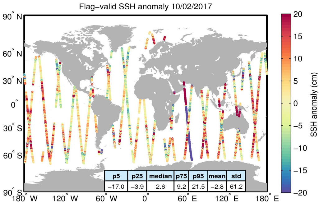
Figure 5. Geographical distribution of flag-valid 1-Hz SSH anomaly data over oceans and lakes for 10/02/2017. The statistical values shown in the table refer to the SSH anomaly in cm and are calculated over all measurements shown in the figure.
