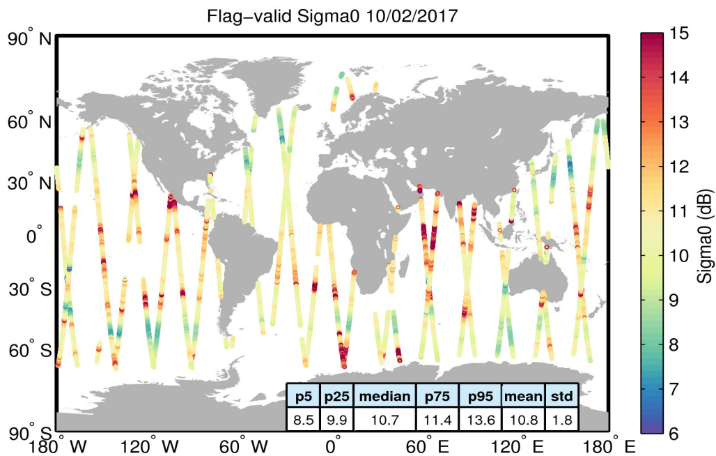
Figure 23. Geographical distribution of flag-valid sigma0 data over oceans and lakes for 10/02/2017. The statistical values shown in the table refer to the sigma0 in dB and are calculated over all measurements shown in the figure.
