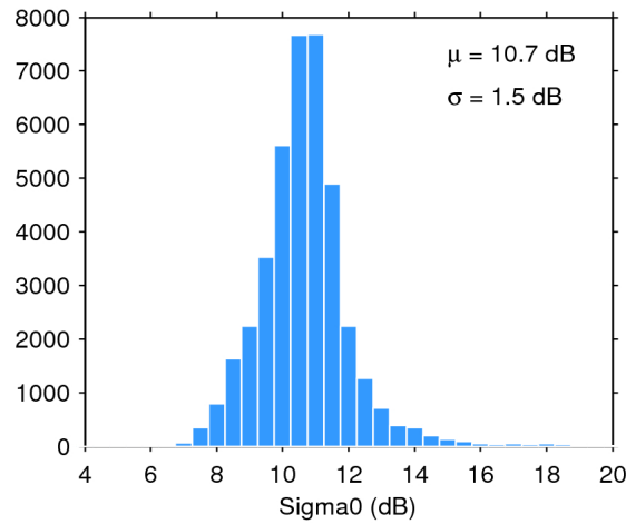
Figure 28. Histogram of science-valid sigma0 over oceans and lakes for 10/02/2017. The mean ( \mu ) and standard deviation ( \sigma ) are also shown. Note that values outside [4 20] dB are excluded from the histogram for the sake of readability but not from the computation of \mu and \sigma .
