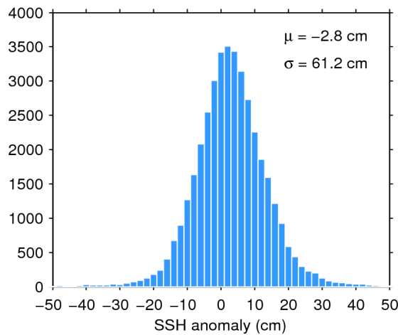
Figure 7. Histogram of flag-valid SSH anomaly over oceans and lakes for 10/02/2017. The mean ( \mu ) and standard deviation ( \sigma ) are also shown. Note that values outside [-50 50] cm are excluded from the histogram for the sake of readability but not from the computation of \mu and \sigma .
