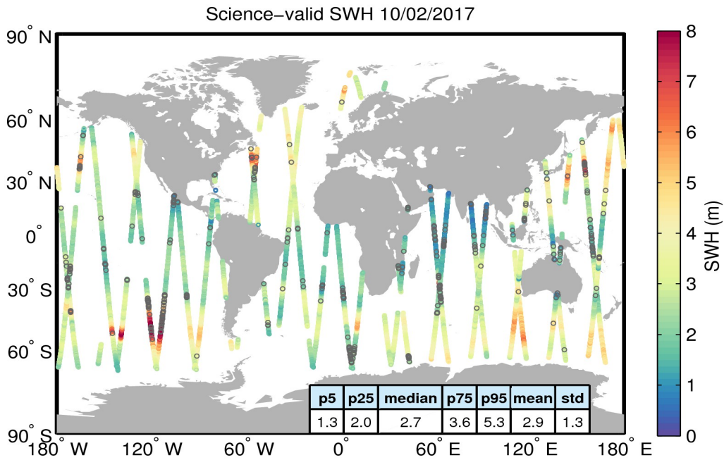
Figure 19. Geographical distribution of science-valid SWH data over oceans and lakes for 10/02/2017. The statistical values shown in the table refer to the SWH in m and are calculated over all measurements shown in the figure. Gray circles denote records that have been rejected based on the editing criteria described in Table 3.
