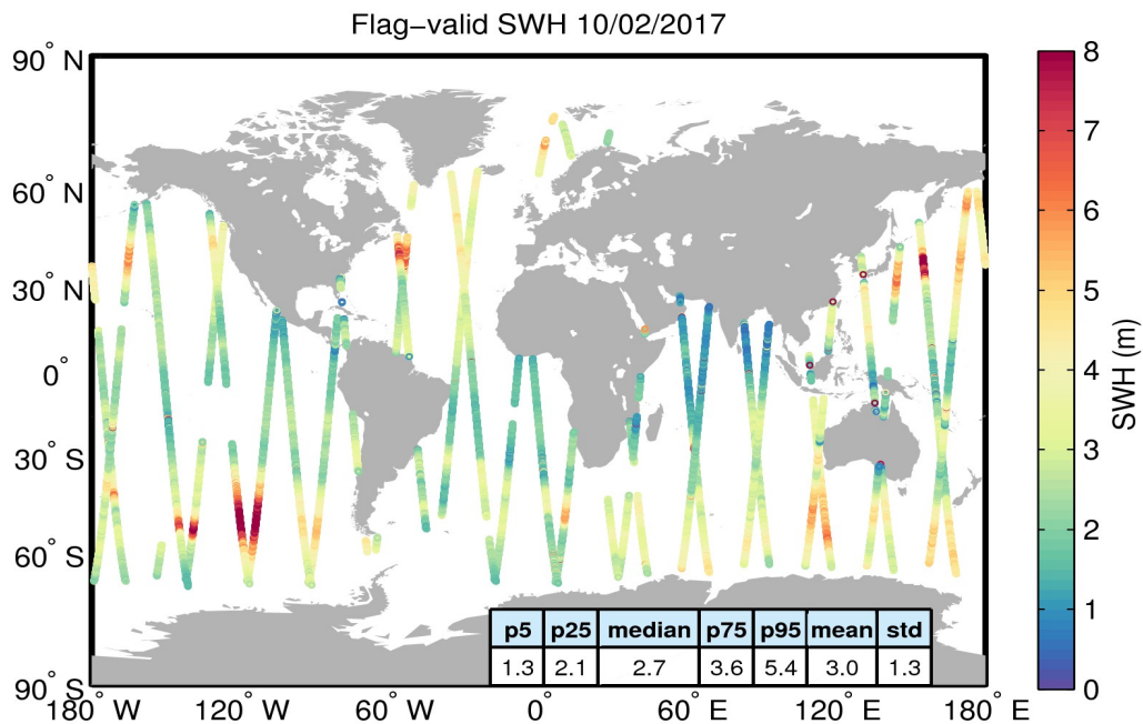
Figure 15. Geographical distribution of flag-valid SWH data over oceans and lakes for 10/02/2017. The statistical values shown in the table refer to the SWH in m and are calculated over all measurements shown in the figure.
