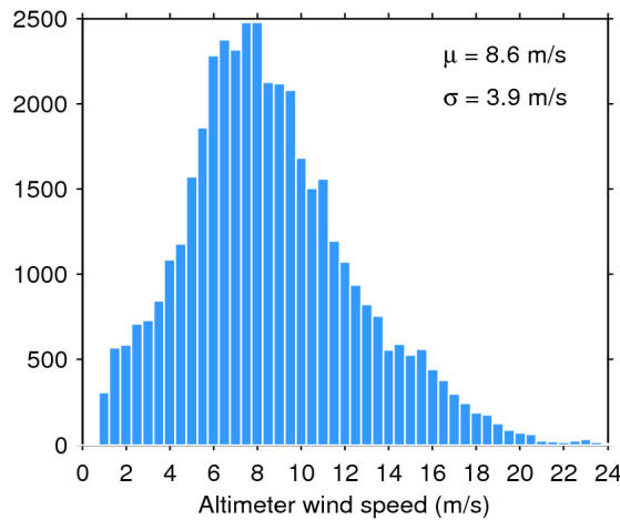
Figure 33. Histogram of flag-valid wind over oceans and lakes for 10/02/2017. The mean ( \mu ) and standard deviation ( \sigma ) are also shown. Note that values larger than 24 m/s are excluded from the histogram for the sake of readability but not from the computation of \mu and \sigma .
