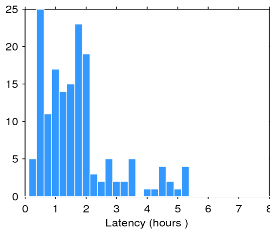
Figure 2. Histogram of the data latency for 10/02/2017. The y-axis denotes the number of files that are made available with a delay of x-hours with respect to the mean time of the records stored in the file.
