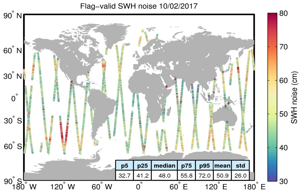
Figure 18. Geographical distribution of flag-valid 20-Hz SWH measurement noise over oceans and lakes for 10/02/2017. The statistical values shown in the table refer to the SWH noise and are calculated over all measurements shown in the figure.
