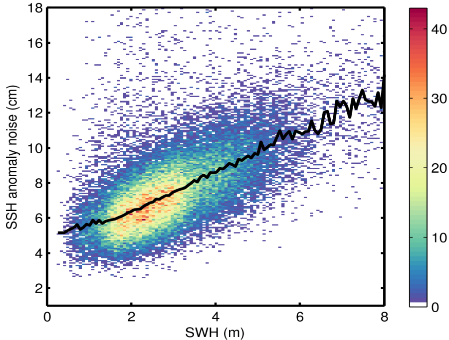
Figure 9. 2D histogram showing flag-valid SSH anomaly noise as a function of SWH for 10/02/2017. The black line denotes the median SSH anomaly noise as a function of SWH.
