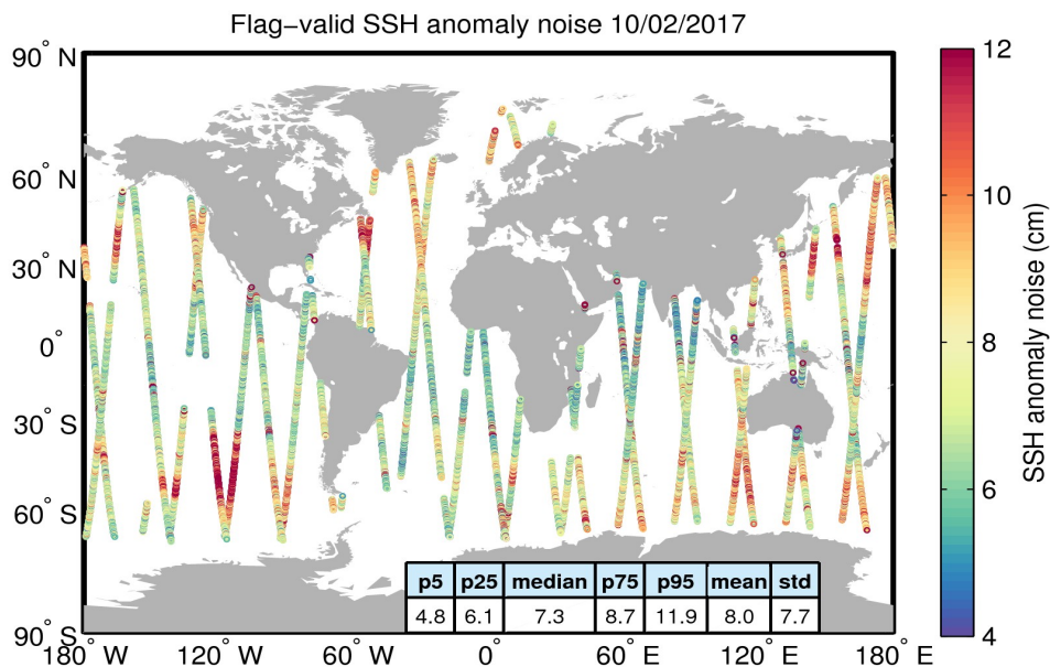
Figure 8. Geographical distribution of flag-valid 20-Hz SSH anomaly measurement noise over oceans and lakes for 10/02/2017. The statistical values shown in the table refer to the SSH anomaly noise and are calculated over all measurements shown in the figure.
