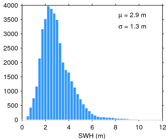
Figure 20. Histogram of science-valid SWH over oceans and lakes for 10/02/2017. The mean ( \mu ) and standard deviation ( \sigma ) are also shown. Note that values larger than 12 m are excluded from the histogram for the sake of readability but not from the computation of \mu and \sigma .
