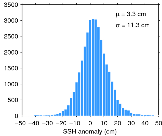
Figure 11. Histogram of science-valid SSH anomaly over oceans and lakes for 10/02/2017. The mean ( \mu ) and standard deviation ( \sigma ) are also shown. Note that values outside [-50 50] cm are excluded from the histogram for the sake of readability but not from the computation of \mu and \sigma .
