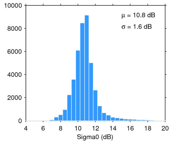
Figure 25. Histogram of flag-valid sigma0 over oceans and lakes for 09/02/2017. The mean ( \mu ) and standard deviation ( \sigma ) are also shown. Note that values outside [4 20] dB are excluded from the histogram for the sake of readability but not from the computation of \mu and \sigma .
