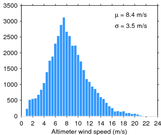
Figure 35. Histogram of science-valid wind over oceans and lakes for 09/02/2017. The mean ( \mu ) and standard deviation ( \sigma ) are also shown. Note that values larger than 24 m/s are excluded from the histogram for the sake of readability but not from the computation of \mu and \sigma .
