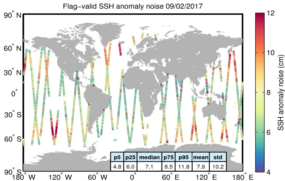
Figure 8. Geographical distribution of flag-valid 20-Hz SSH anomaly measurement noise over oceans and lakes for 09/02/2017. The statistical values shown in the table refer to the SSH anomaly noise and are calculated over all measurements shown in the figure.
