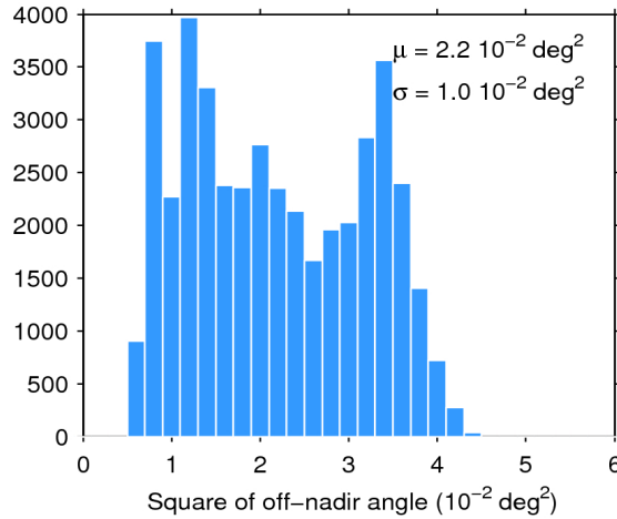
Figure 39. Histogram of flag-valid mispointing over oceans and lakes for 09/02/2017. The mean ( \mu ) and standard deviation ( \sigma ) are also shown. Note that values larger than 6 \cdot 10^{-2} \text{ deg}^2 are excluded from the histogram for the sake of readability but not from the computation of \mu and \sigma .
