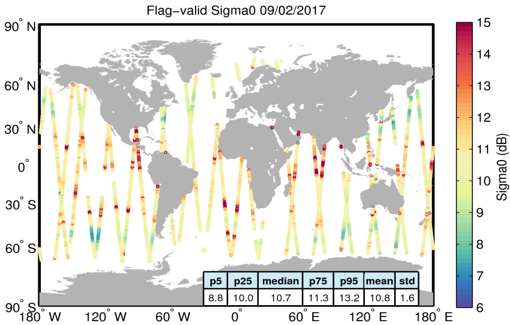
Figure 23. Geographical distribution of flag-valid sigma0 data over oceans and lakes for 09/02/2017. The statistical values shown in the table refer to the sigma0 in dB and are calculated over all measurements shown in the figure.
