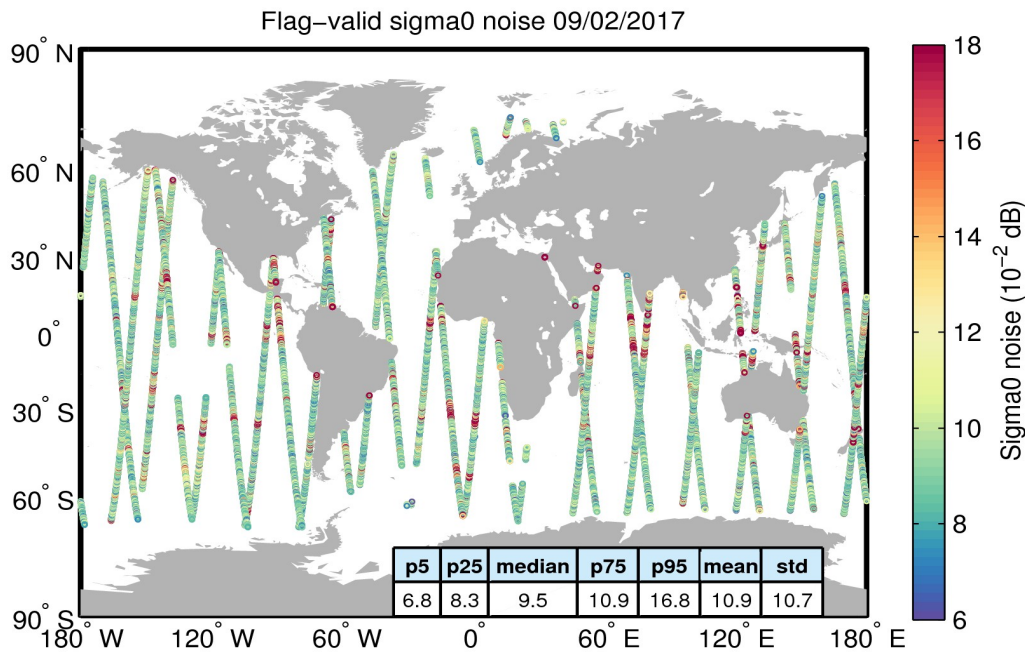
Figure 26. Geographical distribution of flag-valid 20-Hz sigma0 measurement noise over oceans and lakes for 09/02/2017. The statistical values shown in the table refer to the sigma0 noise and are calculated over all measurements shown in the figure.
