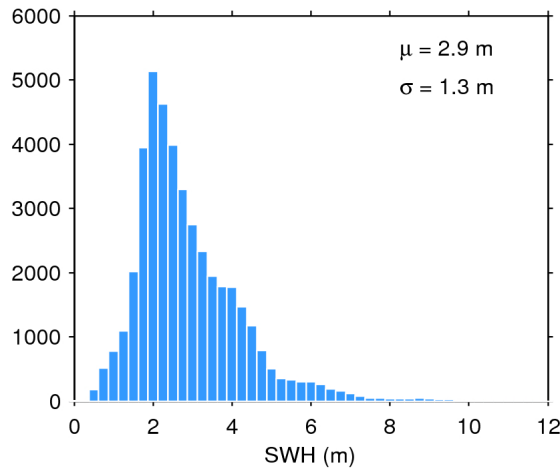
Figure 20. Histogram of science-valid SWH over oceans and lakes for 09/02/2017. The mean ( \mu ) and standard deviation ( \sigma ) are also shown. Note that values larger than 12 m are excluded from the histogram for the sake of readability but not from the computation of \mu and \sigma .
