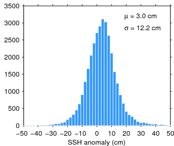
Figure 11. Histogram of science-valid SSH anomaly over oceans and lakes for 09/02/2017. The mean ( \mu ) and standard deviation ( \sigma ) are also shown. Note that values outside [-50 50] cm are excluded from the histogram for the sake of readability but not from the computation of \mu and \sigma .
