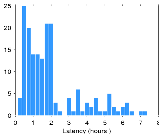
Figure 2. Histogram of the data latency for 09/02/2017. The y-axis denotes the number of files that are made available with a delay of x-hours with respect to the mean time of the records stored in the file.
