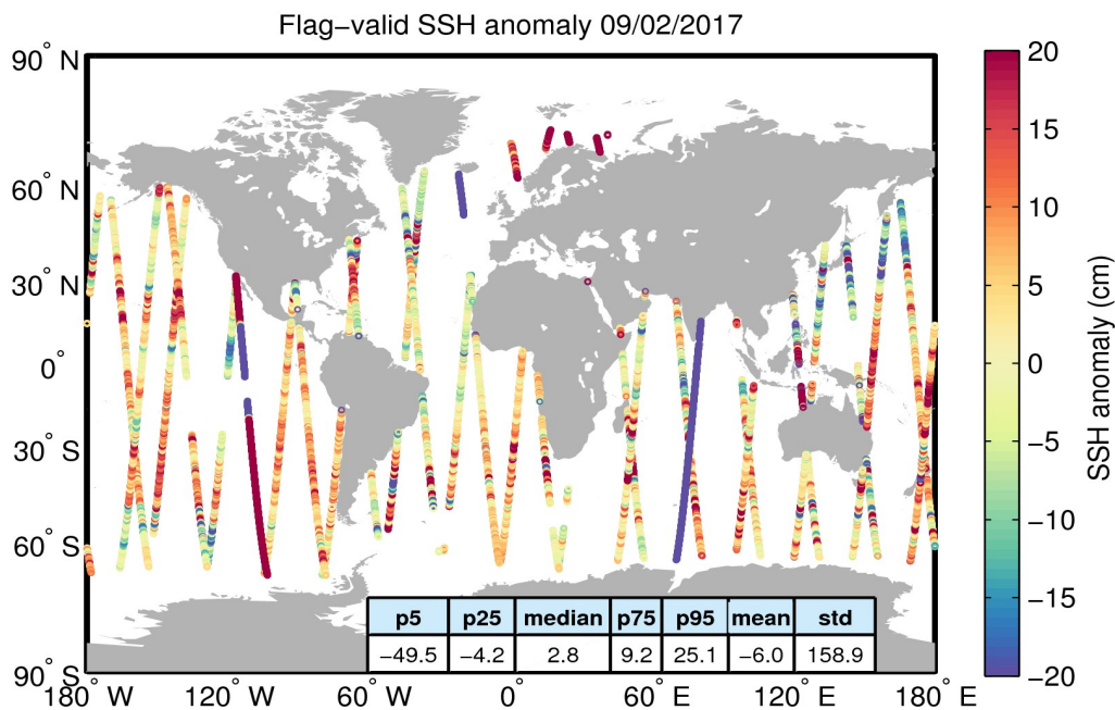
Figure 5. Geographical distribution of flag-valid 1-Hz SSH anomaly data over oceans and lakes for 09/02/2017. The statistical values shown in the table refer to the SSH anomaly in cm and are calculated over all measurements shown in the figure.
