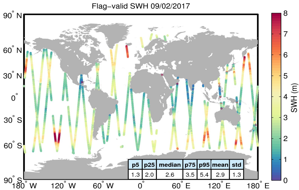
Figure 15. Geographical distribution of flag-valid SWH data over oceans and lakes for 09/02/2017. The statistical values shown in the table refer to the SWH in m and are calculated over all measurements shown in the figure.
