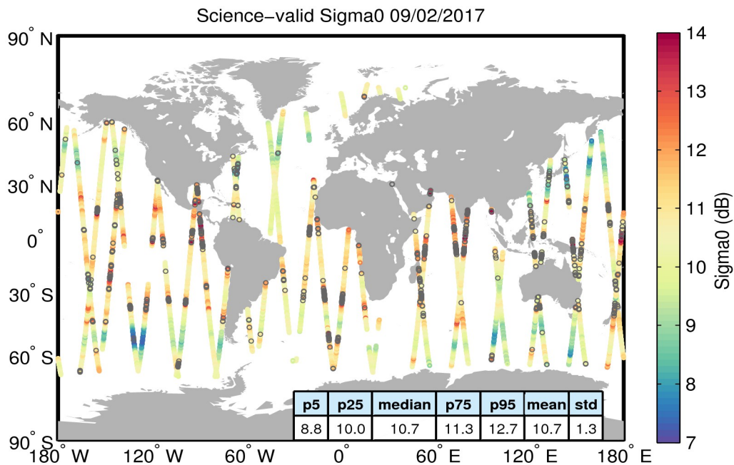
Figure 27. Geographical distribution of science-valid sigma0 data over oceans and lakes for 09/02/2017. The statistical values shown in the table refer to the sigma0 in dB and are calculated over all measurements shown in the figure. Gray circles denote records that have been rejected based on the editing criteria described in Table 4.
