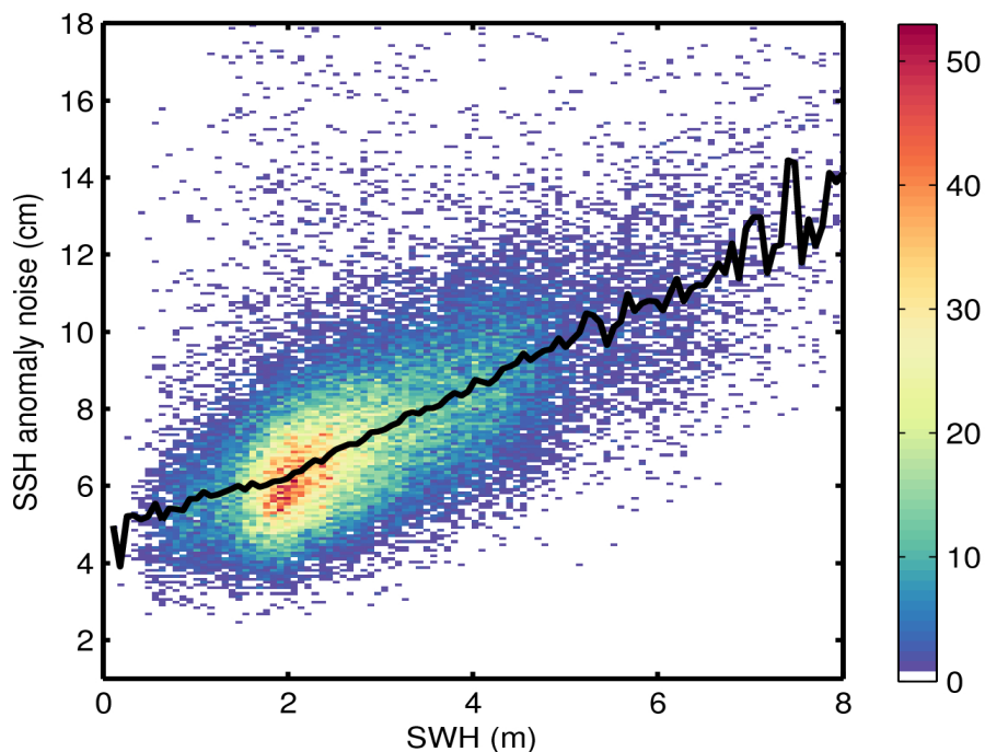
Figure 9. 2D histogram showing flag-valid SSH anomaly noise as a function of SWH for 09/02/2017. The black line denotes the median SSH anomaly noise as a function of SWH.
