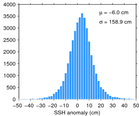
Figure 7. Histogram of flag-valid SSH anomaly over oceans and lakes for 09/02/2017. The mean ( \mu ) and standard deviation ( \sigma ) are also shown. Note that values outside [-50 50] cm are excluded from the histogram for the sake of readability but not from the computation of \mu and \sigma .
