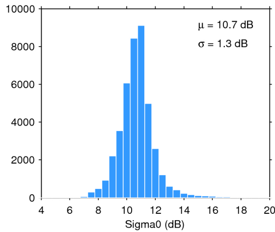
Figure 28. Histogram of science-valid sigma0 over oceans and lakes for 09/02/2017. The mean ( \mu ) and standard deviation ( \sigma ) are also shown. Note that values outside [4 20] dB are excluded from the histogram for the sake of readability but not from the computation of \mu and \sigma .
