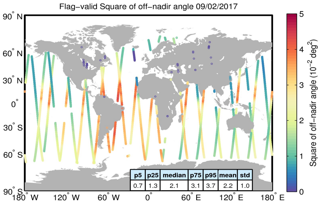
Figure 37. Geographical distribution of flag-valid mispointing data over oceans and lakes for 09/02/2017. The statistical values shown in the table refer to the mispointing in 10^{-2} deg 2 and are calculated over all measurements shown in the figure.
