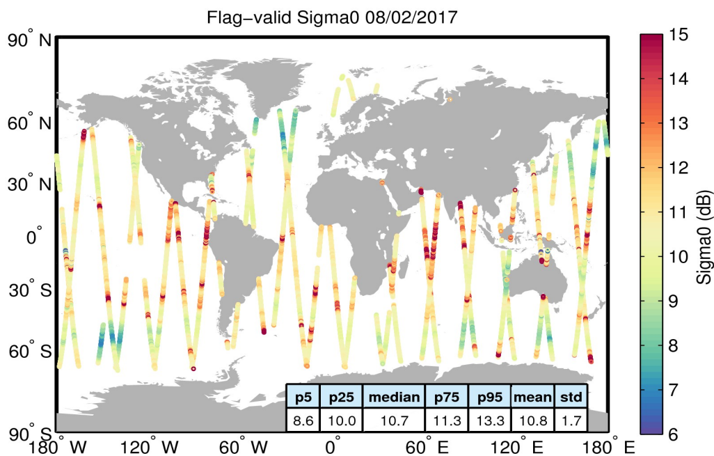
Figure 23. Geographical distribution of flag-valid sigma0 data over oceans and lakes for 08/02/2017. The statistical values shown in the table refer to the sigma0 in dB and are calculated over all measurements shown in the figure.
