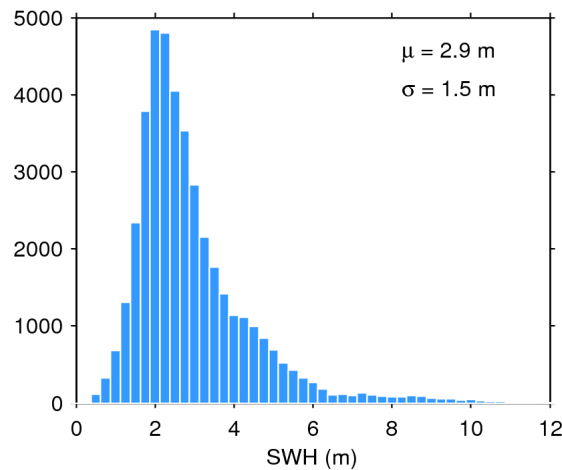
Figure 20. Histogram of science-valid SWH over oceans and lakes for 08/02/2017. The mean ( \mu ) and standard deviation ( \sigma ) are also shown. Note that values larger than 12 m are excluded from the histogram for the sake of readability but not from the computation of \mu and \sigma .
