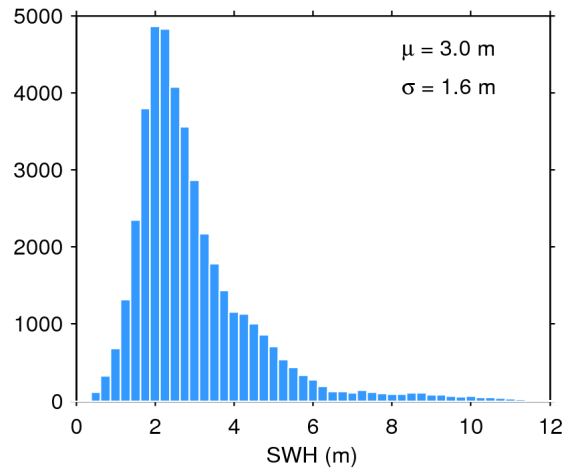
Figure 17. Histogram of flag-valid SWH over oceans and lakes for 08/02/2017. The mean ( \mu ) and standard deviation ( \sigma ) are also shown. Note that values larger than 12 m are excluded from the histogram for the sake of readability but not from the computation of \mu and \sigma .
