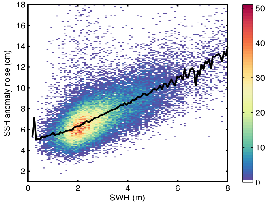
Figure 9. 2D histogram showing flag-valid SSH anomaly noise as a function of SWH for 08/02/2017. The black line denotes the median SSH anomaly noise as a function of SWH.
