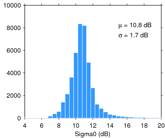
Figure 25. Histogram of flag-valid sigma0 over oceans and lakes for 08/02/2017. The mean ( \mu ) and standard deviation ( \sigma ) are also shown. Note that values outside [4 20] dB are excluded from the histogram for the sake of readability but not from the computation of \mu and \sigma .
