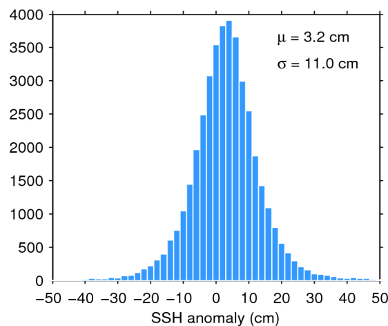
Figure 11. Histogram of science-valid SSH anomaly over oceans and lakes for 08/02/2017. The mean ( \mu ) and standard deviation ( \sigma ) are also shown. Note that values outside [-50 50] cm are excluded from the histogram for the sake of readability but not from the computation of \mu and \sigma .
