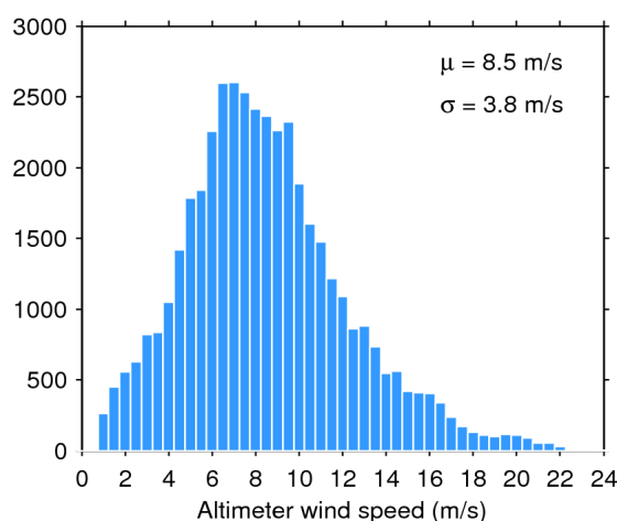
Figure 35. Histogram of science-valid wind over oceans and lakes for 08/02/2017. The mean ( \mu ) and standard deviation ( \sigma ) are also shown. Note that values larger than 24 m/s are excluded from the histogram for the sake of readability but not from the computation of \mu and \sigma .
