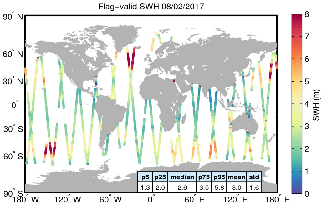
Figure 15. Geographical distribution of flag-valid SWH data over oceans and lakes for 08/02/2017. The statistical values shown in the table refer to the SWH in m and are calculated over all measurements shown in the figure.
