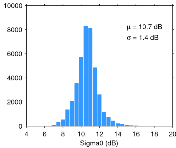
Figure 28. Histogram of science-valid sigma0 over oceans and lakes for 08/02/2017. The mean ( \mu ) and standard deviation ( \sigma ) are also shown. Note that values outside [4 20] dB are excluded from the histogram for the sake of readability but not from the computation of \mu and \sigma .
