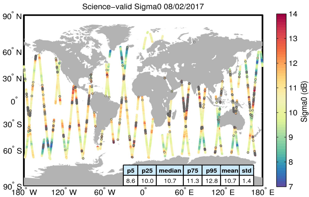
Figure 27. Geographical distribution of science-valid sigma0 data over oceans and lakes for 08/02/2017. The statistical values shown in the table refer to the sigma0 in dB and are calculated over all measurements shown in the figure. Gray circles denote records that have been rejected based on the editing criteria described in Table 4.
