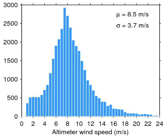
Figure 33. Histogram of flag-valid wind over oceans and lakes for 07/02/2017. The mean ( \mu ) and standard deviation ( \sigma ) are also shown. Note that values larger than 24 m/s are excluded from the histogram for the sake of readability but not from the computation of \mu and \sigma .
