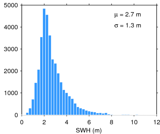
Figure 20. Histogram of science-valid SWH over oceans and lakes for 07/02/2017. The mean ( \mu ) and standard deviation ( \sigma ) are also shown. Note that values larger than 12 m are excluded from the histogram for the sake of readability but not from the computation of \mu and \sigma .
