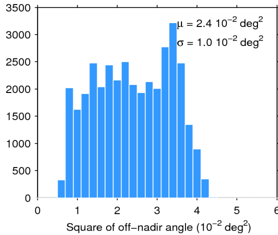
Figure 39. Histogram of flag-valid mispointing over oceans and lakes for 07/02/2017. The mean ( \mu ) and standard deviation ( \sigma ) are also shown. Note that values larger than 6 \cdot 10^{-2} \text{ deg}^2 are excluded from the histogram for the sake of readability but not from the computation of \mu and \sigma .
