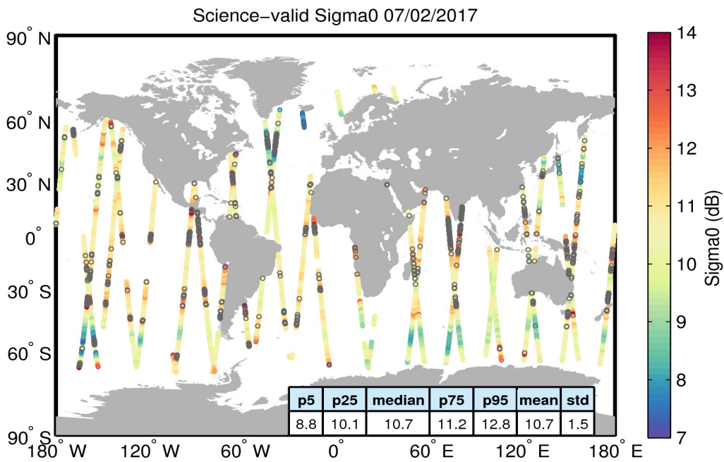
Figure 27. Geographical distribution of science-valid sigma0 data over oceans and lakes for 07/02/2017. The statistical values shown in the table refer to the sigma0 in dB and are calculated over all measurements shown in the figure. Gray circles denote records that have been rejected based on the editing criteria described in Table 4.
