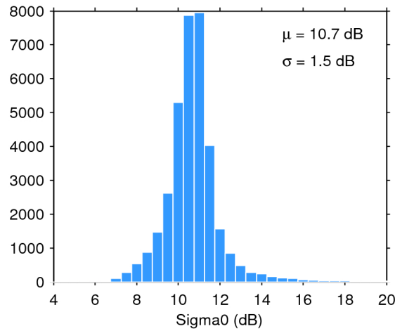
Figure 28. Histogram of science-valid sigma0 over oceans and lakes for 07/02/2017. The mean ( \mu ) and standard deviation ( \sigma ) are also shown. Note that values outside [4 20] dB are excluded from the histogram for the sake of readability but not from the computation of \mu and \sigma .
