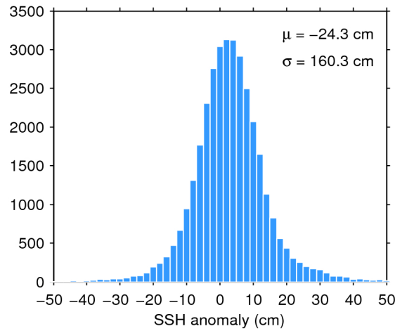
Figure 7. Histogram of flag-valid SSH anomaly over oceans and lakes for 07/02/2017. The mean ( \mu ) and standard deviation ( \sigma ) are also shown. Note that values outside [-50\ 50] cm are excluded from the histogram for the sake of readability but not from the computation of \mu and \sigma .
