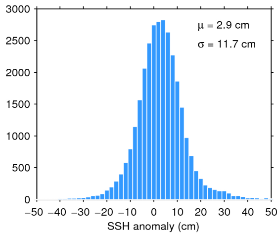
Figure 11. Histogram of science-valid SSH anomaly over oceans and lakes for 07/02/2017. The mean ( \mu ) and standard deviation ( \sigma ) are also shown. Note that values outside [-50 50] cm are excluded from the histogram for the sake of readability but not from the computation of \mu and \sigma .
