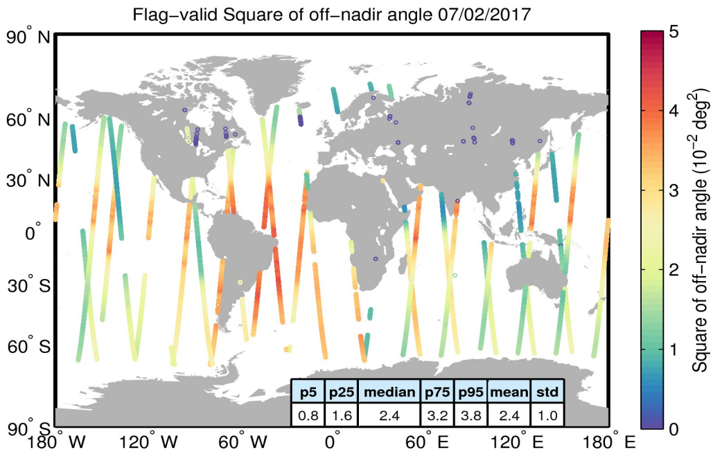
Figure 37. Geographical distribution of flag-valid mispointing data over oceans and lakes for 07/02/2017. The statistical values shown in the table refer to the mispointing in 10^{-2} \text{ deg}^2 and are calculated over all measurements shown in the figure.
