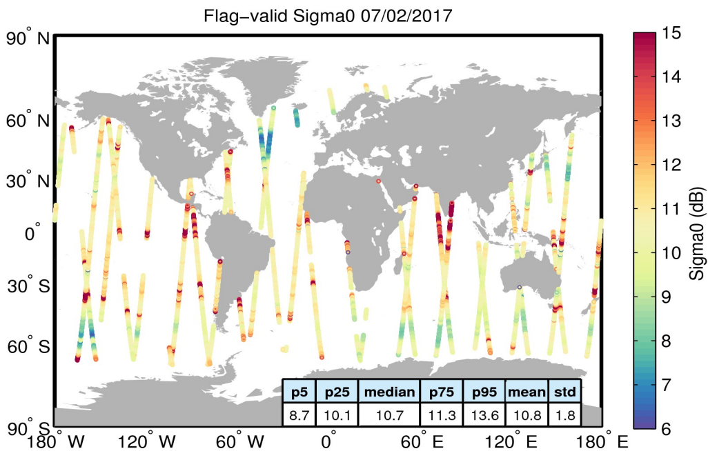
Figure 23. Geographical distribution of flag-valid sigma0 data over oceans and lakes for 07/02/2017. The statistical values shown in the table refer to the sigma0 in dB and are calculated over all measurements shown in the figure.
