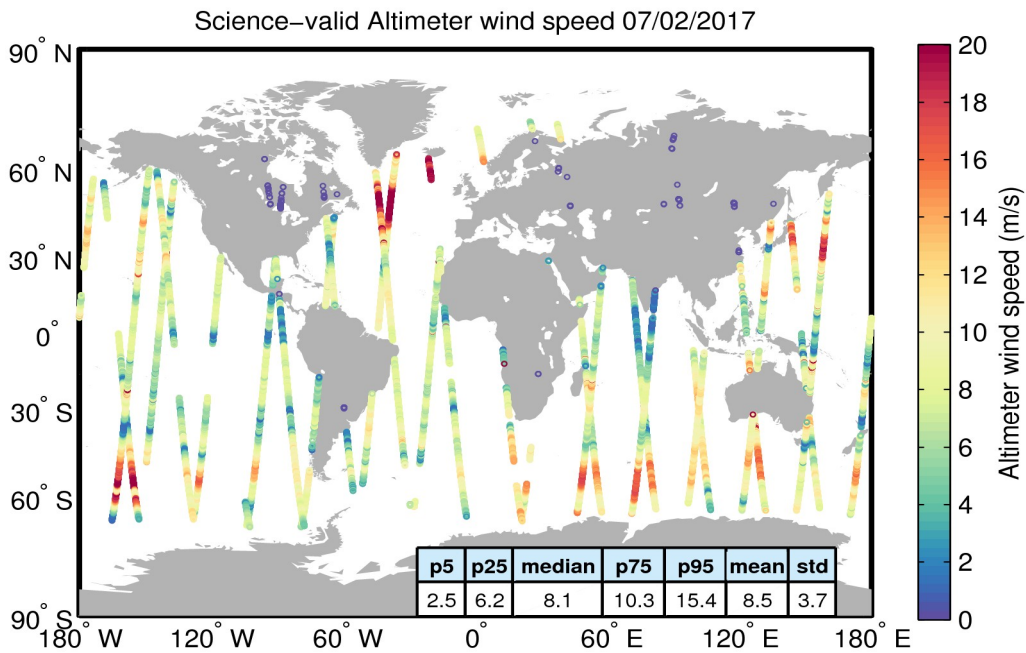
Figure 34. Geographical distribution of science-valid wind data over oceans and lakes for 07/02/2017. The statistical values shown in the table refer to the wind in m/s and are calculated over all measurements shown in the figure. Gray circles denote records that have been rejected based on the editing criteria described in Table 5.
