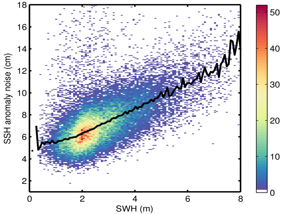
Figure 9. 2D histogram showing flag-valid SSH anomaly noise as a function of SWH for 07/02/2017. The black line denotes the median SSH anomaly noise as a function of SWH.
