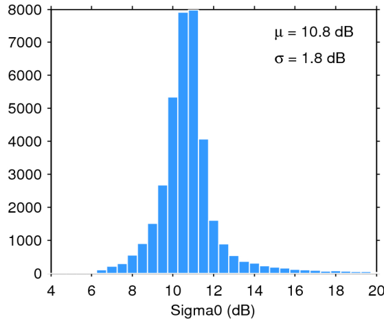
Figure 25. Histogram of flag-valid sigma0 over oceans and lakes for 07/02/2017. The mean ( \mu ) and standard deviation ( \sigma ) are also shown. Note that values outside [4 20] dB are excluded from the histogram for the sake of readability but not from the computation of \mu and \sigma .
