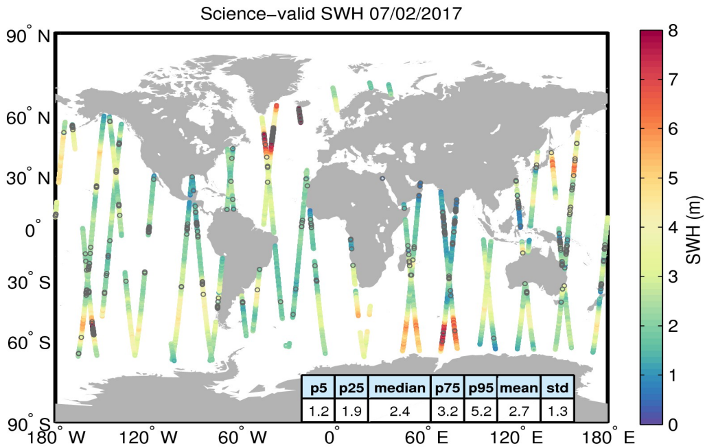
Figure 19. Geographical distribution of science-valid SWH data over oceans and lakes for 07/02/2017. The statistical values shown in the table refer to the SWH in m and are calculated over all measurements shown in the figure. Gray circles denote records that have been rejected based on the editing criteria described in Table 3.
