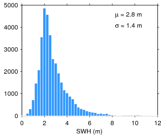
Figure 17. Histogram of flag-valid SWH over oceans and lakes for 07/02/2017. The mean ( \mu ) and standard deviation ( \sigma ) are also shown. Note that values larger than 12 m are excluded from the histogram for the sake of readability but not from the computation of \mu and \sigma .
