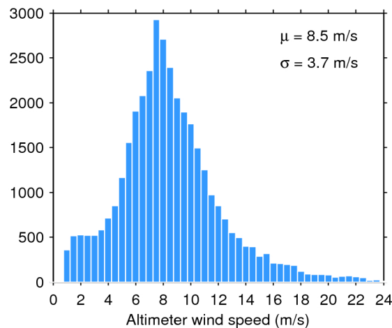
Figure 35. Histogram of science-valid wind over oceans and lakes for 07/02/2017. The mean ( \mu ) and standard deviation ( \sigma ) are also shown. Note that values larger than 24 m/s are excluded from the histogram for the sake of readability but not from the computation of \mu and \sigma .
