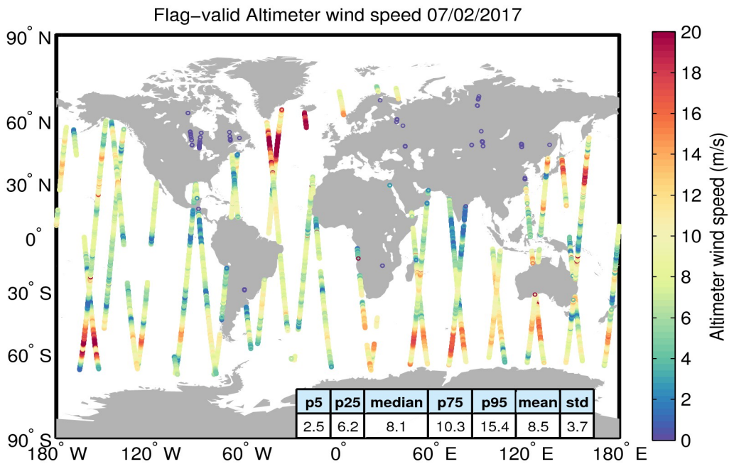
Figure 31. Geographical distribution of flag-valid wind data over oceans and lakes for 07/02/2017. The statistical values shown in the table refer to the wind in m/s and are calculated over all measurements shown in the figure.
