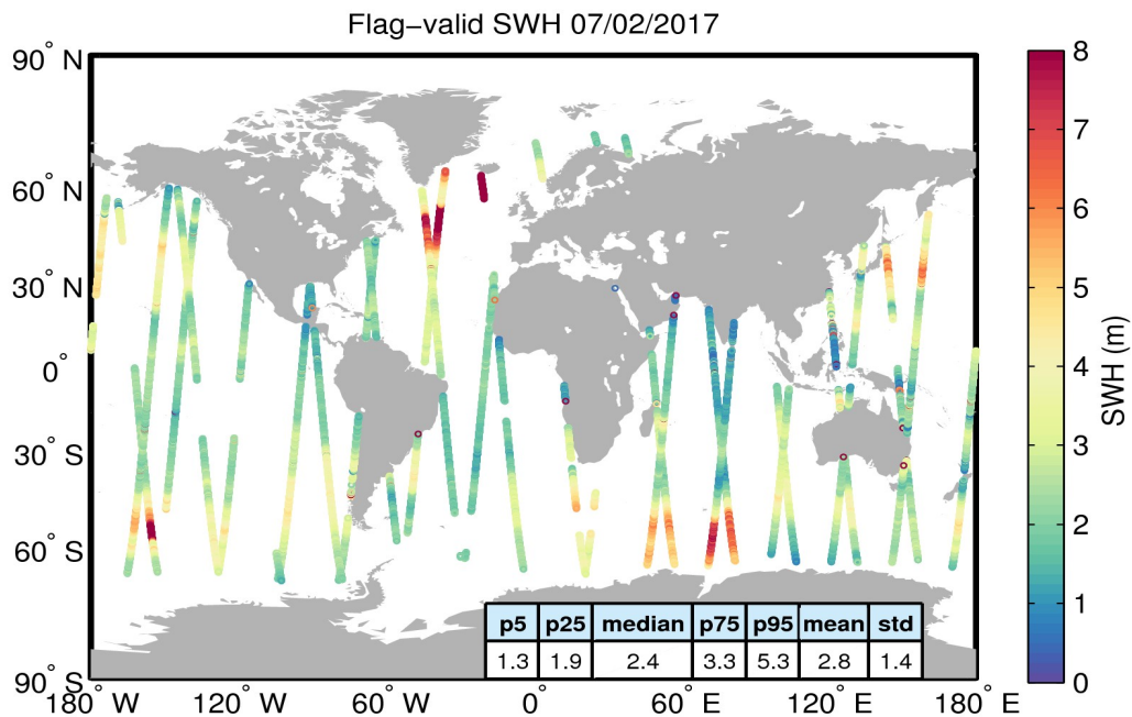
Figure 15. Geographical distribution of flag-valid SWH data over oceans and lakes for 07/02/2017. The statistical values shown in the table refer to the SWH in m and are calculated over all measurements shown in the figure.
