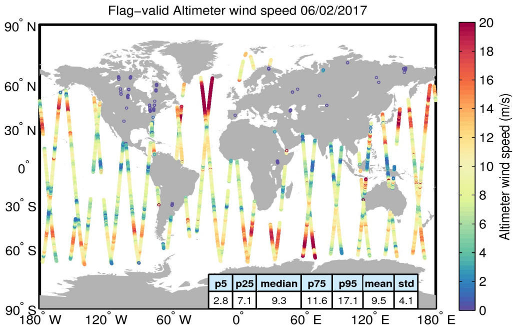
Figure 31. Geographical distribution of flag-valid wind data over oceans and lakes for 06/02/2017. The statistical values shown in the table refer to the wind in m/s and are calculated over all measurements shown in the figure.
