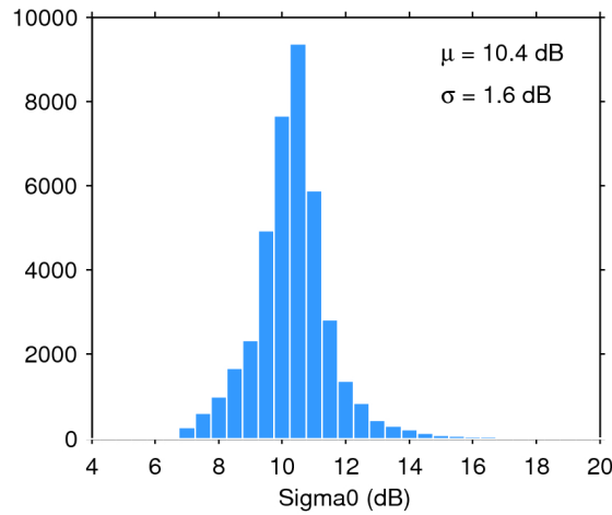
Figure 28. Histogram of science-valid sigma0 over oceans and lakes for 06/02/2017. The mean ( \mu ) and standard deviation ( \sigma ) are also shown. Note that values outside [4 20] dB are excluded from the histogram for the sake of readability but not from the computation of \mu and \sigma .
