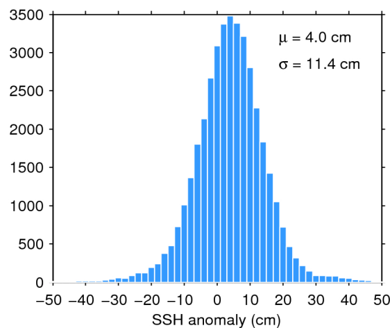
Figure 11. Histogram of science-valid SSH anomaly over oceans and lakes for 06/02/2017. The mean ( \mu ) and standard deviation ( \sigma ) are also shown. Note that values outside [-50 50] cm are excluded from the histogram for the sake of readability but not from the computation of \mu and \sigma .
