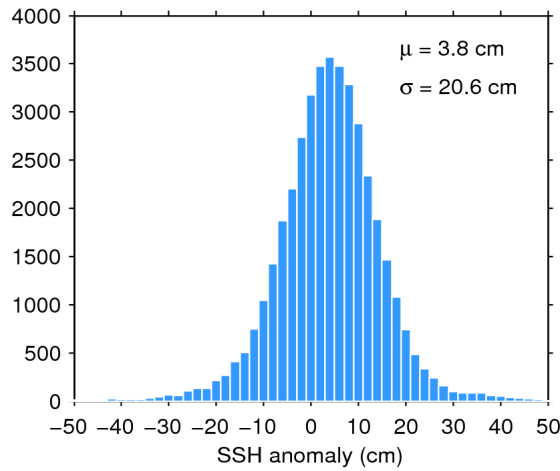
Figure 7. Histogram of flag-valid SSH anomaly over oceans and lakes for 06/02/2017. The mean ( \mu ) and standard deviation ( \sigma ) are also shown. Note that values outside [-50 50] cm are excluded from the histogram for the sake of readability but not from the computation of \mu and \sigma .
