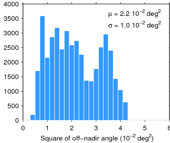
Figure 39. Histogram of flag-valid mispointing over oceans and lakes for 06/02/2017. The mean ( \mu ) and standard deviation ( \sigma ) are also shown. Note that values larger than 6 \cdot 10^{-2} \text{ deg}^2 are excluded from the histogram for the sake of readability but not from the computation of \mu and \sigma .
