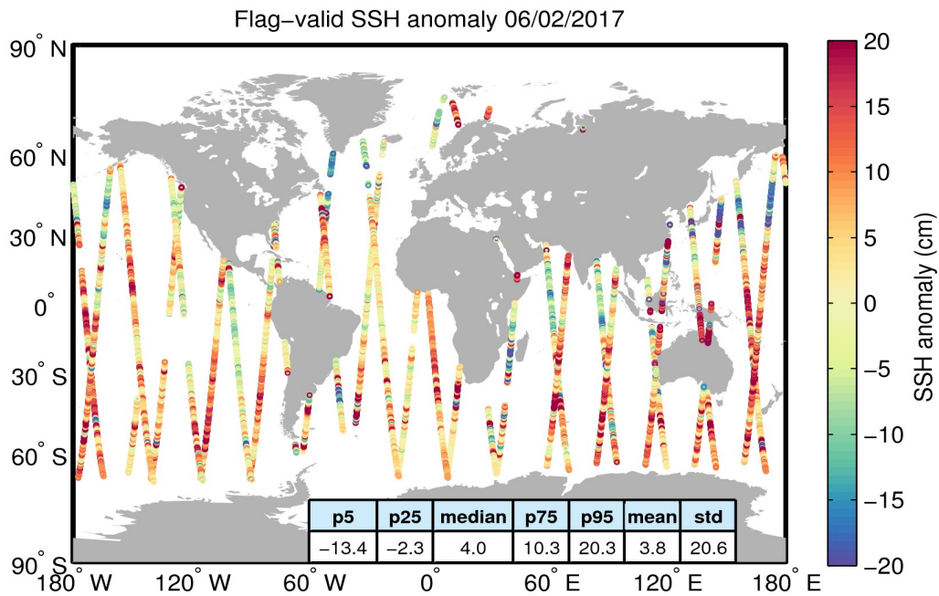
Figure 5. Geographical distribution of flag-valid 1-Hz SSH anomaly data over oceans and lakes for 06/02/2017. The statistical values shown in the table refer to the SSH anomaly in cm and are calculated over all measurements shown in the figure.
