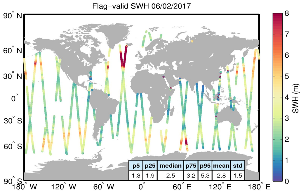
Figure 15. Geographical distribution of flag-valid SWH data over oceans and lakes for 06/02/2017. The statistical values shown in the table refer to the SWH in m and are calculated over all measurements shown in the figure.
