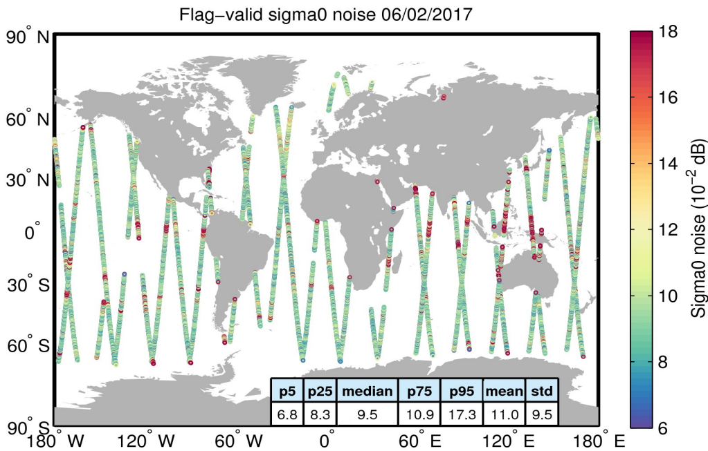
Figure 26. Geographical distribution of flag-valid 20-Hz sigma0 measurement noise over oceans and lakes for 06/02/2017. The statistical values shown in the table refer to the sigma0 noise and are calculated over all measurements shown in the figure.
