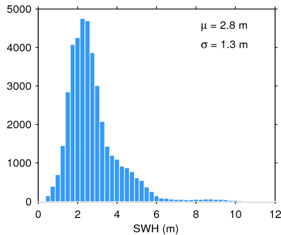
Figure 20. Histogram of science-valid SWH over oceans and lakes for 06/02/2017. The mean ( \mu ) and standard deviation ( \sigma ) are also shown. Note that values larger than 12 m are excluded from the histogram for the sake of readability but not from the computation of \mu and \sigma .
