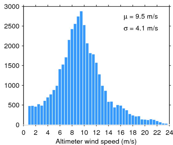
Figure 35. Histogram of science-valid wind over oceans and lakes for 06/02/2017. The mean ( \mu ) and standard deviation ( \sigma ) are also shown. Note that values larger than 24 m/s are excluded from the histogram for the sake of readability but not from the computation of \mu and \sigma .
