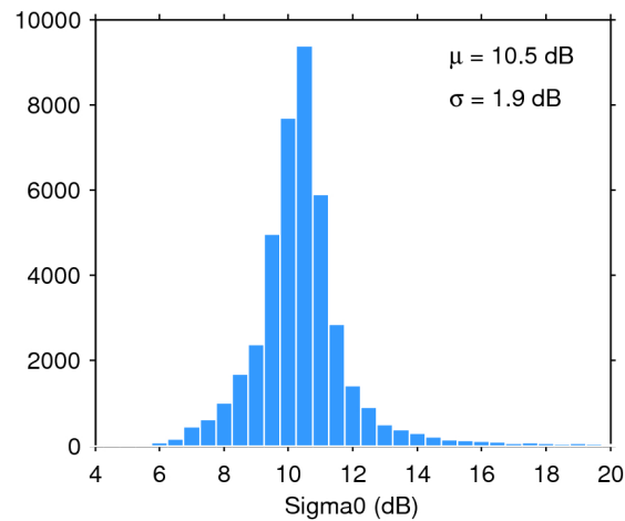
Figure 25. Histogram of flag-valid sigma0 over oceans and lakes for 06/02/2017. The mean ( \mu ) and standard deviation ( \sigma ) are also shown. Note that values outside [4 20] dB are excluded from the histogram for the sake of readability but not from the computation of \mu and \sigma .
