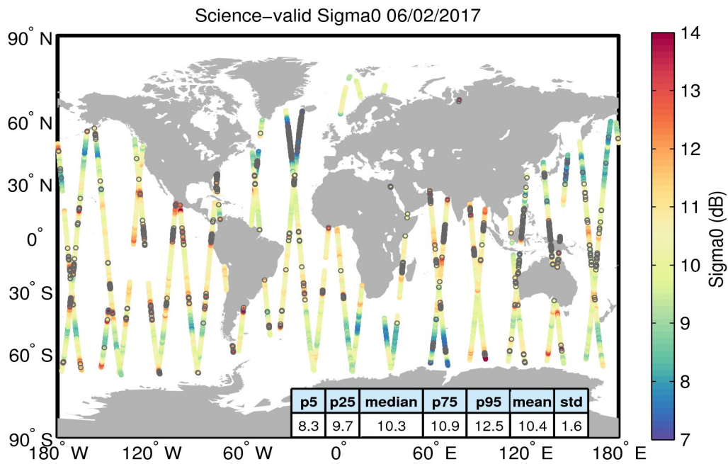
Figure 27. Geographical distribution of science-valid sigma0 data over oceans and lakes for 06/02/2017. The statistical values shown in the table refer to the sigma0 in dB and are calculated over all measurements shown in the figure. Gray circles denote records that have been rejected based on the editing criteria described in Table 4.
