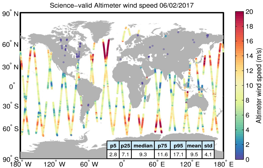
Figure 34. Geographical distribution of science-valid wind data over oceans and lakes for 06/02/2017. The statistical values shown in the table refer to the wind in m/s and are calculated over all measurements shown in the figure. Gray circles denote records that have been rejected based on the editing criteria described in Table 5.
