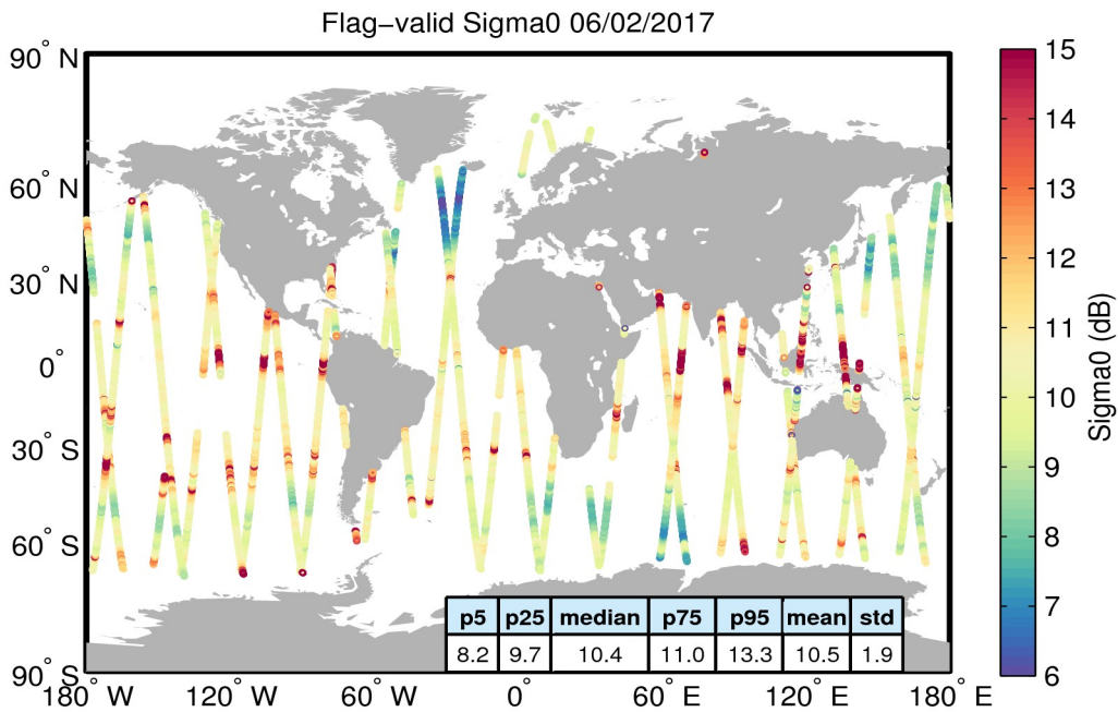
Figure 23. Geographical distribution of flag-valid sigma0 data over oceans and lakes for 06/02/2017. The statistical values shown in the table refer to the sigma0 in dB and are calculated over all measurements shown in the figure.
