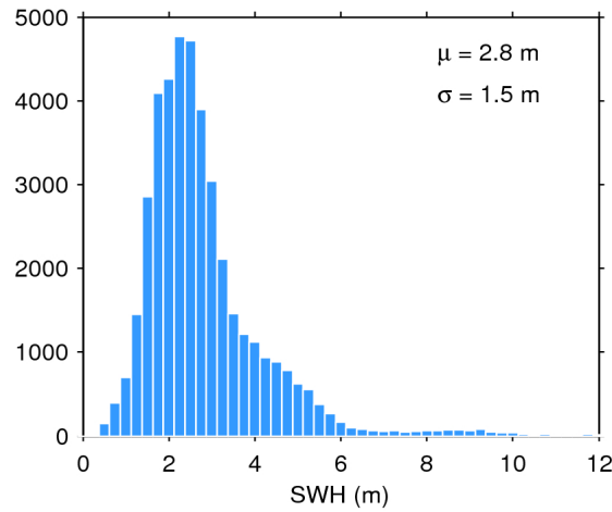
Figure 17. Histogram of flag-valid SWH over oceans and lakes for 06/02/2017. The mean ( \mu ) and standard deviation ( \sigma ) are also shown. Note that values larger than 12 m are excluded from the histogram for the sake of readability but not from the computation of \mu and \sigma .
