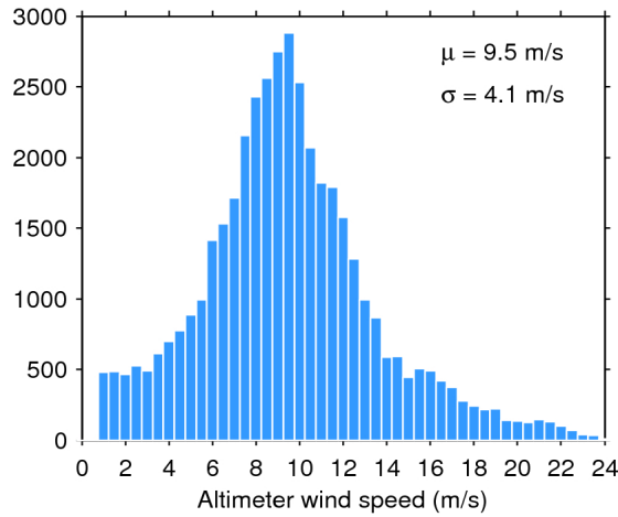
Figure 33. Histogram of flag-valid wind over oceans and lakes for 06/02/2017. The mean ( \mu ) and standard deviation ( \sigma ) are also shown. Note that values larger than 24 m/s are excluded from the histogram for the sake of readability but not from the computation of \mu and \sigma .
