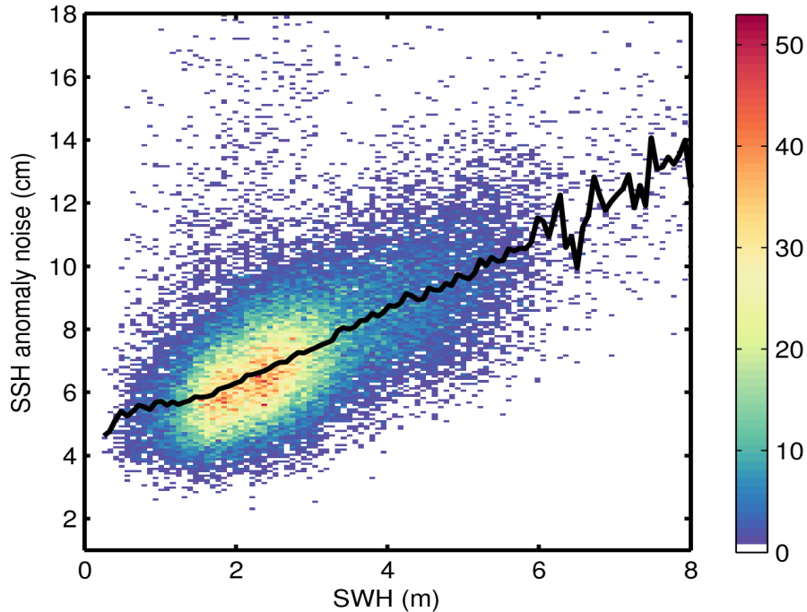
Figure 9. 2D histogram showing flag-valid SSH anomaly noise as a function of SWH for 06/02/2017. The black line denotes the median SSH anomaly noise as a function of SWH.
