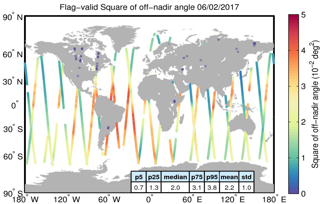
Figure 37. Geographical distribution of flag-valid mispointing data over oceans and lakes for 06/02/2017. The statistical values shown in the table refer to the mispointing in 10^{-2} deg 2 and are calculated over all measurements shown in the figure.
