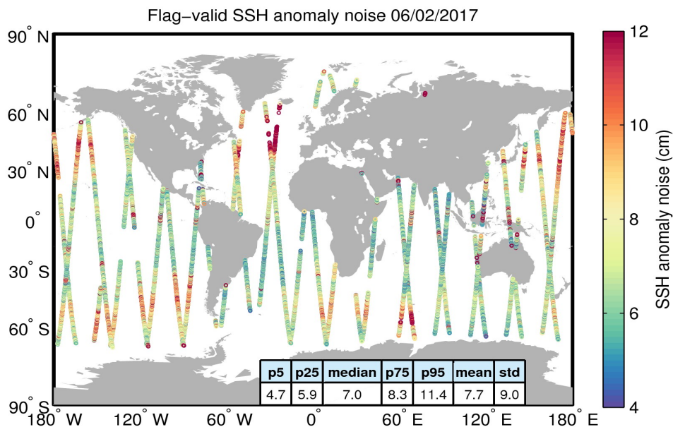
Figure 8. Geographical distribution of flag-valid 20-Hz SSH anomaly measurement noise over oceans and lakes for 06/02/2017. The statistical values shown in the table refer to the SSH anomaly noise and are calculated over all measurements shown in the figure.
