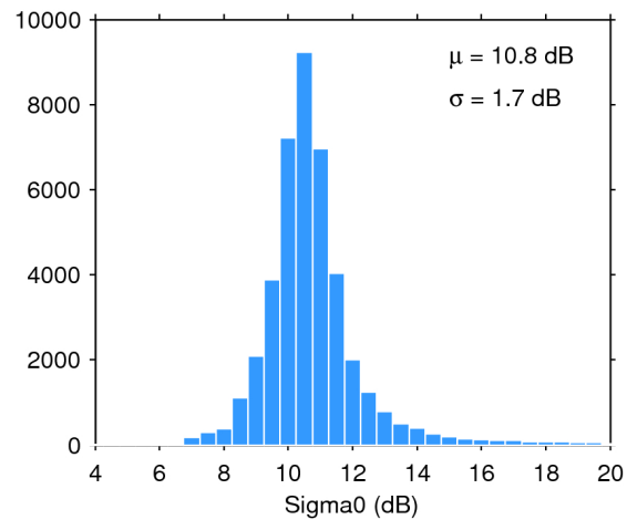
Figure 25. Histogram of flag-valid sigma0 over oceans and lakes for 05/02/2017. The mean ( \mu ) and standard deviation ( \sigma ) are also shown. Note that values outside [4 20] dB are excluded from the histogram for the sake of readability but not from the computation of \mu and \sigma .
