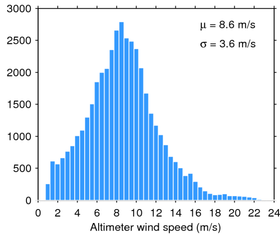
Figure 33. Histogram of flag-valid wind over oceans and lakes for 05/02/2017. The mean ( \mu ) and standard deviation ( \sigma ) are also shown. Note that values larger than 24 m/s are excluded from the histogram for the sake of readability but not from the computation of \mu and \sigma .
