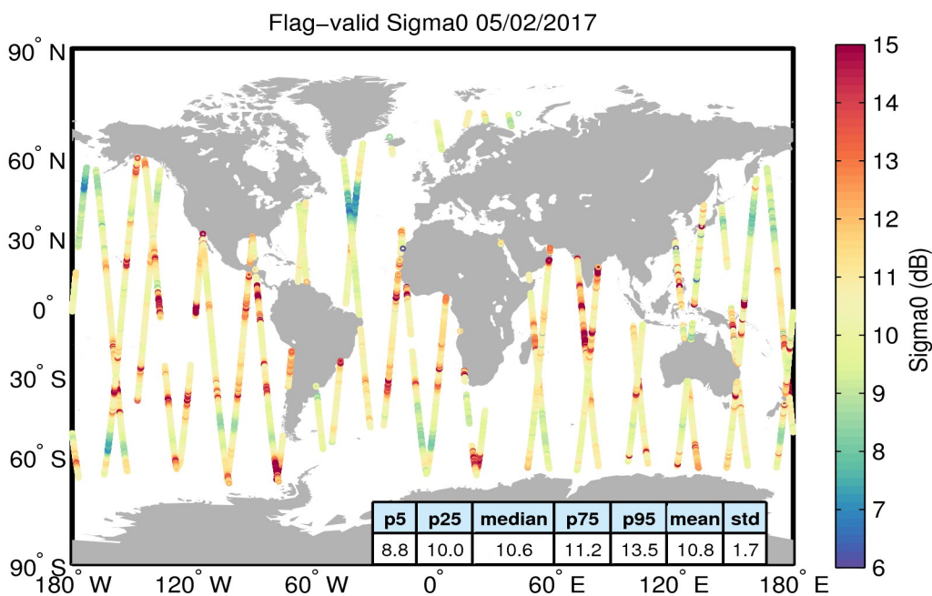
Figure 23. Geographical distribution of flag-valid sigma0 data over oceans and lakes for 05/02/2017. The statistical values shown in the table refer to the sigma0 in dB and are calculated over all measurements shown in the figure.
