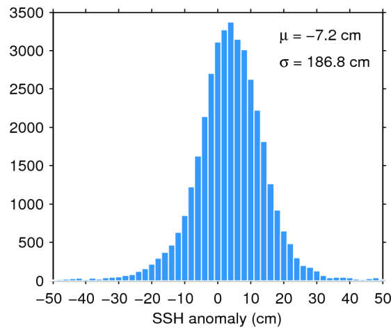
Figure 7. Histogram of flag-valid SSH anomaly over oceans and lakes for 05/02/2017. The mean ( \mu ) and standard deviation ( \sigma ) are also shown. Note that values outside [-50 50] cm are excluded from the histogram for the sake of readability but not from the computation of \mu and \sigma .
