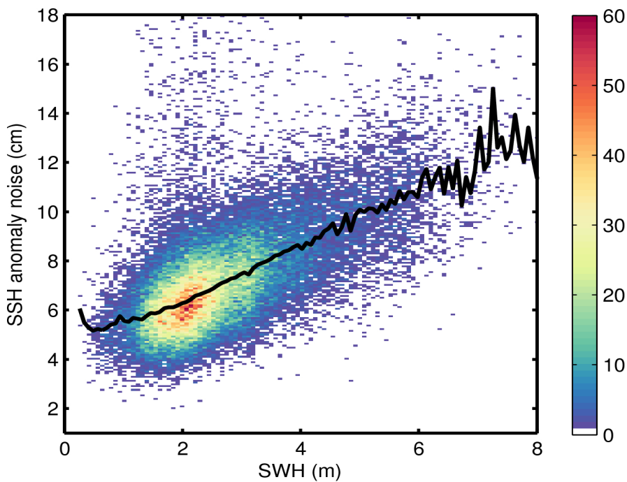
Figure 9. 2D histogram showing flag-valid SSH anomaly noise as a function of SWH for 05/02/2017. The black line denotes the median SSH anomaly noise as a function of SWH.
