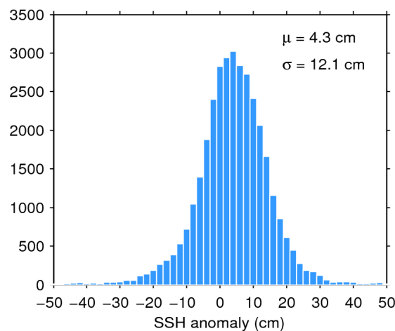
Figure 11. Histogram of science-valid SSH anomaly over oceans and lakes for 05/02/2017. The mean ( \mu ) and standard deviation ( \sigma ) are also shown. Note that values outside [-50 50] cm are excluded from the histogram for the sake of readability but not from the computation of \mu and \sigma .
