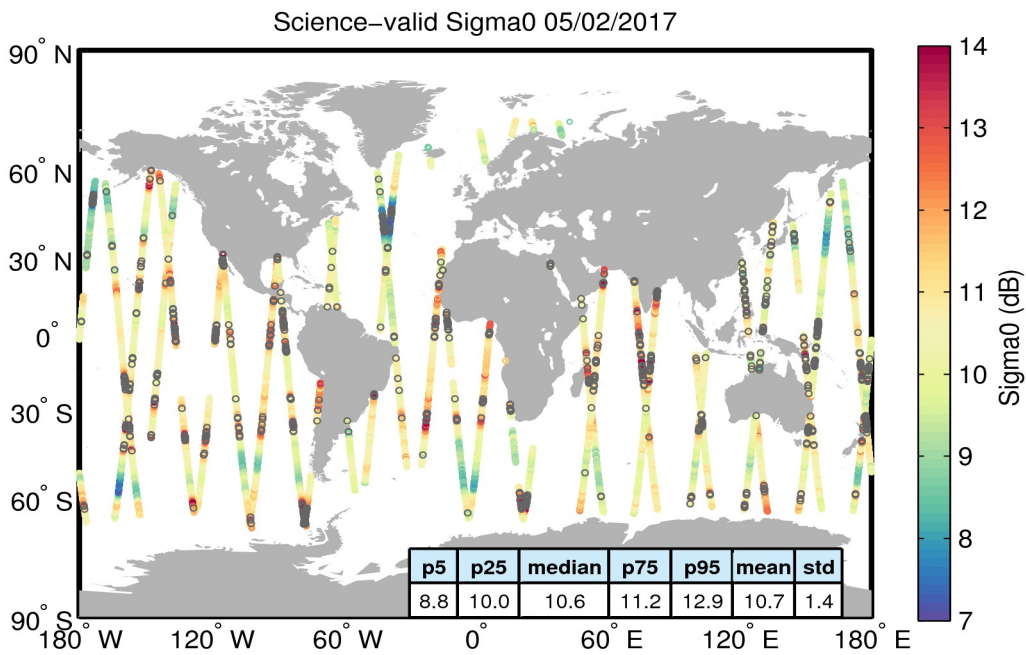
Figure 27. Geographical distribution of science-valid sigma0 data over oceans and lakes for 05/02/2017. The statistical values shown in the table refer to the sigma0 in dB and are calculated over all measurements shown in the figure. Gray circles denote records that have been rejected based on the editing criteria described in Table 4.
