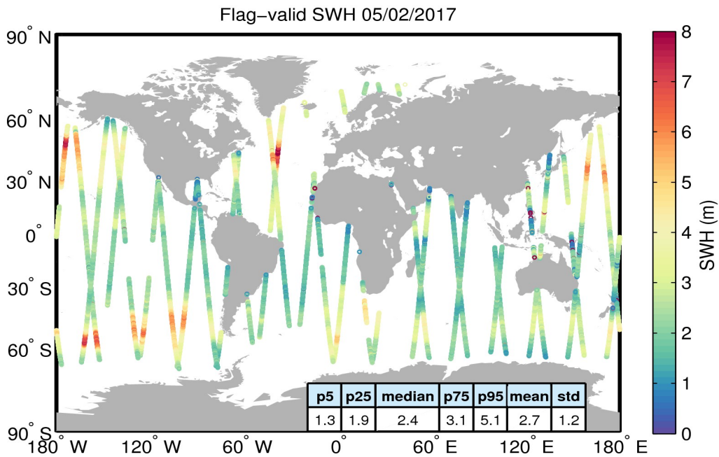
Figure 15. Geographical distribution of flag-valid SWH data over oceans and lakes for 05/02/2017. The statistical values shown in the table refer to the SWH in m and are calculated over all measurements shown in the figure.
