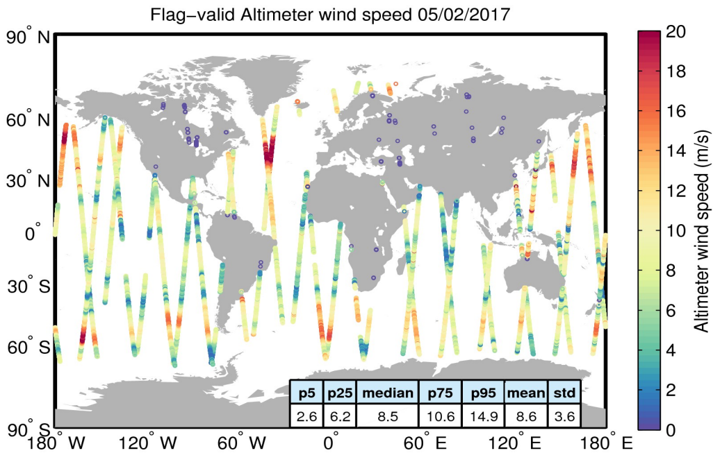
Figure 31. Geographical distribution of flag-valid wind data over oceans and lakes for 05/02/2017. The statistical values shown in the table refer to the wind in m/s and are calculated over all measurements shown in the figure.
