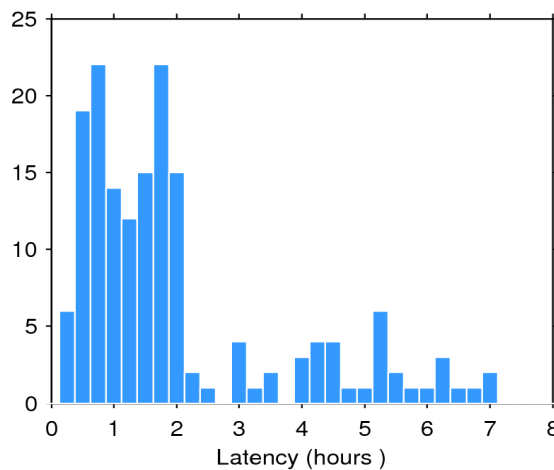
Figure 2. Histogram of the data latency for 05/02/2017. The y-axis denotes the number of files that are made available with a delay of x-hours with respect to the mean time of the records stored in the file.
