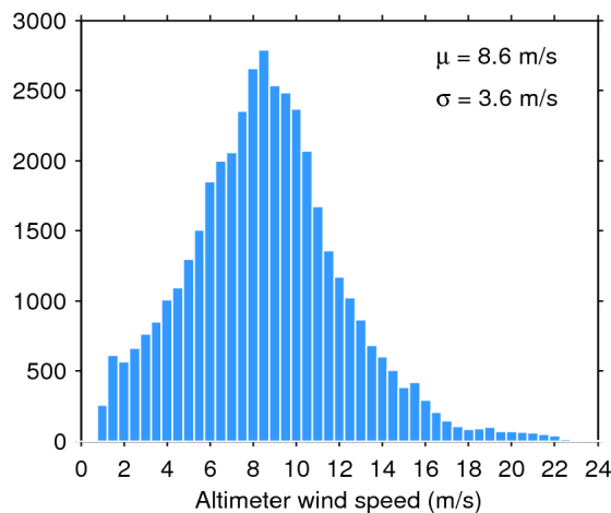
Figure 35. Histogram of science-valid wind over oceans and lakes for 05/02/2017. The mean ( \mu ) and standard deviation ( \sigma ) are also shown. Note that values larger than 24 m/s are excluded from the histogram for the sake of readability but not from the computation of \mu and \sigma .
