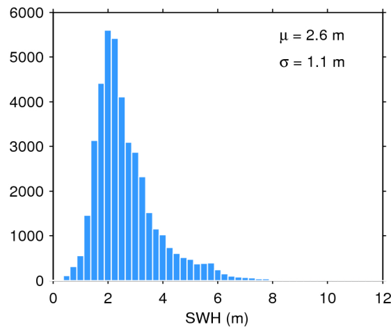
Figure 20. Histogram of science-valid SWH over oceans and lakes for 05/02/2017. The mean ( \mu ) and standard deviation ( \sigma ) are also shown. Note that values larger than 12 m are excluded from the histogram for the sake of readability but not from the computation of \mu and \sigma .
