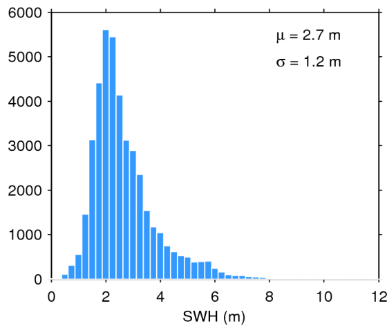
Figure 17. Histogram of flag-valid SWH over oceans and lakes for 05/02/2017. The mean ( \mu ) and standard deviation ( \sigma ) are also shown. Note that values larger than 12 m are excluded from the histogram for the sake of readability but not from the computation of \mu and \sigma .
