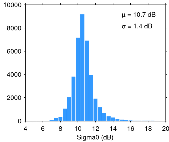
Figure 28. Histogram of science-valid sigma0 over oceans and lakes for 05/02/2017. The mean ( \mu ) and standard deviation ( \sigma ) are also shown. Note that values outside [4 20] dB are excluded from the histogram for the sake of readability but not from the computation of \mu and \sigma .
