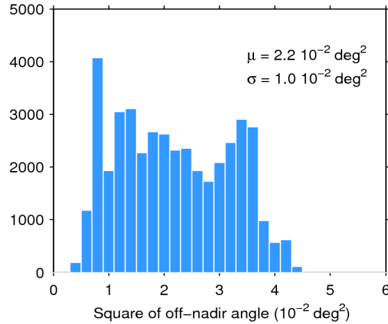
Figure 39. Histogram of flag-valid mispointing over oceans and lakes for 05/02/2017. The mean ( \mu ) and standard deviation ( \sigma ) are also shown. Note that values larger than 6 \cdot 10^{-2} \text{ deg}^2 are excluded from the histogram for the sake of readability but not from the computation of \mu and \sigma .
