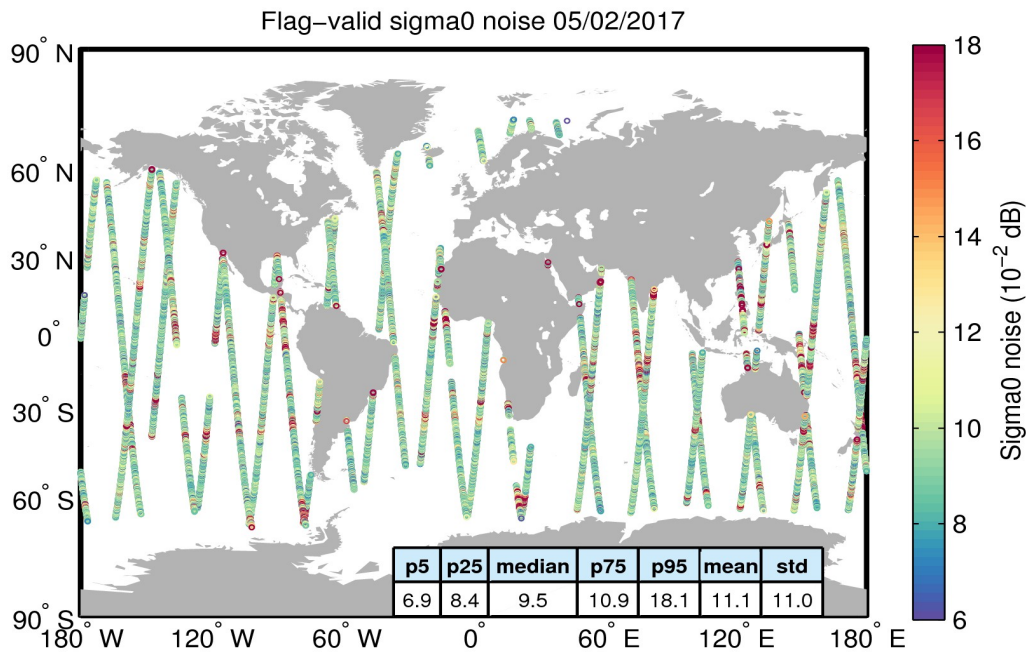
Figure 26. Geographical distribution of flag-valid 20-Hz sigma0 measurement noise over oceans and lakes for 05/02/2017. The statistical values shown in the table refer to the sigma0 noise and are calculated over all measurements shown in the figure.
