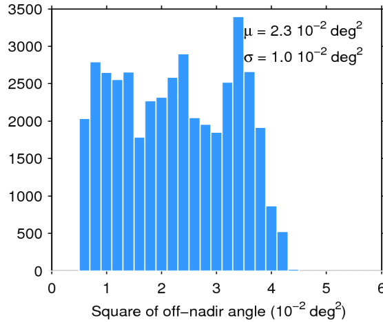
Figure 39. Histogram of flag-valid mispointing over oceans and lakes for 04/02/2017. The mean ( \mu ) and standard deviation ( \sigma ) are also shown. Note that values larger than 6 \cdot 10^{-2} \text{ deg}^2 are excluded from the histogram for the sake of readability but not from the computation of \mu and \sigma .
