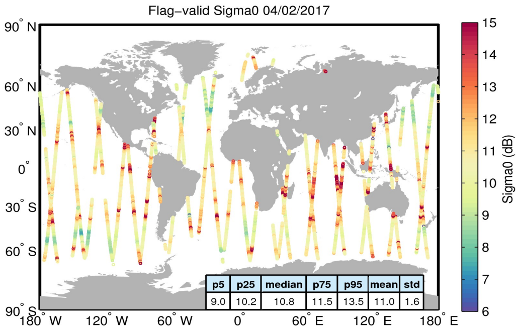
Figure 23. Geographical distribution of flag-valid sigma0 data over oceans and lakes for 04/02/2017. The statistical values shown in the table refer to the sigma0 in dB and are calculated over all measurements shown in the figure.
