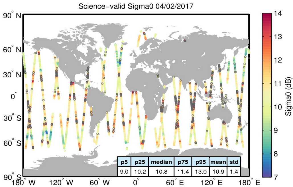
Figure 27. Geographical distribution of science-valid sigma0 data over oceans and lakes for 04/02/2017. The statistical values shown in the table refer to the sigma0 in dB and are calculated over all measurements shown in the figure. Gray circles denote records that have been rejected based on the editing criteria described in Table 4.
