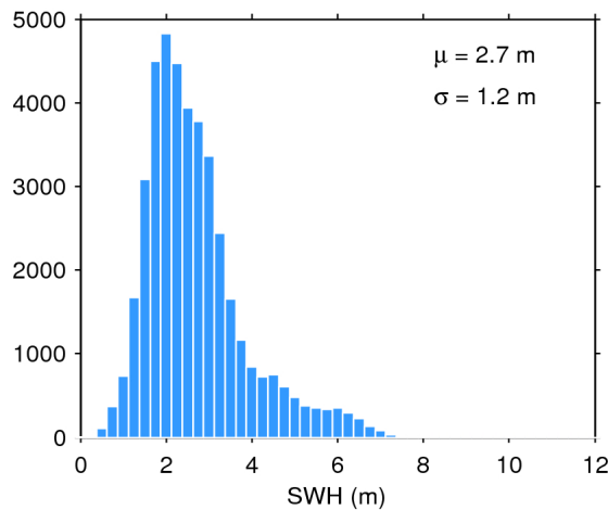
Figure 20. Histogram of science-valid SWH over oceans and lakes for 04/02/2017. The mean ( \mu ) and standard deviation ( \sigma ) are also shown. Note that values larger than 12 m are excluded from the histogram for the sake of readability but not from the computation of \mu and \sigma .
