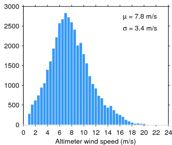
Figure 35. Histogram of science-valid wind over oceans and lakes for 04/02/2017. The mean ( \mu ) and standard deviation ( \sigma ) are also shown. Note that values larger than 24 m/s are excluded from the histogram for the sake of readability but not from the computation of \mu and \sigma .
