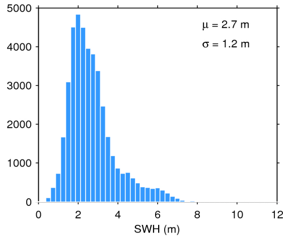
Figure 17. Histogram of flag-valid SWH over oceans and lakes for 04/02/2017. The mean ( \mu ) and standard deviation ( \sigma ) are also shown. Note that values larger than 12 m are excluded from the histogram for the sake of readability but not from the computation of \mu and \sigma .
