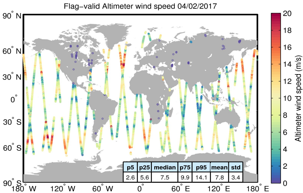
Figure 31. Geographical distribution of flag-valid wind data over oceans and lakes for 04/02/2017. The statistical values shown in the table refer to the wind in m/s and are calculated over all measurements shown in the figure.
