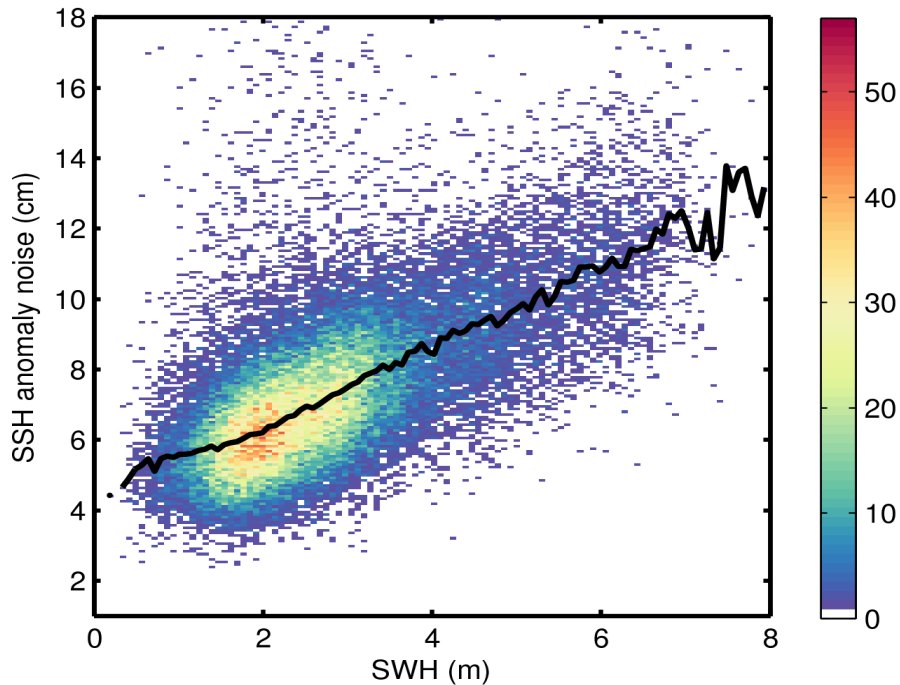
Figure 9. 2D histogram showing flag-valid SSH anomaly noise as a function of SWH for 04/02/2017. The black line denotes the median SSH anomaly noise as a function of SWH.
