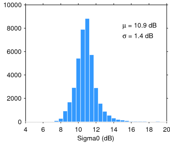
Figure 28. Histogram of science-valid sigma0 over oceans and lakes for 04/02/2017. The mean ( \mu ) and standard deviation ( \sigma ) are also shown. Note that values outside [4 20] dB are excluded from the histogram for the sake of readability but not from the computation of \mu and \sigma .
