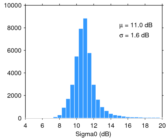
Figure 25. Histogram of flag-valid sigma0 over oceans and lakes for 04/02/2017. The mean ( \mu ) and standard deviation ( \sigma ) are also shown. Note that values outside [4 20] dB are excluded from the histogram for the sake of readability but not from the computation of \mu and \sigma .
