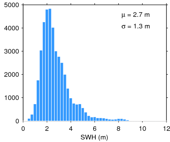
Figure 17. Histogram of flag-valid SWH over oceans and lakes for 03/02/2017. The mean ( \mu ) and standard deviation ( \sigma ) are also shown. Note that values larger than 12 m are excluded from the histogram for the sake of readability but not from the computation of \mu and \sigma .
