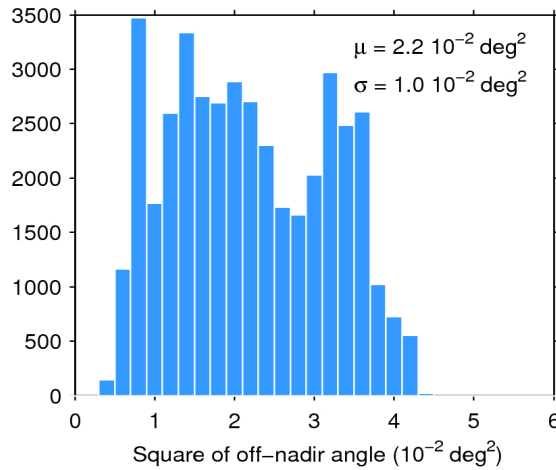
Figure 39. Histogram of flag-valid mispointing over oceans and lakes for 03/02/2017. The mean ( \mu ) and standard deviation ( \sigma ) are also shown. Note that values larger than 6 \cdot 10^{-2} \text{ deg}^2 are excluded from the histogram for the sake of readability but not from the computation of \mu and \sigma .
