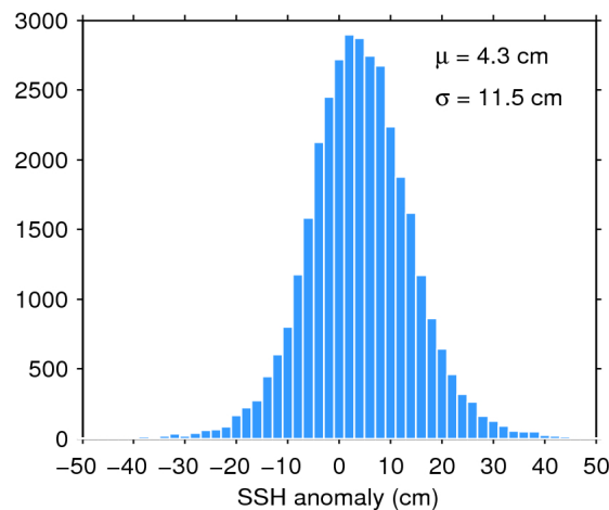
Figure 11. Histogram of science-valid SSH anomaly over oceans and lakes for 03/02/2017. The mean ( \mu ) and standard deviation ( \sigma ) are also shown. Note that values outside [-50 50] cm are excluded from the histogram for the sake of readability but not from the computation of \mu and \sigma .
