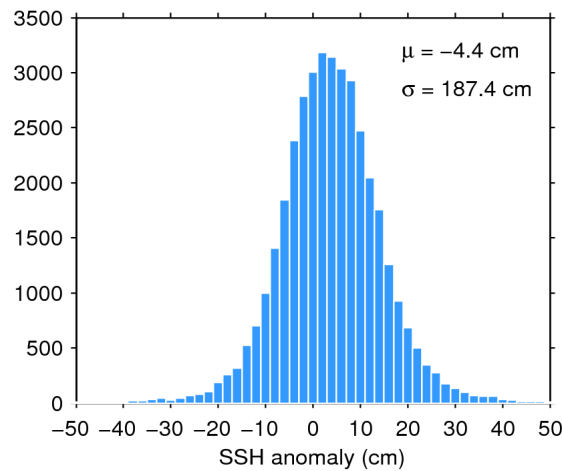
Figure 7. Histogram of flag-valid SSH anomaly over oceans and lakes for 03/02/2017. The mean ( \mu ) and standard deviation ( \sigma ) are also shown. Note that values outside [-50 50] cm are excluded from the histogram for the sake of readability but not from the computation of \mu and \sigma .
