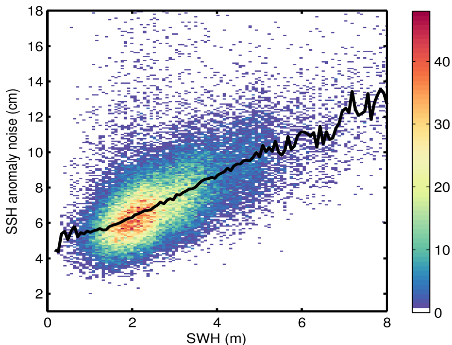
Figure 9. 2D histogram showing flag-valid SSH anomaly noise as a function of SWH for 03/02/2017. The black line denotes the median SSH anomaly noise as a function of SWH.
