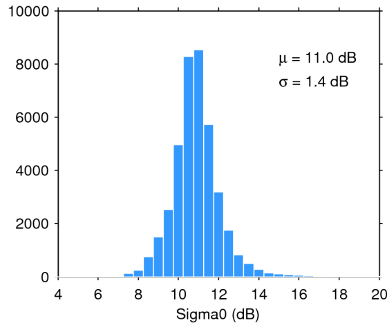
Figure 28. Histogram of science-valid sigma0 over oceans and lakes for 03/02/2017. The mean ( \mu ) and standard deviation ( \sigma ) are also shown. Note that values outside [4 20] dB are excluded from the histogram for the sake of readability but not from the computation of \mu and \sigma .
