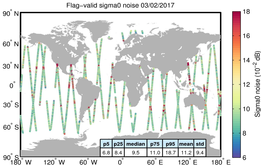
Figure 26. Geographical distribution of flag-valid 20-Hz sigma0 measurement noise over oceans and lakes for 03/02/2017. The statistical values shown in the table refer to the sigma0 noise and are calculated over all measurements shown in the figure.
