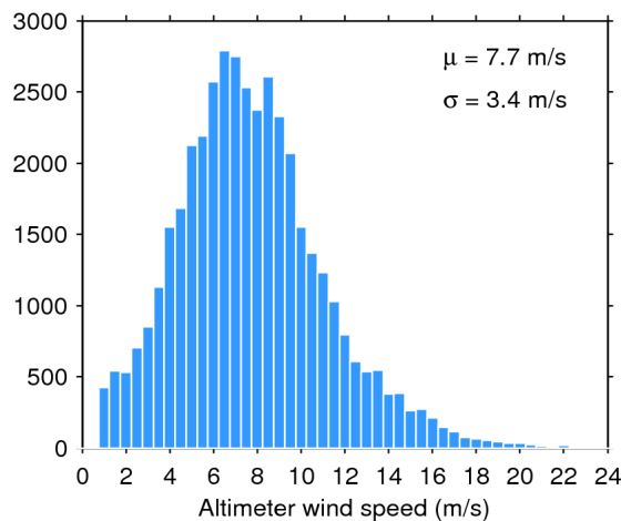
Figure 35. Histogram of science-valid wind over oceans and lakes for 03/02/2017. The mean ( \mu ) and standard deviation ( \sigma ) are also shown. Note that values larger than 24 m/s are excluded from the histogram for the sake of readability but not from the computation of \mu and \sigma .
