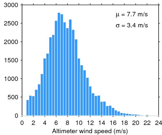
Figure 33. Histogram of flag-valid wind over oceans and lakes for 03/02/2017. The mean ( \mu ) and standard deviation ( \sigma ) are also shown. Note that values larger than 24 m/s are excluded from the histogram for the sake of readability but not from the computation of \mu and \sigma .
