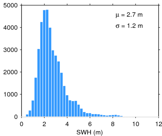
Figure 20. Histogram of science-valid SWH over oceans and lakes for 03/02/2017. The mean ( \mu ) and standard deviation ( \sigma ) are also shown. Note that values larger than 12 m are excluded from the histogram for the sake of readability but not from the computation of \mu and \sigma .
