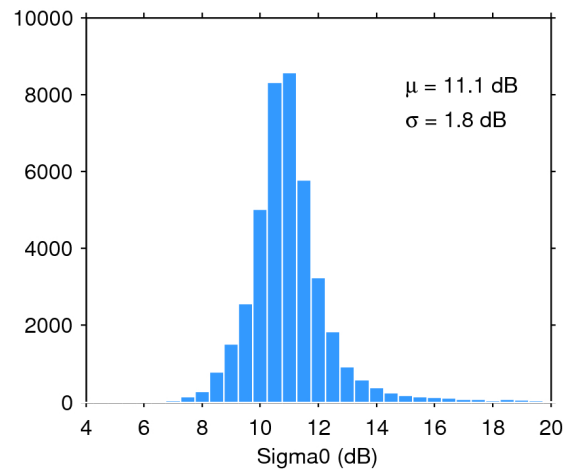
Figure 25. Histogram of flag-valid sigma0 over oceans and lakes for 03/02/2017. The mean ( \mu ) and standard deviation ( \sigma ) are also shown. Note that values outside [4 20] dB are excluded from the histogram for the sake of readability but not from the computation of \mu and \sigma .
