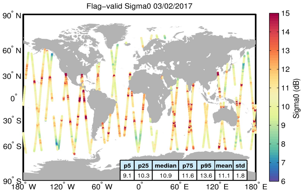
Figure 23. Geographical distribution of flag-valid sigma0 data over oceans and lakes for 03/02/2017. The statistical values shown in the table refer to the sigma0 in dB and are calculated over all measurements shown in the figure.
