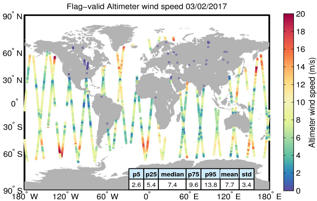
Figure 31. Geographical distribution of flag-valid wind data over oceans and lakes for 03/02/2017. The statistical values shown in the table refer to the wind in m/s and are calculated over all measurements shown in the figure.
