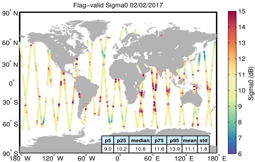
Figure 23. Geographical distribution of flag-valid sigma0 data over oceans and lakes for 02/02/2017. The statistical values shown in the table refer to the sigma0 in dB and are calculated over all measurements shown in the figure.
