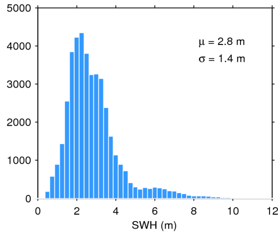
Figure 17. Histogram of flag-valid SWH over oceans and lakes for 02/02/2017. The mean ( \mu ) and standard deviation ( \sigma ) are also shown. Note that values larger than 12 m are excluded from the histogram for the sake of readability but not from the computation of \mu and \sigma .
