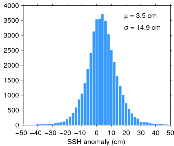
Figure 7. Histogram of flag-valid SSH anomaly over oceans and lakes for 02/02/2017. The mean ( \mu ) and standard deviation ( \sigma ) are also shown. Note that values outside [-50 50] cm are excluded from the histogram for the sake of readability but not from the computation of \mu and \sigma .
