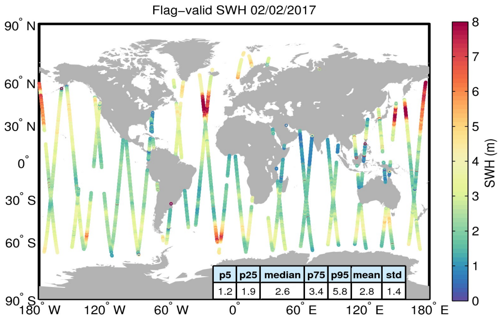
Figure 15. Geographical distribution of flag-valid SWH data over oceans and lakes for 02/02/2017. The statistical values shown in the table refer to the SWH in m and are calculated over all measurements shown in the figure.
