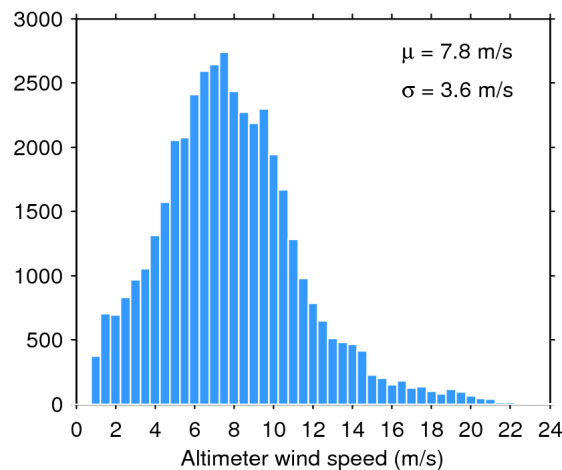
Figure 35. Histogram of science-valid wind over oceans and lakes for 02/02/2017. The mean ( \mu ) and standard deviation ( \sigma ) are also shown. Note that values larger than 24 m/s are excluded from the histogram for the sake of readability but not from the computation of \mu and \sigma .
