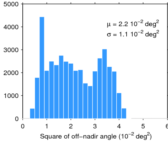
Figure 39. Histogram of flag-valid mispointing over oceans and lakes for 02/02/2017. The mean ( \mu ) and standard deviation ( \sigma ) are also shown. Note that values larger than 6 \cdot 10^{-2} \text{ deg}^2 are excluded from the histogram for the sake of readability but not from the computation of \mu and \sigma .
