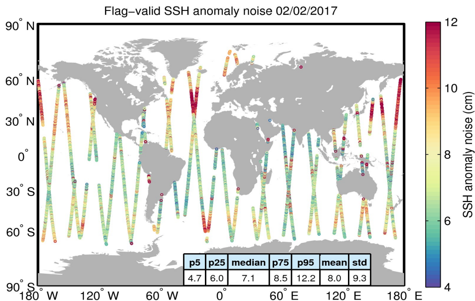
Figure 8. Geographical distribution of flag-valid 20-Hz SSH anomaly measurement noise over oceans and lakes for 02/02/2017. The statistical values shown in the table refer to the SSH anomaly noise and are calculated over all measurements shown in the figure.
