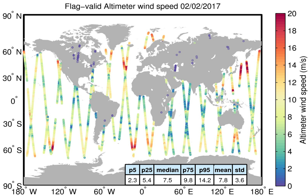
Figure 31. Geographical distribution of flag-valid wind data over oceans and lakes for 02/02/2017. The statistical values shown in the table refer to the wind in m/s and are calculated over all measurements shown in the figure.
