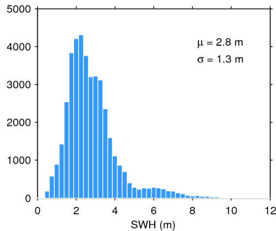
Figure 20. Histogram of science-valid SWH over oceans and lakes for 02/02/2017. The mean ( \mu ) and standard deviation ( \sigma ) are also shown. Note that values larger than 12 m are excluded from the histogram for the sake of readability but not from the computation of \mu and \sigma .
