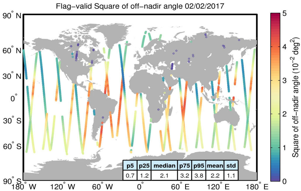
Figure 37. Geographical distribution of flag-valid mispointing data over oceans and lakes for 02/02/2017. The statistical values shown in the table refer to the mispointing in 10^{-2} deg 2 and are calculated over all measurements shown in the figure.
