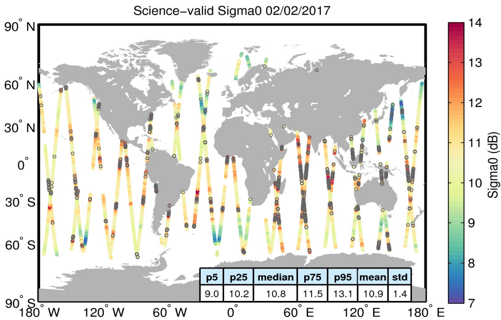
Figure 27. Geographical distribution of science-valid sigma0 data over oceans and lakes for 02/02/2017. The statistical values shown in the table refer to the sigma0 in dB and are calculated over all measurements shown in the figure. Gray circles denote records that have been rejected based on the editing criteria described in Table 4.
