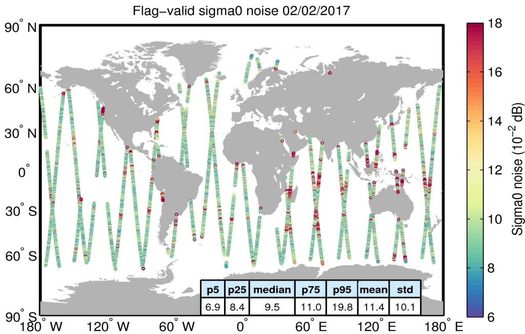
Figure 26. Geographical distribution of flag-valid 20-Hz sigma0 measurement noise over oceans and lakes for 02/02/2017. The statistical values shown in the table refer to the sigma0 noise and are calculated over all measurements shown in the figure.
