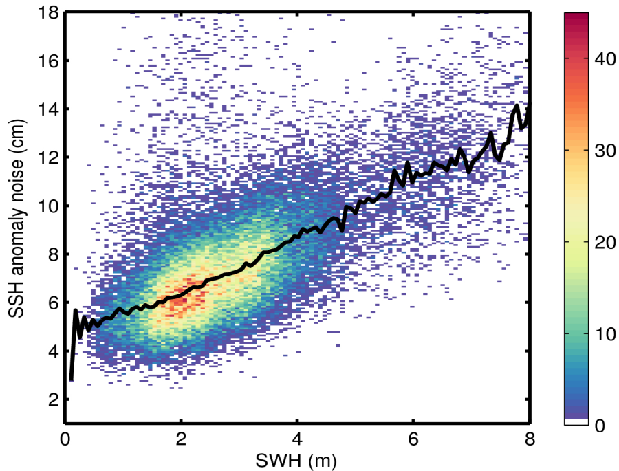
Figure 9. 2D histogram showing flag-valid SSH anomaly noise as a function of SWH for 02/02/2017. The black line denotes the median SSH anomaly noise as a function of SWH.
