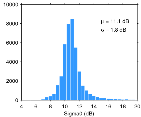
Figure 25. Histogram of flag-valid sigma0 over oceans and lakes for 02/02/2017. The mean ( \mu ) and standard deviation ( \sigma ) are also shown. Note that values outside [4 20] dB are excluded from the histogram for the sake of readability but not from the computation of \mu and \sigma .
