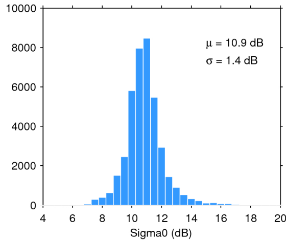
Figure 28. Histogram of science-valid sigma0 over oceans and lakes for 02/02/2017. The mean ( \mu ) and standard deviation ( \sigma ) are also shown. Note that values outside [4 20] dB are excluded from the histogram for the sake of readability but not from the computation of \mu and \sigma .
