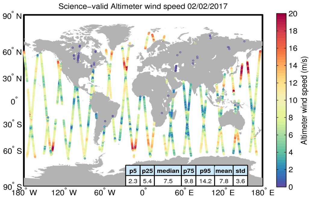
Figure 34. Geographical distribution of science-valid wind data over oceans and lakes for 02/02/2017. The statistical values shown in the table refer to the wind in m/s and are calculated over all measurements shown in the figure. Gray circles denote records that have been rejected based on the editing criteria described in Table 5.
