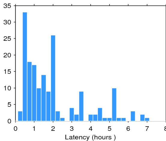
Figure 2. Histogram of the data latency for 01/02/2017. The y-axis denotes the number of files that are made available with a delay of x-hours with respect to the mean time of the records stored in the file.
