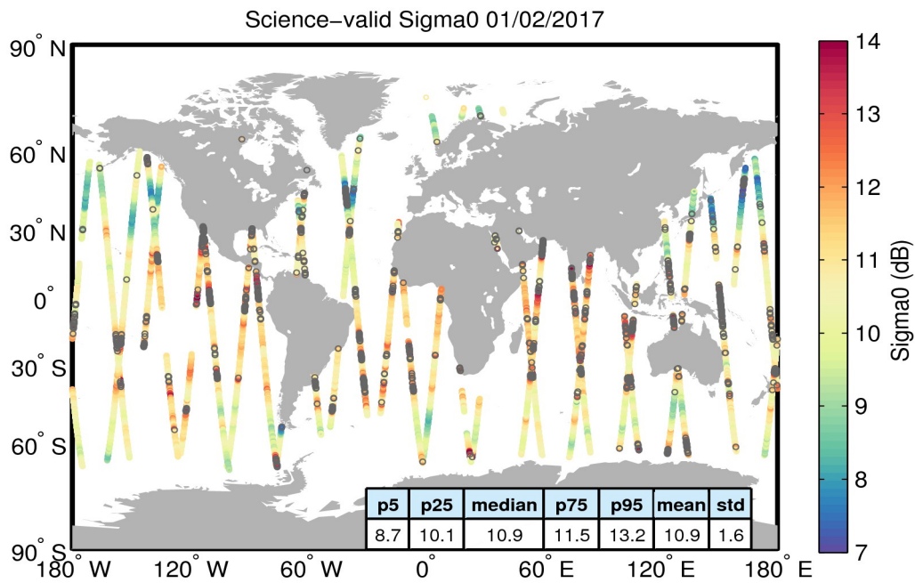
Figure 27. Geographical distribution of science-valid sigma0 data over oceans and lakes for 01/02/2017. The statistical values shown in the table refer to the sigma0 in dB and are calculated over all measurements shown in the figure. Gray circles denote records that have been rejected based on the editing criteria described in Table 4.
