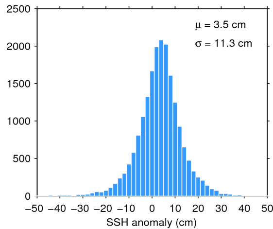
Figure 11. Histogram of science-valid SSH anomaly over oceans and lakes for 01/02/2017. The mean ( \mu ) and standard deviation ( \sigma ) are also shown. Note that values outside [-50 50] cm are excluded from the histogram for the sake of readability but not from the computation of \mu and \sigma .
