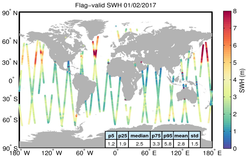
Figure 15. Geographical distribution of flag-valid SWH data over oceans and lakes for 01/02/2017. The statistical values shown in the table refer to the SWH in m and are calculated over all measurements shown in the figure.
