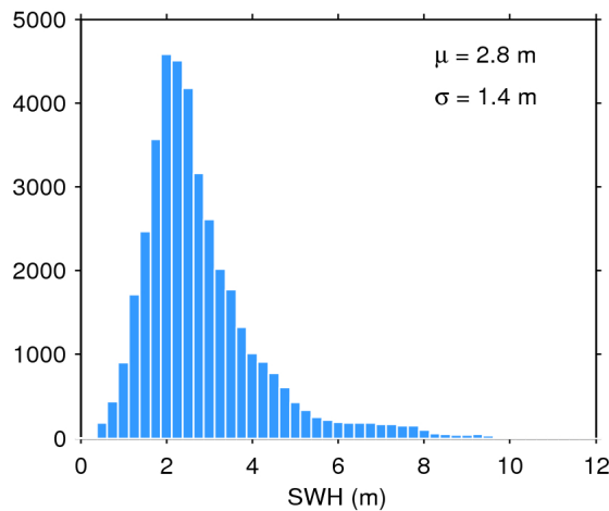
Figure 20. Histogram of science-valid SWH over oceans and lakes for 01/02/2017. The mean ( \mu ) and standard deviation ( \sigma ) are also shown. Note that values larger than 12 m are excluded from the histogram for the sake of readability but not from the computation of \mu and \sigma .
