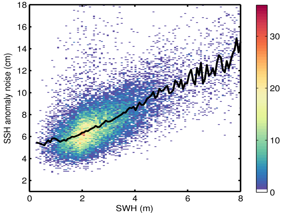
Figure 9. 2D histogram showing flag-valid SSH anomaly noise as a function of SWH for 01/02/2017. The black line denotes the median SSH anomaly noise as a function of SWH.
