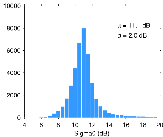
Figure 25. Histogram of flag-valid sigma0 over oceans and lakes for 01/02/2017. The mean ( \mu ) and standard deviation ( \sigma ) are also shown. Note that values outside [4 20] dB are excluded from the histogram for the sake of readability but not from the computation of \mu and \sigma .
