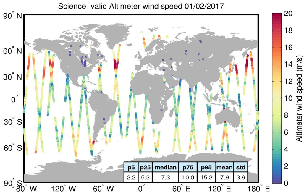
Figure 34. Geographical distribution of science-valid wind data over oceans and lakes for 01/02/2017. The statistical values shown in the table refer to the wind in m/s and are calculated over all measurements shown in the figure. Gray circles denote records that have been rejected based on the editing criteria described in Table 5.
