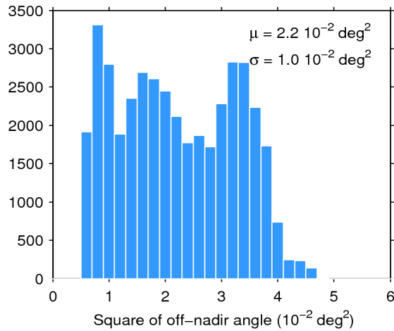
Figure 39. Histogram of flag-valid mispointing over oceans and lakes for 01/02/2017. The mean ( \mu ) and standard deviation ( \sigma ) are also shown. Note that values larger than 6 \cdot 10^{-2} \text{ deg}^2 are excluded from the histogram for the sake of readability but not from the computation of \mu and \sigma .
