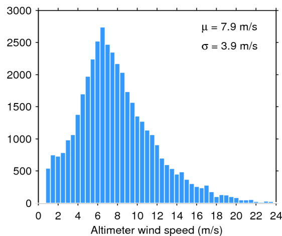
Figure 35. Histogram of science-valid wind over oceans and lakes for 01/02/2017. The mean ( \mu ) and standard deviation ( \sigma ) are also shown. Note that values larger than 24 m/s are excluded from the histogram for the sake of readability but not from the computation of \mu and \sigma .
