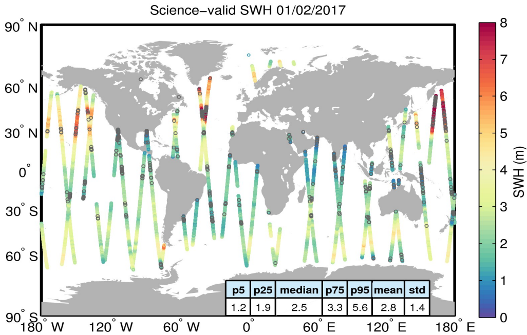
Figure 19. Geographical distribution of science-valid SWH data over oceans and lakes for 01/02/2017. The statistical values shown in the table refer to the SWH in m and are calculated over all measurements shown in the figure. Gray circles denote records that have been rejected based on the editing criteria described in Table 3.
