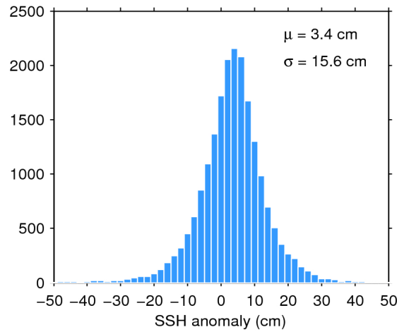
Figure 7. Histogram of flag-valid SSH anomaly over oceans and lakes for 01/02/2017. The mean ( \mu ) and standard deviation ( \sigma ) are also shown. Note that values outside [-50 50] cm are excluded from the histogram for the sake of readability but not from the computation of \mu and \sigma .
