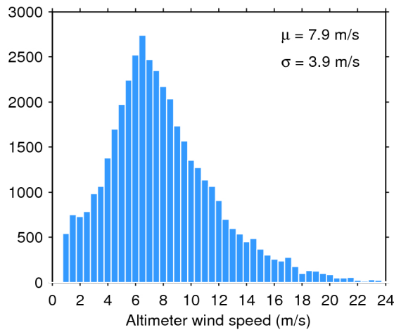
Figure 33. Histogram of flag-valid wind over oceans and lakes for 01/02/2017. The mean ( \mu ) and standard deviation ( \sigma ) are also shown. Note that values larger than 24 m/s are excluded from the histogram for the sake of readability but not from the computation of \mu and \sigma .
