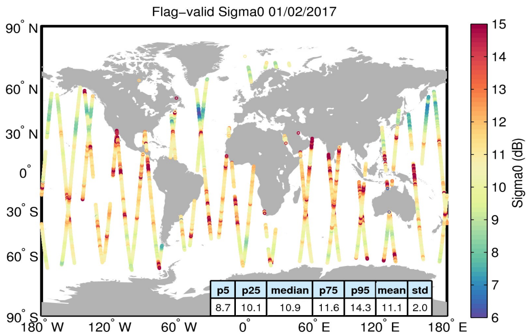
Figure 23. Geographical distribution of flag-valid sigma0 data over oceans and lakes for 01/02/2017. The statistical values shown in the table refer to the sigma0 in dB and are calculated over all measurements shown in the figure.
