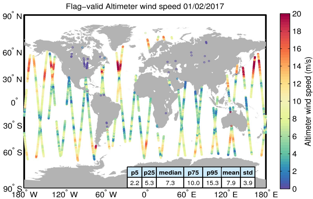
Figure 31. Geographical distribution of flag-valid wind data over oceans and lakes for 01/02/2017. The statistical values shown in the table refer to the wind in m/s and are calculated over all measurements shown in the figure.
