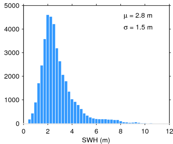
Figure 17. Histogram of flag-valid SWH over oceans and lakes for 01/02/2017. The mean ( \mu ) and standard deviation ( \sigma ) are also shown. Note that values larger than 12 m are excluded from the histogram for the sake of readability but not from the computation of \mu and \sigma .
