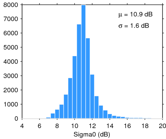
Figure 28. Histogram of science-valid sigma0 over oceans and lakes for 01/02/2017. The mean ( \mu ) and standard deviation ( \sigma ) are also shown. Note that values outside [4 20] dB are excluded from the histogram for the sake of readability but not from the computation of \mu and \sigma .
