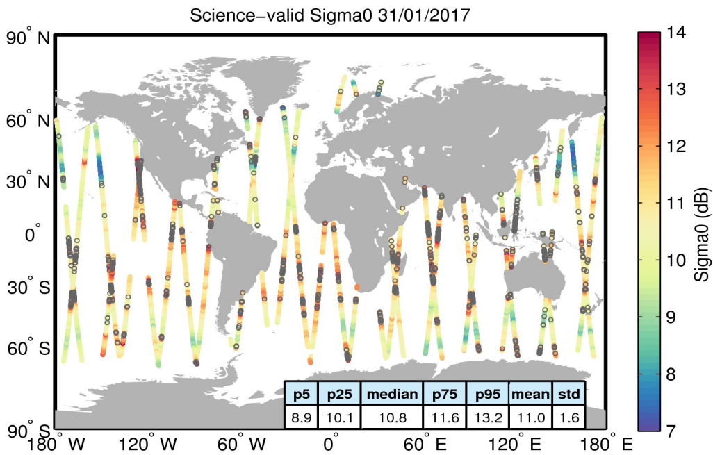
Figure 27. Geographical distribution of science-valid sigma0 data over oceans and lakes for 31/01/2017. The statistical values shown in the table refer to the sigma0 in dB and are calculated over all measurements shown in the figure. Gray circles denote records that have been rejected based on the editing criteria described in Table 4.
