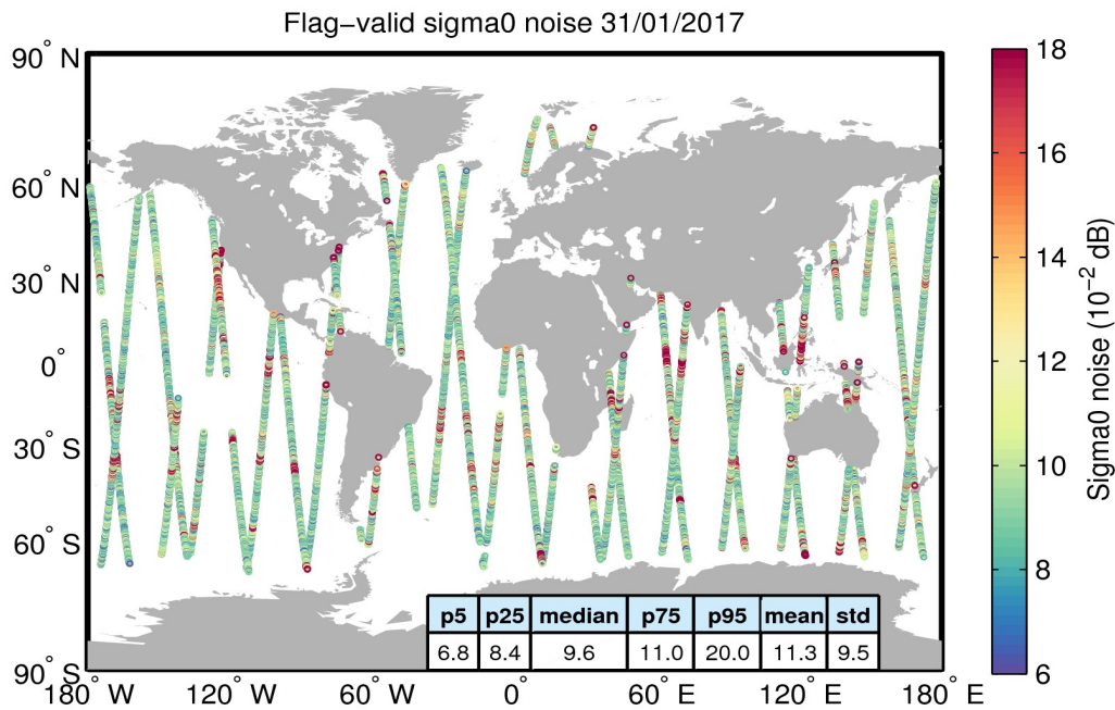
Figure 26. Geographical distribution of flag-valid 20-Hz sigma0 measurement noise over oceans and lakes for 31/01/2017. The statistical values shown in the table refer to the sigma0 noise and are calculated over all measurements shown in the figure.
