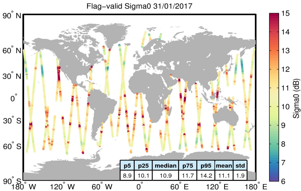
Figure 23. Geographical distribution of flag-valid sigma0 data over oceans and lakes for 31/01/2017. The statistical values shown in the table refer to the sigma0 in dB and are calculated over all measurements shown in the figure.
