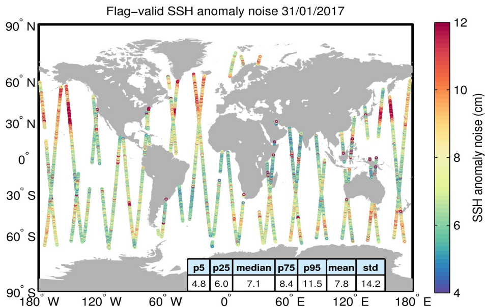
Figure 8. Geographical distribution of flag-valid 20-Hz SSH anomaly measurement noise over oceans and lakes for 31/01/2017. The statistical values shown in the table refer to the SSH anomaly noise and are calculated over all measurements shown in the figure.
