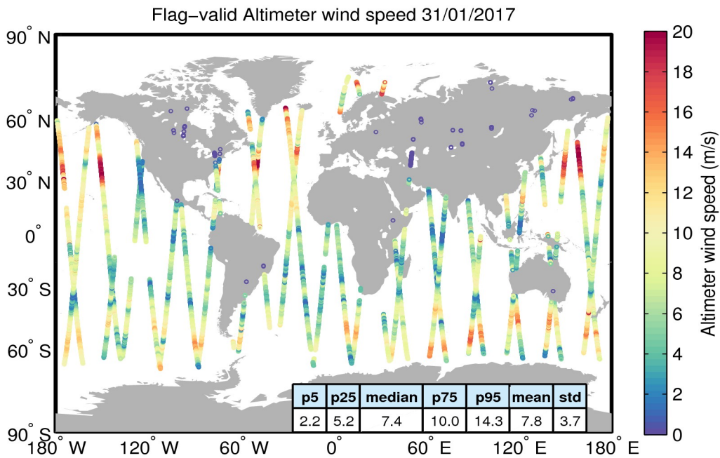
Figure 31. Geographical distribution of flag-valid wind data over oceans and lakes for 31/01/2017. The statistical values shown in the table refer to the wind in m/s and are calculated over all measurements shown in the figure.
