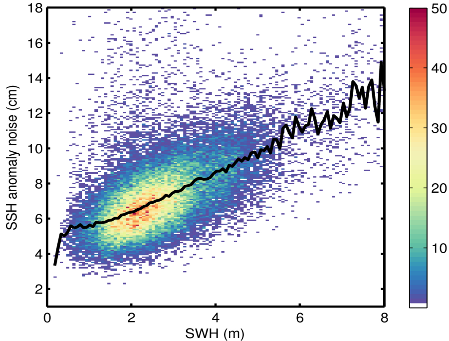
Figure 9. 2D histogram showing flag-valid SSH anomaly noise as a function of SWH for 31/01/2017. The black line denotes the median SSH anomaly noise as a function of SWH.
