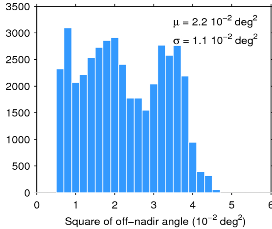
Figure 39. Histogram of flag-valid mispointing over oceans and lakes for 31/01/2017. The mean ( \mu ) and standard deviation ( \sigma ) are also shown. Note that values larger than 6 \cdot 10^{-2} \text{ deg}^2 are excluded from the histogram for the sake of readability but not from the computation of \mu and \sigma .
