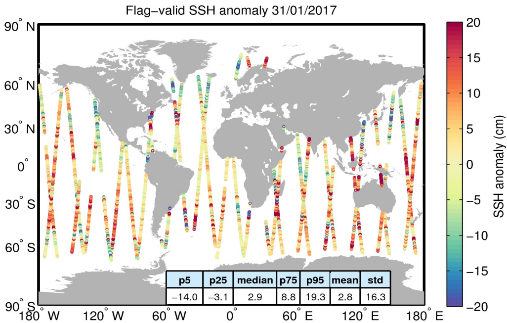
Figure 5. Geographical distribution of flag-valid 1-Hz SSH anomaly data over oceans and lakes for 31/01/2017. The statistical values shown in the table refer to the SSH anomaly in cm and are calculated over all measurements shown in the figure.
