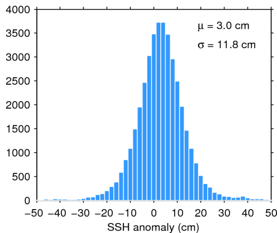
Figure 11. Histogram of science-valid SSH anomaly over oceans and lakes for 31/01/2017. The mean ( \mu ) and standard deviation ( \sigma ) are also shown. Note that values outside [-50 50] cm are excluded from the histogram for the sake of readability but not from the computation of \mu and \sigma .
