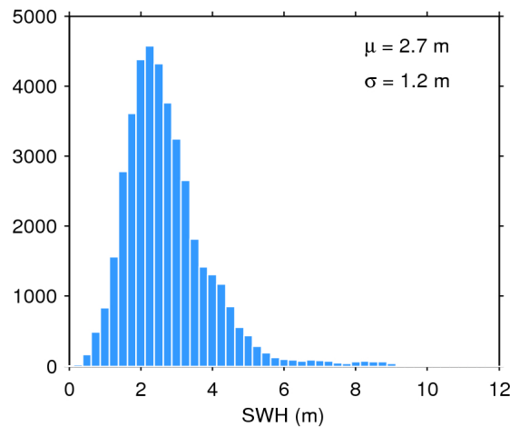
Figure 20. Histogram of science-valid SWH over oceans and lakes for 31/01/2017. The mean ( \mu ) and standard deviation ( \sigma ) are also shown. Note that values larger than 12 m are excluded from the histogram for the sake of readability but not from the computation of \mu and \sigma .
