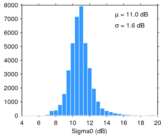
Figure 28. Histogram of science-valid sigma0 over oceans and lakes for 31/01/2017. The mean ( \mu ) and standard deviation ( \sigma ) are also shown. Note that values outside [4 20] dB are excluded from the histogram for the sake of readability but not from the computation of \mu and \sigma .
