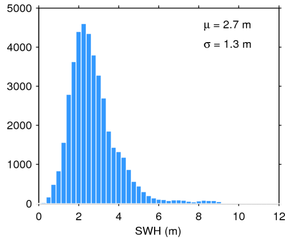
Figure 17. Histogram of flag-valid SWH over oceans and lakes for 31/01/2017. The mean ( \mu ) and standard deviation ( \sigma ) are also shown. Note that values larger than 12 m are excluded from the histogram for the sake of readability but not from the computation of \mu and \sigma .
