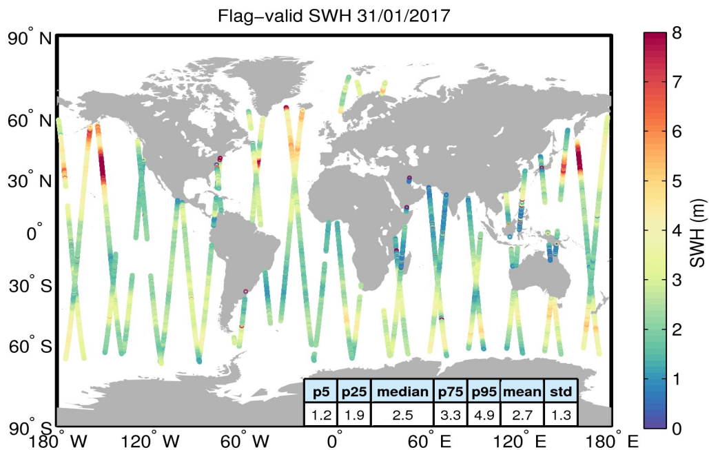
Figure 15. Geographical distribution of flag-valid SWH data over oceans and lakes for 31/01/2017. The statistical values shown in the table refer to the SWH in m and are calculated over all measurements shown in the figure.
