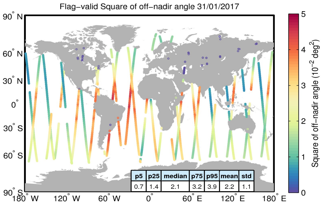
Figure 37. Geographical distribution of flag-valid mispointing data over oceans and lakes for 31/01/2017. The statistical values shown in the table refer to the mispointing in 10^{-2} deg 2 and are calculated over all measurements shown in the figure.
