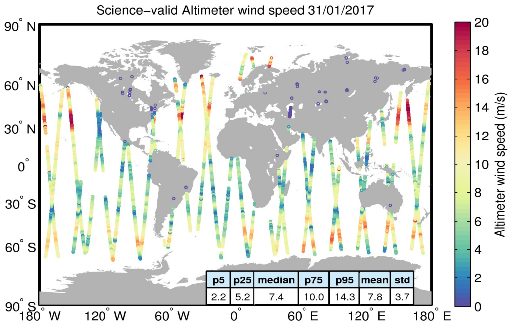
Figure 34. Geographical distribution of science-valid wind data over oceans and lakes for 31/01/2017. The statistical values shown in the table refer to the wind in m/s and are calculated over all measurements shown in the figure. Gray circles denote records that have been rejected based on the editing criteria described in Table 5.
