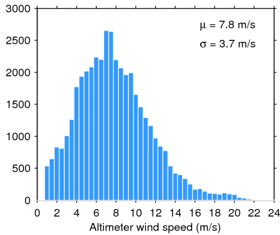
Figure 33. Histogram of flag-valid wind over oceans and lakes for 31/01/2017. The mean ( \mu ) and standard deviation ( \sigma ) are also shown. Note that values larger than 24 m/s are excluded from the histogram for the sake of readability but not from the computation of \mu and \sigma .
