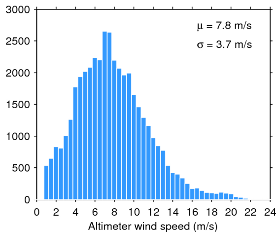
Figure 35. Histogram of science-valid wind over oceans and lakes for 31/01/2017. The mean ( \mu ) and standard deviation ( \sigma ) are also shown. Note that values larger than 24 m/s are excluded from the histogram for the sake of readability but not from the computation of \mu and \sigma .
