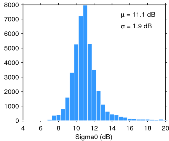
Figure 25. Histogram of flag-valid sigma0 over oceans and lakes for 31/01/2017. The mean ( \mu ) and standard deviation ( \sigma ) are also shown. Note that values outside [4 20] dB are excluded from the histogram for the sake of readability but not from the computation of \mu and \sigma .
