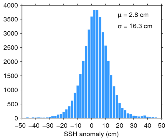
Figure 7. Histogram of flag-valid SSH anomaly over oceans and lakes for 31/01/2017. The mean ( \mu ) and standard deviation ( \sigma ) are also shown. Note that values outside [-50 50] cm are excluded from the histogram for the sake of readability but not from the computation of \mu and \sigma .
