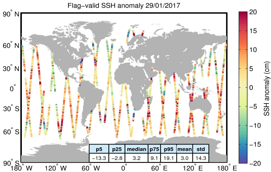
Figure 5. Geographical distribution of flag-valid 1-Hz SSH anomaly data over oceans and lakes for 29/01/2017. The statistical values shown in the table refer to the SSH anomaly in cm and are calculated over all measurements shown in the figure.
