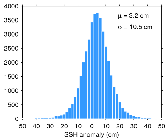
Figure 11. Histogram of science-valid SSH anomaly over oceans and lakes for 29/01/2017. The mean ( \mu ) and standard deviation ( \sigma ) are also shown. Note that values outside [-50 50] cm are excluded from the histogram for the sake of readability but not from the computation of \mu and \sigma .
