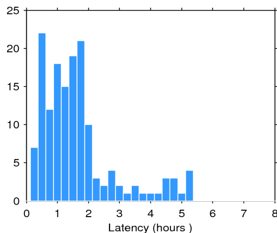
Figure 2. Histogram of the data latency for 29/01/2017. The y-axis denotes the number of files that are made available with a delay of x-hours with respect to the mean time of the records stored in the file.
