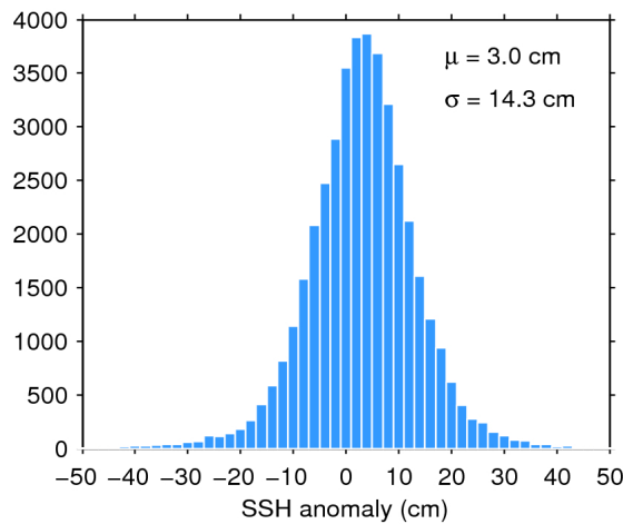
Figure 7. Histogram of flag-valid SSH anomaly over oceans and lakes for 29/01/2017. The mean ( \mu ) and standard deviation ( \sigma ) are also shown. Note that values outside [-50\ 50] cm are excluded from the histogram for the sake of readability but not from the computation of \mu and \sigma .
