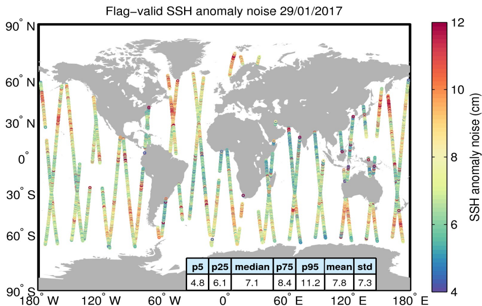
Figure 8. Geographical distribution of flag-valid 20-Hz SSH anomaly measurement noise over oceans and lakes for 29/01/2017. The statistical values shown in the table refer to the SSH anomaly noise and are calculated over all measurements shown in the figure.
