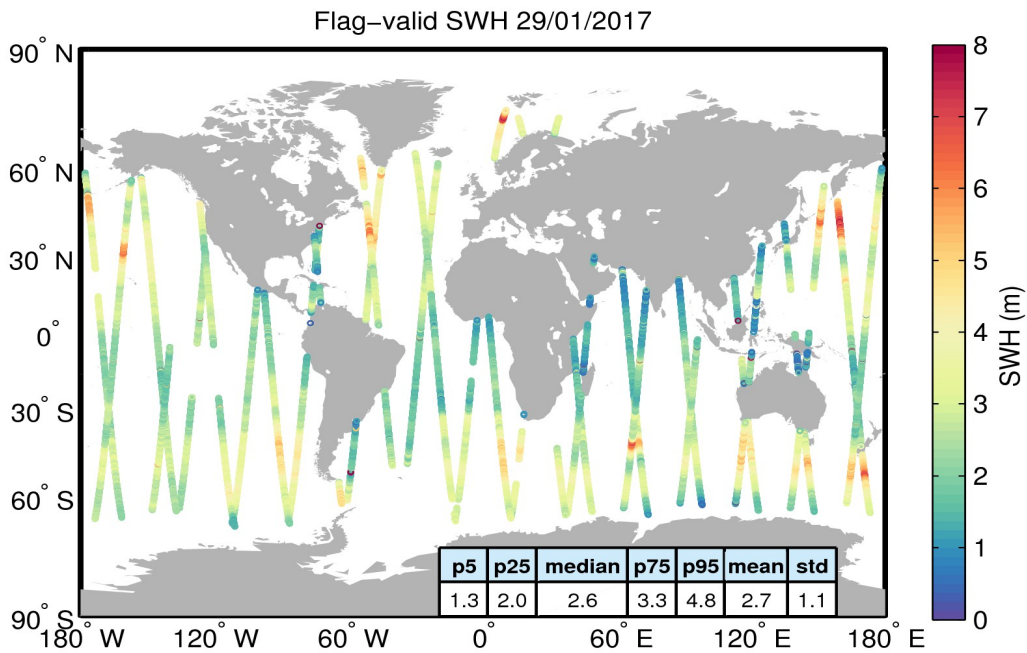
Figure 15. Geographical distribution of flag-valid SWH data over oceans and lakes for 29/01/2017. The statistical values shown in the table refer to the SWH in m and are calculated over all measurements shown in the figure.
