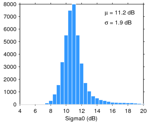
Figure 25. Histogram of flag-valid sigma0 over oceans and lakes for 29/01/2017. The mean ( \mu ) and standard deviation ( \sigma ) are also shown. Note that values outside [4 20] dB are excluded from the histogram for the sake of readability but not from the computation of \mu and \sigma .
