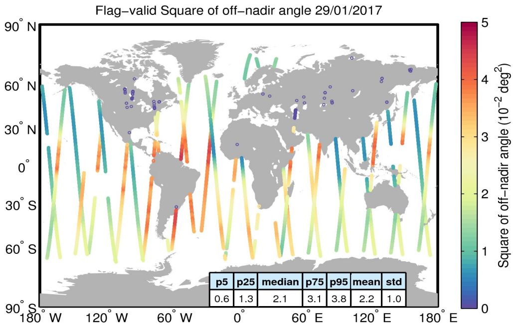
Figure 37. Geographical distribution of flag-valid mispointing data over oceans and lakes for 29/01/2017. The statistical values shown in the table refer to the mispointing in 10^{-2} deg 2 and are calculated over all measurements shown in the figure.
