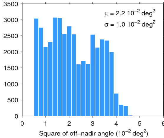
Figure 39. Histogram of flag-valid mispointing over oceans and lakes for 29/01/2017. The mean ( \mu ) and standard deviation ( \sigma ) are also shown. Note that values larger than 6 \cdot 10^{-2} \text{ deg}^2 are excluded from the histogram for the sake of readability but not from the computation of \mu and \sigma .
