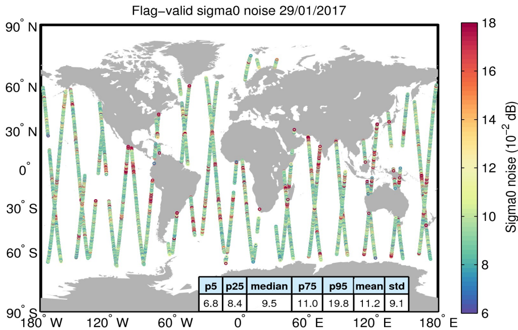
Figure 26. Geographical distribution of flag-valid 20-Hz sigma0 measurement noise over oceans and lakes for 29/01/2017. The statistical values shown in the table refer to the sigma0 noise and are calculated over all measurements shown in the figure.
