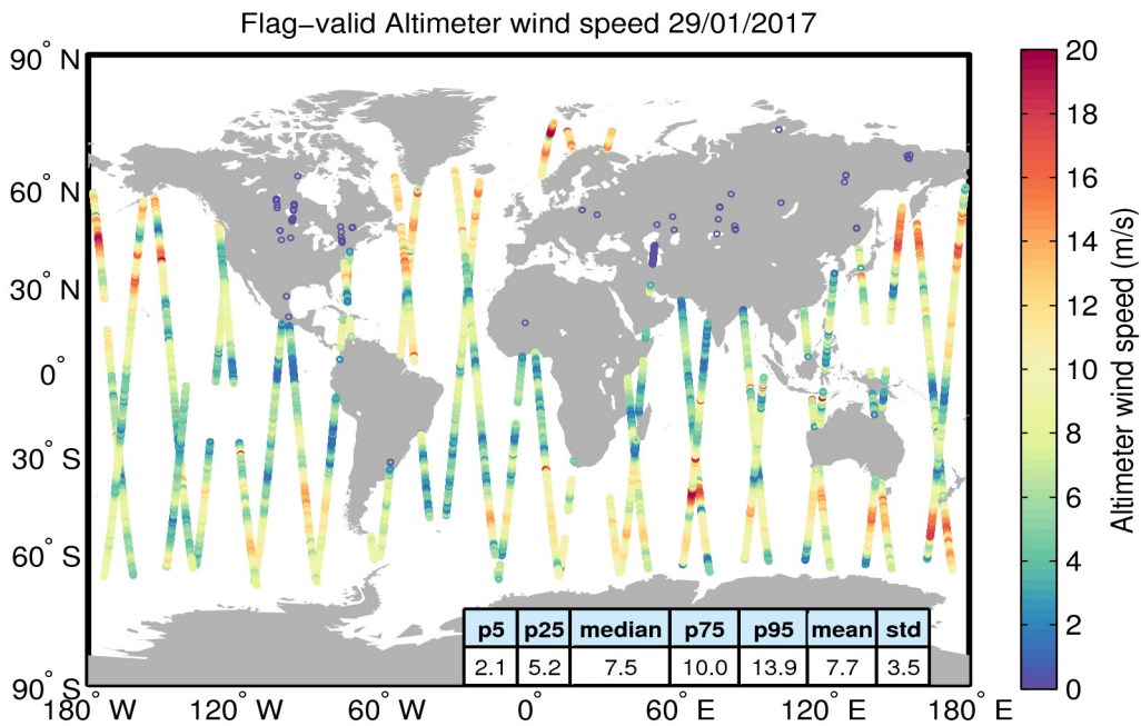
Figure 31. Geographical distribution of flag-valid wind data over oceans and lakes for 29/01/2017. The statistical values shown in the table refer to the wind in m/s and are calculated over all measurements shown in the figure.
