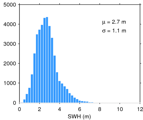
Figure 17. Histogram of flag-valid SWH over oceans and lakes for 29/01/2017. The mean ( \mu ) and standard deviation ( \sigma ) are also shown. Note that values larger than 12 m are excluded from the histogram for the sake of readability but not from the computation of \mu and \sigma .
