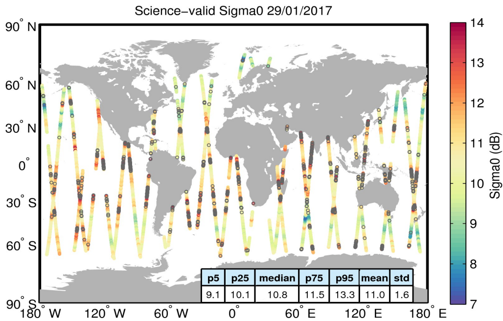
Figure 27. Geographical distribution of science-valid sigma0 data over oceans and lakes for 29/01/2017. The statistical values shown in the table refer to the sigma0 in dB and are calculated over all measurements shown in the figure. Gray circles denote records that have been rejected based on the editing criteria described in Table 4.
