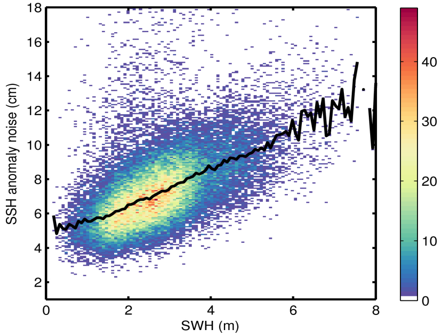
Figure 9. 2D histogram showing flag-valid SSH anomaly noise as a function of SWH for 29/01/2017. The black line denotes the median SSH anomaly noise as a function of SWH.
