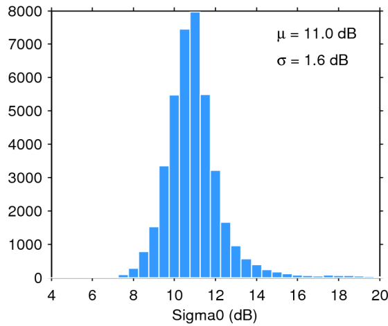
Figure 28. Histogram of science-valid sigma0 over oceans and lakes for 29/01/2017. The mean ( \mu ) and standard deviation ( \sigma ) are also shown. Note that values outside [4 20] dB are excluded from the histogram for the sake of readability but not from the computation of \mu and \sigma .
