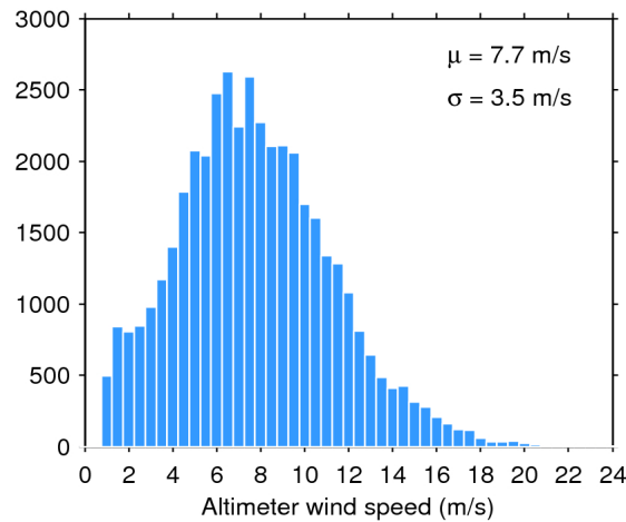
Figure 33. Histogram of flag-valid wind over oceans and lakes for 29/01/2017. The mean ( \mu ) and standard deviation ( \sigma ) are also shown. Note that values larger than 24 m/s are excluded from the histogram for the sake of readability but not from the computation of \mu and \sigma .
