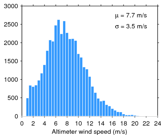
Figure 35. Histogram of science-valid wind over oceans and lakes for 29/01/2017. The mean ( \mu ) and standard deviation ( \sigma ) are also shown. Note that values larger than 24 m/s are excluded from the histogram for the sake of readability but not from the computation of \mu and \sigma .
