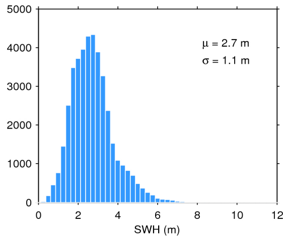
Figure 20. Histogram of science-valid SWH over oceans and lakes for 29/01/2017. The mean ( \mu ) and standard deviation ( \sigma ) are also shown. Note that values larger than 12 m are excluded from the histogram for the sake of readability but not from the computation of \mu and \sigma .
