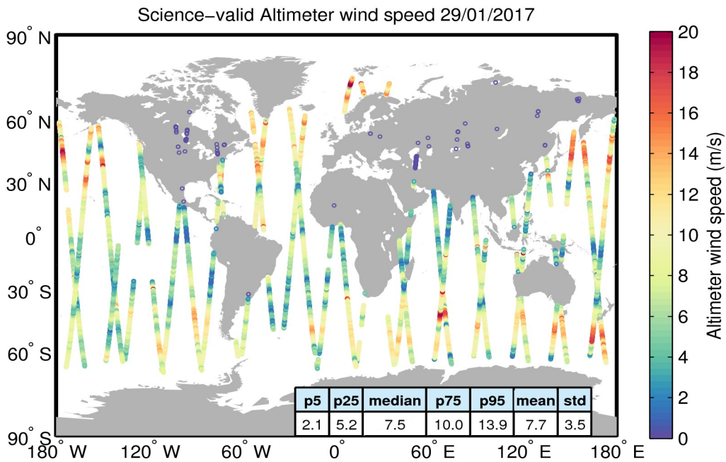
Figure 34. Geographical distribution of science-valid wind data over oceans and lakes for 29/01/2017. The statistical values shown in the table refer to the wind in m/s and are calculated over all measurements shown in the figure. Gray circles denote records that have been rejected based on the editing criteria described in Table 5.
