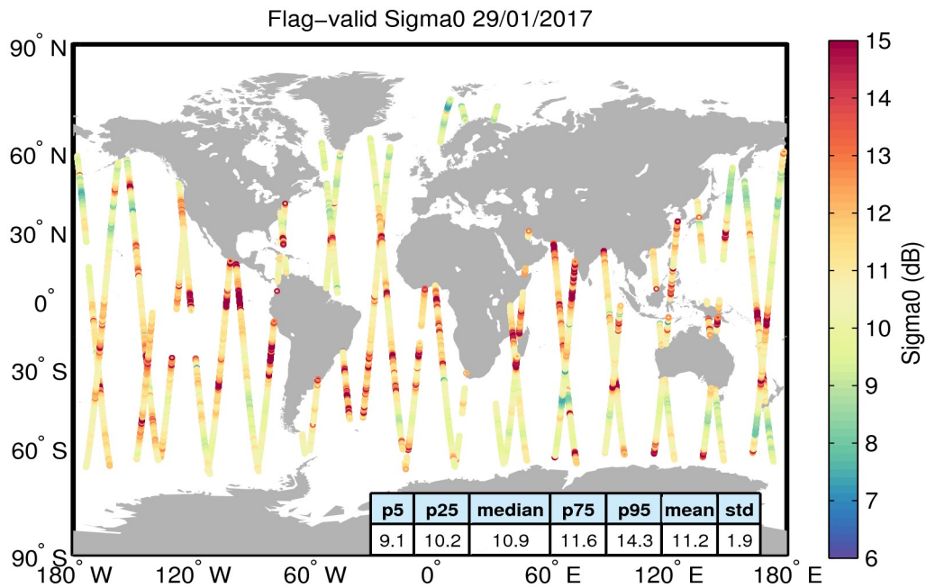
Figure 23. Geographical distribution of flag-valid sigma0 data over oceans and lakes for 29/01/2017. The statistical values shown in the table refer to the sigma0 in dB and are calculated over all measurements shown in the figure.
