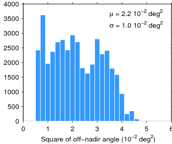
Figure 39. Histogram of flag-valid mispointing over oceans and lakes for 28/01/2017. The mean ( \mu ) and standard deviation ( \sigma ) are also shown. Note that values larger than 6 \cdot 10^{-2} \text{ deg}^2 are excluded from the histogram for the sake of readability but not from the computation of \mu and \sigma .
