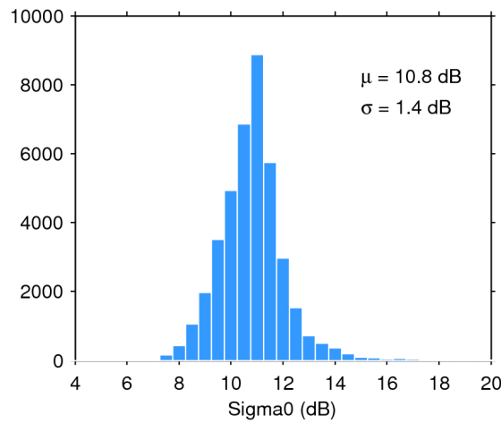
Figure 28. Histogram of science-valid sigma0 over oceans and lakes for 28/01/2017. The mean ( \mu ) and standard deviation ( \sigma ) are also shown. Note that values outside [4 20] dB are excluded from the histogram for the sake of readability but not from the computation of \mu and \sigma .
