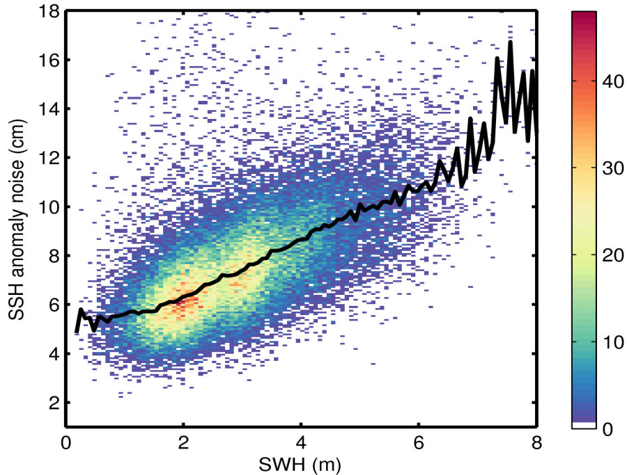
Figure 9. 2D histogram showing flag-valid SSH anomaly noise as a function of SWH for 28/01/2017. The black line denotes the median SSH anomaly noise as a function of SWH.
