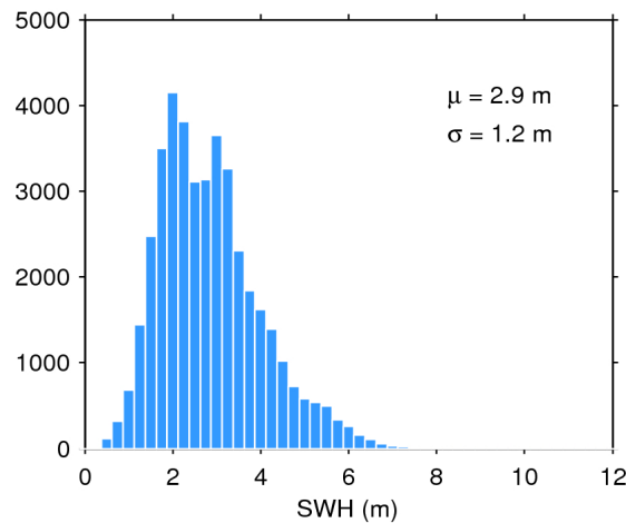
Figure 20. Histogram of science-valid SWH over oceans and lakes for 28/01/2017. The mean ( \mu ) and standard deviation ( \sigma ) are also shown. Note that values larger than 12 m are excluded from the histogram for the sake of readability but not from the computation of \mu and \sigma .
