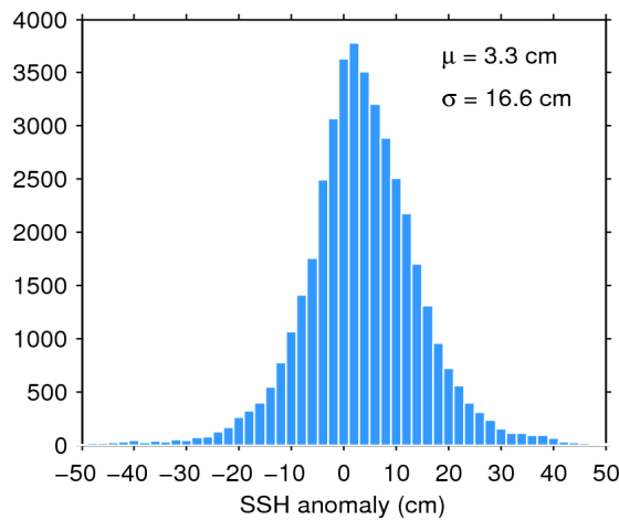
Figure 7. Histogram of flag-valid SSH anomaly over oceans and lakes for 28/01/2017. The mean ( \mu ) and standard deviation ( \sigma ) are also shown. Note that values outside [-50 50] cm are excluded from the histogram for the sake of readability but not from the computation of \mu and \sigma .
