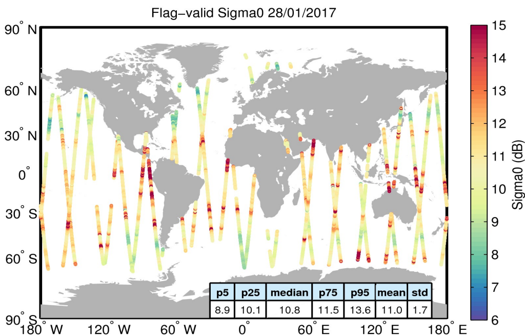
Figure 23. Geographical distribution of flag-valid sigma0 data over oceans and lakes for 28/01/2017. The statistical values shown in the table refer to the sigma0 in dB and are calculated over all measurements shown in the figure.
