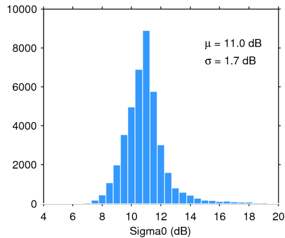
Figure 25. Histogram of flag-valid sigma0 over oceans and lakes for 28/01/2017. The mean ( \mu ) and standard deviation ( \sigma ) are also shown. Note that values outside [4 20] dB are excluded from the histogram for the sake of readability but not from the computation of \mu and \sigma .
