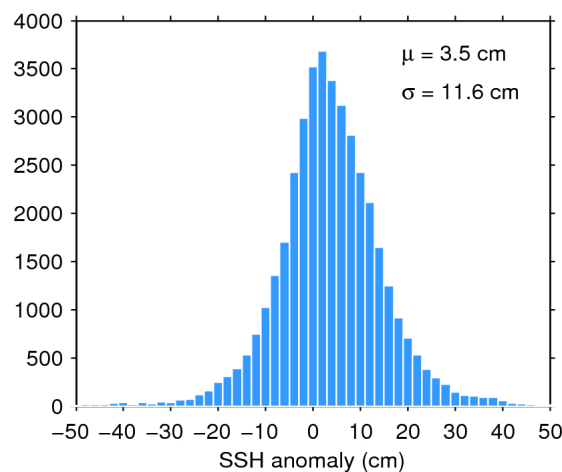
Figure 11. Histogram of science-valid SSH anomaly over oceans and lakes for 28/01/2017. The mean ( \mu ) and standard deviation ( \sigma ) are also shown. Note that values outside [-50 50] cm are excluded from the histogram for the sake of readability but not from the computation of \mu and \sigma .
