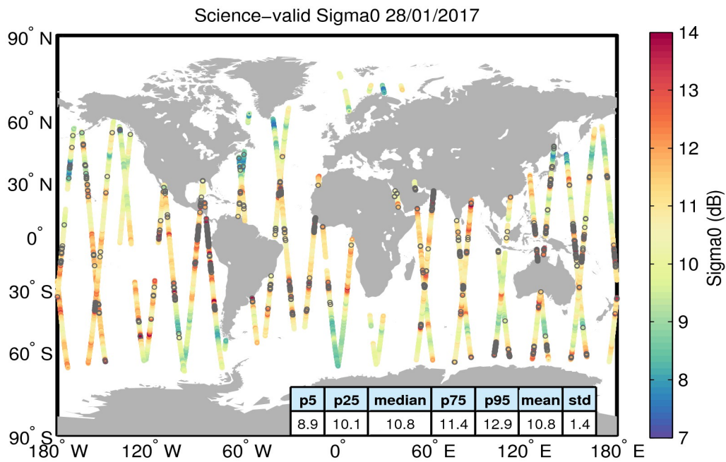
Figure 27. Geographical distribution of science-valid sigma0 data over oceans and lakes for 28/01/2017. The statistical values shown in the table refer to the sigma0 in dB and are calculated over all measurements shown in the figure. Gray circles denote records that have been rejected based on the editing criteria described in Table 4.
