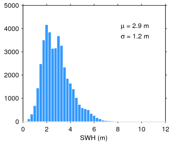
Figure 17. Histogram of flag-valid SWH over oceans and lakes for 28/01/2017. The mean ( \mu ) and standard deviation ( \sigma ) are also shown. Note that values larger than 12 m are excluded from the histogram for the sake of readability but not from the computation of \mu and \sigma .
