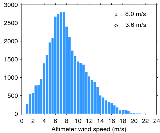
Figure 33. Histogram of flag-valid wind over oceans and lakes for 28/01/2017. The mean ( \mu ) and standard deviation ( \sigma ) are also shown. Note that values larger than 24 m/s are excluded from the histogram for the sake of readability but not from the computation of \mu and \sigma .
