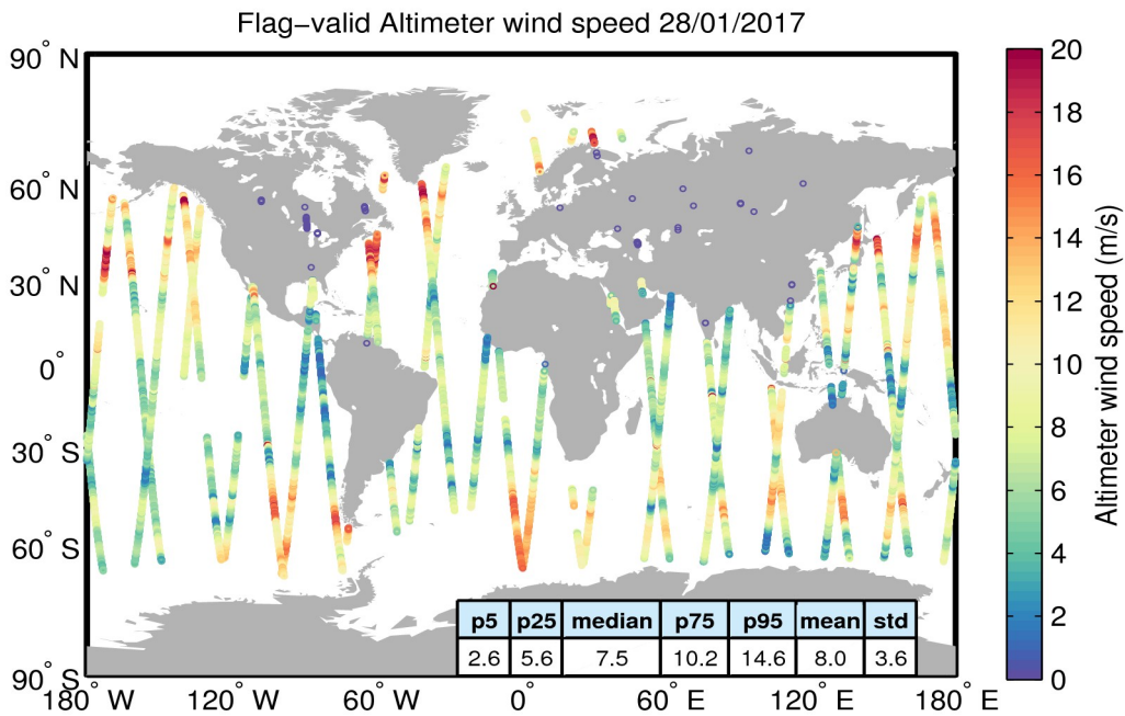
Figure 31. Geographical distribution of flag-valid wind data over oceans and lakes for 28/01/2017. The statistical values shown in the table refer to the wind in m/s and are calculated over all measurements shown in the figure.
