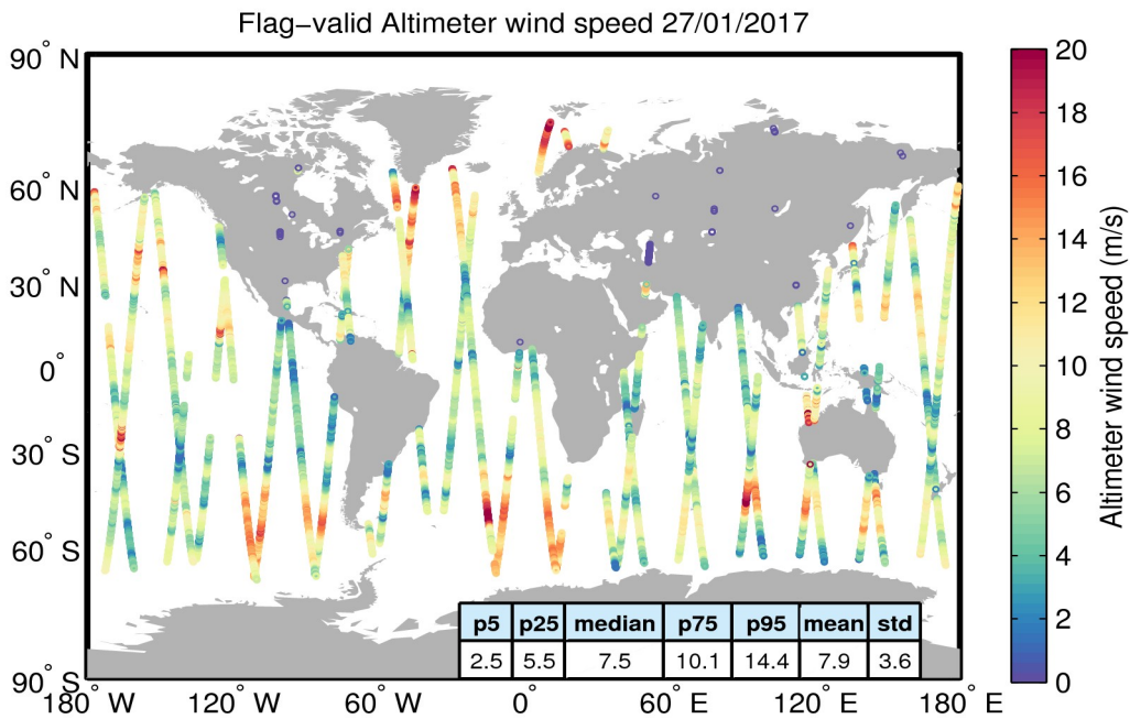
Figure 31. Geographical distribution of flag-valid wind data over oceans and lakes for 27/01/2017. The statistical values shown in the table refer to the wind in m/s and are calculated over all measurements shown in the figure.
