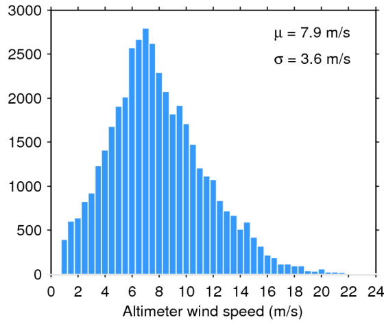
Figure 33. Histogram of flag-valid wind over oceans and lakes for 27/01/2017. The mean ( \mu ) and standard deviation ( \sigma ) are also shown. Note that values larger than 24 m/s are excluded from the histogram for the sake of readability but not from the computation of \mu and \sigma .
