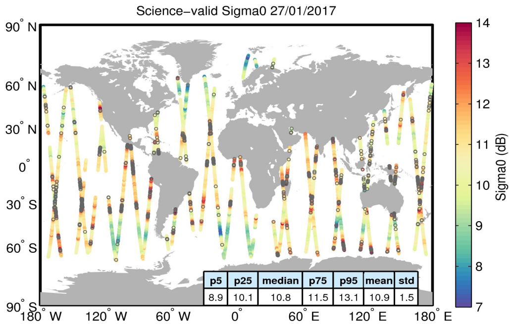
Figure 27. Geographical distribution of science-valid sigma0 data over oceans and lakes for 27/01/2017. The statistical values shown in the table refer to the sigma0 in dB and are calculated over all measurements shown in the figure. Gray circles denote records that have been rejected based on the editing criteria described in Table 4.
