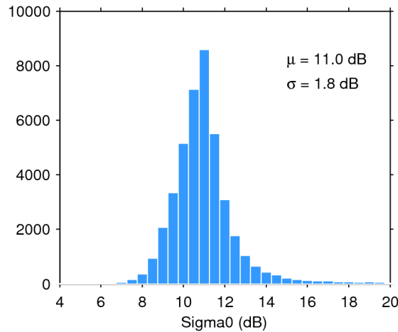
Figure 25. Histogram of flag-valid sigma0 over oceans and lakes for 27/01/2017. The mean ( \mu ) and standard deviation ( \sigma ) are also shown. Note that values outside [4 20] dB are excluded from the histogram for the sake of readability but not from the computation of \mu and \sigma .
