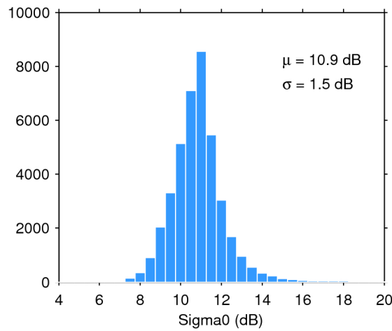
Figure 28. Histogram of science-valid sigma0 over oceans and lakes for 27/01/2017. The mean ( \mu ) and standard deviation ( \sigma ) are also shown. Note that values outside [4 20] dB are excluded from the histogram for the sake of readability but not from the computation of \mu and \sigma .
