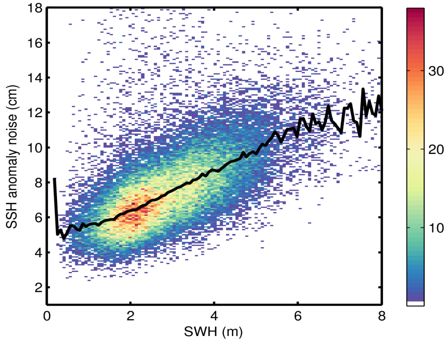
Figure 9. 2D histogram showing flag-valid SSH anomaly noise as a function of SWH for 27/01/2017. The black line denotes the median SSH anomaly noise as a function of SWH.
