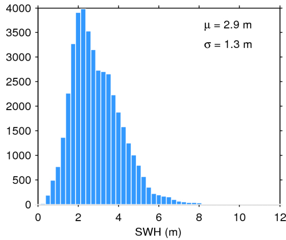
Figure 17. Histogram of flag-valid SWH over oceans and lakes for 27/01/2017. The mean ( \mu ) and standard deviation ( \sigma ) are also shown. Note that values larger than 12 m are excluded from the histogram for the sake of readability but not from the computation of \mu and \sigma .
