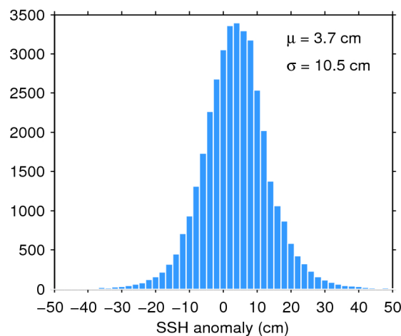
Figure 11. Histogram of science-valid SSH anomaly over oceans and lakes for 27/01/2017. The mean ( \mu ) and standard deviation ( \sigma ) are also shown. Note that values outside [-50 50] cm are excluded from the histogram for the sake of readability but not from the computation of \mu and \sigma .
