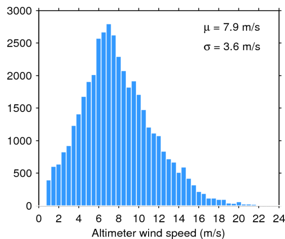
Figure 35. Histogram of science-valid wind over oceans and lakes for 27/01/2017. The mean ( \mu ) and standard deviation ( \sigma ) are also shown. Note that values larger than 24 m/s are excluded from the histogram for the sake of readability but not from the computation of \mu and \sigma .
