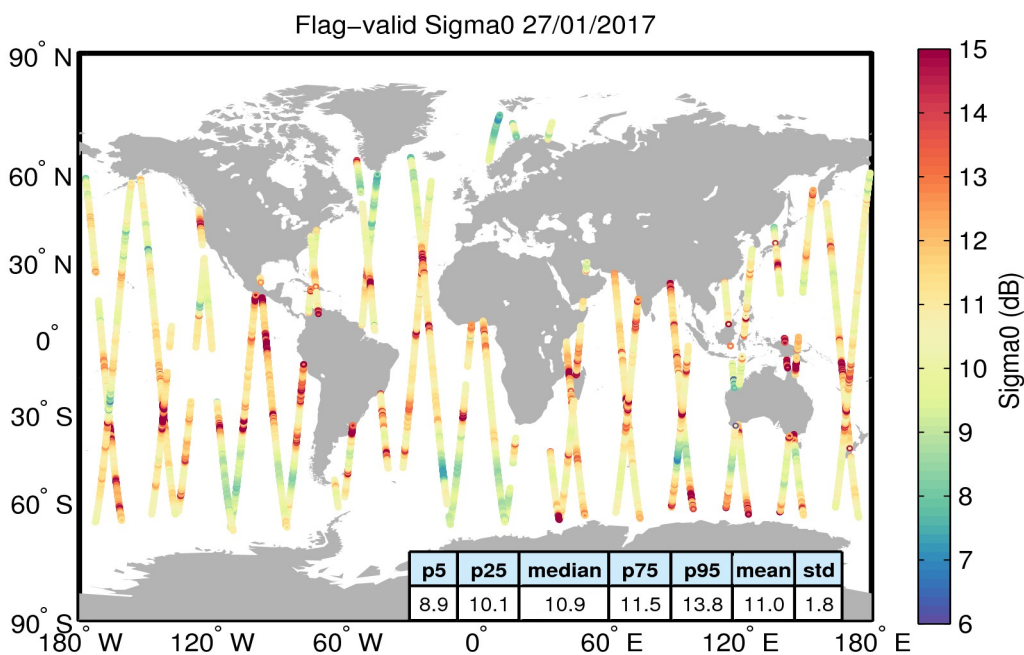
Figure 23. Geographical distribution of flag-valid sigma0 data over oceans and lakes for 27/01/2017. The statistical values shown in the table refer to the sigma0 in dB and are calculated over all measurements shown in the figure.
