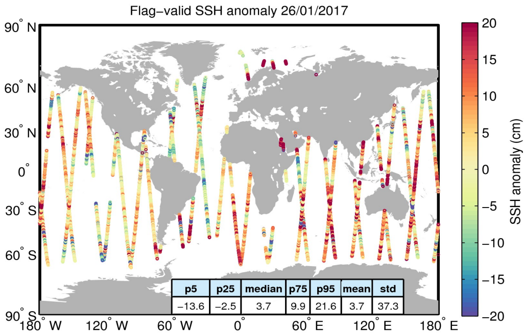
Figure 5. Geographical distribution of flag-valid 1-Hz SSH anomaly data over oceans and lakes for 26/01/2017. The statistical values shown in the table refer to the SSH anomaly in cm and are calculated over all measurements shown in the figure.
