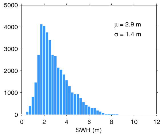
Figure 17. Histogram of flag-valid SWH over oceans and lakes for 26/01/2017. The mean ( \mu ) and standard deviation ( \sigma ) are also shown. Note that values larger than 12 m are excluded from the histogram for the sake of readability but not from the computation of \mu and \sigma .
