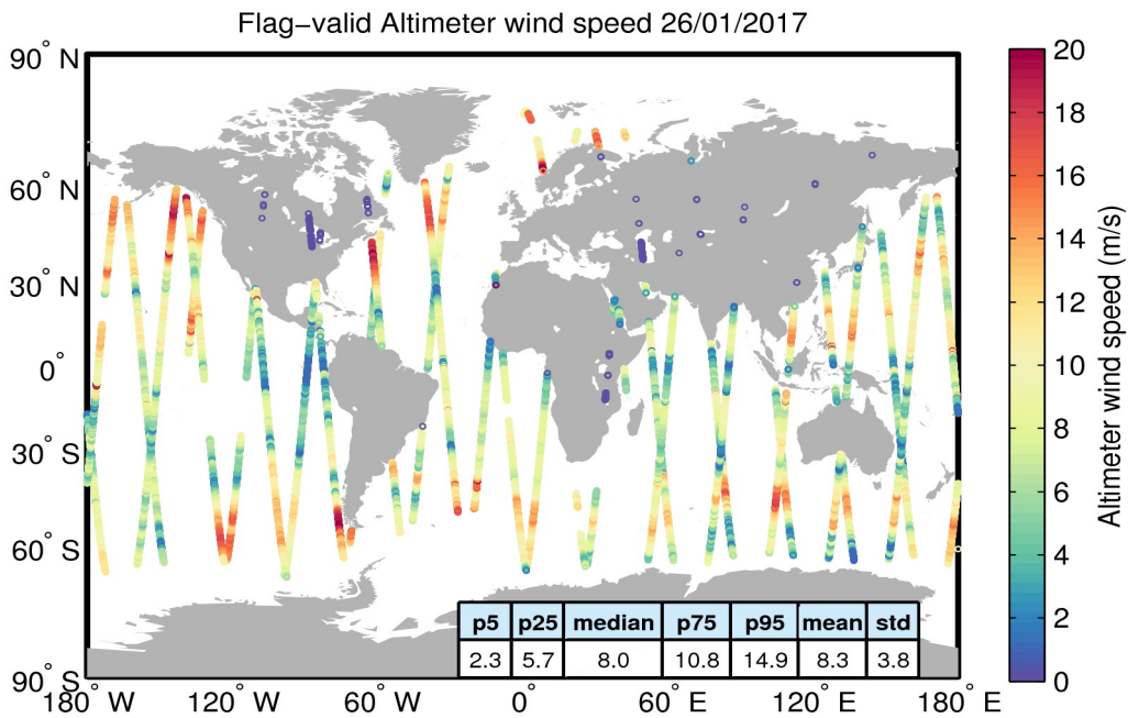
Figure 31. Geographical distribution of flag-valid wind data over oceans and lakes for 26/01/2017. The statistical values shown in the table refer to the wind in m/s and are calculated over all measurements shown in the figure.
