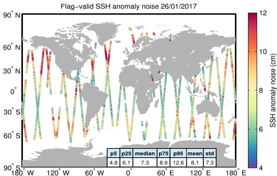
Figure 8. Geographical distribution of flag-valid 20-Hz SSH anomaly measurement noise over oceans and lakes for 26/01/2017. The statistical values shown in the table refer to the SSH anomaly noise and are calculated over all measurements shown in the figure.
