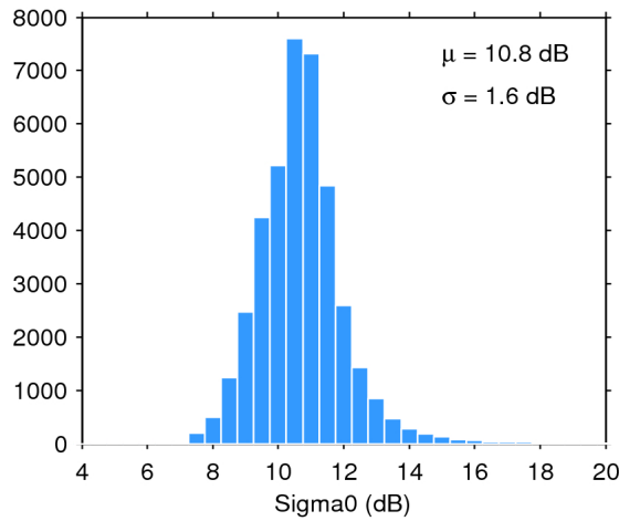
Figure 28. Histogram of science-valid sigma0 over oceans and lakes for 26/01/2017. The mean ( \mu ) and standard deviation ( \sigma ) are also shown. Note that values outside [4 20] dB are excluded from the histogram for the sake of readability but not from the computation of \mu and \sigma .
