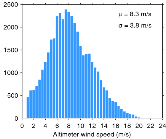
Figure 33. Histogram of flag-valid wind over oceans and lakes for 26/01/2017. The mean ( \mu ) and standard deviation ( \sigma ) are also shown. Note that values larger than 24 m/s are excluded from the histogram for the sake of readability but not from the computation of \mu and \sigma .
