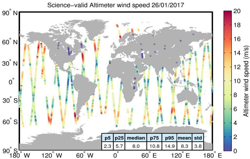
Figure 34. Geographical distribution of science-valid wind data over oceans and lakes for 26/01/2017. The statistical values shown in the table refer to the wind in m/s and are calculated over all measurements shown in the figure. Gray circles denote records that have been rejected based on the editing criteria described in Table 5.
