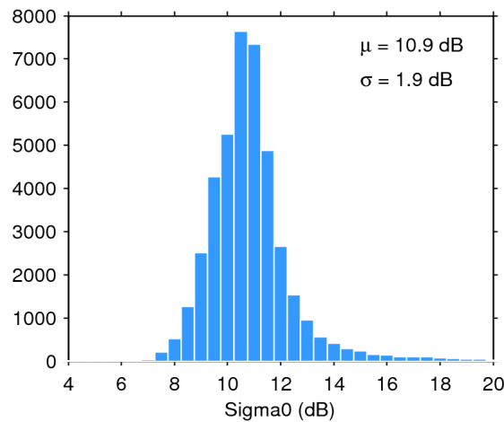
Figure 25. Histogram of flag-valid sigma0 over oceans and lakes for 26/01/2017. The mean ( \mu ) and standard deviation ( \sigma ) are also shown. Note that values outside [4 20] dB are excluded from the histogram for the sake of readability but not from the computation of \mu and \sigma .
