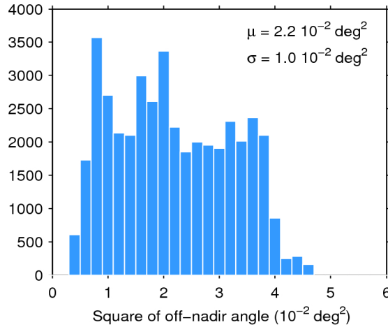
Figure 39. Histogram of flag-valid mispointing over oceans and lakes for 26/01/2017. The mean ( \mu ) and standard deviation ( \sigma ) are also shown. Note that values larger than 6 \cdot 10^{-2} \text{ deg}^2 are excluded from the histogram for the sake of readability but not from the computation of \mu and \sigma .
