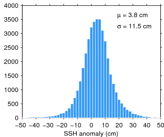
Figure 11. Histogram of science-valid SSH anomaly over oceans and lakes for 26/01/2017. The mean ( \mu ) and standard deviation ( \sigma ) are also shown. Note that values outside [-50 50] cm are excluded from the histogram for the sake of readability but not from the computation of \mu and \sigma .
