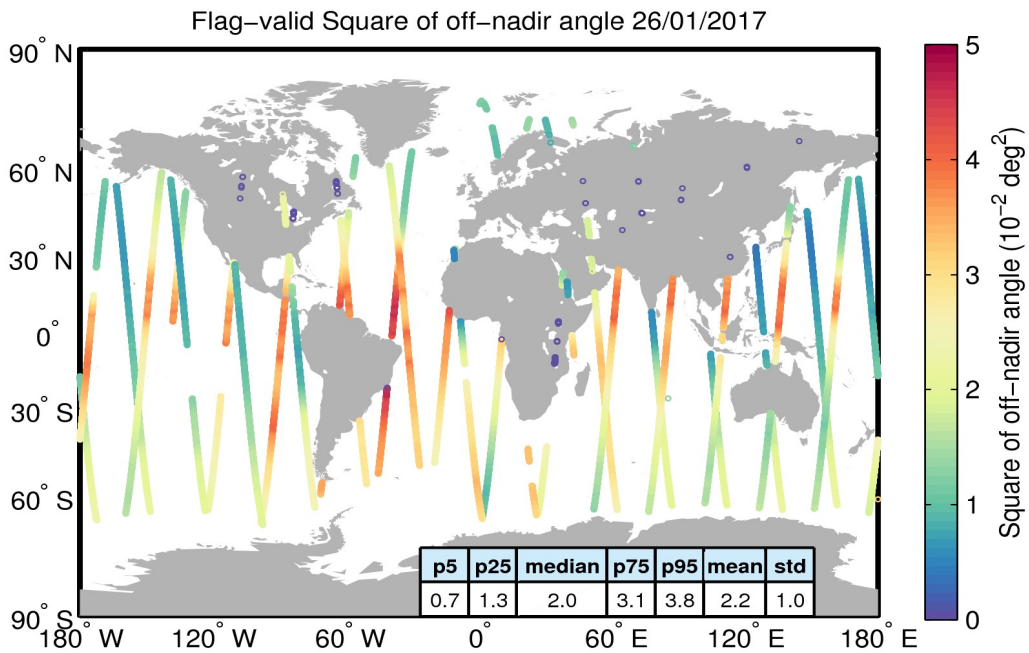
Figure 37. Geographical distribution of flag-valid mispointing data over oceans and lakes for 26/01/2017. The statistical values shown in the table refer to the mispointing in 10^{-2} deg 2 and are calculated over all measurements shown in the figure.
