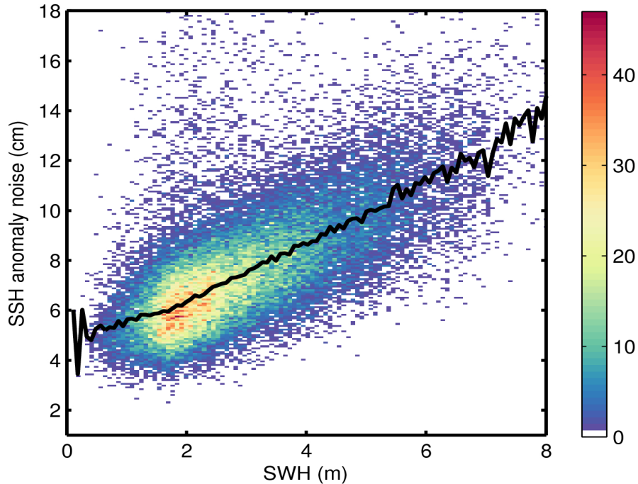
Figure 9. 2D histogram showing flag-valid SSH anomaly noise as a function of SWH for 26/01/2017. The black line denotes the median SSH anomaly noise as a function of SWH.
