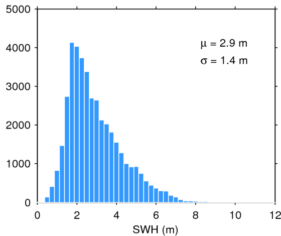
Figure 20. Histogram of science-valid SWH over oceans and lakes for 26/01/2017. The mean ( \mu ) and standard deviation ( \sigma ) are also shown. Note that values larger than 12 m are excluded from the histogram for the sake of readability but not from the computation of \mu and \sigma .
