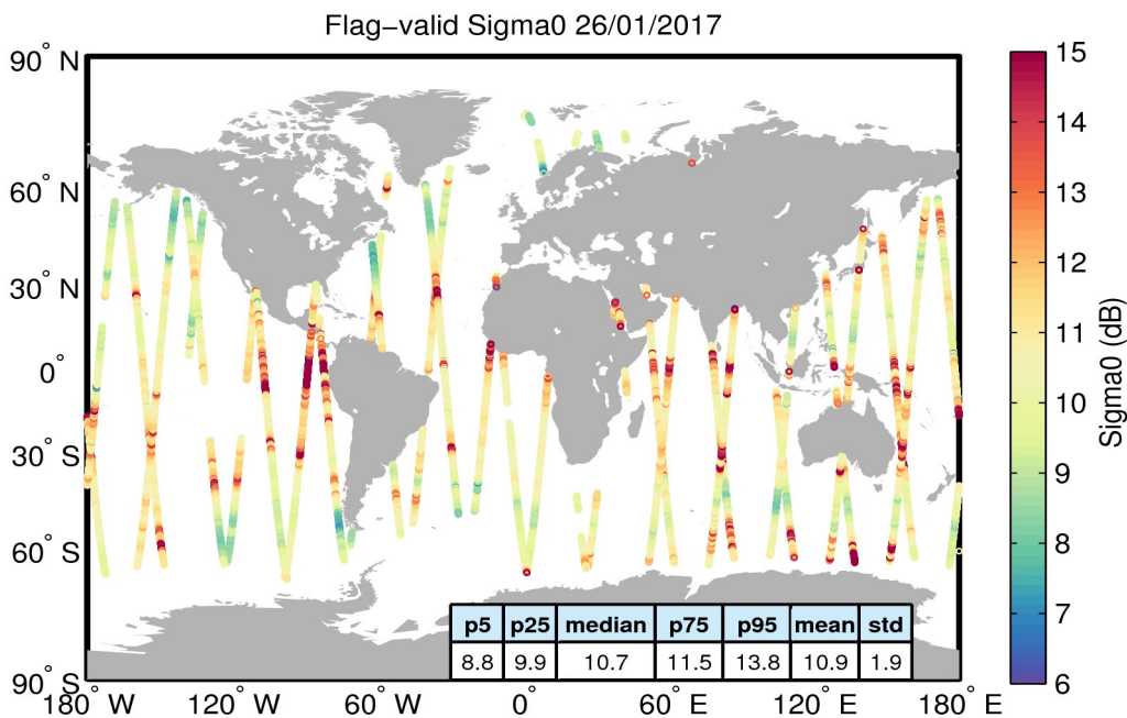
Figure 23. Geographical distribution of flag-valid sigma0 data over oceans and lakes for 26/01/2017. The statistical values shown in the table refer to the sigma0 in dB and are calculated over all measurements shown in the figure.
