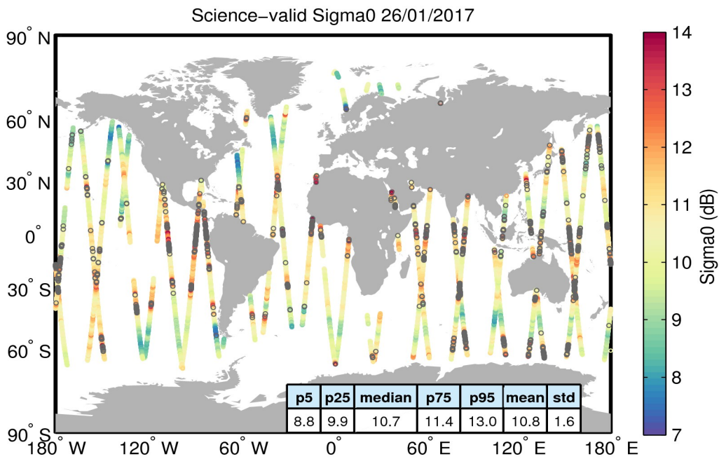
Figure 27. Geographical distribution of science-valid sigma0 data over oceans and lakes for 26/01/2017. The statistical values shown in the table refer to the sigma0 in dB and are calculated over all measurements shown in the figure. Gray circles denote records that have been rejected based on the editing criteria described in Table 4.
