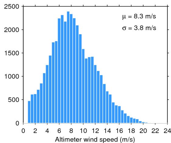
Figure 35. Histogram of science-valid wind over oceans and lakes for 26/01/2017. The mean ( \mu ) and standard deviation ( \sigma ) are also shown. Note that values larger than 24 m/s are excluded from the histogram for the sake of readability but not from the computation of \mu and \sigma .
