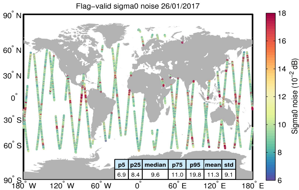
Figure 26. Geographical distribution of flag-valid 20-Hz sigma0 measurement noise over oceans and lakes for 26/01/2017. The statistical values shown in the table refer to the sigma0 noise and are calculated over all measurements shown in the figure.
