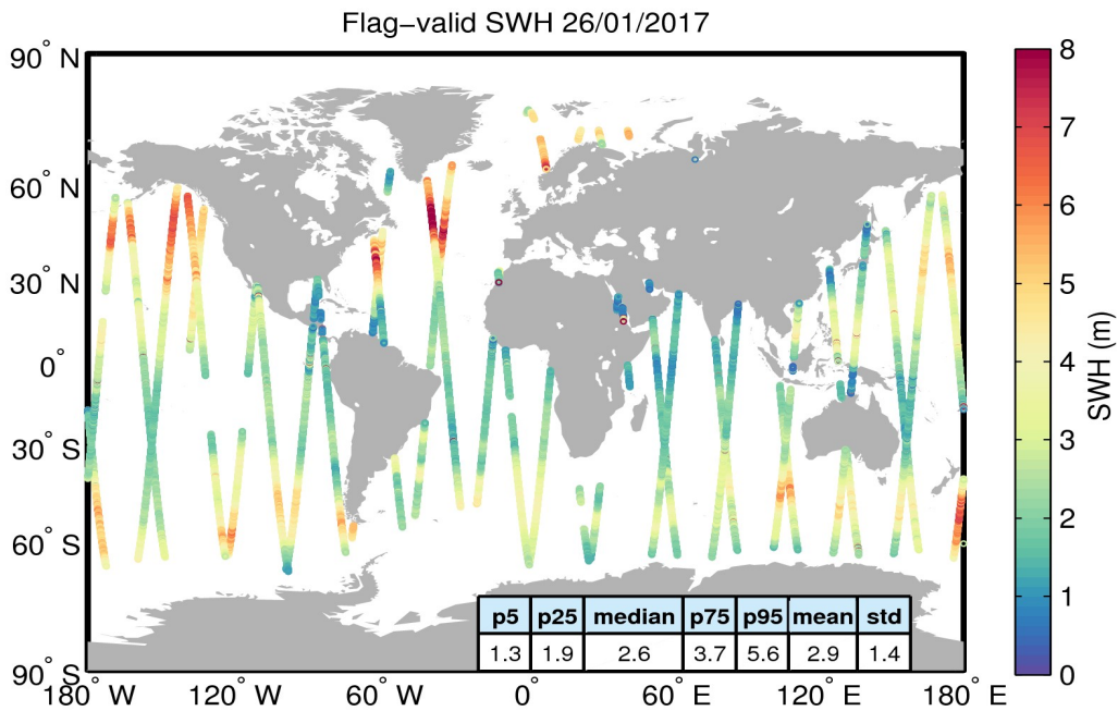
Figure 15. Geographical distribution of flag-valid SWH data over oceans and lakes for 26/01/2017. The statistical values shown in the table refer to the SWH in m and are calculated over all measurements shown in the figure.
