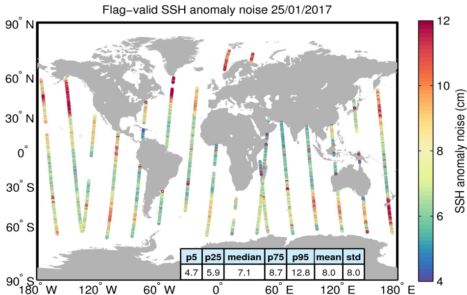
Figure 8. Geographical distribution of flag-valid 20-Hz SSH anomaly measurement noise over oceans and lakes for 25/01/2017. The statistical values shown in the table refer to the SSH anomaly noise and are calculated over all measurements shown in the figure.
