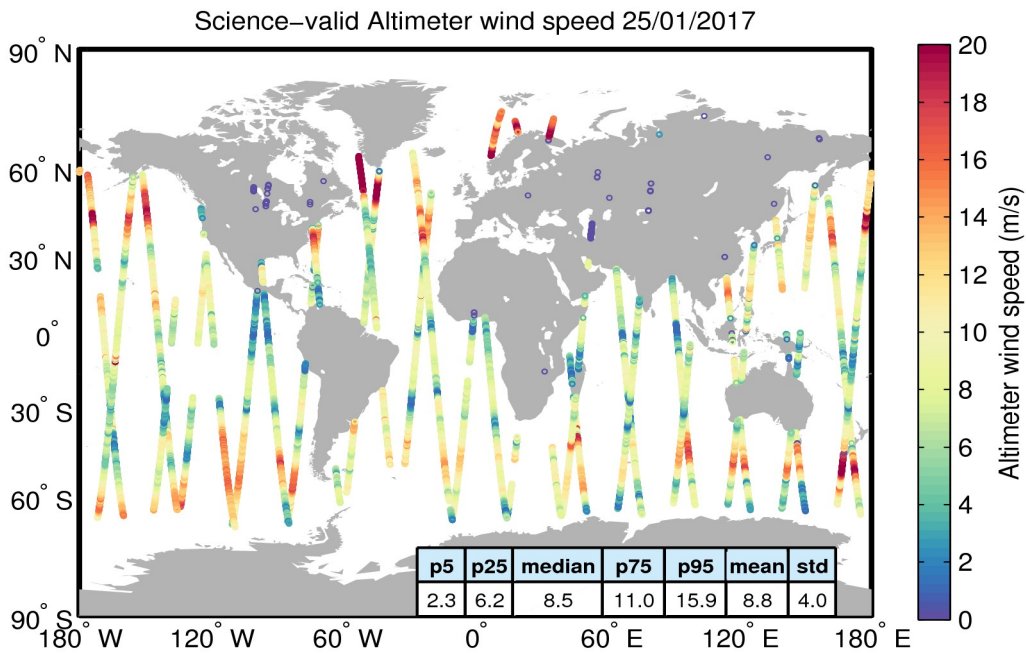
Figure 34. Geographical distribution of science-valid wind data over oceans and lakes for 25/01/2017. The statistical values shown in the table refer to the wind in m/s and are calculated over all measurements shown in the figure. Gray circles denote records that have been rejected based on the editing criteria described in Table 5.
