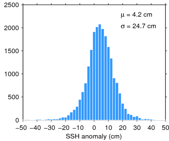
Figure 7. Histogram of flag-valid SSH anomaly over oceans and lakes for 25/01/2017. The mean ( \mu ) and standard deviation ( \sigma ) are also shown. Note that values outside [-50 50] cm are excluded from the histogram for the sake of readability but not from the computation of \mu and \sigma .
