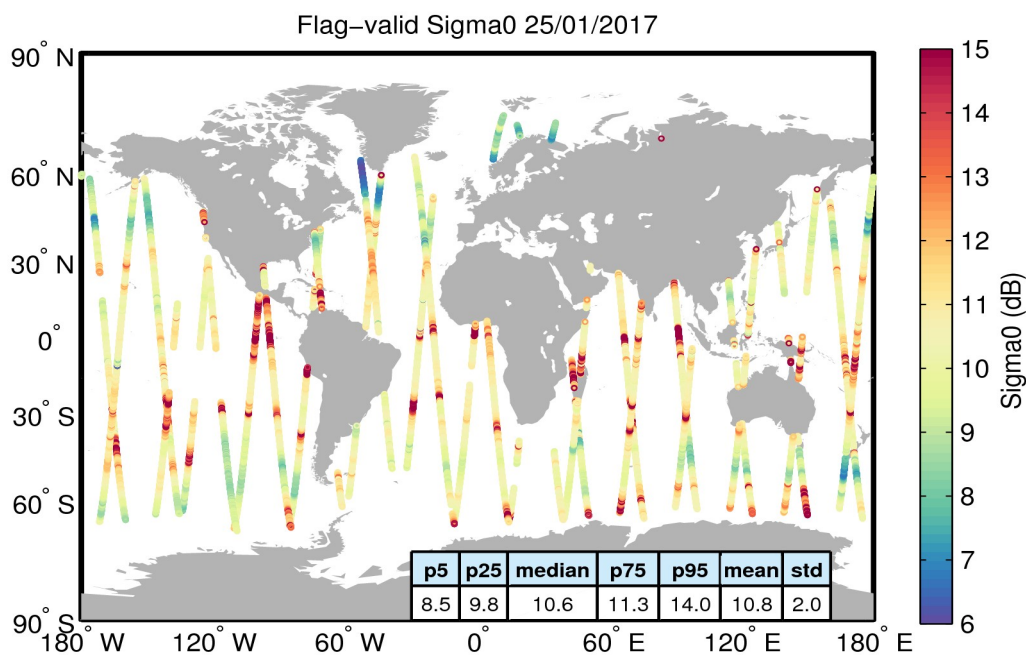
Figure 23. Geographical distribution of flag-valid sigma0 data over oceans and lakes for 25/01/2017. The statistical values shown in the table refer to the sigma0 in dB and are calculated over all measurements shown in the figure.
