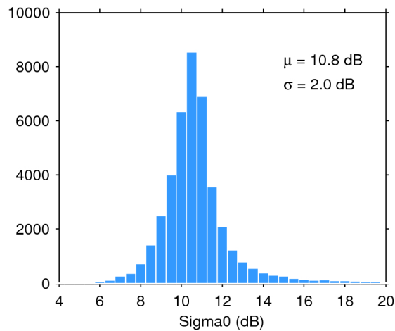
Figure 25. Histogram of flag-valid sigma0 over oceans and lakes for 25/01/2017. The mean ( \mu ) and standard deviation ( \sigma ) are also shown. Note that values outside [4 20] dB are excluded from the histogram for the sake of readability but not from the computation of \mu and \sigma .
