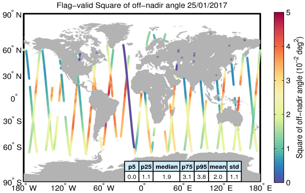
Figure 37. Geographical distribution of flag-valid mispointing data over oceans and lakes for 25/01/2017. The statistical values shown in the table refer to the mispointing in 10^{-2} deg 2 and are calculated over all measurements shown in the figure.
