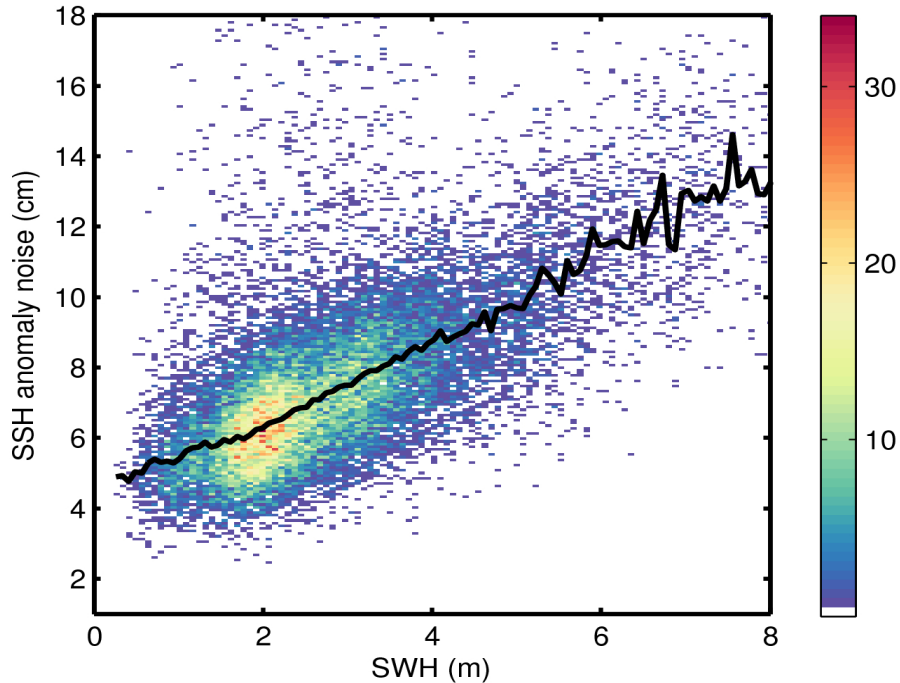
Figure 9. 2D histogram showing flag-valid SSH anomaly noise as a function of SWH for 25/01/2017. The black line denotes the median SSH anomaly noise as a function of SWH.
