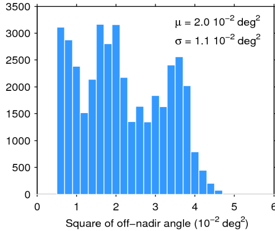
Figure 39. Histogram of flag-valid mispointing over oceans and lakes for 25/01/2017. The mean ( \mu ) and standard deviation ( \sigma ) are also shown. Note that values larger than 6 \cdot 10^{-2} \text{ deg}^2 are excluded from the histogram for the sake of readability but not from the computation of \mu and \sigma .
