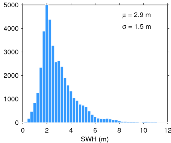
Figure 20. Histogram of science-valid SWH over oceans and lakes for 25/01/2017. The mean ( \mu ) and standard deviation ( \sigma ) are also shown. Note that values larger than 12 m are excluded from the histogram for the sake of readability but not from the computation of \mu and \sigma .
