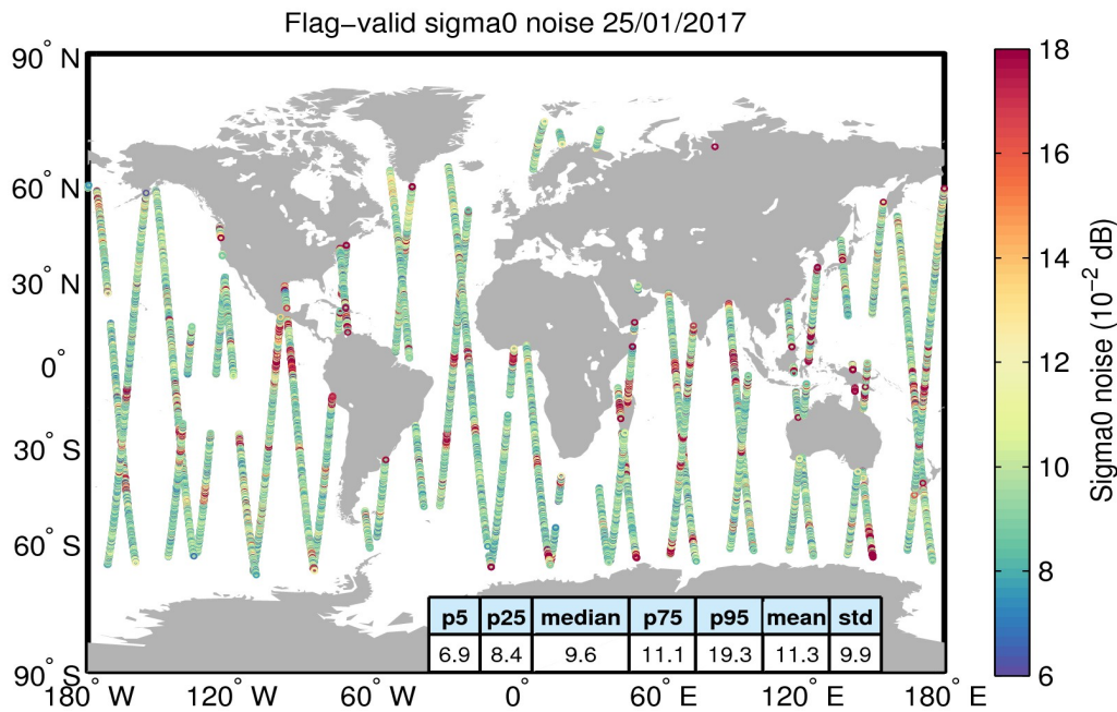
Figure 26. Geographical distribution of flag-valid 20-Hz sigma0 measurement noise over oceans and lakes for 25/01/2017. The statistical values shown in the table refer to the sigma0 noise and are calculated over all measurements shown in the figure.
