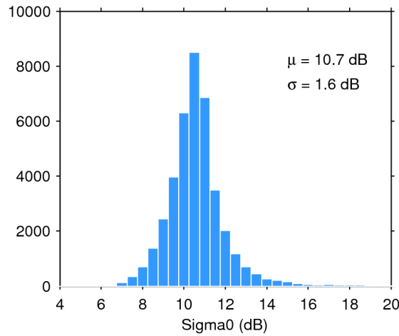
Figure 28. Histogram of science-valid sigma0 over oceans and lakes for 25/01/2017. The mean ( \mu ) and standard deviation ( \sigma ) are also shown. Note that values outside [4 20] dB are excluded from the histogram for the sake of readability but not from the computation of \mu and \sigma .
