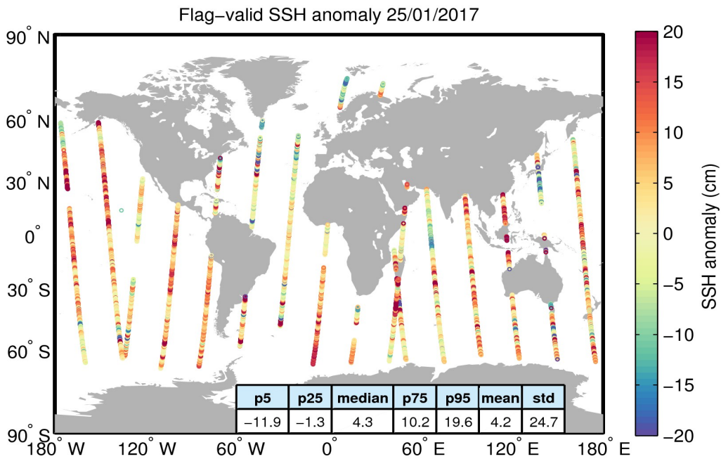
Figure 5. Geographical distribution of flag-valid 1-Hz SSH anomaly data over oceans and lakes for 25/01/2017. The statistical values shown in the table refer to the SSH anomaly in cm and are calculated over all measurements shown in the figure.
