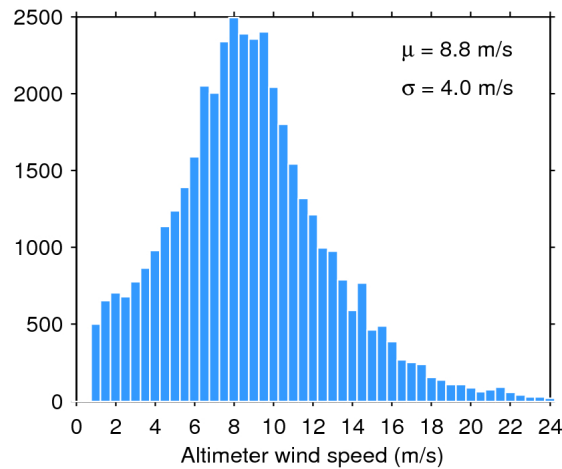
Figure 33. Histogram of flag-valid wind over oceans and lakes for 25/01/2017. The mean ( \mu ) and standard deviation ( \sigma ) are also shown. Note that values larger than 24 m/s are excluded from the histogram for the sake of readability but not from the computation of \mu and \sigma .
