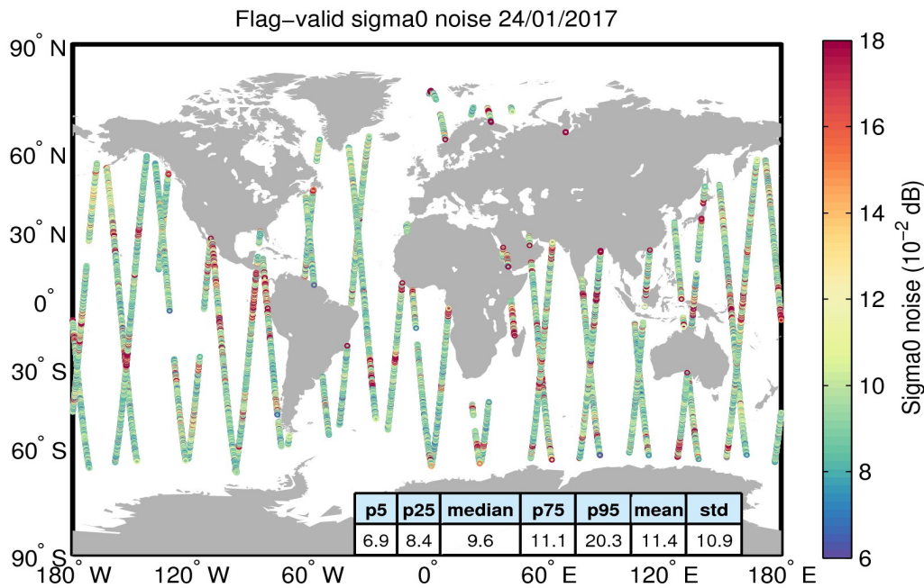
Figure 26. Geographical distribution of flag-valid 20-Hz sigma0 measurement noise over oceans and lakes for 24/01/2017. The statistical values shown in the table refer to the sigma0 noise and are calculated over all measurements shown in the figure.
