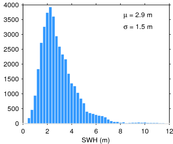
Figure 20. Histogram of science-valid SWH over oceans and lakes for 24/01/2017. The mean ( \mu ) and standard deviation ( \sigma ) are also shown. Note that values larger than 12 m are excluded from the histogram for the sake of readability but not from the computation of \mu and \sigma .
