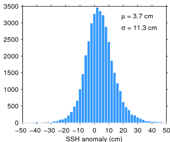
Figure 11. Histogram of science-valid SSH anomaly over oceans and lakes for 24/01/2017. The mean ( \mu ) and standard deviation ( \sigma ) are also shown. Note that values outside [-50 50] cm are excluded from the histogram for the sake of readability but not from the computation of \mu and \sigma .
