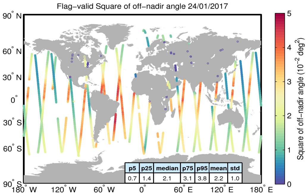
Figure 37. Geographical distribution of flag-valid mispointing data over oceans and lakes for 24/01/2017. The statistical values shown in the table refer to the mispointing in 10^{-2} deg 2 and are calculated over all measurements shown in the figure.
