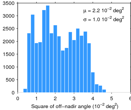
Figure 39. Histogram of flag-valid mispointing over oceans and lakes for 24/01/2017. The mean ( \mu ) and standard deviation ( \sigma ) are also shown. Note that values larger than 6 \cdot 10^{-2} \text{ deg}^2 are excluded from the histogram for the sake of readability but not from the computation of \mu and \sigma .
