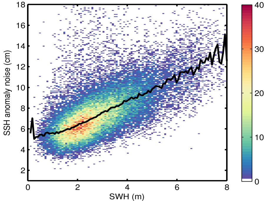
Figure 9. 2D histogram showing flag-valid SSH anomaly noise as a function of SWH for 24/01/2017. The black line denotes the median SSH anomaly noise as a function of SWH.
