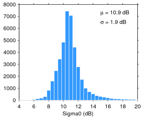
Figure 25. Histogram of flag-valid sigma0 over oceans and lakes for 24/01/2017. The mean ( \mu ) and standard deviation ( \sigma ) are also shown. Note that values outside [4 20] dB are excluded from the histogram for the sake of readability but not from the computation of \mu and \sigma .
