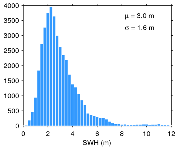
Figure 17. Histogram of flag-valid SWH over oceans and lakes for 24/01/2017. The mean ( \mu ) and standard deviation ( \sigma ) are also shown. Note that values larger than 12 m are excluded from the histogram for the sake of readability but not from the computation of \mu and \sigma .
