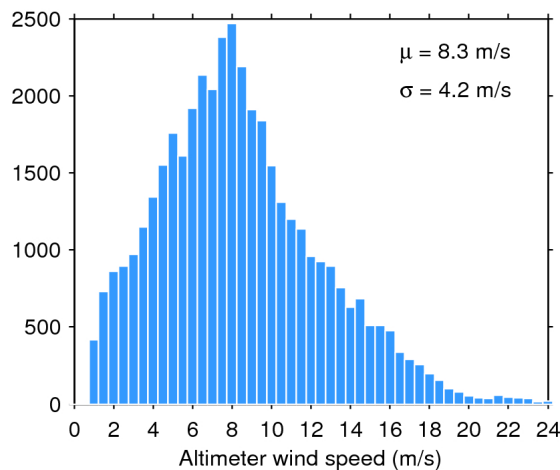
Figure 35. Histogram of science-valid wind over oceans and lakes for 24/01/2017. The mean ( \mu ) and standard deviation ( \sigma ) are also shown. Note that values larger than 24 m/s are excluded from the histogram for the sake of readability but not from the computation of \mu and \sigma .
