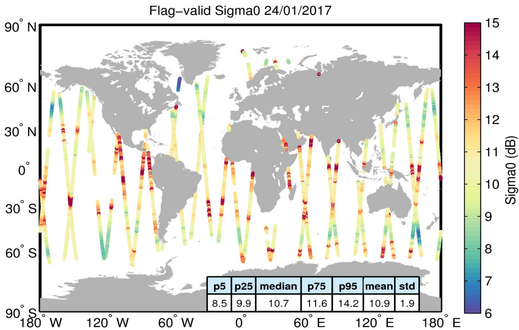
Figure 23. Geographical distribution of flag-valid sigma0 data over oceans and lakes for 24/01/2017. The statistical values shown in the table refer to the sigma0 in dB and are calculated over all measurements shown in the figure.
