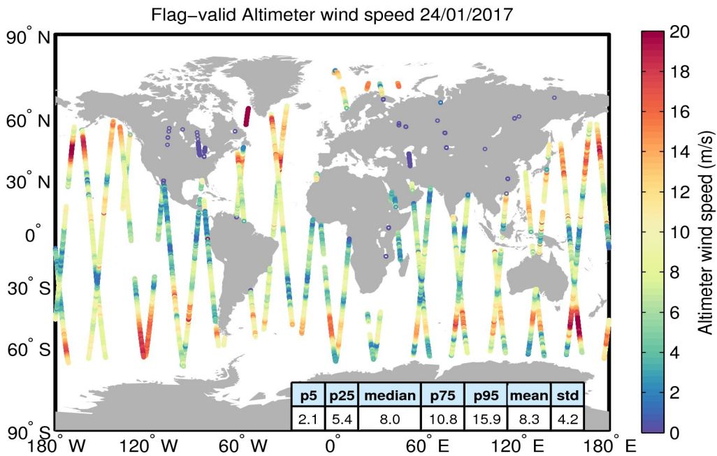
Figure 31. Geographical distribution of flag-valid wind data over oceans and lakes for 24/01/2017. The statistical values shown in the table refer to the wind in m/s and are calculated over all measurements shown in the figure.
