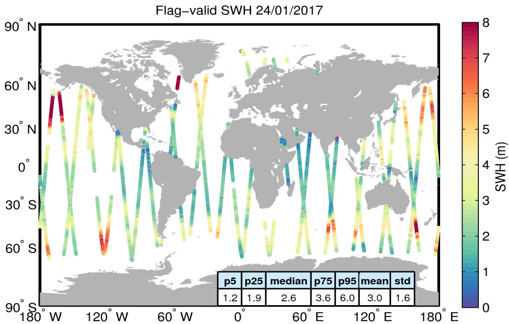
Figure 15. Geographical distribution of flag-valid SWH data over oceans and lakes for 24/01/2017. The statistical values shown in the table refer to the SWH in m and are calculated over all measurements shown in the figure.
