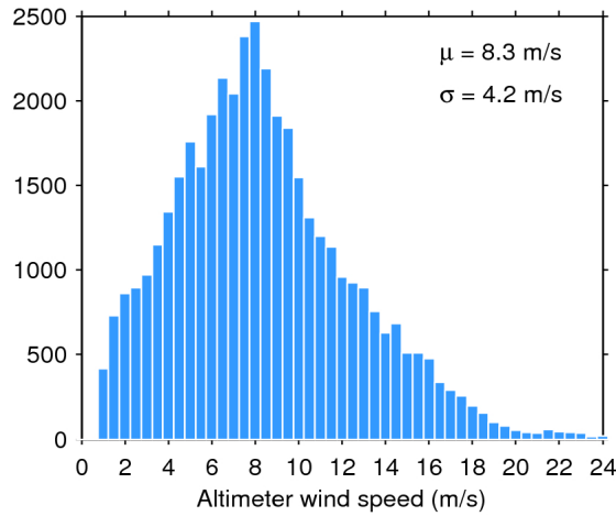
Figure 33. Histogram of flag-valid wind over oceans and lakes for 24/01/2017. The mean ( \mu ) and standard deviation ( \sigma ) are also shown. Note that values larger than 24 m/s are excluded from the histogram for the sake of readability but not from the computation of \mu and \sigma .
