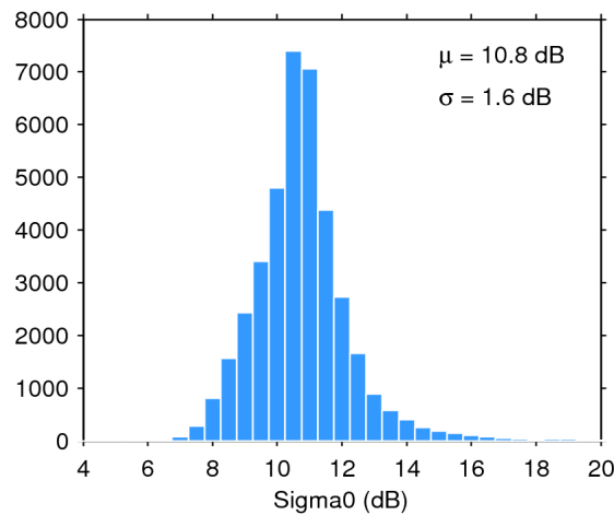
Figure 28. Histogram of science-valid sigma0 over oceans and lakes for 24/01/2017. The mean ( \mu ) and standard deviation ( \sigma ) are also shown. Note that values outside [4 20] dB are excluded from the histogram for the sake of readability but not from the computation of \mu and \sigma .
