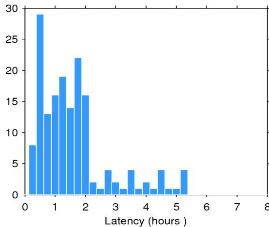
Figure 2. Histogram of the data latency for 24/01/2017. The y-axis denotes the number of files that are made available with a delay of x-hours with respect to the mean time of the records stored in the file.
