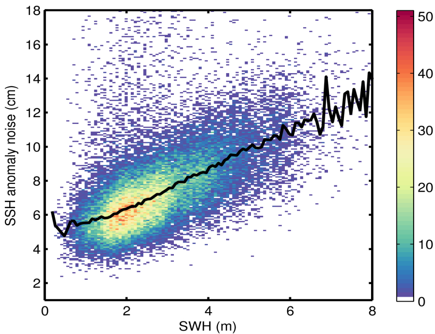
Figure 9. 2D histogram showing flag-valid SSH anomaly noise as a function of SWH for 23/01/2017. The black line denotes the median SSH anomaly noise as a function of SWH.
