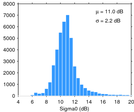
Figure 25. Histogram of flag-valid sigma0 over oceans and lakes for 23/01/2017. The mean ( \mu ) and standard deviation ( \sigma ) are also shown. Note that values outside [4 20] dB are excluded from the histogram for the sake of readability but not from the computation of \mu and \sigma .
