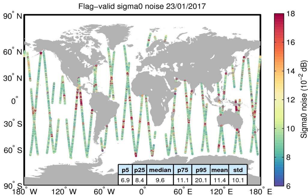
Figure 26. Geographical distribution of flag-valid 20-Hz sigma0 measurement noise over oceans and lakes for 23/01/2017. The statistical values shown in the table refer to the sigma0 noise and are calculated over all measurements shown in the figure.
