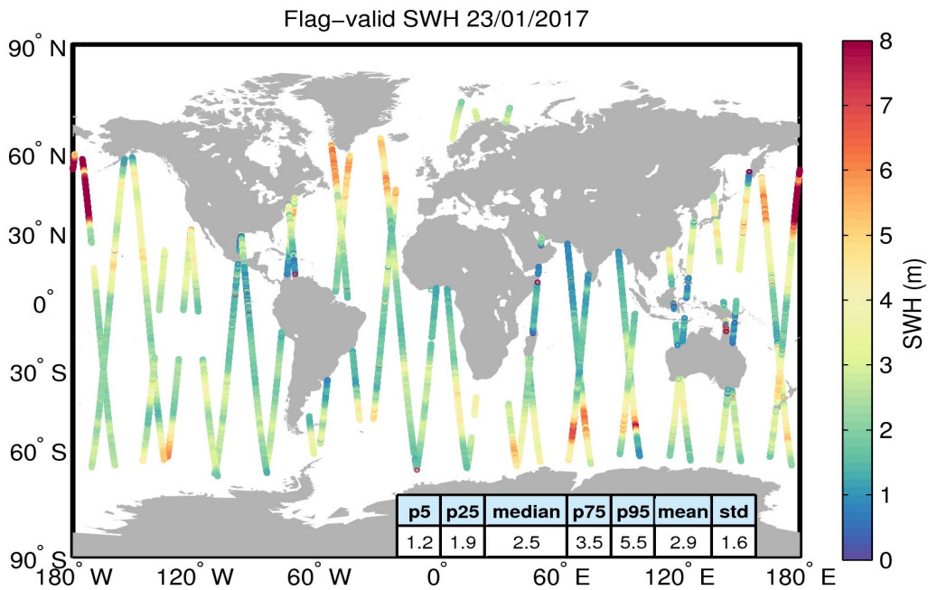
Figure 15. Geographical distribution of flag-valid SWH data over oceans and lakes for 23/01/2017. The statistical values shown in the table refer to the SWH in m and are calculated over all measurements shown in the figure.
