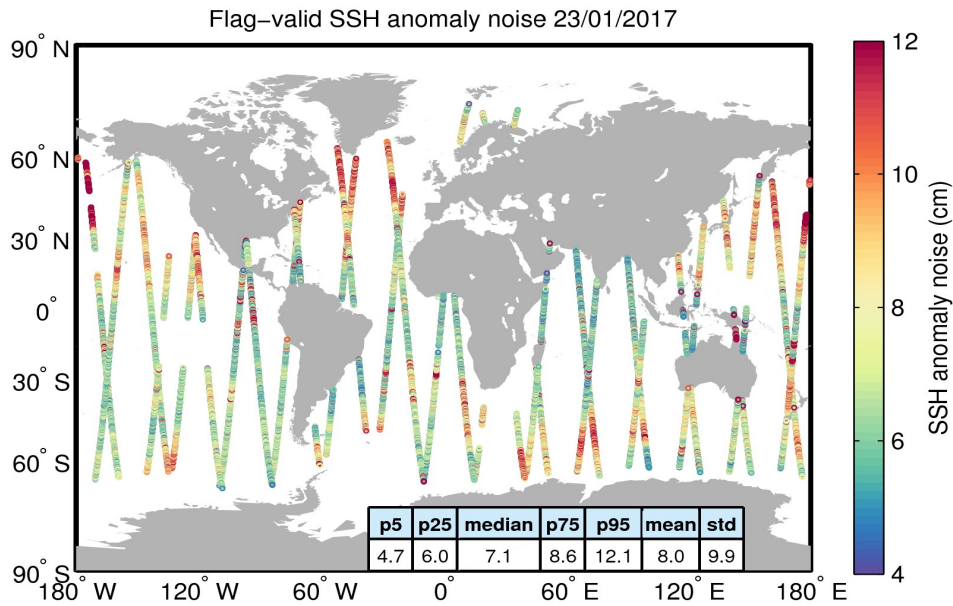
Figure 8. Geographical distribution of flag-valid 20-Hz SSH anomaly measurement noise over oceans and lakes for 23/01/2017. The statistical values shown in the table refer to the SSH anomaly noise and are calculated over all measurements shown in the figure.
