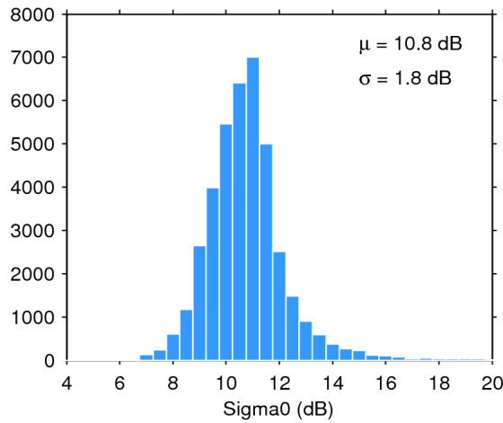
Figure 28. Histogram of science-valid sigma0 over oceans and lakes for 23/01/2017. The mean ( \mu ) and standard deviation ( \sigma ) are also shown. Note that values outside [4 20] dB are excluded from the histogram for the sake of readability but not from the computation of \mu and \sigma .
