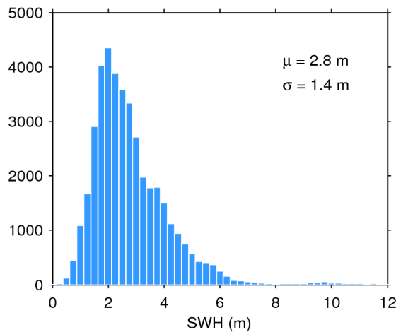
Figure 20. Histogram of science-valid SWH over oceans and lakes for 23/01/2017. The mean ( \mu ) and standard deviation ( \sigma ) are also shown. Note that values larger than 12 m are excluded from the histogram for the sake of readability but not from the computation of \mu and \sigma .
