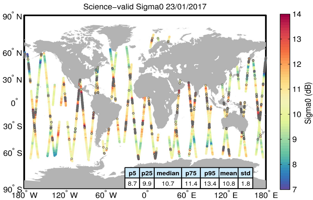
Figure 27. Geographical distribution of science-valid sigma0 data over oceans and lakes for 23/01/2017. The statistical values shown in the table refer to the sigma0 in dB and are calculated over all measurements shown in the figure. Gray circles denote records that have been rejected based on the editing criteria described in Table 4.
