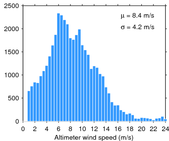
Figure 35. Histogram of science-valid wind over oceans and lakes for 23/01/2017. The mean ( \mu ) and standard deviation ( \sigma ) are also shown. Note that values larger than 24 m/s are excluded from the histogram for the sake of readability but not from the computation of \mu and \sigma .
