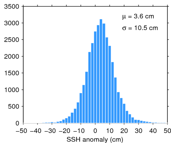
Figure 11. Histogram of science-valid SSH anomaly over oceans and lakes for 23/01/2017. The mean ( \mu ) and standard deviation ( \sigma ) are also shown. Note that values outside [-50 50] cm are excluded from the histogram for the sake of readability but not from the computation of \mu and \sigma .
