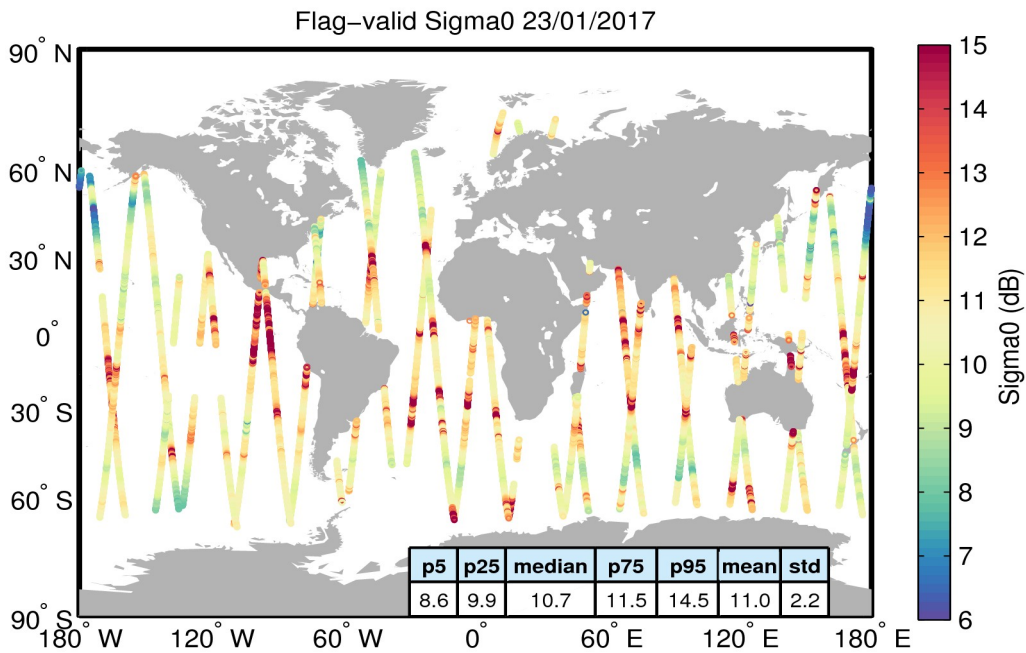
Figure 23. Geographical distribution of flag-valid sigma0 data over oceans and lakes for 23/01/2017. The statistical values shown in the table refer to the sigma0 in dB and are calculated over all measurements shown in the figure.
