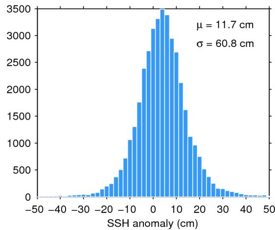
Figure 7. Histogram of flag-valid SSH anomaly over oceans and lakes for 23/01/2017. The mean ( \mu ) and standard deviation ( \sigma ) are also shown. Note that values outside [-50 50] cm are excluded from the histogram for the sake of readability but not from the computation of \mu and \sigma .
