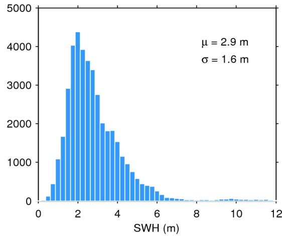
Figure 17. Histogram of flag-valid SWH over oceans and lakes for 23/01/2017. The mean ( \mu ) and standard deviation ( \sigma ) are also shown. Note that values larger than 12 m are excluded from the histogram for the sake of readability but not from the computation of \mu and \sigma .
