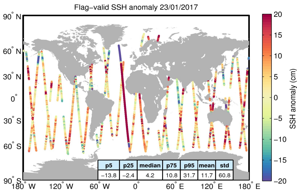
Figure 5. Geographical distribution of flag-valid 1-Hz SSH anomaly data over oceans and lakes for 23/01/2017. The statistical values shown in the table refer to the SSH anomaly in cm and are calculated over all measurements shown in the figure.
