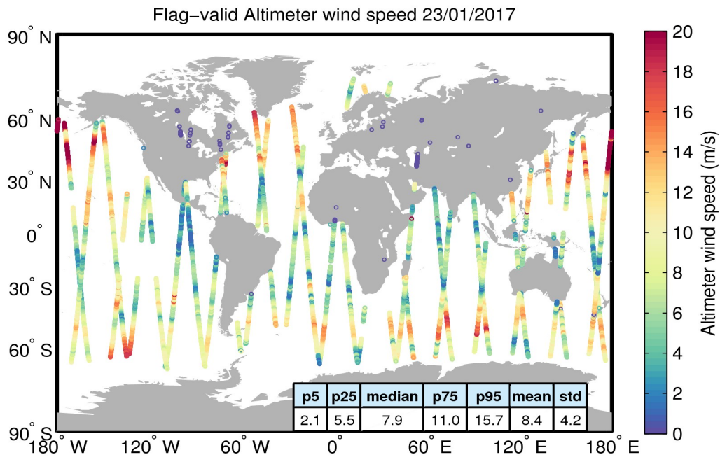
Figure 31. Geographical distribution of flag-valid wind data over oceans and lakes for 23/01/2017. The statistical values shown in the table refer to the wind in m/s and are calculated over all measurements shown in the figure.
