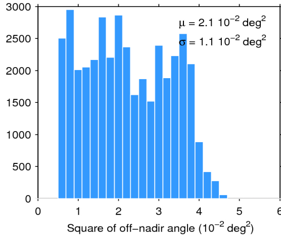
Figure 39. Histogram of flag-valid mispointing over oceans and lakes for 23/01/2017. The mean ( \mu ) and standard deviation ( \sigma ) are also shown. Note that values larger than 6 \cdot 10^{-2} \text{ deg}^2 are excluded from the histogram for the sake of readability but not from the computation of \mu and \sigma .
