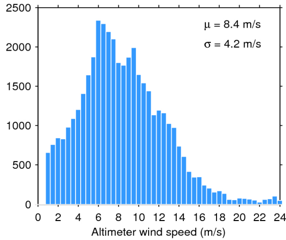
Figure 33. Histogram of flag-valid wind over oceans and lakes for 23/01/2017. The mean ( \mu ) and standard deviation ( \sigma ) are also shown. Note that values larger than 24 m/s are excluded from the histogram for the sake of readability but not from the computation of \mu and \sigma .
