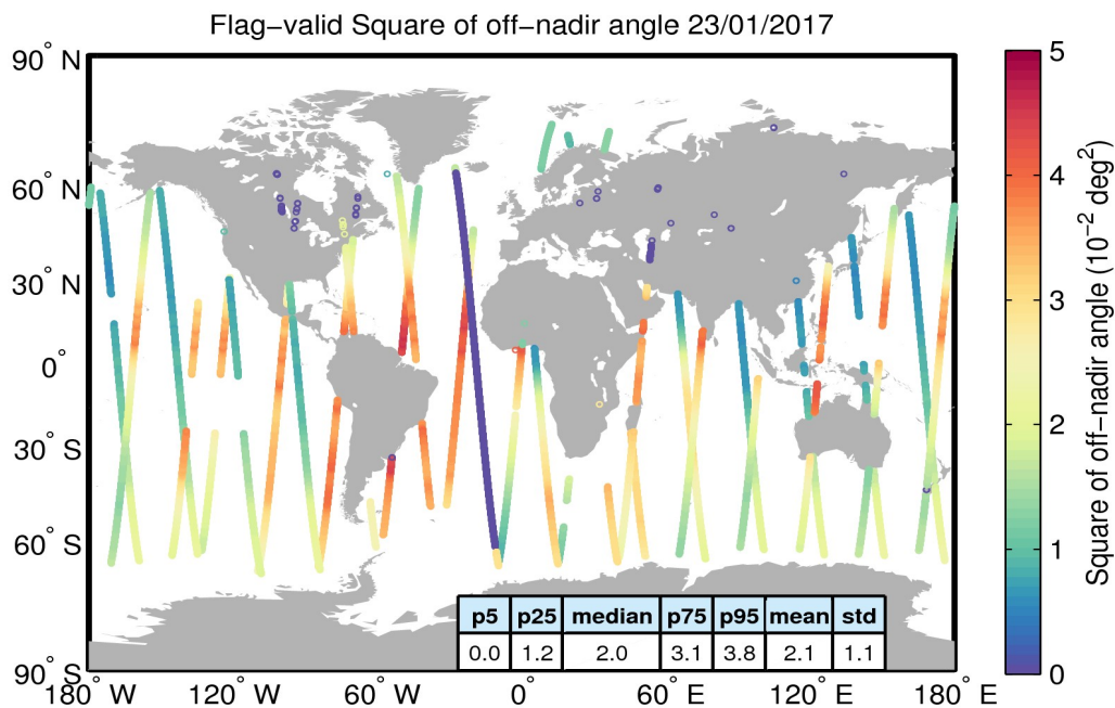
Figure 37. Geographical distribution of flag-valid mispointing data over oceans and lakes for 23/01/2017. The statistical values shown in the table refer to the mispointing in 10^{-2} deg 2 and are calculated over all measurements shown in the figure.
