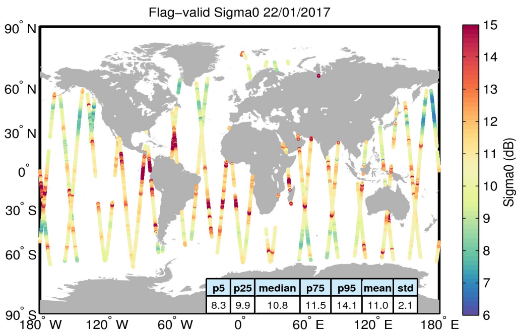
Figure 23. Geographical distribution of flag-valid sigma0 data over oceans and lakes for 22/01/2017. The statistical values shown in the table refer to the sigma0 in dB and are calculated over all measurements shown in the figure.
