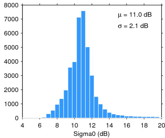
Figure 25. Histogram of flag-valid sigma0 over oceans and lakes for 22/01/2017. The mean ( \mu ) and standard deviation ( \sigma ) are also shown. Note that values outside [4 20] dB are excluded from the histogram for the sake of readability but not from the computation of \mu and \sigma .
