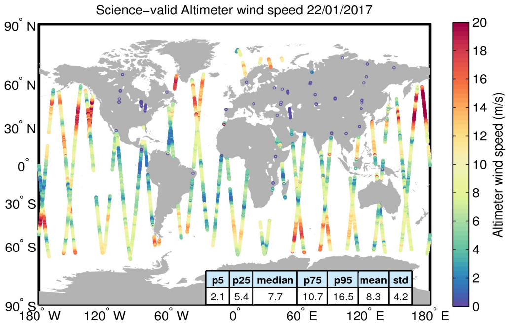
Figure 34. Geographical distribution of science-valid wind data over oceans and lakes for 22/01/2017. The statistical values shown in the table refer to the wind in m/s and are calculated over all measurements shown in the figure. Gray circles denote records that have been rejected based on the editing criteria described in Table 5.
