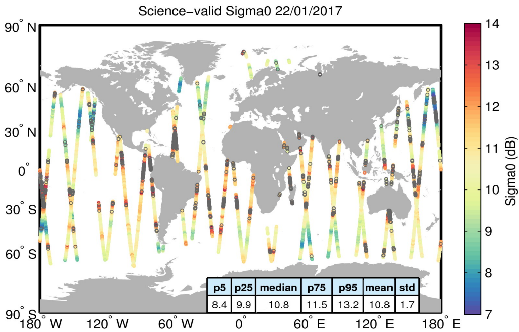
Figure 27. Geographical distribution of science-valid sigma0 data over oceans and lakes for 22/01/2017. The statistical values shown in the table refer to the sigma0 in dB and are calculated over all measurements shown in the figure. Gray circles denote records that have been rejected based on the editing criteria described in Table 4.
