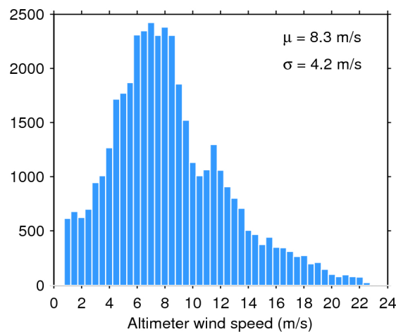
Figure 35. Histogram of science-valid wind over oceans and lakes for 22/01/2017. The mean ( \mu ) and standard deviation ( \sigma ) are also shown. Note that values larger than 24 m/s are excluded from the histogram for the sake of readability but not from the computation of \mu and \sigma .
