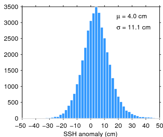
Figure 11. Histogram of science-valid SSH anomaly over oceans and lakes for 22/01/2017. The mean ( \mu ) and standard deviation ( \sigma ) are also shown. Note that values outside [-50 50] cm are excluded from the histogram for the sake of readability but not from the computation of \mu and \sigma .
