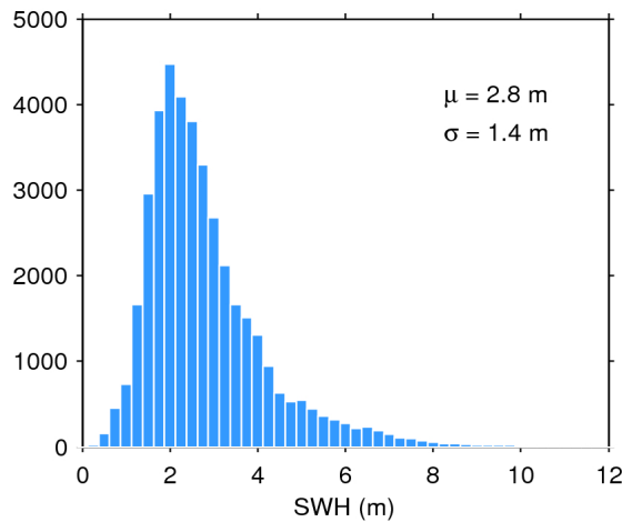
Figure 20. Histogram of science-valid SWH over oceans and lakes for 22/01/2017. The mean ( \mu ) and standard deviation ( \sigma ) are also shown. Note that values larger than 12 m are excluded from the histogram for the sake of readability but not from the computation of \mu and \sigma .
