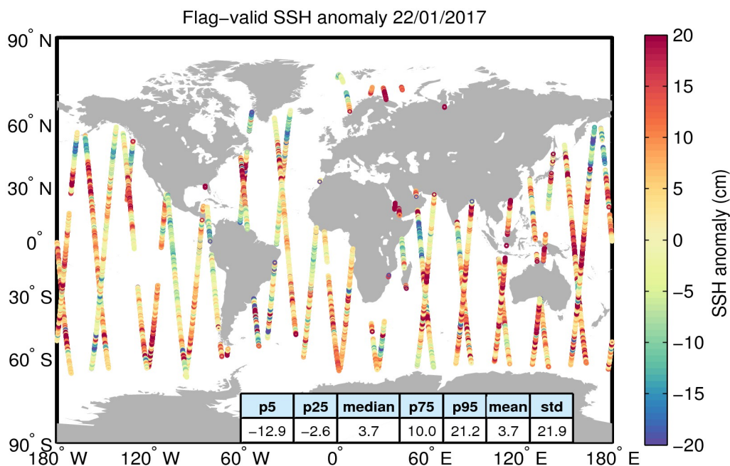
Figure 5. Geographical distribution of flag-valid 1-Hz SSH anomaly data over oceans and lakes for 22/01/2017. The statistical values shown in the table refer to the SSH anomaly in cm and are calculated over all measurements shown in the figure.
