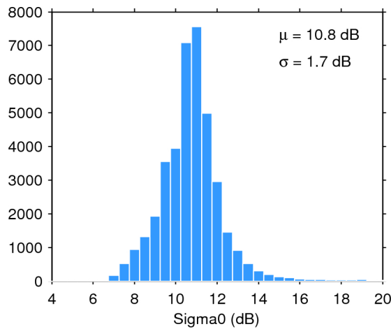
Figure 28. Histogram of science-valid sigma0 over oceans and lakes for 22/01/2017. The mean ( \mu ) and standard deviation ( \sigma ) are also shown. Note that values outside [4 20] dB are excluded from the histogram for the sake of readability but not from the computation of \mu and \sigma .
