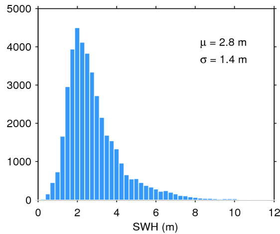
Figure 17. Histogram of flag-valid SWH over oceans and lakes for 22/01/2017. The mean ( \mu ) and standard deviation ( \sigma ) are also shown. Note that values larger than 12 m are excluded from the histogram for the sake of readability but not from the computation of \mu and \sigma .
