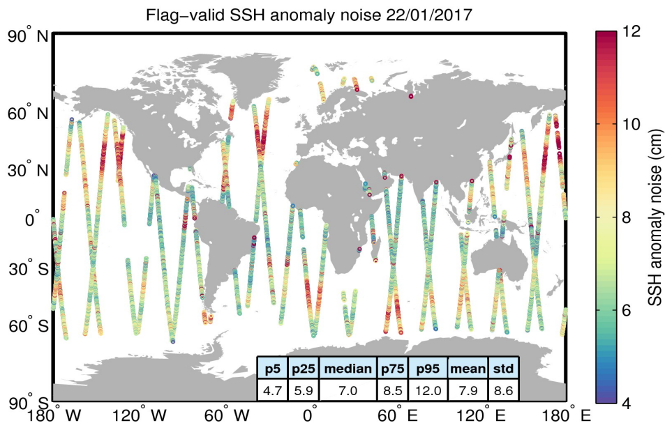
Figure 8. Geographical distribution of flag-valid 20-Hz SSH anomaly measurement noise over oceans and lakes for 22/01/2017. The statistical values shown in the table refer to the SSH anomaly noise and are calculated over all measurements shown in the figure.
