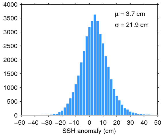
Figure 7. Histogram of flag-valid SSH anomaly over oceans and lakes for 22/01/2017. The mean ( \mu ) and standard deviation ( \sigma ) are also shown. Note that values outside [-50 50] cm are excluded from the histogram for the sake of readability but not from the computation of \mu and \sigma .
