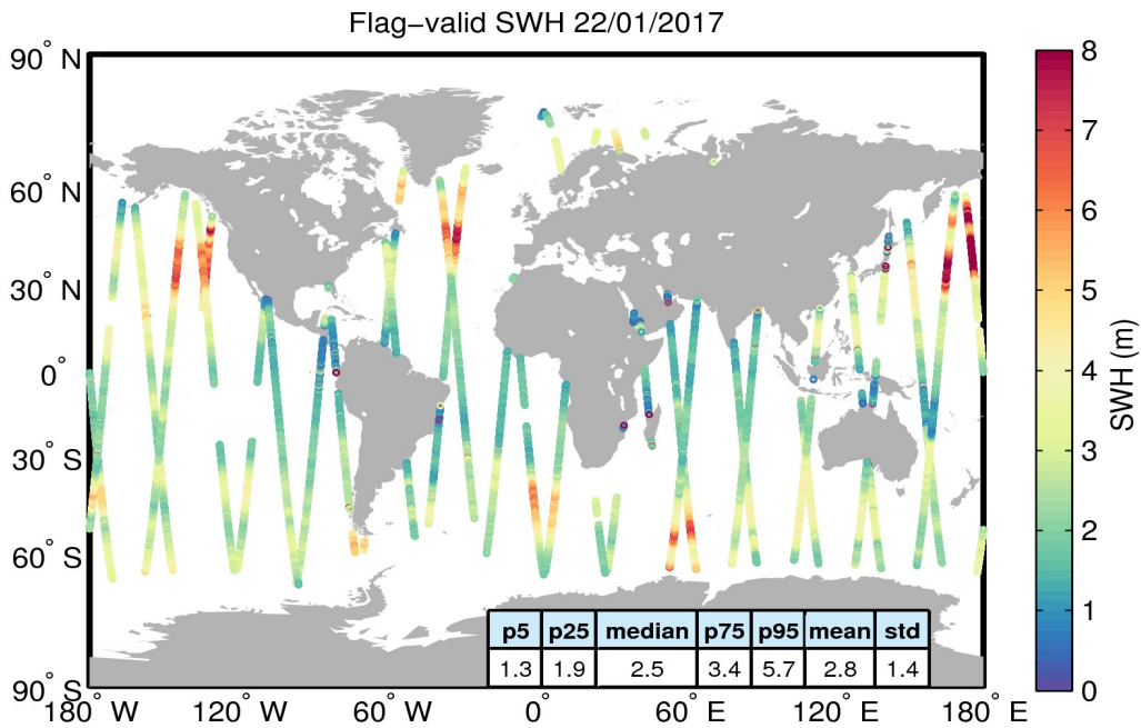
Figure 15. Geographical distribution of flag-valid SWH data over oceans and lakes for 22/01/2017. The statistical values shown in the table refer to the SWH in m and are calculated over all measurements shown in the figure.
