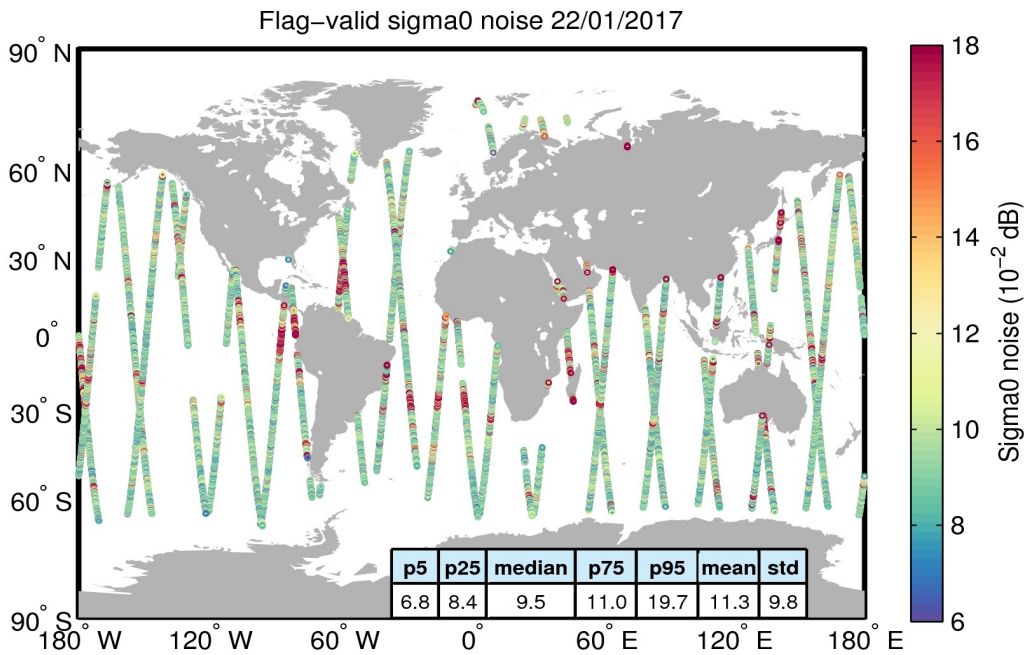
Figure 26. Geographical distribution of flag-valid 20-Hz sigma0 measurement noise over oceans and lakes for 22/01/2017. The statistical values shown in the table refer to the sigma0 noise and are calculated over all measurements shown in the figure.
