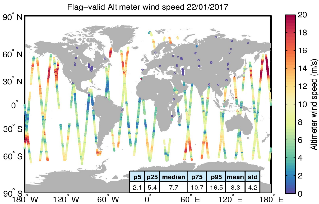
Figure 31. Geographical distribution of flag-valid wind data over oceans and lakes for 22/01/2017. The statistical values shown in the table refer to the wind in m/s and are calculated over all measurements shown in the figure.
