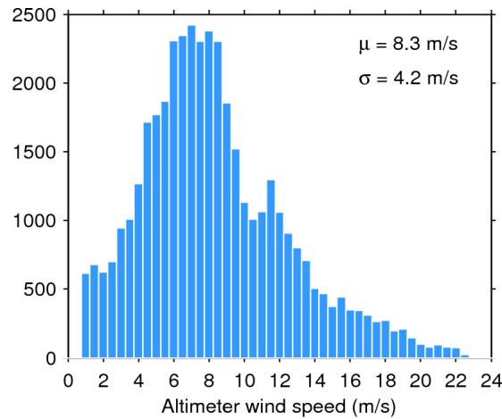
Figure 33. Histogram of flag-valid wind over oceans and lakes for 22/01/2017. The mean ( \mu ) and standard deviation ( \sigma ) are also shown. Note that values larger than 24 m/s are excluded from the histogram for the sake of readability but not from the computation of \mu and \sigma .
