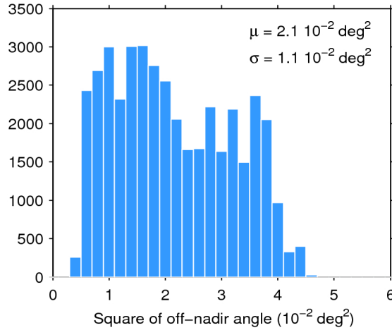
Figure 39. Histogram of flag-valid mispointing over oceans and lakes for 22/01/2017. The mean ( \mu ) and standard deviation ( \sigma ) are also shown. Note that values larger than 6 \cdot 10^{-2} \text{ deg}^2 are excluded from the histogram for the sake of readability but not from the computation of \mu and \sigma .
