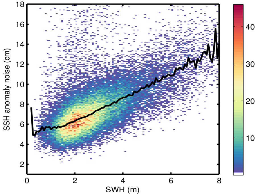
Figure 9. 2D histogram showing flag-valid SSH anomaly noise as a function of SWH for 22/01/2017. The black line denotes the median SSH anomaly noise as a function of SWH.
