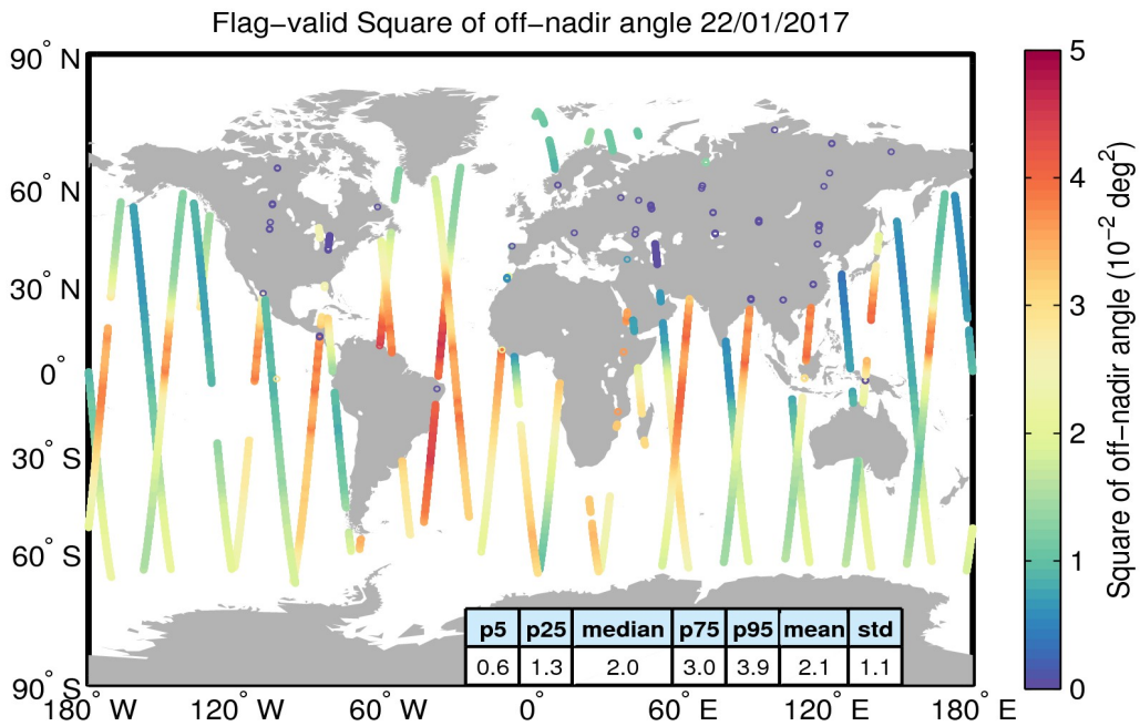
Figure 37. Geographical distribution of flag-valid mispointing data over oceans and lakes for 22/01/2017. The statistical values shown in the table refer to the mispointing in 10^{-2} deg 2 and are calculated over all measurements shown in the figure.
