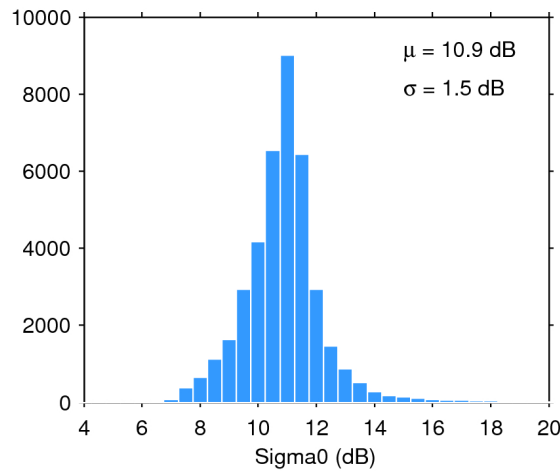
Figure 28. Histogram of science-valid sigma0 over oceans and lakes for 21/01/2017. The mean ( \mu ) and standard deviation ( \sigma ) are also shown. Note that values outside [4 20] dB are excluded from the histogram for the sake of readability but not from the computation of \mu and \sigma .
