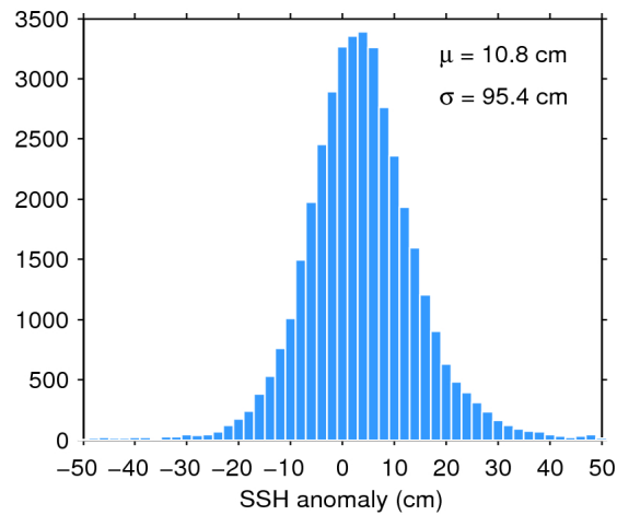
Figure 7. Histogram of flag-valid SSH anomaly over oceans and lakes for 21/01/2017. The mean ( \mu ) and standard deviation ( \sigma ) are also shown. Note that values outside [-50 50] cm are excluded from the histogram for the sake of readability but not from the computation of \mu and \sigma .
