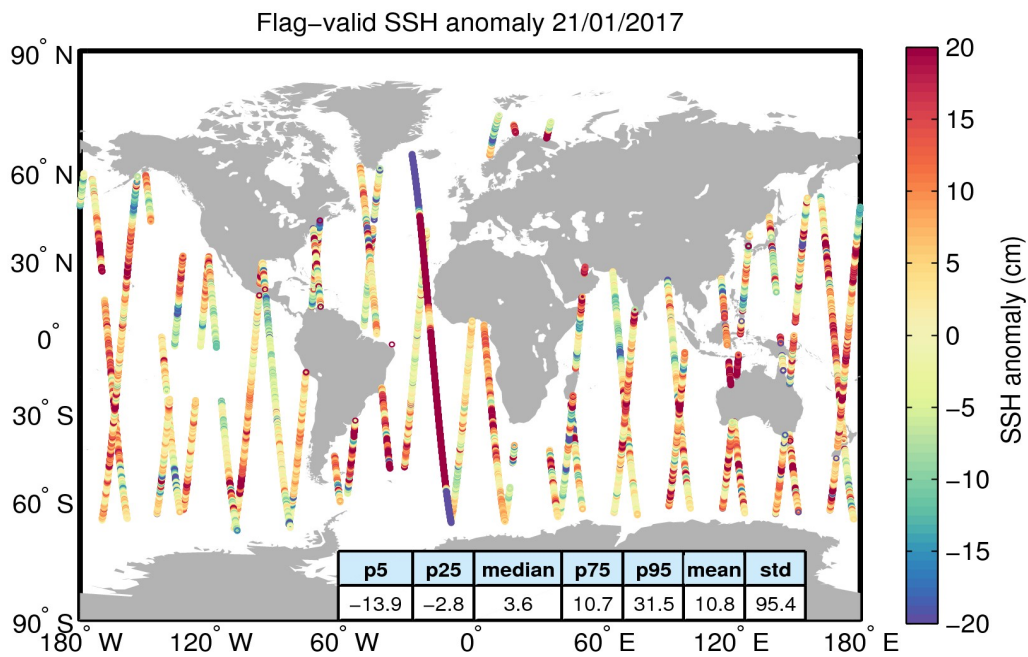
Figure 5. Geographical distribution of flag-valid 1-Hz SSH anomaly data over oceans and lakes for 21/01/2017. The statistical values shown in the table refer to the SSH anomaly in cm and are calculated over all measurements shown in the figure.
