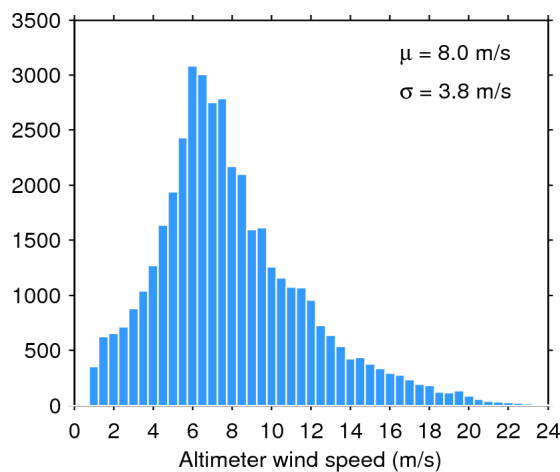
Figure 35. Histogram of science-valid wind over oceans and lakes for 21/01/2017. The mean ( \mu ) and standard deviation ( \sigma ) are also shown. Note that values larger than 24 m/s are excluded from the histogram for the sake of readability but not from the computation of \mu and \sigma .
