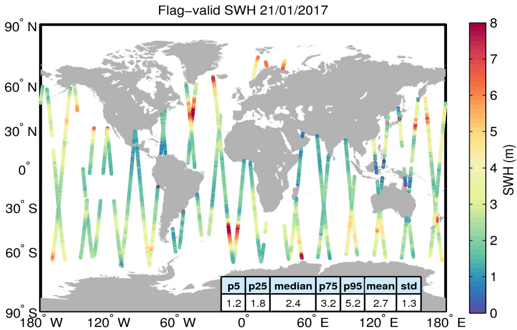
Figure 15. Geographical distribution of flag-valid SWH data over oceans and lakes for 21/01/2017. The statistical values shown in the table refer to the SWH in m and are calculated over all measurements shown in the figure.
