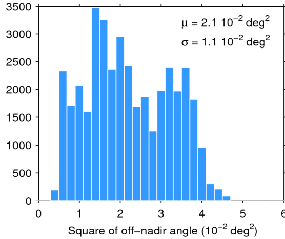
Figure 39. Histogram of flag-valid mispointing over oceans and lakes for 21/01/2017. The mean ( \mu ) and standard deviation ( \sigma ) are also shown. Note that values larger than 6 \cdot 10^{-2} \text{ deg}^2 are excluded from the histogram for the sake of readability but not from the computation of \mu and \sigma .
