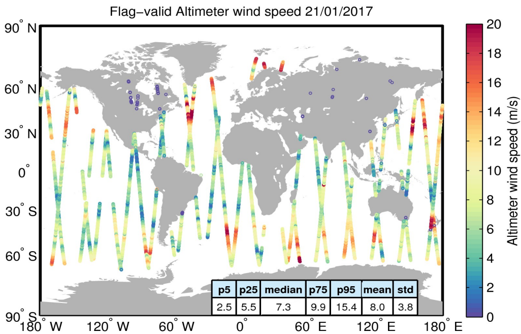
Figure 31. Geographical distribution of flag-valid wind data over oceans and lakes for 21/01/2017. The statistical values shown in the table refer to the wind in m/s and are calculated over all measurements shown in the figure.
