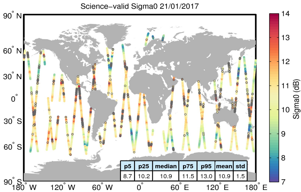
Figure 27. Geographical distribution of science-valid sigma0 data over oceans and lakes for 21/01/2017. The statistical values shown in the table refer to the sigma0 in dB and are calculated over all measurements shown in the figure. Gray circles denote records that have been rejected based on the editing criteria described in Table 4.
