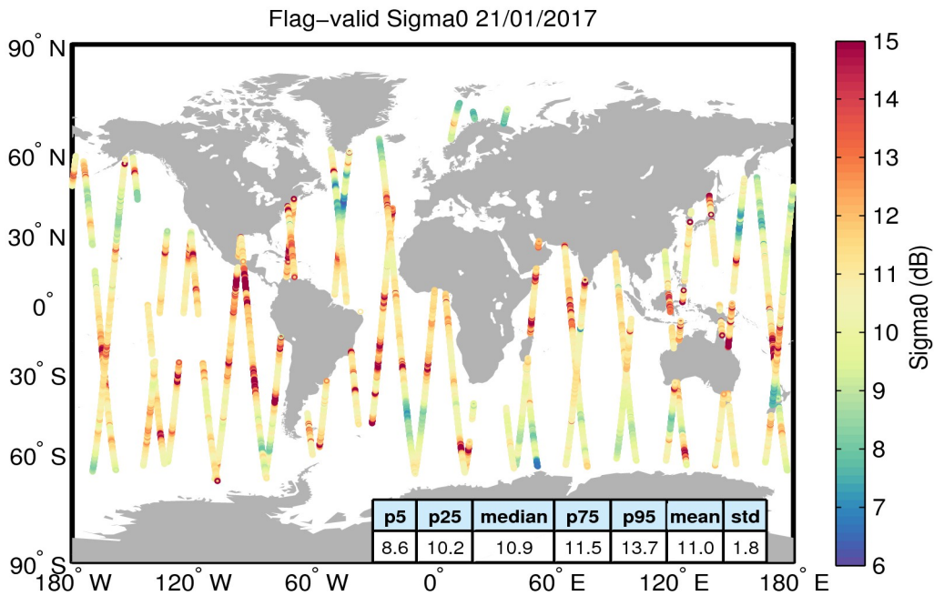
Figure 23. Geographical distribution of flag-valid sigma0 data over oceans and lakes for 21/01/2017. The statistical values shown in the table refer to the sigma0 in dB and are calculated over all measurements shown in the figure.
