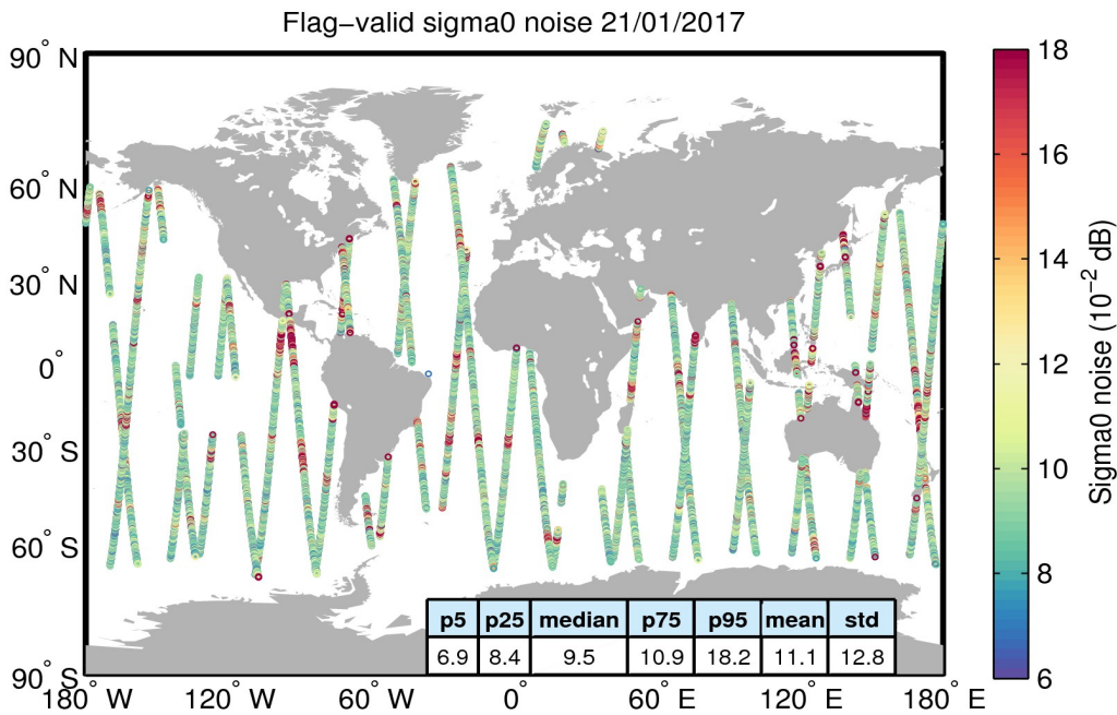
Figure 26. Geographical distribution of flag-valid 20-Hz sigma0 measurement noise over oceans and lakes for 21/01/2017. The statistical values shown in the table refer to the sigma0 noise and are calculated over all measurements shown in the figure.
