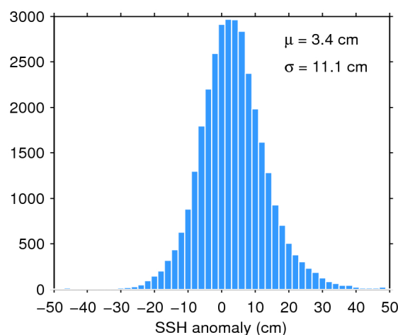
Figure 11. Histogram of science-valid SSH anomaly over oceans and lakes for 21/01/2017. The mean ( \mu ) and standard deviation ( \sigma ) are also shown. Note that values outside [-50 50] cm are excluded from the histogram for the sake of readability but not from the computation of \mu and \sigma .
