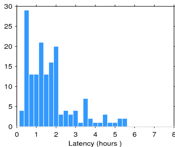
Figure 2. Histogram of the data latency for 21/01/2017. The y-axis denotes the number of files that are made available with a delay of x-hours with respect to the mean time of the records stored in the file.
