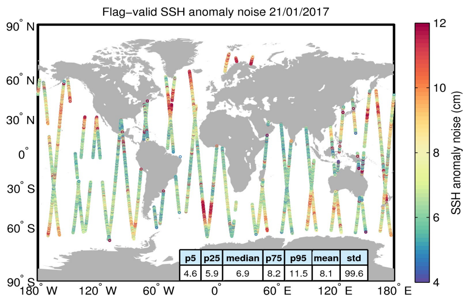
Figure 8. Geographical distribution of flag-valid 20-Hz SSH anomaly measurement noise over oceans and lakes for 21/01/2017. The statistical values shown in the table refer to the SSH anomaly noise and are calculated over all measurements shown in the figure.
