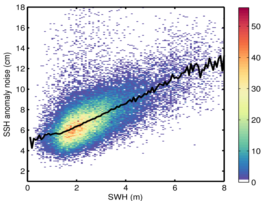
Figure 9. 2D histogram showing flag-valid SSH anomaly noise as a function of SWH for 21/01/2017. The black line denotes the median SSH anomaly noise as a function of SWH.
