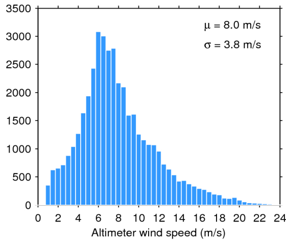
Figure 33. Histogram of flag-valid wind over oceans and lakes for 21/01/2017. The mean ( \mu ) and standard deviation ( \sigma ) are also shown. Note that values larger than 24 m/s are excluded from the histogram for the sake of readability but not from the computation of \mu and \sigma .
