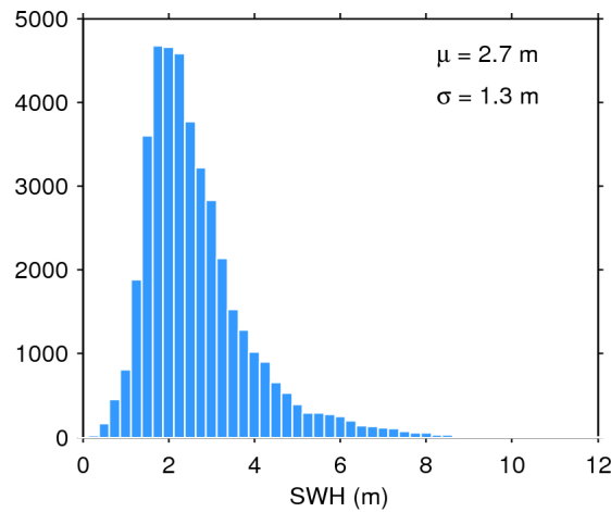
Figure 17. Histogram of flag-valid SWH over oceans and lakes for 21/01/2017. The mean ( \mu ) and standard deviation ( \sigma ) are also shown. Note that values larger than 12 m are excluded from the histogram for the sake of readability but not from the computation of \mu and \sigma .
