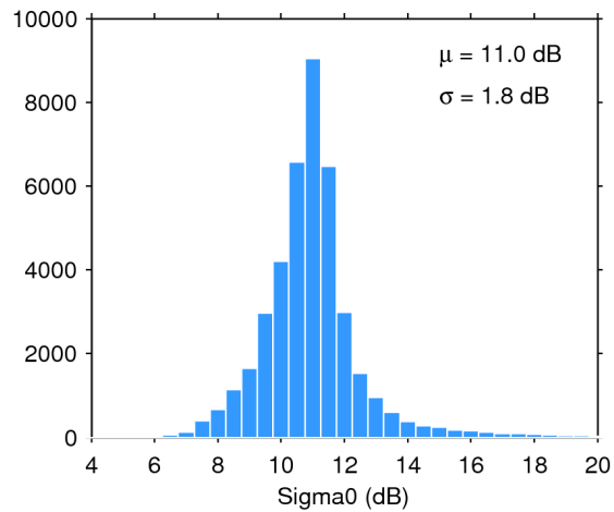
Figure 25. Histogram of flag-valid sigma0 over oceans and lakes for 21/01/2017. The mean ( \mu ) and standard deviation ( \sigma ) are also shown. Note that values outside [4 20] dB are excluded from the histogram for the sake of readability but not from the computation of \mu and \sigma .
