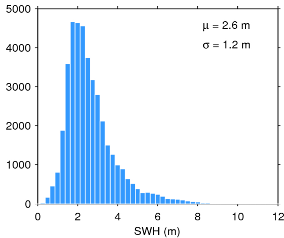
Figure 20. Histogram of science-valid SWH over oceans and lakes for 21/01/2017. The mean ( \mu ) and standard deviation ( \sigma ) are also shown. Note that values larger than 12 m are excluded from the histogram for the sake of readability but not from the computation of \mu and \sigma .
