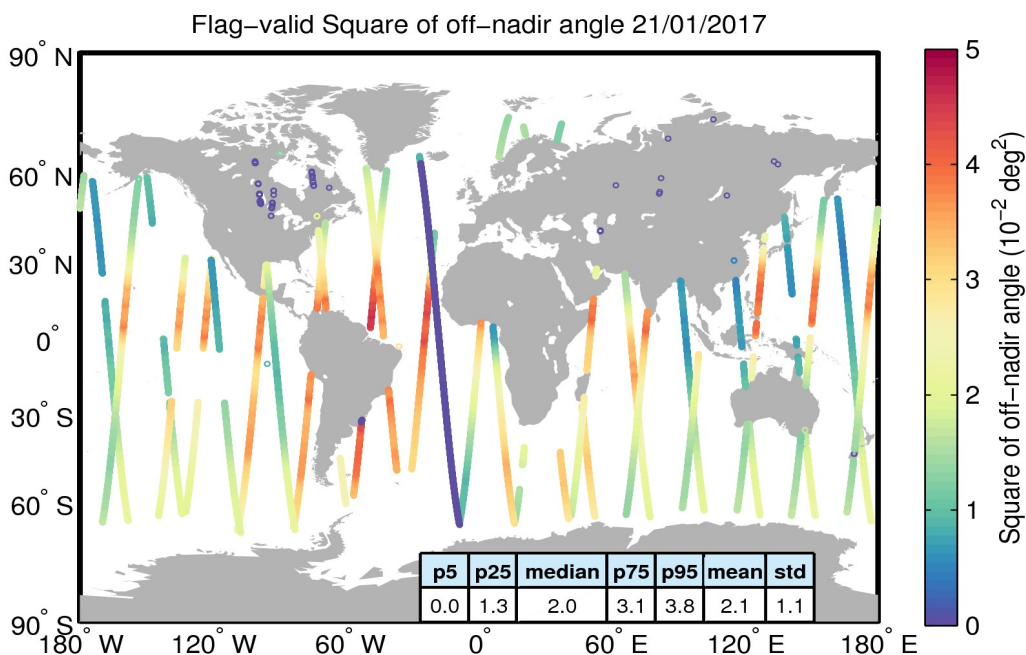
Figure 37. Geographical distribution of flag-valid mispointing data over oceans and lakes for 21/01/2017. The statistical values shown in the table refer to the mispointing in 10^{-2} deg 2 and are calculated over all measurements shown in the figure.
