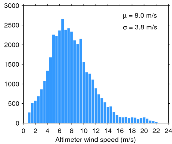
Figure 33. Histogram of flag-valid wind over oceans and lakes for 20/01/2017. The mean ( \mu ) and standard deviation ( \sigma ) are also shown. Note that values larger than 24 m/s are excluded from the histogram for the sake of readability but not from the computation of \mu and \sigma .
