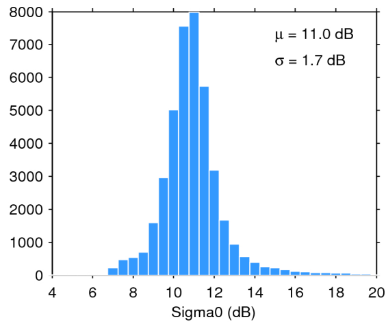
Figure 25. Histogram of flag-valid sigma0 over oceans and lakes for 20/01/2017. The mean ( \mu ) and standard deviation ( \sigma ) are also shown. Note that values outside [4 20] dB are excluded from the histogram for the sake of readability but not from the computation of \mu and \sigma .
