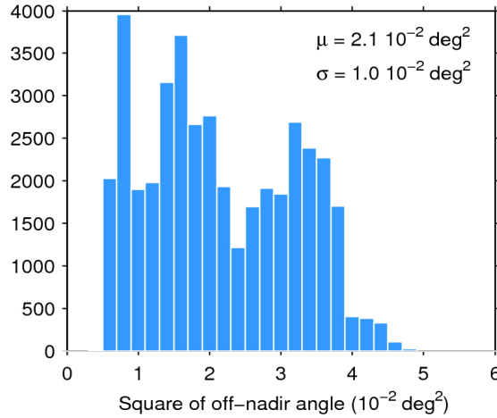
Figure 39. Histogram of flag-valid mispointing over oceans and lakes for 20/01/2017. The mean ( \mu ) and standard deviation ( \sigma ) are also shown. Note that values larger than 6 \cdot 10^{-2} \text{ deg}^2 are excluded from the histogram for the sake of readability but not from the computation of \mu and \sigma .
