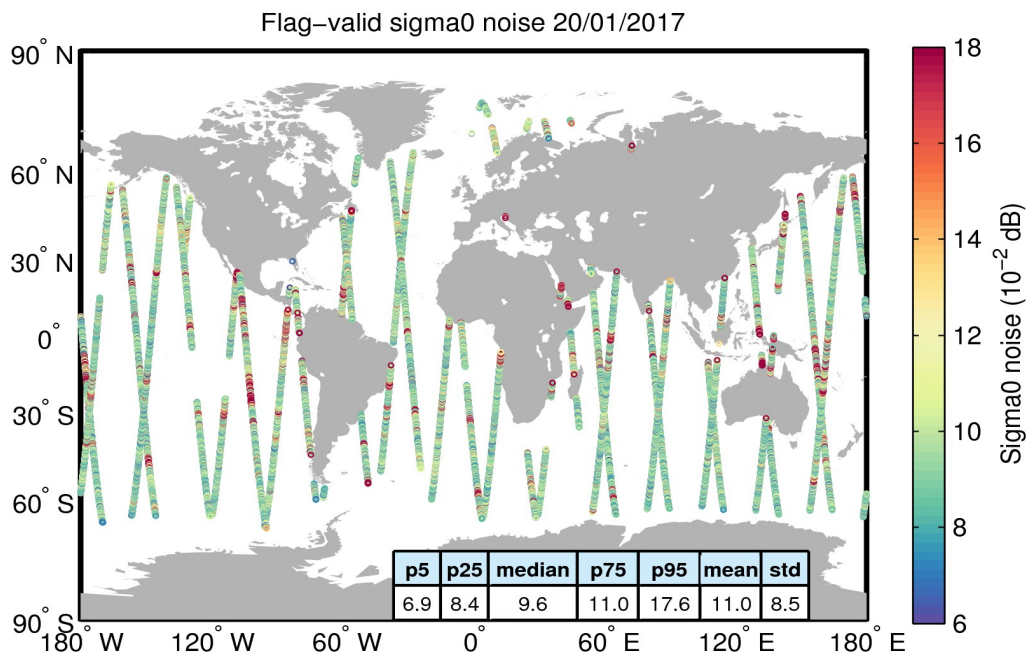
Figure 26. Geographical distribution of flag-valid 20-Hz sigma0 measurement noise over oceans and lakes for 20/01/2017. The statistical values shown in the table refer to the sigma0 noise and are calculated over all measurements shown in the figure.
