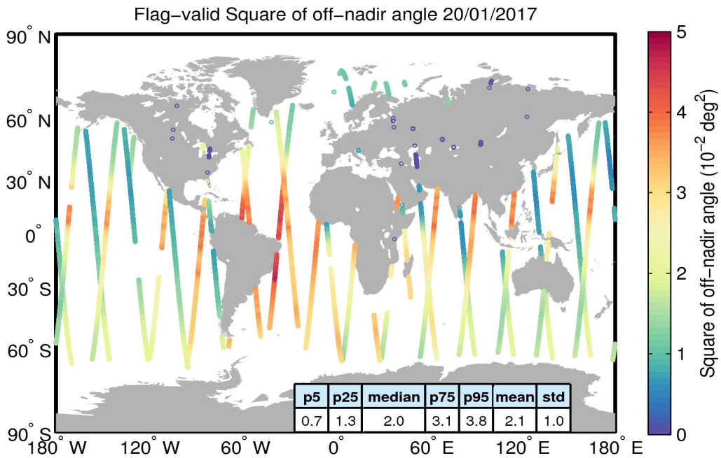
Figure 37. Geographical distribution of flag-valid mispointing data over oceans and lakes for 20/01/2017. The statistical values shown in the table refer to the mispointing in 10^{-2} deg 2 and are calculated over all measurements shown in the figure.
