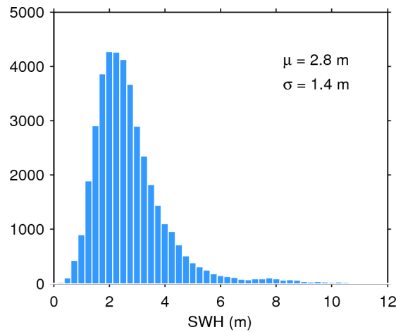
Figure 17. Histogram of flag-valid SWH over oceans and lakes for 20/01/2017. The mean ( \mu ) and standard deviation ( \sigma ) are also shown. Note that values larger than 12 m are excluded from the histogram for the sake of readability but not from the computation of \mu and \sigma .
