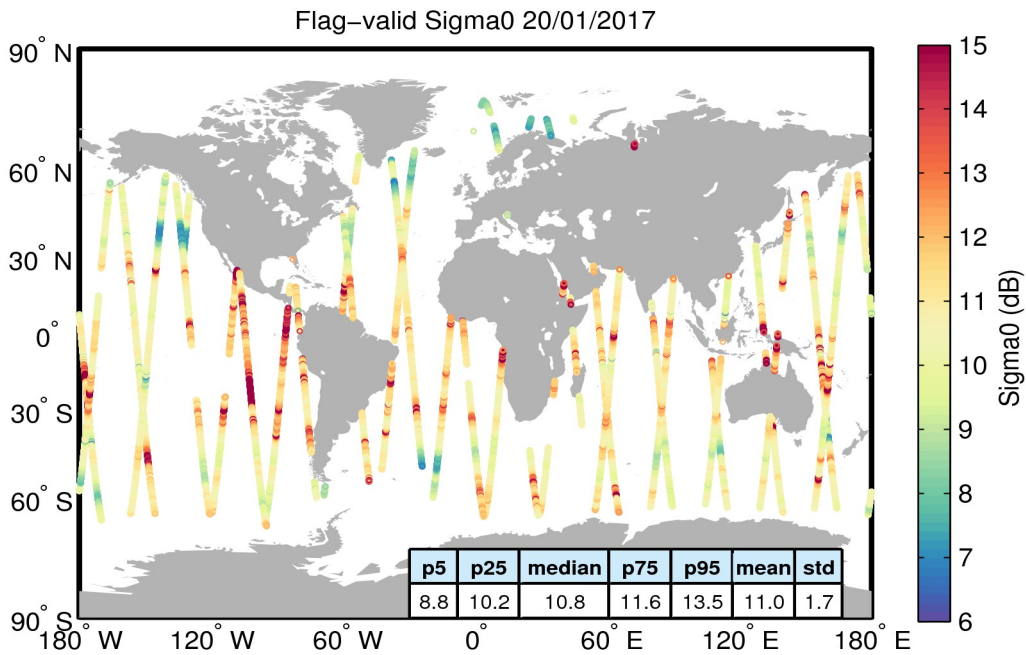
Figure 23. Geographical distribution of flag-valid sigma0 data over oceans and lakes for 20/01/2017. The statistical values shown in the table refer to the sigma0 in dB and are calculated over all measurements shown in the figure.
