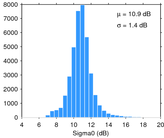
Figure 28. Histogram of science-valid sigma0 over oceans and lakes for 20/01/2017. The mean ( \mu ) and standard deviation ( \sigma ) are also shown. Note that values outside [4 20] dB are excluded from the histogram for the sake of readability but not from the computation of \mu and \sigma .
