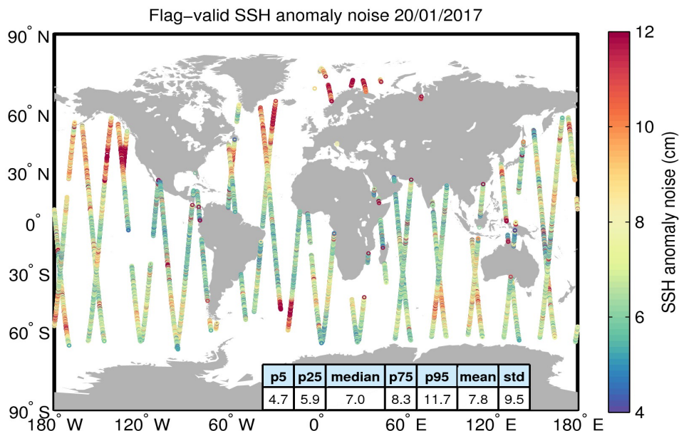
Figure 8. Geographical distribution of flag-valid 20-Hz SSH anomaly measurement noise over oceans and lakes for 20/01/2017. The statistical values shown in the table refer to the SSH anomaly noise and are calculated over all measurements shown in the figure.
