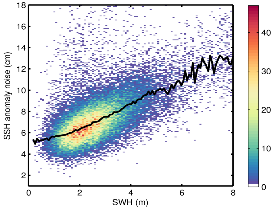
Figure 9. 2D histogram showing flag-valid SSH anomaly noise as a function of SWH for 20/01/2017. The black line denotes the median SSH anomaly noise as a function of SWH.
