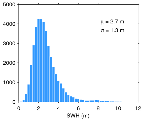
Figure 20. Histogram of science-valid SWH over oceans and lakes for 20/01/2017. The mean ( \mu ) and standard deviation ( \sigma ) are also shown. Note that values larger than 12 m are excluded from the histogram for the sake of readability but not from the computation of \mu and \sigma .
