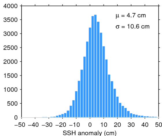
Figure 11. Histogram of science-valid SSH anomaly over oceans and lakes for 20/01/2017. The mean ( \mu ) and standard deviation ( \sigma ) are also shown. Note that values outside [-50 50] cm are excluded from the histogram for the sake of readability but not from the computation of \mu and \sigma .
