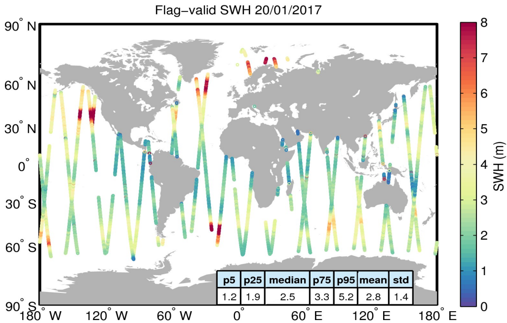
Figure 15. Geographical distribution of flag-valid SWH data over oceans and lakes for 20/01/2017. The statistical values shown in the table refer to the SWH in m and are calculated over all measurements shown in the figure.
