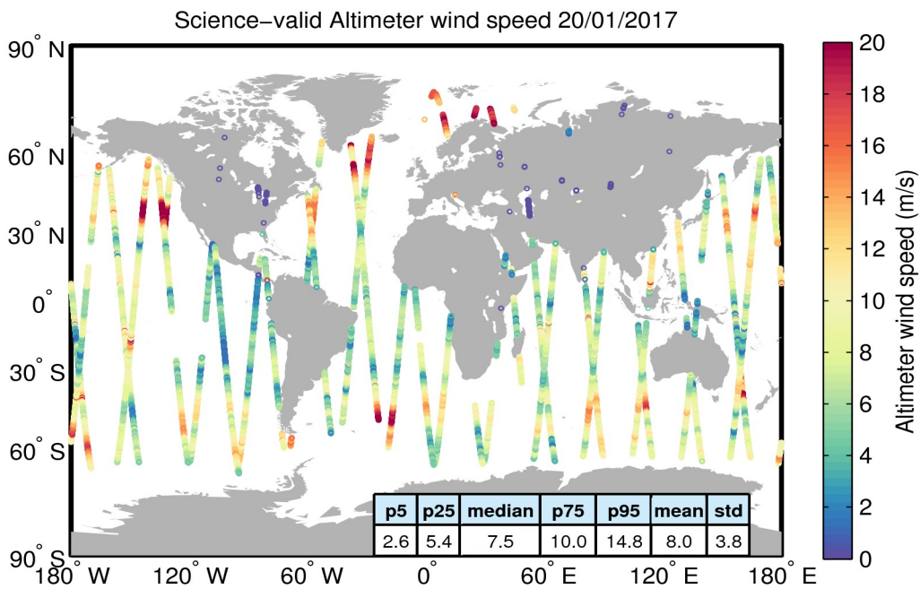
Figure 34. Geographical distribution of science-valid wind data over oceans and lakes for 20/01/2017. The statistical values shown in the table refer to the wind in m/s and are calculated over all measurements shown in the figure. Gray circles denote records that have been rejected based on the editing criteria described in Table 5.
