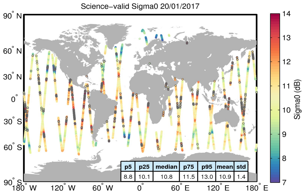
Figure 27. Geographical distribution of science-valid sigma0 data over oceans and lakes for 20/01/2017. The statistical values shown in the table refer to the sigma0 in dB and are calculated over all measurements shown in the figure. Gray circles denote records that have been rejected based on the editing criteria described in Table 4.
