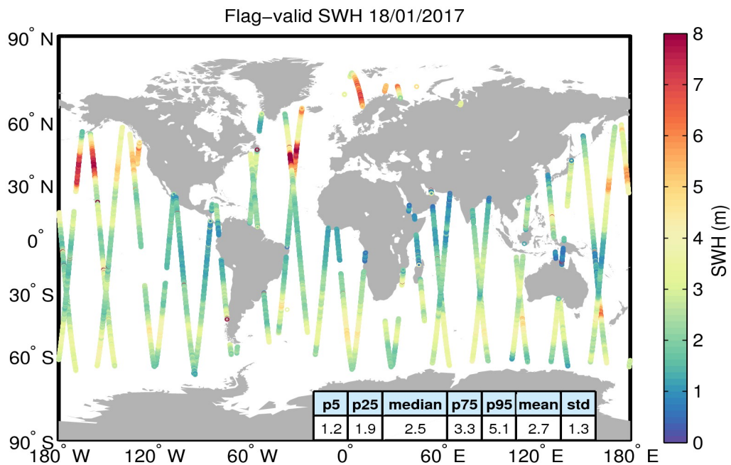
Figure 15. Geographical distribution of flag-valid SWH data over oceans and lakes for 18/01/2017. The statistical values shown in the table refer to the SWH in m and are calculated over all measurements shown in the figure.
