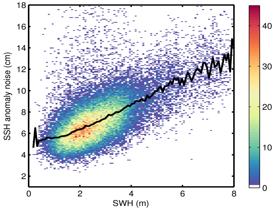
Figure 9. 2D histogram showing flag-valid SSH anomaly noise as a function of SWH for 18/01/2017. The black line denotes the median SSH anomaly noise as a function of SWH.
