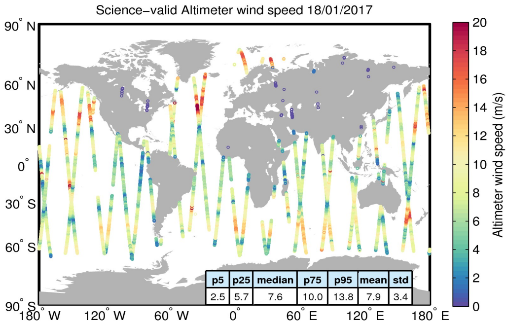
Figure 34. Geographical distribution of science-valid wind data over oceans and lakes for 18/01/2017. The statistical values shown in the table refer to the wind in m/s and are calculated over all measurements shown in the figure. Gray circles denote records that have been rejected based on the editing criteria described in Table 5.
