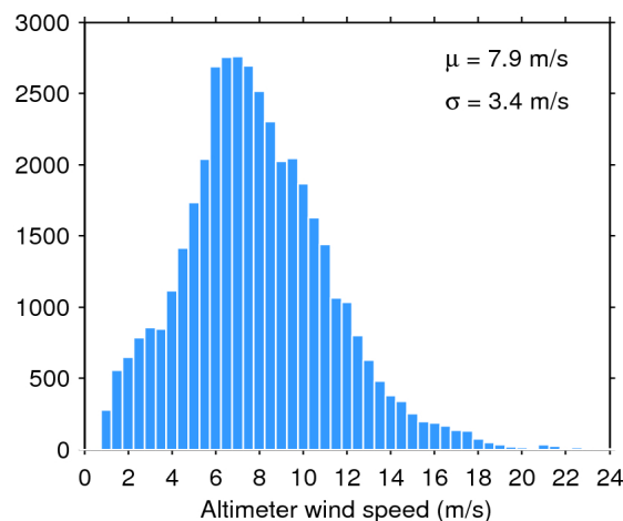
Figure 35. Histogram of science-valid wind over oceans and lakes for 18/01/2017. The mean ( \mu ) and standard deviation ( \sigma ) are also shown. Note that values larger than 24 m/s are excluded from the histogram for the sake of readability but not from the computation of \mu and \sigma .
