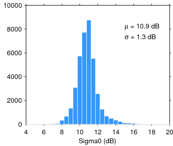
Figure 28. Histogram of science-valid sigma0 over oceans and lakes for 18/01/2017. The mean ( \mu ) and standard deviation ( \sigma ) are also shown. Note that values outside [4 20] dB are excluded from the histogram for the sake of readability but not from the computation of \mu and \sigma .
