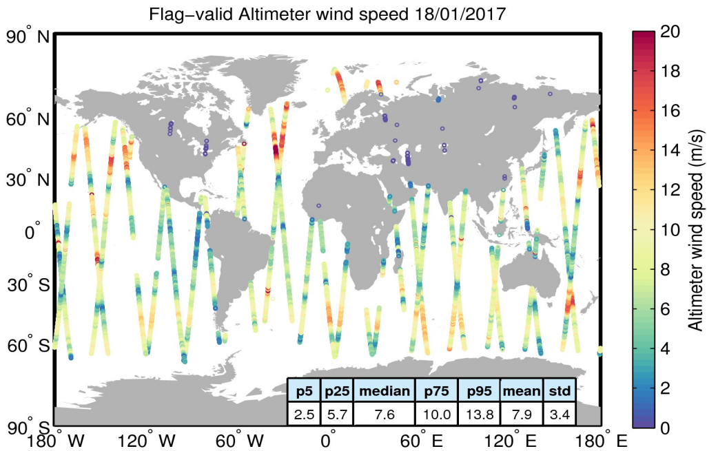
Figure 31. Geographical distribution of flag-valid wind data over oceans and lakes for 18/01/2017. The statistical values shown in the table refer to the wind in m/s and are calculated over all measurements shown in the figure.
