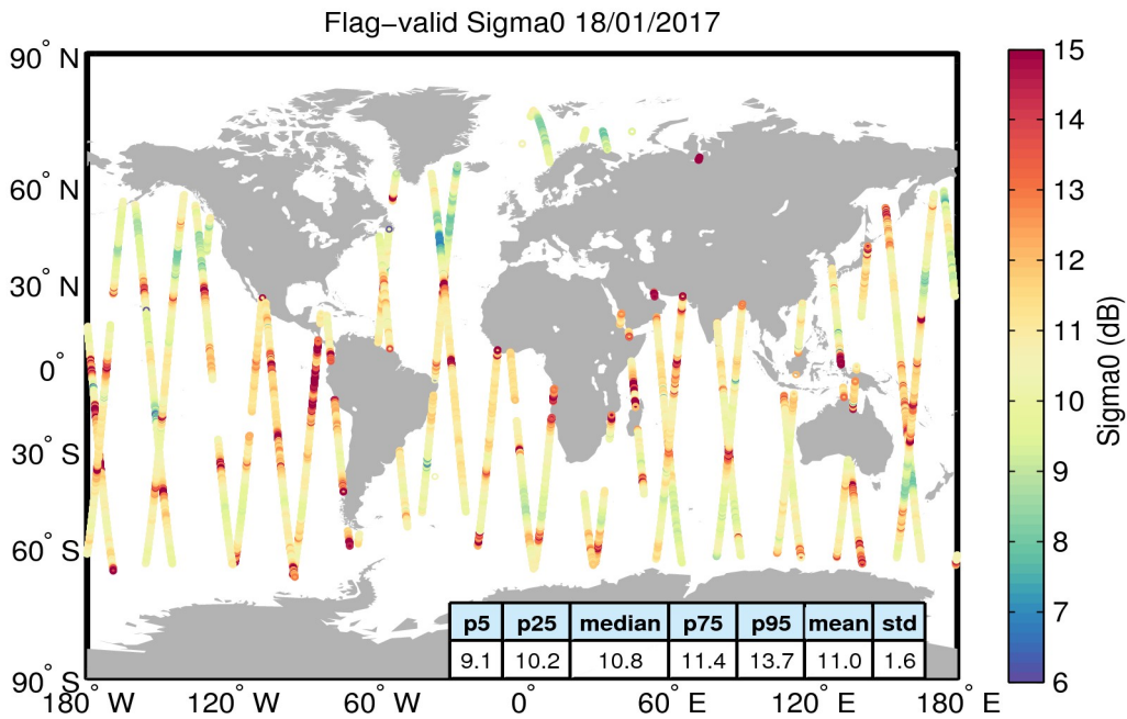
Figure 23. Geographical distribution of flag-valid sigma0 data over oceans and lakes for 18/01/2017. The statistical values shown in the table refer to the sigma0 in dB and are calculated over all measurements shown in the figure.
