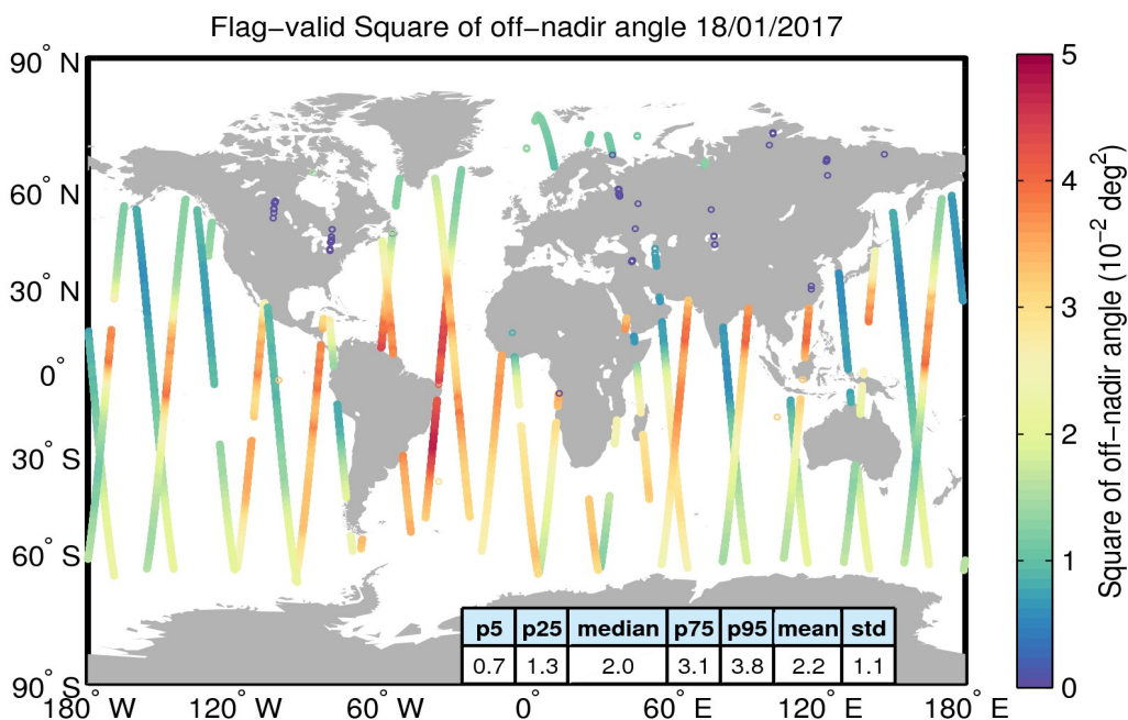
Figure 37. Geographical distribution of flag-valid mispointing data over oceans and lakes for 18/01/2017. The statistical values shown in the table refer to the mispointing in 10^{-2} deg 2 and are calculated over all measurements shown in the figure.
