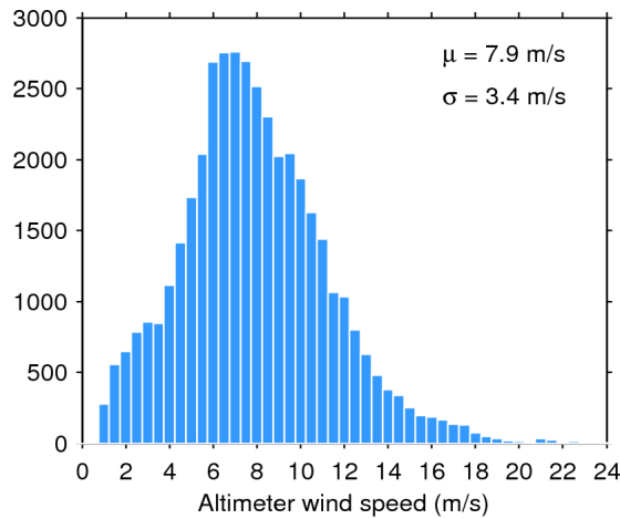
Figure 33. Histogram of flag-valid wind over oceans and lakes for 18/01/2017. The mean ( \mu ) and standard deviation ( \sigma ) are also shown. Note that values larger than 24 m/s are excluded from the histogram for the sake of readability but not from the computation of \mu and \sigma .
