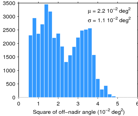
Figure 39. Histogram of flag-valid mispointing over oceans and lakes for 18/01/2017. The mean ( \mu ) and standard deviation ( \sigma ) are also shown. Note that values larger than 6 \cdot 10^{-2} \text{ deg}^2 are excluded from the histogram for the sake of readability but not from the computation of \mu and \sigma .
