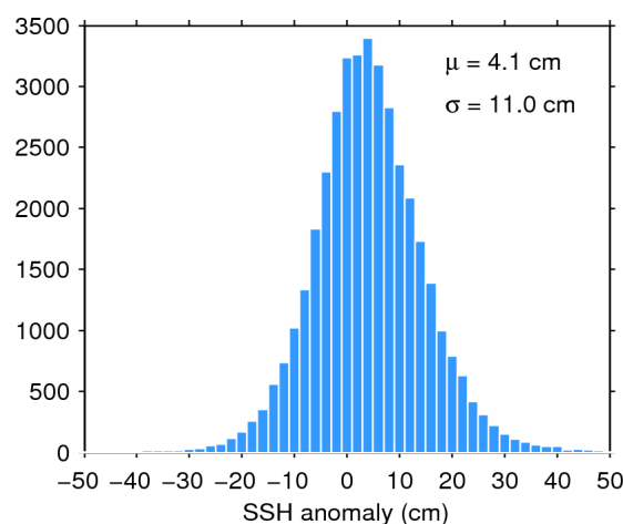
Figure 11. Histogram of science-valid SSH anomaly over oceans and lakes for 18/01/2017. The mean ( \mu ) and standard deviation ( \sigma ) are also shown. Note that values outside [-50 50] cm are excluded from the histogram for the sake of readability but not from the computation of \mu and \sigma .
