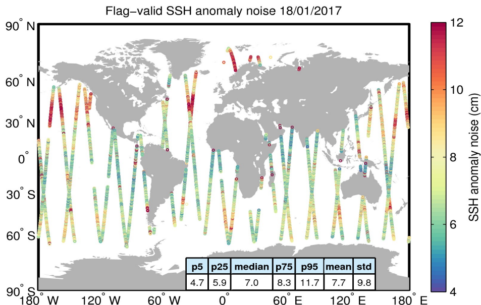
Figure 8. Geographical distribution of flag-valid 20-Hz SSH anomaly measurement noise over oceans and lakes for 18/01/2017. The statistical values shown in the table refer to the SSH anomaly noise and are calculated over all measurements shown in the figure.
