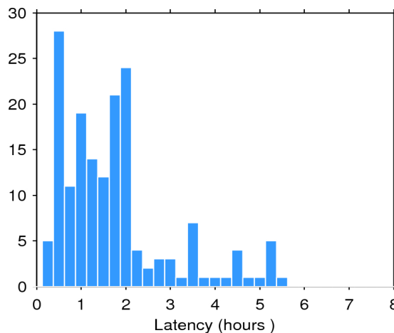
Figure 2. Histogram of the data latency for 18/01/2017. The y-axis denotes the number of files that are made available with a delay of x-hours with respect to the mean time of the records stored in the file.
