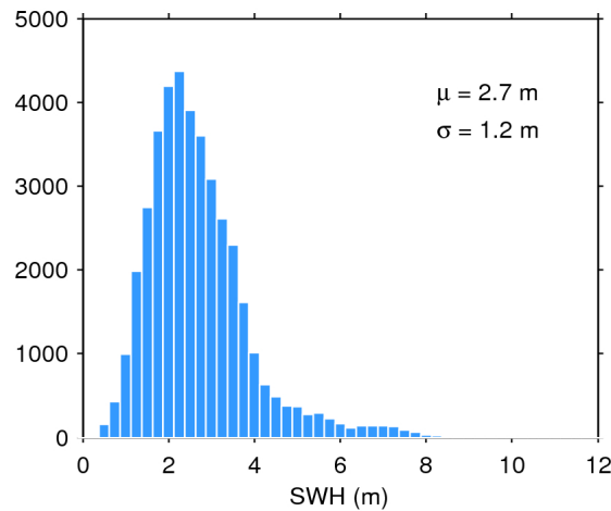
Figure 20. Histogram of science-valid SWH over oceans and lakes for 18/01/2017. The mean ( \mu ) and standard deviation ( \sigma ) are also shown. Note that values larger than 12 m are excluded from the histogram for the sake of readability but not from the computation of \mu and \sigma .
