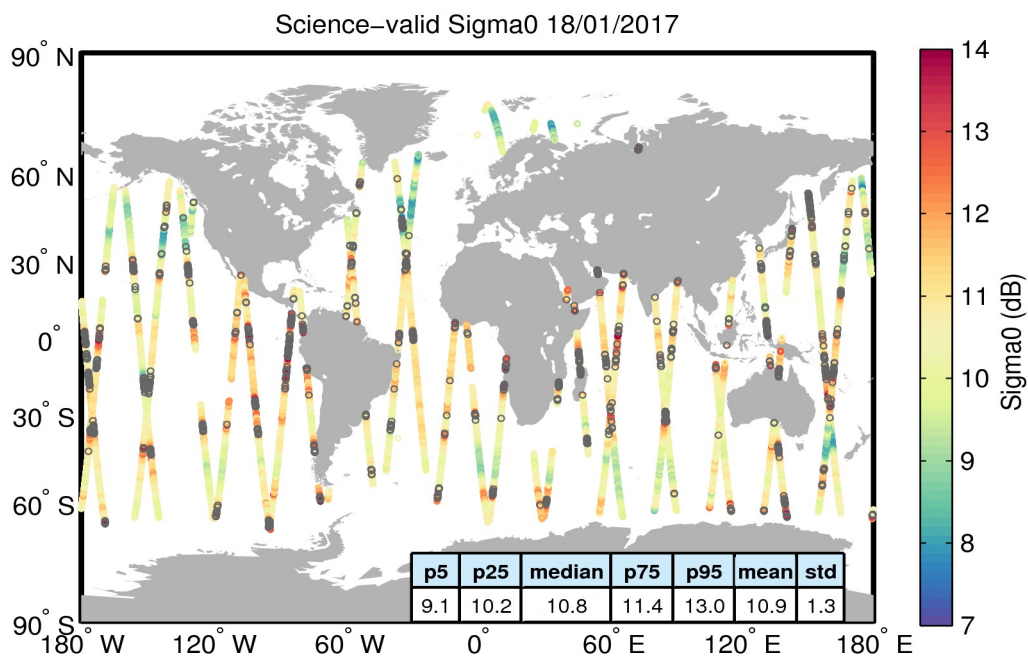
Figure 27. Geographical distribution of science-valid sigma0 data over oceans and lakes for 18/01/2017. The statistical values shown in the table refer to the sigma0 in dB and are calculated over all measurements shown in the figure. Gray circles denote records that have been rejected based on the editing criteria described in Table 4.
