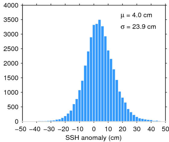
Figure 7. Histogram of flag-valid SSH anomaly over oceans and lakes for 18/01/2017. The mean ( \mu ) and standard deviation ( \sigma ) are also shown. Note that values outside [-50 50] cm are excluded from the histogram for the sake of readability but not from the computation of \mu and \sigma .
