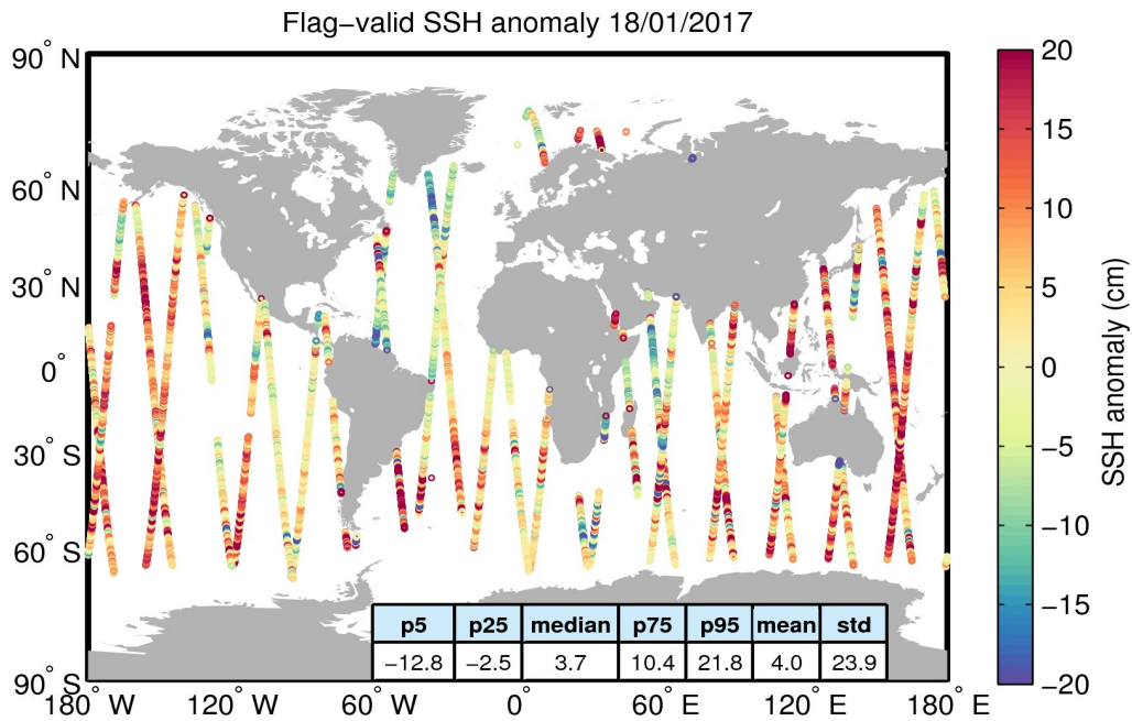
Figure 5. Geographical distribution of flag-valid 1-Hz SSH anomaly data over oceans and lakes for 18/01/2017. The statistical values shown in the table refer to the SSH anomaly in cm and are calculated over all measurements shown in the figure.
