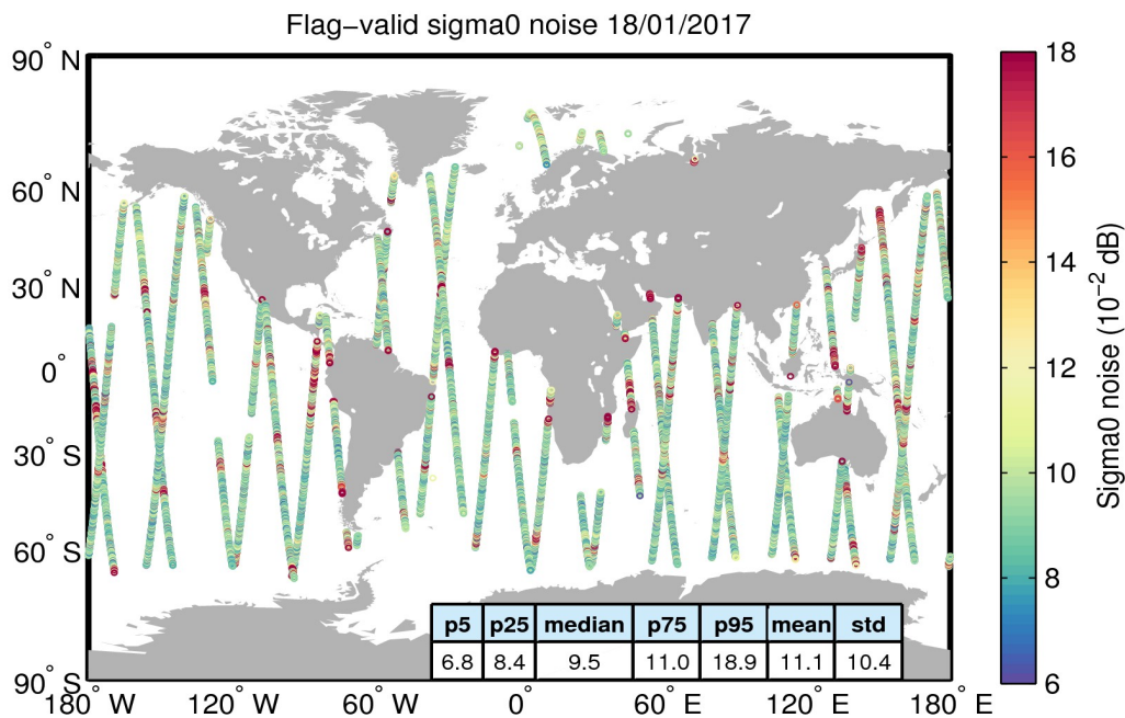
Figure 26. Geographical distribution of flag-valid 20-Hz sigma0 measurement noise over oceans and lakes for 18/01/2017. The statistical values shown in the table refer to the sigma0 noise and are calculated over all measurements shown in the figure.
