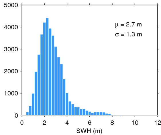
Figure 17. Histogram of flag-valid SWH over oceans and lakes for 18/01/2017. The mean ( \mu ) and standard deviation ( \sigma ) are also shown. Note that values larger than 12 m are excluded from the histogram for the sake of readability but not from the computation of \mu and \sigma .
