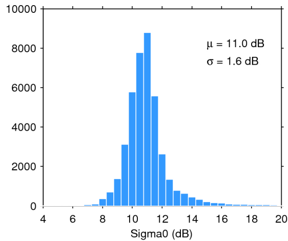
Figure 25. Histogram of flag-valid sigma0 over oceans and lakes for 18/01/2017. The mean ( \mu ) and standard deviation ( \sigma ) are also shown. Note that values outside [4 20] dB are excluded from the histogram for the sake of readability but not from the computation of \mu and \sigma .
