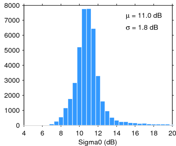
Figure 25. Histogram of flag-valid sigma0 over oceans and lakes for 17/01/2017. The mean ( \mu ) and standard deviation ( \sigma ) are also shown. Note that values outside [4 20] dB are excluded from the histogram for the sake of readability but not from the computation of \mu and \sigma .
