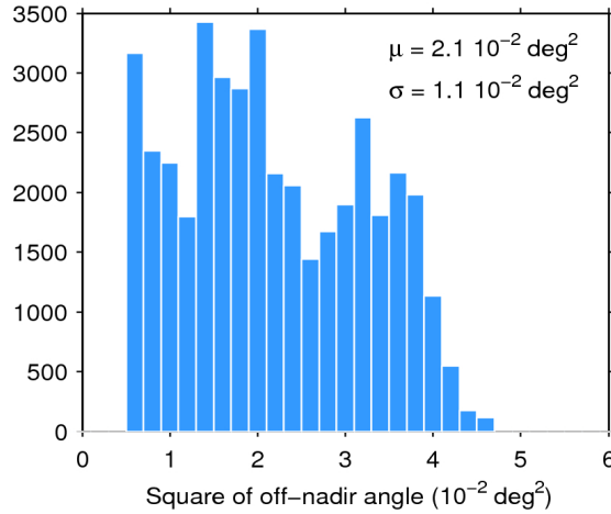
Figure 39. Histogram of flag-valid mispointing over oceans and lakes for 17/01/2017. The mean ( \mu ) and standard deviation ( \sigma ) are also shown. Note that values larger than 6 \cdot 10^{-2} \text{ deg}^2 are excluded from the histogram for the sake of readability but not from the computation of \mu and \sigma .
