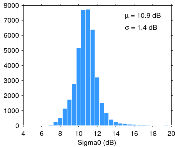
Figure 28. Histogram of science-valid sigma0 over oceans and lakes for 17/01/2017. The mean ( \mu ) and standard deviation ( \sigma ) are also shown. Note that values outside [4 20] dB are excluded from the histogram for the sake of readability but not from the computation of \mu and \sigma .
