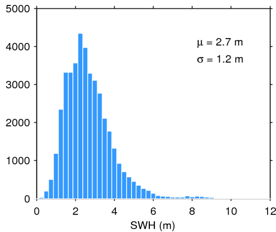
Figure 20. Histogram of science-valid SWH over oceans and lakes for 17/01/2017. The mean ( \mu ) and standard deviation ( \sigma ) are also shown. Note that values larger than 12 m are excluded from the histogram for the sake of readability but not from the computation of \mu and \sigma .
