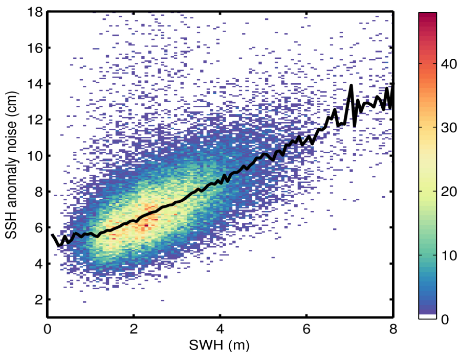
Figure 9. 2D histogram showing flag-valid SSH anomaly noise as a function of SWH for 17/01/2017. The black line denotes the median SSH anomaly noise as a function of SWH.
