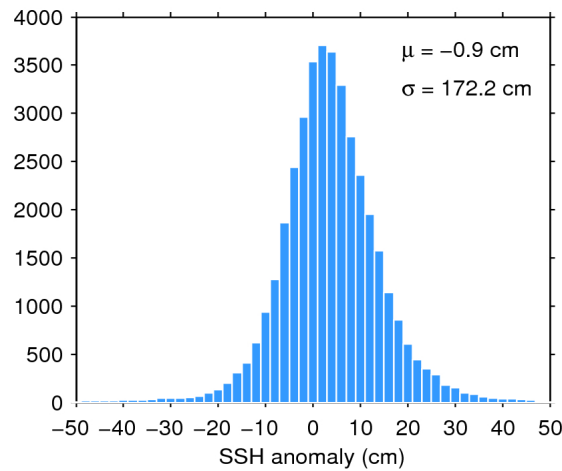
Figure 7. Histogram of flag-valid SSH anomaly over oceans and lakes for 17/01/2017. The mean ( \mu ) and standard deviation ( \sigma ) are also shown. Note that values outside [-50 50] cm are excluded from the histogram for the sake of readability but not from the computation of \mu and \sigma .
