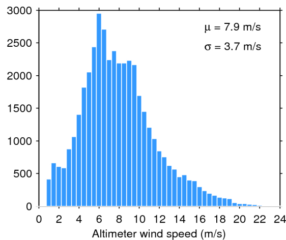
Figure 35. Histogram of science-valid wind over oceans and lakes for 17/01/2017. The mean ( \mu ) and standard deviation ( \sigma ) are also shown. Note that values larger than 24 m/s are excluded from the histogram for the sake of readability but not from the computation of \mu and \sigma .
