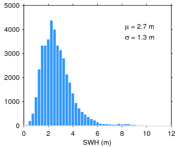
Figure 17. Histogram of flag-valid SWH over oceans and lakes for 17/01/2017. The mean ( \mu ) and standard deviation ( \sigma ) are also shown. Note that values larger than 12 m are excluded from the histogram for the sake of readability but not from the computation of \mu and \sigma .
