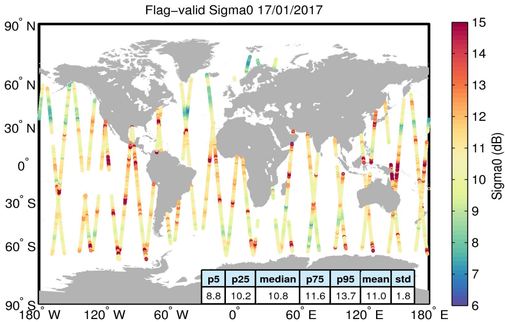
Figure 23. Geographical distribution of flag-valid sigma0 data over oceans and lakes for 17/01/2017. The statistical values shown in the table refer to the sigma0 in dB and are calculated over all measurements shown in the figure.
