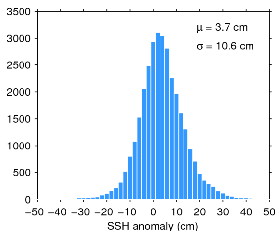
Figure 11. Histogram of science-valid SSH anomaly over oceans and lakes for 17/01/2017. The mean ( \mu ) and standard deviation ( \sigma ) are also shown. Note that values outside [-50 50] cm are excluded from the histogram for the sake of readability but not from the computation of \mu and \sigma .
