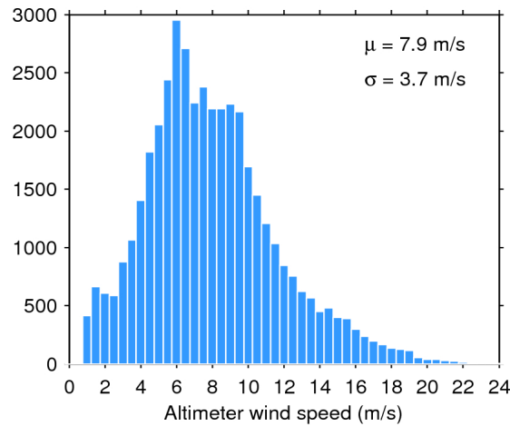
Figure 33. Histogram of flag-valid wind over oceans and lakes for 17/01/2017. The mean ( \mu ) and standard deviation ( \sigma ) are also shown. Note that values larger than 24 m/s are excluded from the histogram for the sake of readability but not from the computation of \mu and \sigma .
