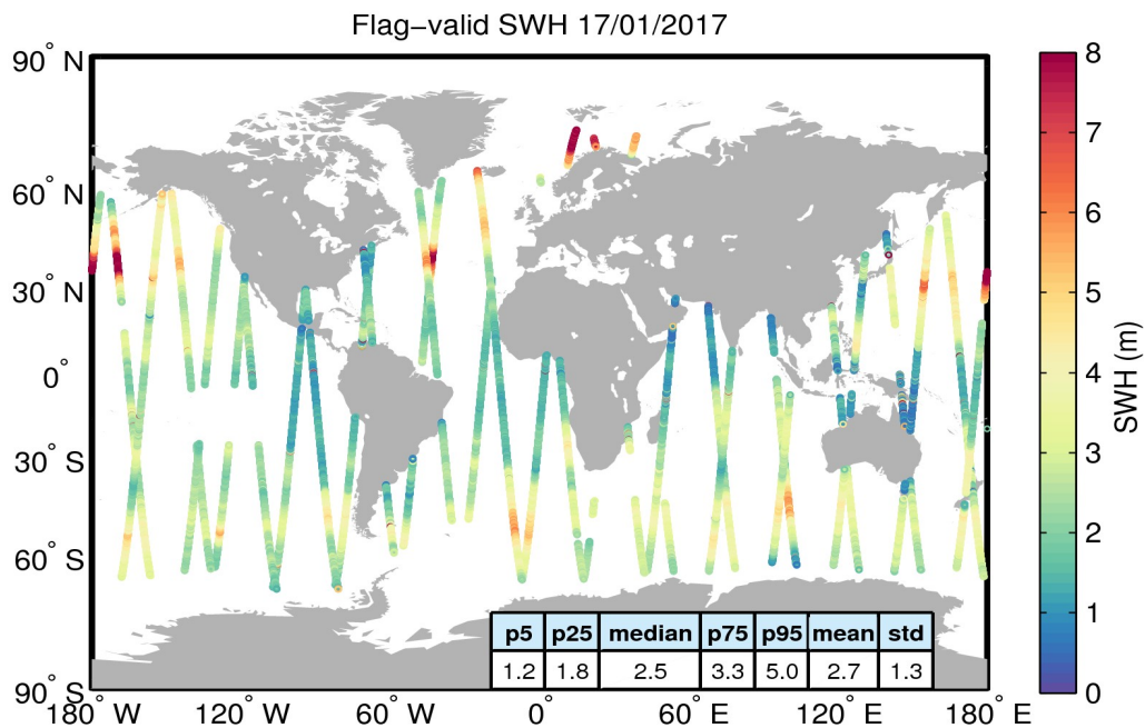
Figure 15. Geographical distribution of flag-valid SWH data over oceans and lakes for 17/01/2017. The statistical values shown in the table refer to the SWH in m and are calculated over all measurements shown in the figure.
