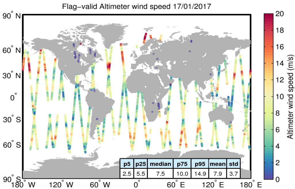
Figure 31. Geographical distribution of flag-valid wind data over oceans and lakes for 17/01/2017. The statistical values shown in the table refer to the wind in m/s and are calculated over all measurements shown in the figure.
