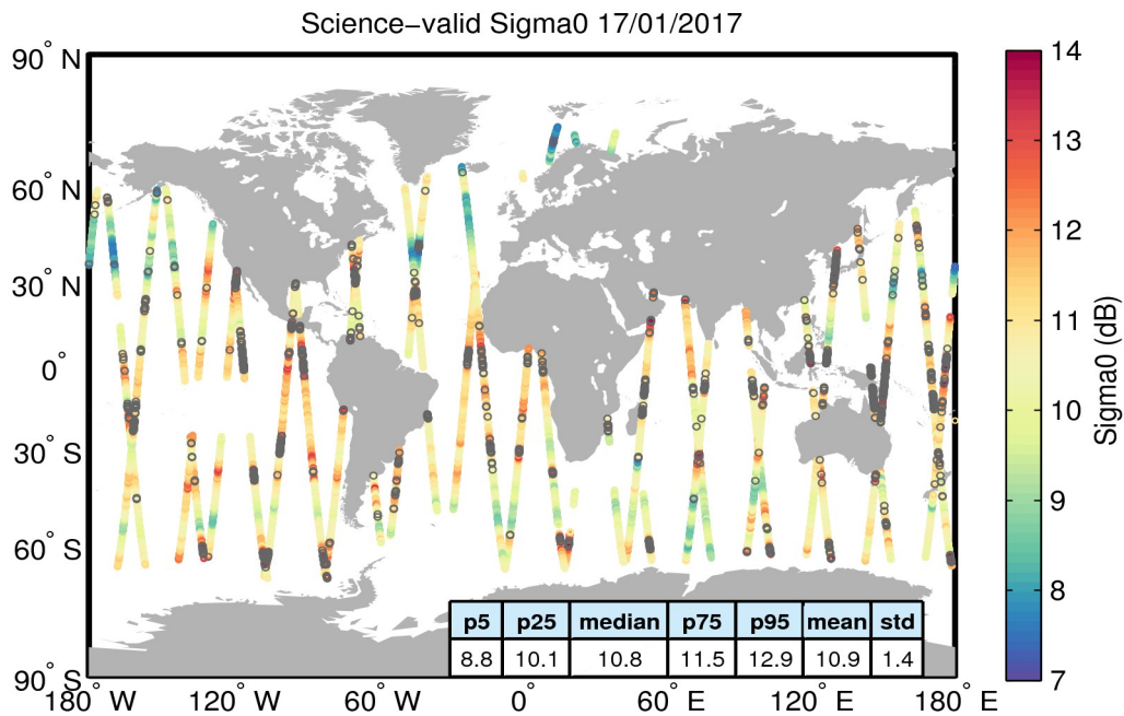
Figure 27. Geographical distribution of science-valid sigma0 data over oceans and lakes for 17/01/2017. The statistical values shown in the table refer to the sigma0 in dB and are calculated over all measurements shown in the figure. Gray circles denote records that have been rejected based on the editing criteria described in Table 4.
