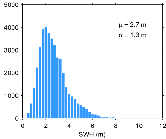
Figure 17. Histogram of flag-valid SWH over oceans and lakes for 16/01/2017. The mean ( \mu ) and standard deviation ( \sigma ) are also shown. Note that values larger than 12 m are excluded from the histogram for the sake of readability but not from the computation of \mu and \sigma .
