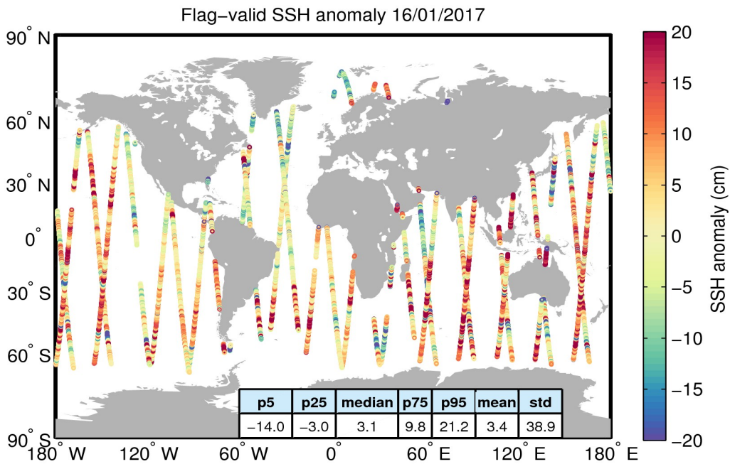
Figure 5. Geographical distribution of flag-valid 1-Hz SSH anomaly data over oceans and lakes for 16/01/2017. The statistical values shown in the table refer to the SSH anomaly in cm and are calculated over all measurements shown in the figure.
