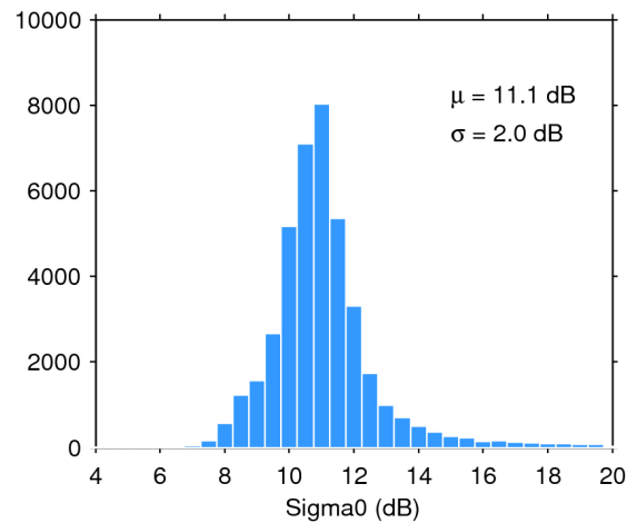
Figure 25. Histogram of flag-valid sigma0 over oceans and lakes for 16/01/2017. The mean ( \mu ) and standard deviation ( \sigma ) are also shown. Note that values outside [4 20] dB are excluded from the histogram for the sake of readability but not from the computation of \mu and \sigma .
