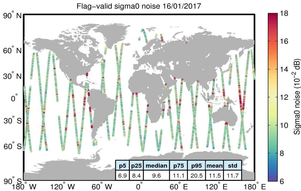
Figure 26. Geographical distribution of flag-valid 20-Hz sigma0 measurement noise over oceans and lakes for 16/01/2017. The statistical values shown in the table refer to the sigma0 noise and are calculated over all measurements shown in the figure.
