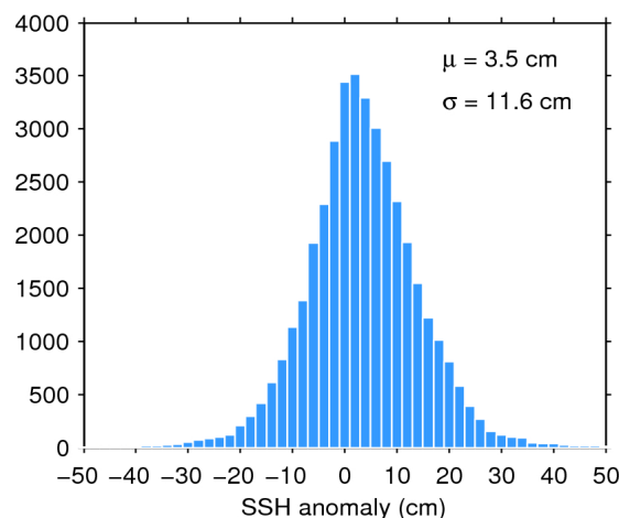
Figure 11. Histogram of science-valid SSH anomaly over oceans and lakes for 16/01/2017. The mean ( \mu ) and standard deviation ( \sigma ) are also shown. Note that values outside [-50 50] cm are excluded from the histogram for the sake of readability but not from the computation of \mu and \sigma .
