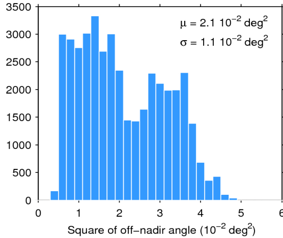
Figure 39. Histogram of flag-valid mispointing over oceans and lakes for 16/01/2017. The mean ( \mu ) and standard deviation ( \sigma ) are also shown. Note that values larger than 6 \cdot 10^{-2} \text{ deg}^2 are excluded from the histogram for the sake of readability but not from the computation of \mu and \sigma .
