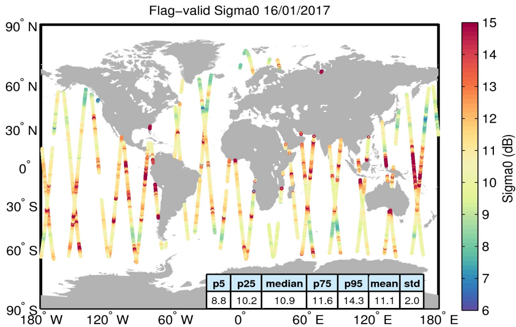
Figure 23. Geographical distribution of flag-valid sigma0 data over oceans and lakes for 16/01/2017. The statistical values shown in the table refer to the sigma0 in dB and are calculated over all measurements shown in the figure.
