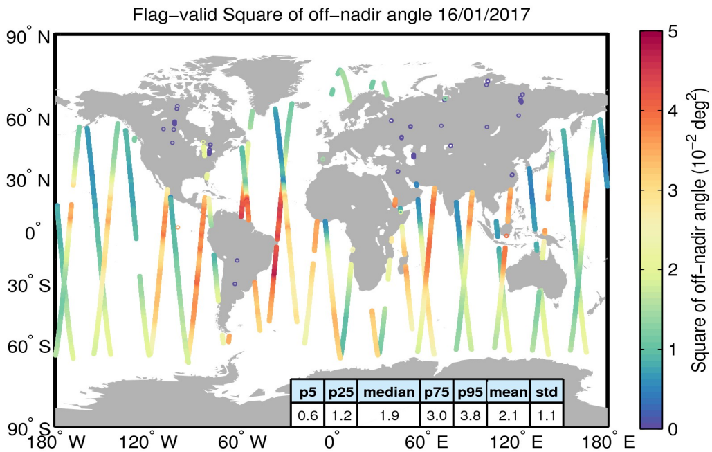
Figure 37. Geographical distribution of flag-valid mispointing data over oceans and lakes for 16/01/2017. The statistical values shown in the table refer to the mispointing in 10^{-2} deg 2 and are calculated over all measurements shown in the figure.
