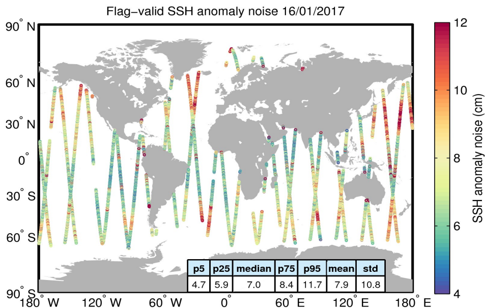
Figure 8. Geographical distribution of flag-valid 20-Hz SSH anomaly measurement noise over oceans and lakes for 16/01/2017. The statistical values shown in the table refer to the SSH anomaly noise and are calculated over all measurements shown in the figure.
