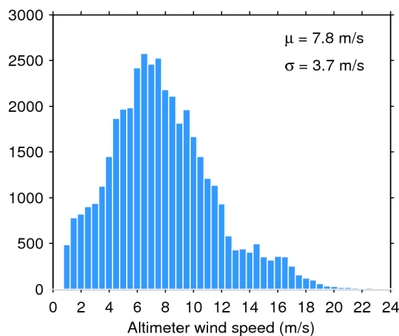
Figure 35. Histogram of science-valid wind over oceans and lakes for 16/01/2017. The mean ( \mu ) and standard deviation ( \sigma ) are also shown. Note that values larger than 24 m/s are excluded from the histogram for the sake of readability but not from the computation of \mu and \sigma .
