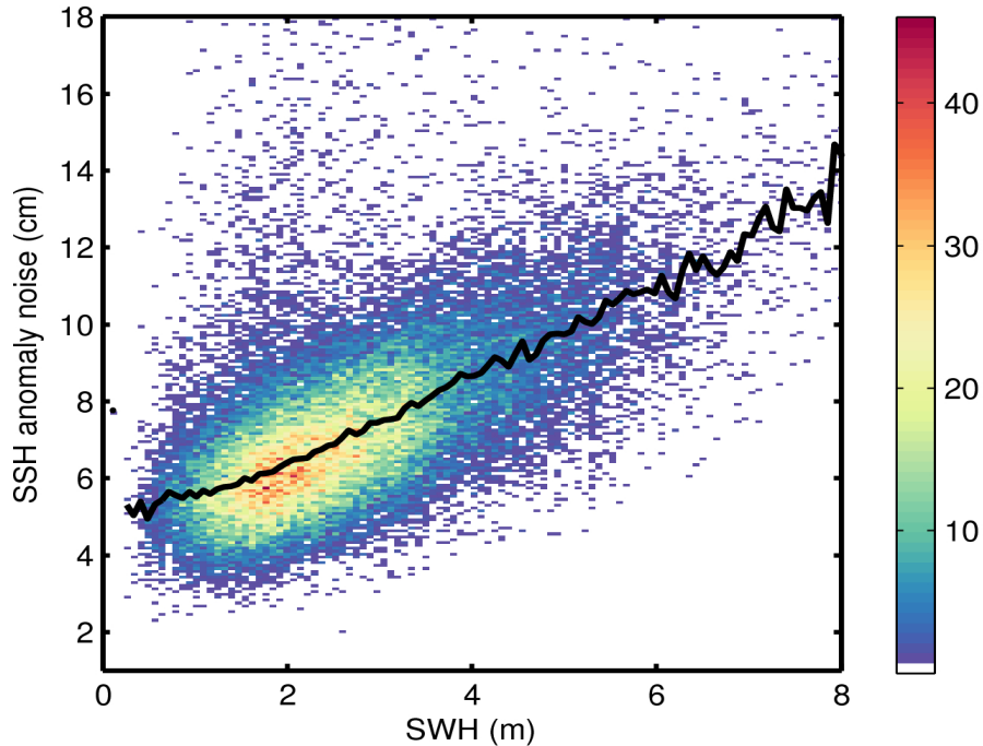
Figure 9. 2D histogram showing flag-valid SSH anomaly noise as a function of SWH for 16/01/2017. The black line denotes the median SSH anomaly noise as a function of SWH.
