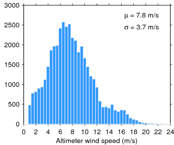
Figure 33. Histogram of flag-valid wind over oceans and lakes for 16/01/2017. The mean ( \mu ) and standard deviation ( \sigma ) are also shown. Note that values larger than 24 m/s are excluded from the histogram for the sake of readability but not from the computation of \mu and \sigma .
