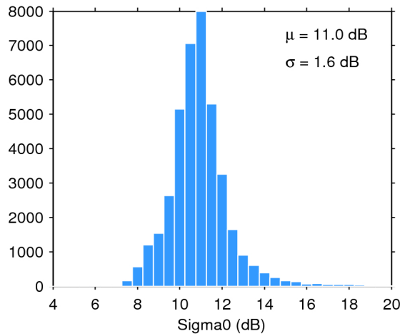
Figure 28. Histogram of science-valid sigma0 over oceans and lakes for 16/01/2017. The mean ( \mu ) and standard deviation ( \sigma ) are also shown. Note that values outside [4 20] dB are excluded from the histogram for the sake of readability but not from the computation of \mu and \sigma .
