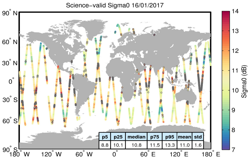
Figure 27. Geographical distribution of science-valid sigma0 data over oceans and lakes for 16/01/2017. The statistical values shown in the table refer to the sigma0 in dB and are calculated over all measurements shown in the figure. Gray circles denote records that have been rejected based on the editing criteria described in Table 4.
