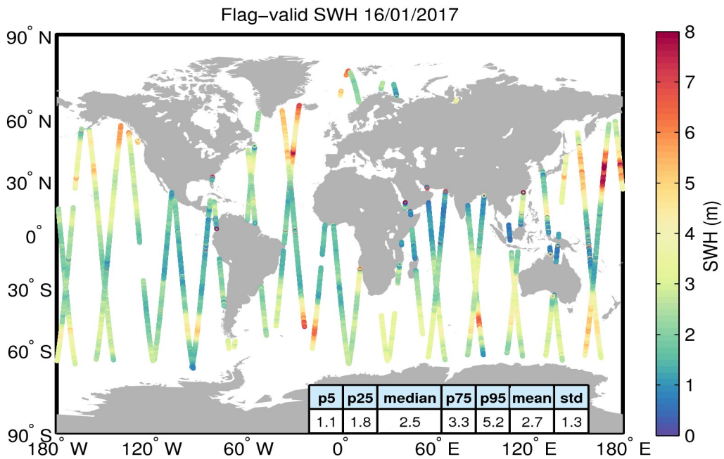
Figure 15. Geographical distribution of flag-valid SWH data over oceans and lakes for 16/01/2017. The statistical values shown in the table refer to the SWH in m and are calculated over all measurements shown in the figure.
