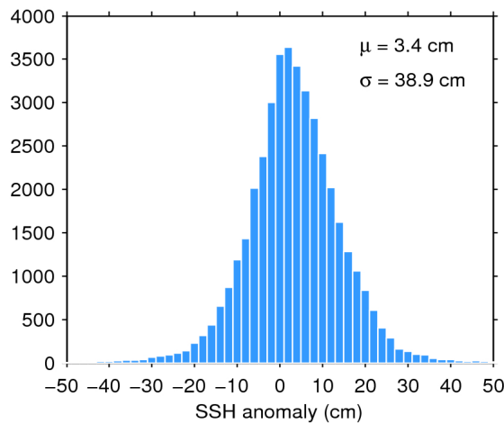
Figure 7. Histogram of flag-valid SSH anomaly over oceans and lakes for 16/01/2017. The mean ( \mu ) and standard deviation ( \sigma ) are also shown. Note that values outside [-50 50] cm are excluded from the histogram for the sake of readability but not from the computation of \mu and \sigma .
