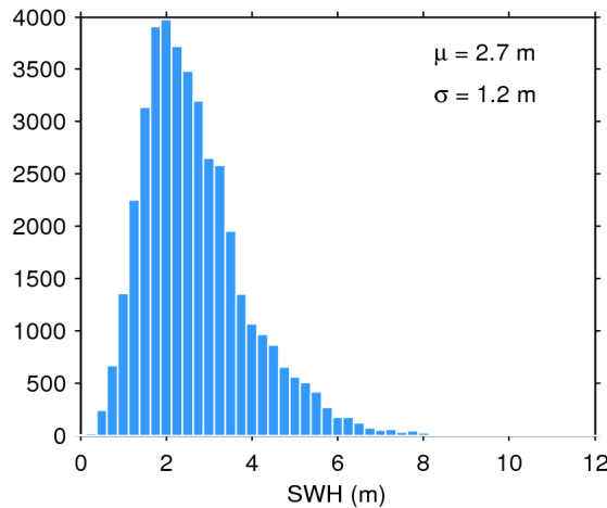
Figure 20. Histogram of science-valid SWH over oceans and lakes for 16/01/2017. The mean ( \mu ) and standard deviation ( \sigma ) are also shown. Note that values larger than 12 m are excluded from the histogram for the sake of readability but not from the computation of \mu and \sigma .
