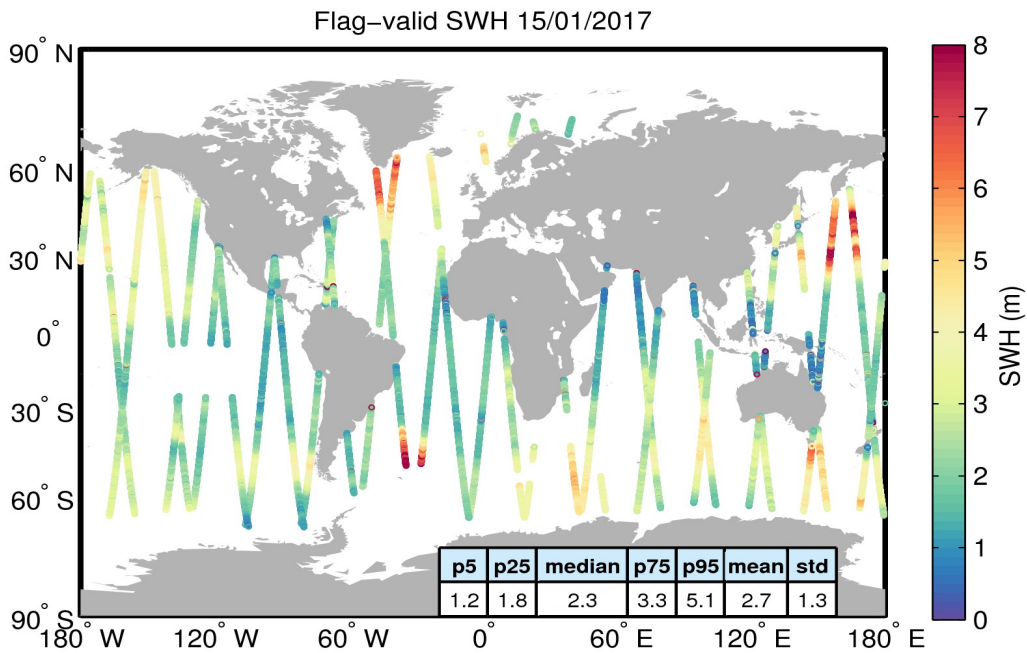
Figure 15. Geographical distribution of flag-valid SWH data over oceans and lakes for 15/01/2017. The statistical values shown in the table refer to the SWH in m and are calculated over all measurements shown in the figure.
