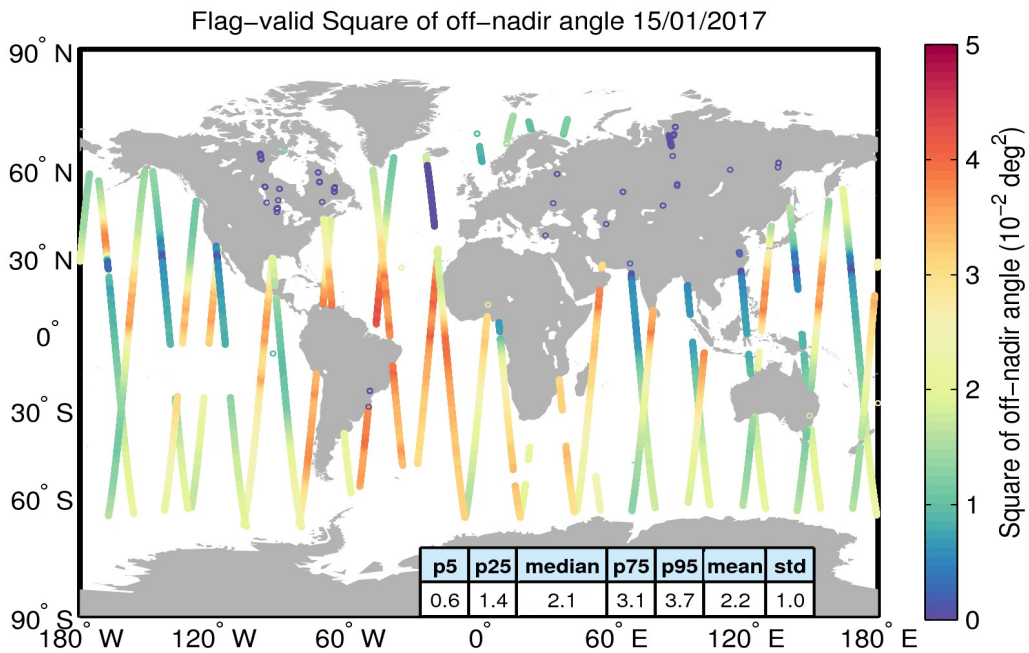
Figure 37. Geographical distribution of flag-valid mispointing data over oceans and lakes for 15/01/2017. The statistical values shown in the table refer to the mispointing in 10^{-2} deg 2 and are calculated over all measurements shown in the figure.
