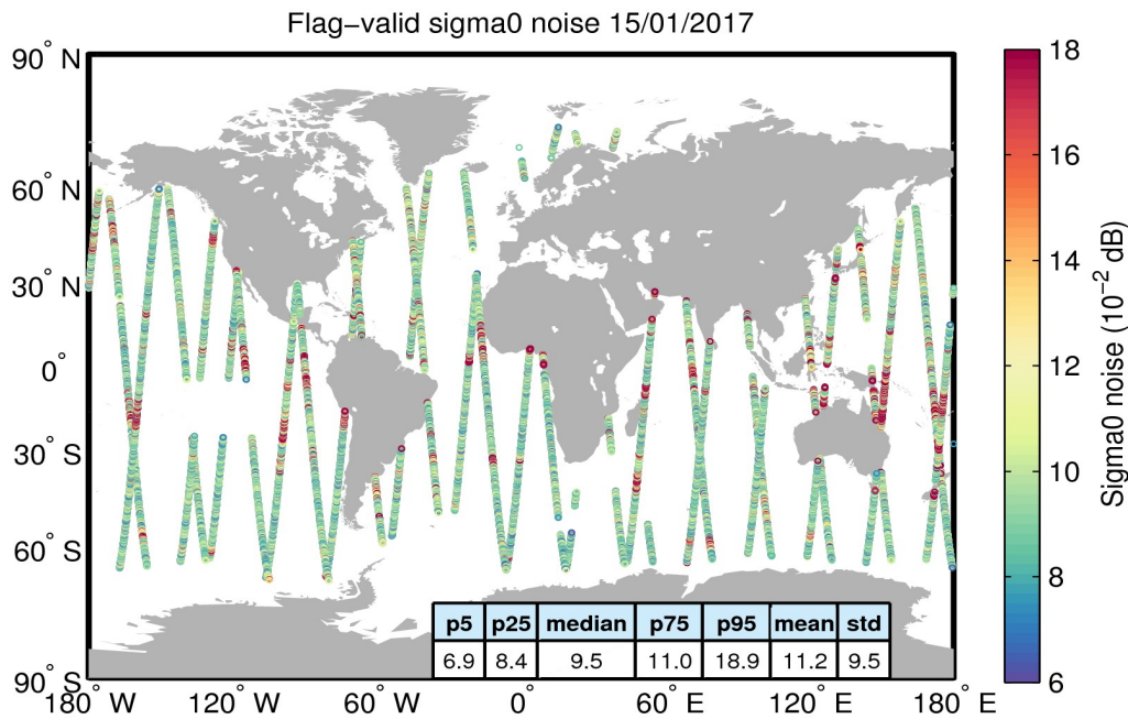
Figure 26. Geographical distribution of flag-valid 20-Hz sigma0 measurement noise over oceans and lakes for 15/01/2017. The statistical values shown in the table refer to the sigma0 noise and are calculated over all measurements shown in the figure.
