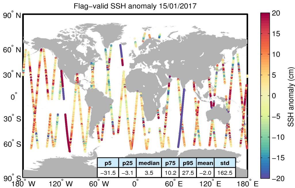
Figure 5. Geographical distribution of flag-valid 1-Hz SSH anomaly data over oceans and lakes for 15/01/2017. The statistical values shown in the table refer to the SSH anomaly in cm and are calculated over all measurements shown in the figure.
