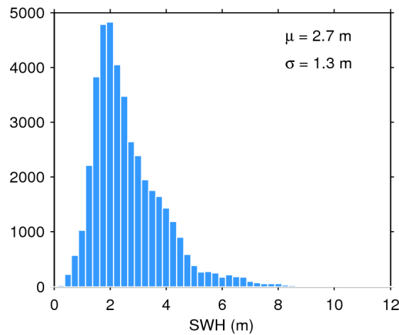
Figure 17. Histogram of flag-valid SWH over oceans and lakes for 15/01/2017. The mean ( \mu ) and standard deviation ( \sigma ) are also shown. Note that values larger than 12 m are excluded from the histogram for the sake of readability but not from the computation of \mu and \sigma .
