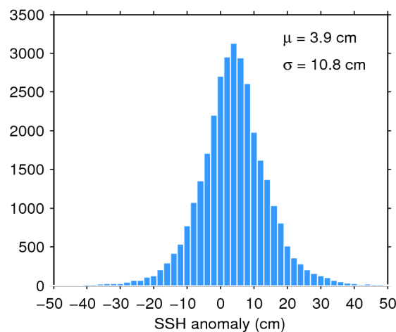
Figure 11. Histogram of science-valid SSH anomaly over oceans and lakes for 15/01/2017. The mean ( \mu ) and standard deviation ( \sigma ) are also shown. Note that values outside [-50 50] cm are excluded from the histogram for the sake of readability but not from the computation of \mu and \sigma .
