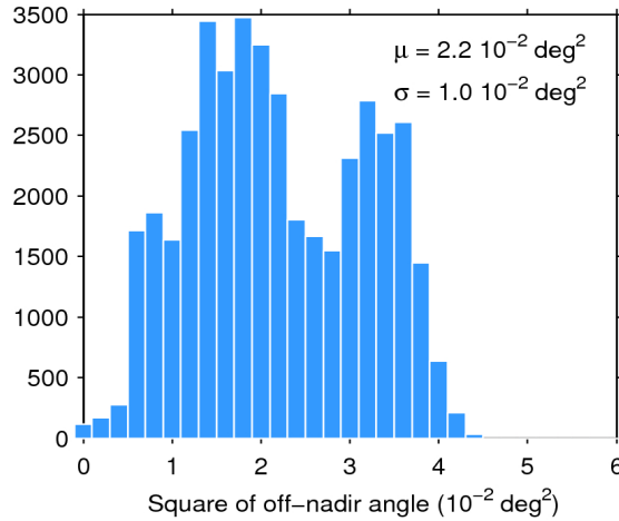
Figure 39. Histogram of flag-valid mispointing over oceans and lakes for 15/01/2017. The mean ( \mu ) and standard deviation ( \sigma ) are also shown. Note that values larger than 6 \cdot 10^{-2} \text{ deg}^2 are excluded from the histogram for the sake of readability but not from the computation of \mu and \sigma .
