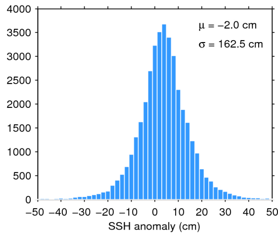
Figure 7. Histogram of flag-valid SSH anomaly over oceans and lakes for 15/01/2017. The mean ( \mu ) and standard deviation ( \sigma ) are also shown. Note that values outside [-50 50] cm are excluded from the histogram for the sake of readability but not from the computation of \mu and \sigma .
