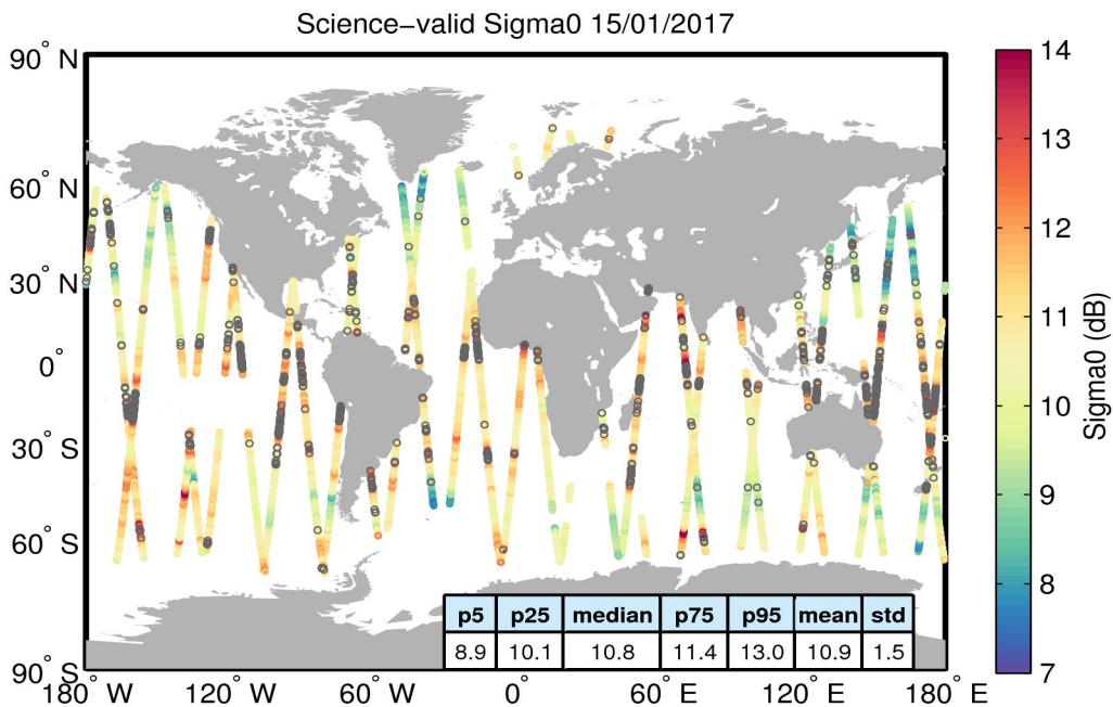
Figure 27. Geographical distribution of science-valid sigma0 data over oceans and lakes for 15/01/2017. The statistical values shown in the table refer to the sigma0 in dB and are calculated over all measurements shown in the figure. Gray circles denote records that have been rejected based on the editing criteria described in Table 4.
