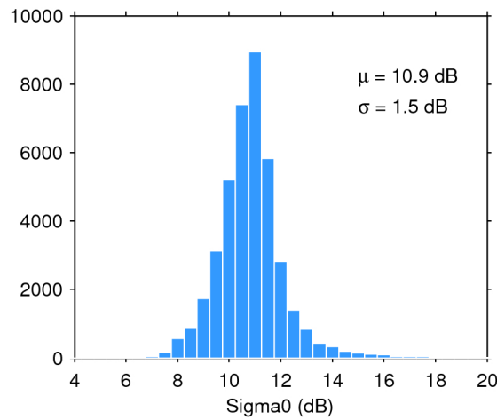
Figure 28. Histogram of science-valid sigma0 over oceans and lakes for 15/01/2017. The mean ( \mu ) and standard deviation ( \sigma ) are also shown. Note that values outside [4 20] dB are excluded from the histogram for the sake of readability but not from the computation of \mu and \sigma .
