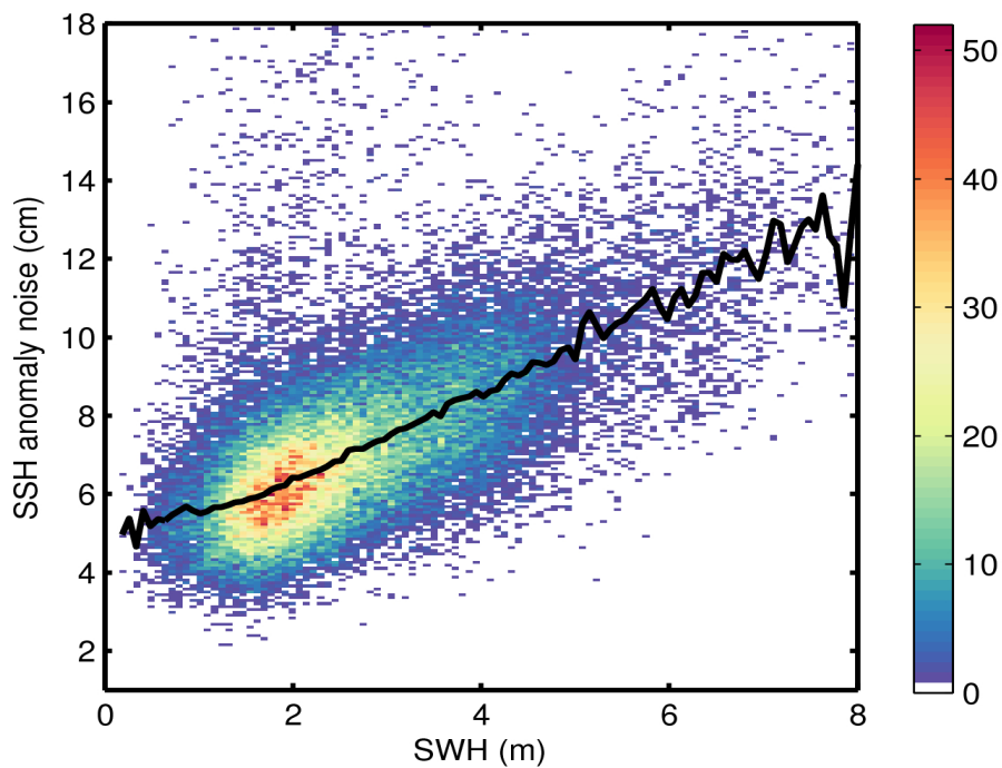
Figure 9. 2D histogram showing flag-valid SSH anomaly noise as a function of SWH for 15/01/2017. The black line denotes the median SSH anomaly noise as a function of SWH.
