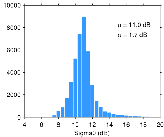
Figure 25. Histogram of flag-valid sigma0 over oceans and lakes for 15/01/2017. The mean ( \mu ) and standard deviation ( \sigma ) are also shown. Note that values outside [4 20] dB are excluded from the histogram for the sake of readability but not from the computation of \mu and \sigma .
