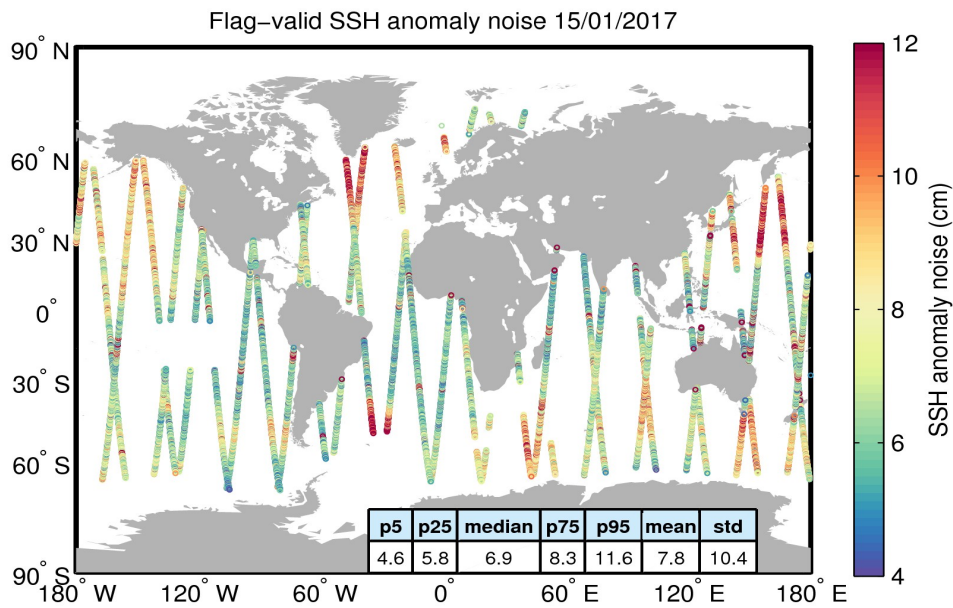
Figure 8. Geographical distribution of flag-valid 20-Hz SSH anomaly measurement noise over oceans and lakes for 15/01/2017. The statistical values shown in the table refer to the SSH anomaly noise and are calculated over all measurements shown in the figure.
