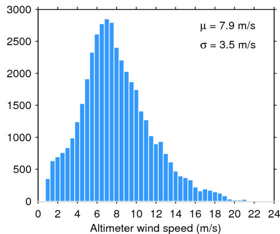
Figure 35. Histogram of science-valid wind over oceans and lakes for 15/01/2017. The mean ( \mu ) and standard deviation ( \sigma ) are also shown. Note that values larger than 24 m/s are excluded from the histogram for the sake of readability but not from the computation of \mu and \sigma .
