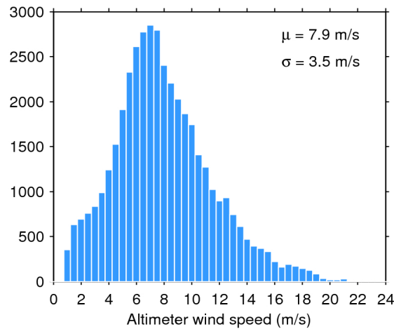
Figure 33. Histogram of flag-valid wind over oceans and lakes for 15/01/2017. The mean ( \mu ) and standard deviation ( \sigma ) are also shown. Note that values larger than 24 m/s are excluded from the histogram for the sake of readability but not from the computation of \mu and \sigma .
