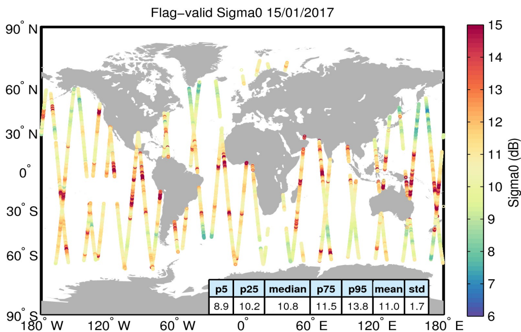
Figure 23. Geographical distribution of flag-valid sigma0 data over oceans and lakes for 15/01/2017. The statistical values shown in the table refer to the sigma0 in dB and are calculated over all measurements shown in the figure.
