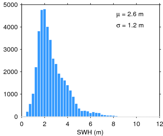
Figure 20. Histogram of science-valid SWH over oceans and lakes for 15/01/2017. The mean ( \mu ) and standard deviation ( \sigma ) are also shown. Note that values larger than 12 m are excluded from the histogram for the sake of readability but not from the computation of \mu and \sigma .
