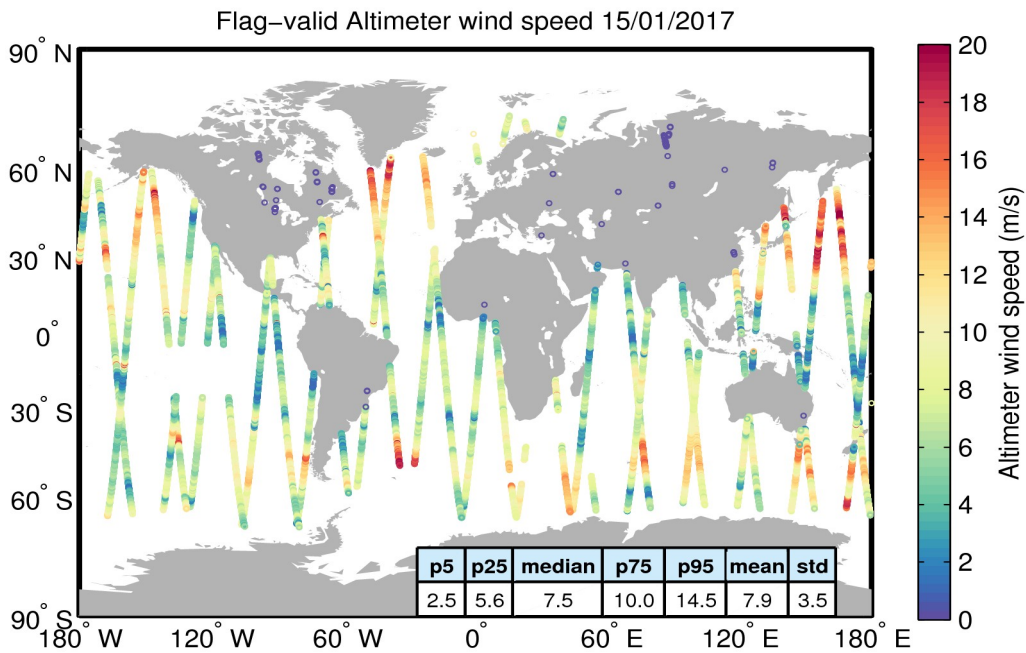
Figure 31. Geographical distribution of flag-valid wind data over oceans and lakes for 15/01/2017. The statistical values shown in the table refer to the wind in m/s and are calculated over all measurements shown in the figure.
