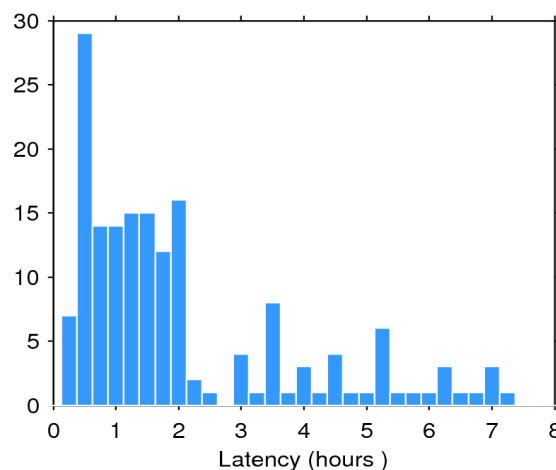
Figure 2. Histogram of the data latency for 15/01/2017. The y-axis denotes the number of files that are made available with a delay of x-hours with respect to the mean time of the records stored in the file.
