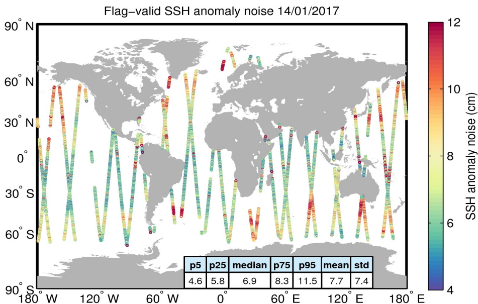
Figure 8. Geographical distribution of flag-valid 20-Hz SSH anomaly measurement noise over oceans and lakes for 14/01/2017. The statistical values shown in the table refer to the SSH anomaly noise and are calculated over all measurements shown in the figure.
