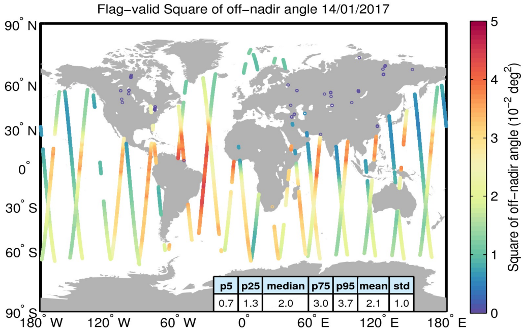
Figure 37. Geographical distribution of flag-valid mispointing data over oceans and lakes for 14/01/2017. The statistical values shown in the table refer to the mispointing in 10^{-2} deg 2 and are calculated over all measurements shown in the figure.
