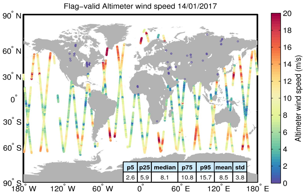
Figure 31. Geographical distribution of flag-valid wind data over oceans and lakes for 14/01/2017. The statistical values shown in the table refer to the wind in m/s and are calculated over all measurements shown in the figure.
