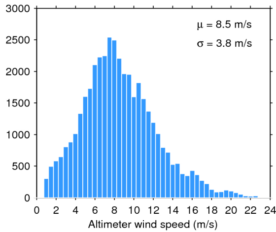
Figure 33. Histogram of flag-valid wind over oceans and lakes for 14/01/2017. The mean ( \mu ) and standard deviation ( \sigma ) are also shown. Note that values larger than 24 m/s are excluded from the histogram for the sake of readability but not from the computation of \mu and \sigma .
