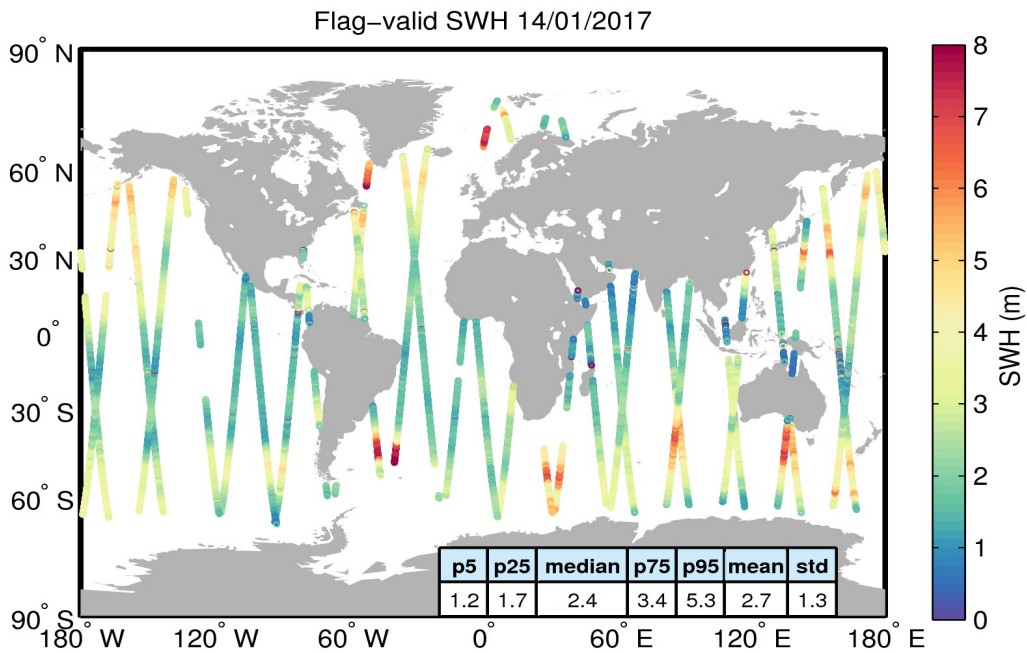
Figure 15. Geographical distribution of flag-valid SWH data over oceans and lakes for 14/01/2017. The statistical values shown in the table refer to the SWH in m and are calculated over all measurements shown in the figure.
