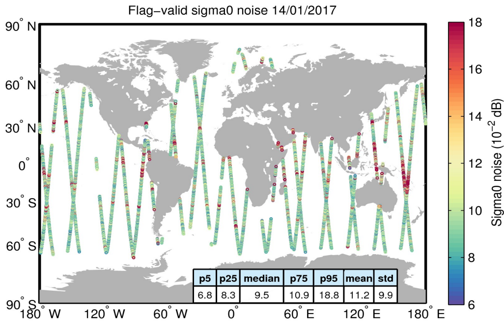
Figure 26. Geographical distribution of flag-valid 20-Hz sigma0 measurement noise over oceans and lakes for 14/01/2017. The statistical values shown in the table refer to the sigma0 noise and are calculated over all measurements shown in the figure.
