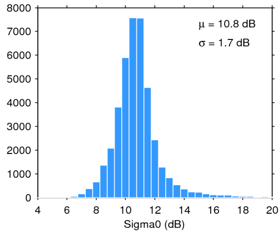
Figure 25. Histogram of flag-valid sigma0 over oceans and lakes for 14/01/2017. The mean ( \mu ) and standard deviation ( \sigma ) are also shown. Note that values outside [4 20] dB are excluded from the histogram for the sake of readability but not from the computation of \mu and \sigma .
