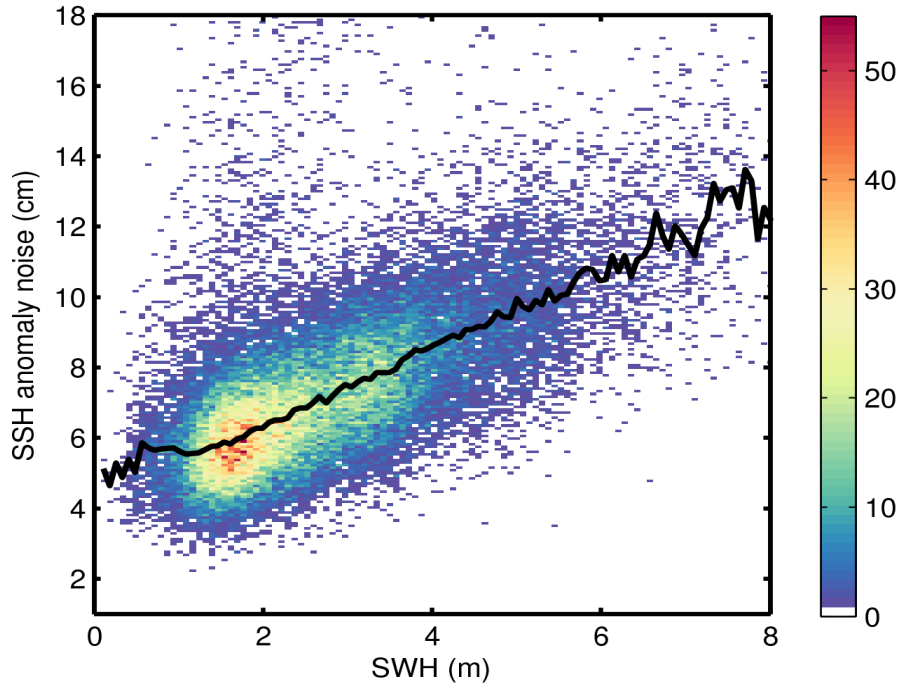
Figure 9. 2D histogram showing flag-valid SSH anomaly noise as a function of SWH for 14/01/2017. The black line denotes the median SSH anomaly noise as a function of SWH.
