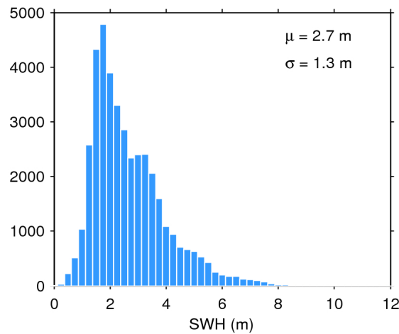
Figure 17. Histogram of flag-valid SWH over oceans and lakes for 14/01/2017. The mean ( \mu ) and standard deviation ( \sigma ) are also shown. Note that values larger than 12 m are excluded from the histogram for the sake of readability but not from the computation of \mu and \sigma .
