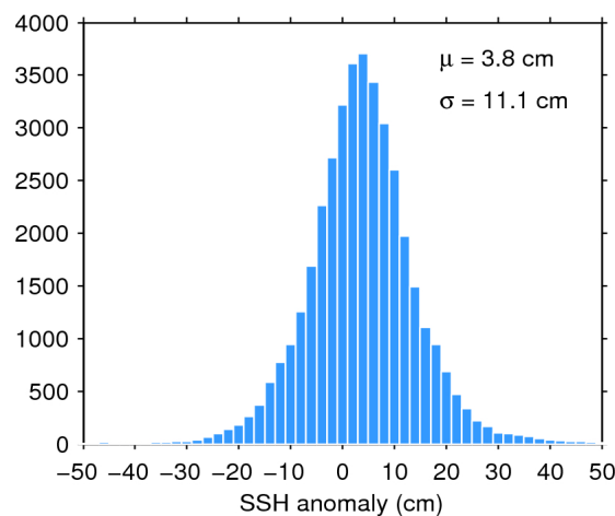
Figure 11. Histogram of science-valid SSH anomaly over oceans and lakes for 14/01/2017. The mean ( \mu ) and standard deviation ( \sigma ) are also shown. Note that values outside [-50 50] cm are excluded from the histogram for the sake of readability but not from the computation of \mu and \sigma .
