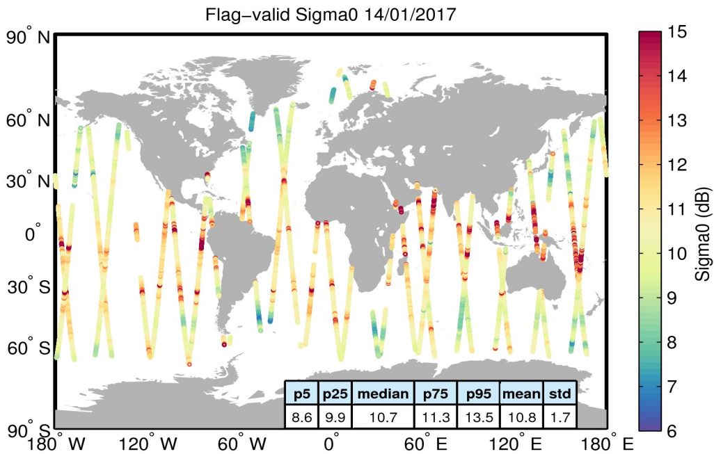
Figure 23. Geographical distribution of flag-valid sigma0 data over oceans and lakes for 14/01/2017. The statistical values shown in the table refer to the sigma0 in dB and are calculated over all measurements shown in the figure.
