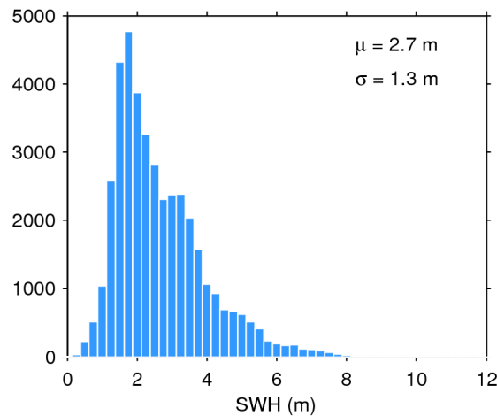
Figure 20. Histogram of science-valid SWH over oceans and lakes for 14/01/2017. The mean ( \mu ) and standard deviation ( \sigma ) are also shown. Note that values larger than 12 m are excluded from the histogram for the sake of readability but not from the computation of \mu and \sigma .
