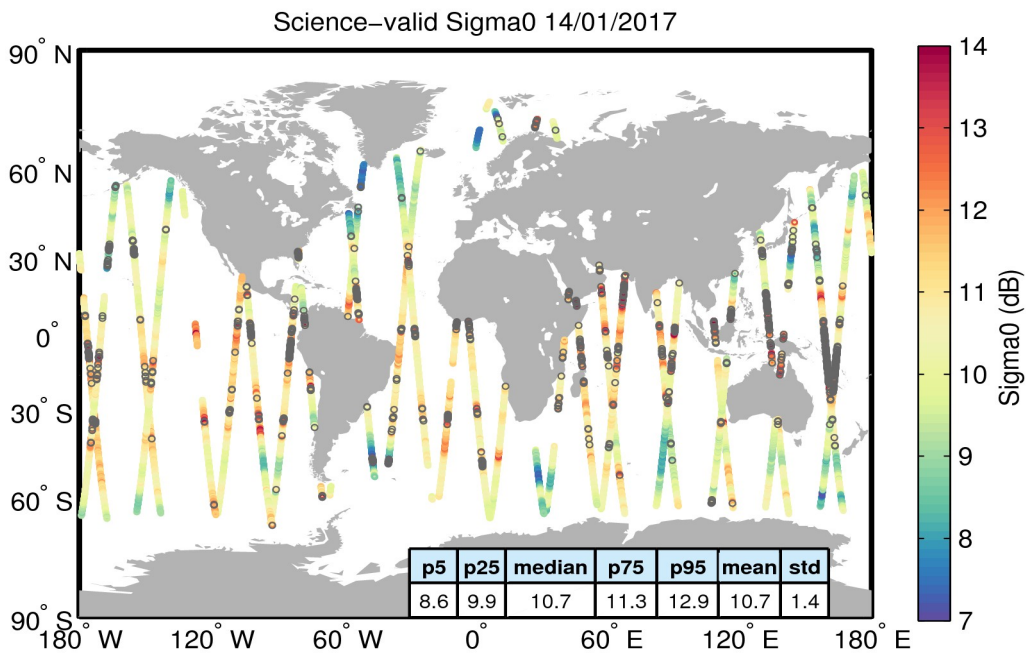
Figure 27. Geographical distribution of science-valid sigma0 data over oceans and lakes for 14/01/2017. The statistical values shown in the table refer to the sigma0 in dB and are calculated over all measurements shown in the figure. Gray circles denote records that have been rejected based on the editing criteria described in Table 4.
