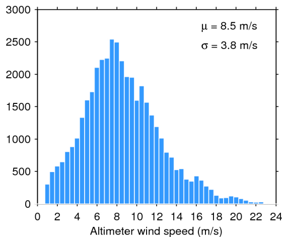
Figure 35. Histogram of science-valid wind over oceans and lakes for 14/01/2017. The mean ( \mu ) and standard deviation ( \sigma ) are also shown. Note that values larger than 24 m/s are excluded from the histogram for the sake of readability but not from the computation of \mu and \sigma .
