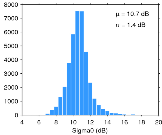
Figure 28. Histogram of science-valid sigma0 over oceans and lakes for 14/01/2017. The mean ( \mu ) and standard deviation ( \sigma ) are also shown. Note that values outside [4 20] dB are excluded from the histogram for the sake of readability but not from the computation of \mu and \sigma .
