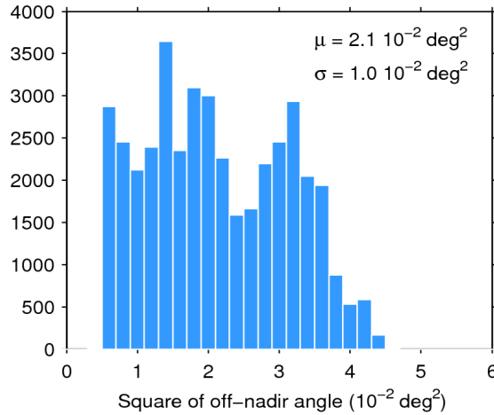
Figure 39. Histogram of flag-valid mispointing over oceans and lakes for 14/01/2017. The mean ( \mu ) and standard deviation ( \sigma ) are also shown. Note that values larger than 6 \cdot 10^{-2} \text{ deg}^2 are excluded from the histogram for the sake of readability but not from the computation of \mu and \sigma .
