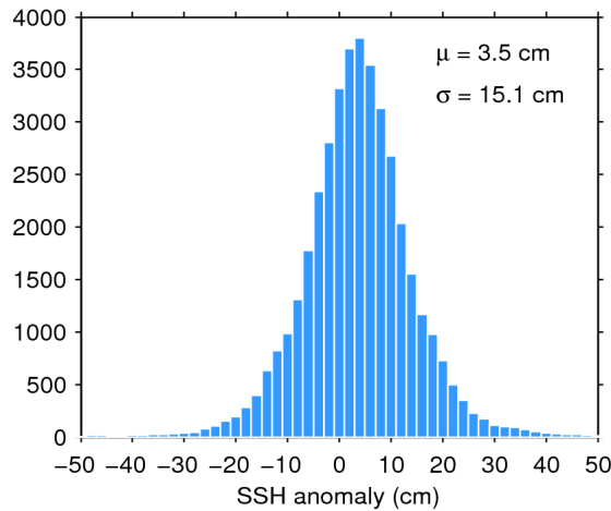
Figure 7. Histogram of flag-valid SSH anomaly over oceans and lakes for 14/01/2017. The mean ( \mu ) and standard deviation ( \sigma ) are also shown. Note that values outside [-50 50] cm are excluded from the histogram for the sake of readability but not from the computation of \mu and \sigma .
