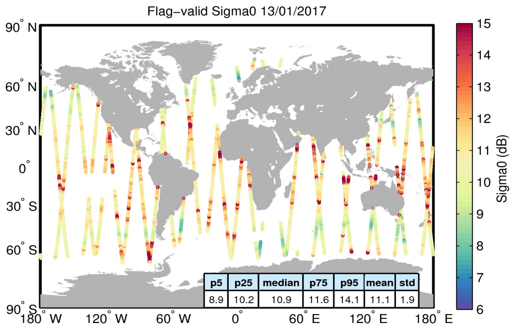
Figure 23. Geographical distribution of flag-valid sigma0 data over oceans and lakes for 13/01/2017. The statistical values shown in the table refer to the sigma0 in dB and are calculated over all measurements shown in the figure.
