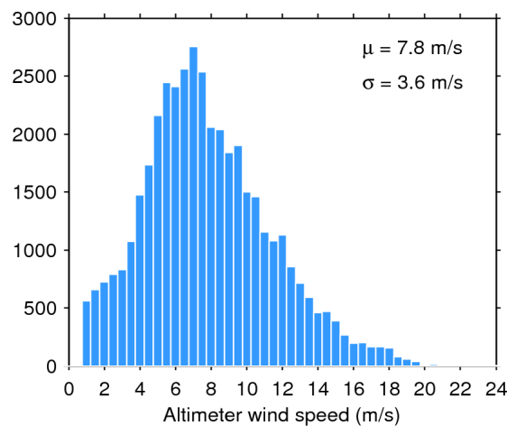
Figure 35. Histogram of science-valid wind over oceans and lakes for 13/01/2017. The mean ( \mu ) and standard deviation ( \sigma ) are also shown. Note that values larger than 24 m/s are excluded from the histogram for the sake of readability but not from the computation of \mu and \sigma .
