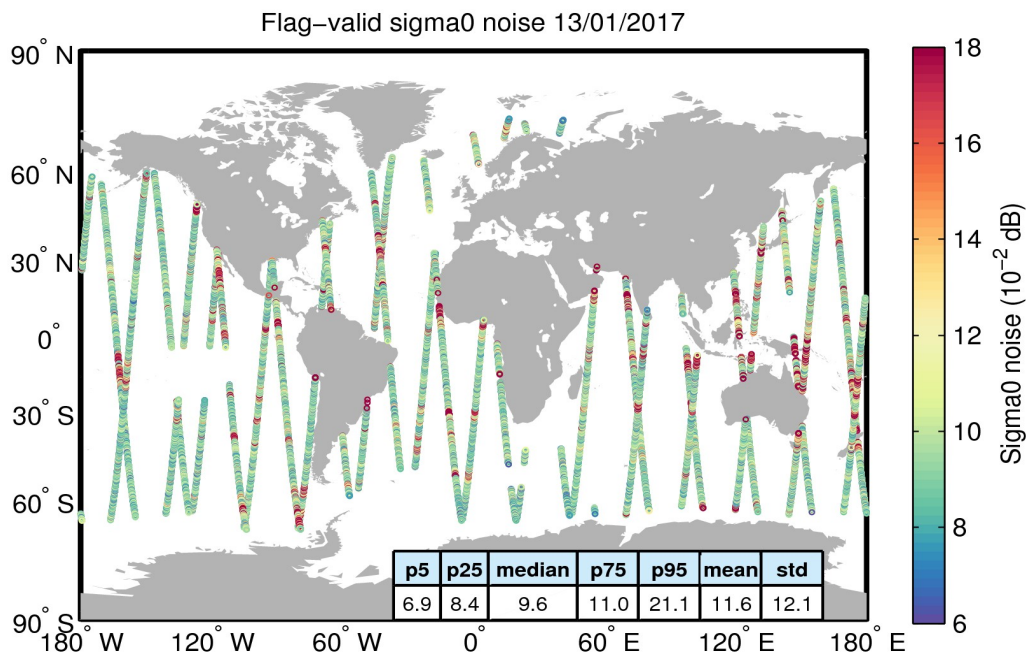
Figure 26. Geographical distribution of flag-valid 20-Hz sigma0 measurement noise over oceans and lakes for 13/01/2017. The statistical values shown in the table refer to the sigma0 noise and are calculated over all measurements shown in the figure.
