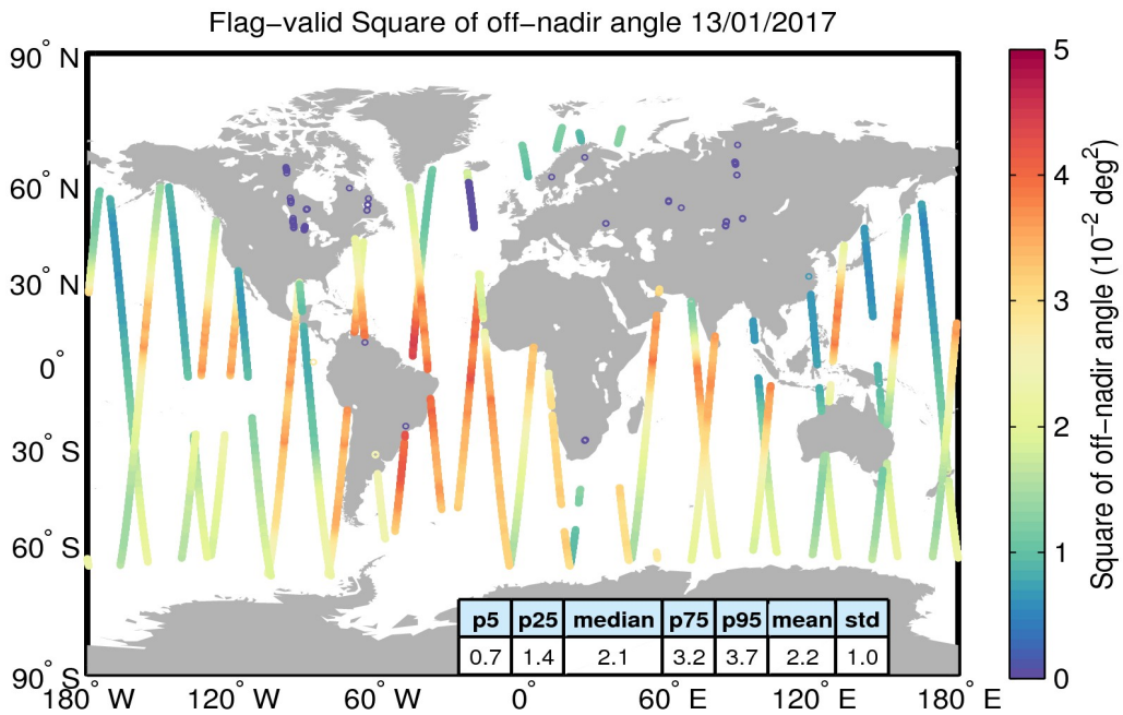
Figure 37. Geographical distribution of flag-valid mispointing data over oceans and lakes for 13/01/2017. The statistical values shown in the table refer to the mispointing in 10^{-2} deg 2 and are calculated over all measurements shown in the figure.
