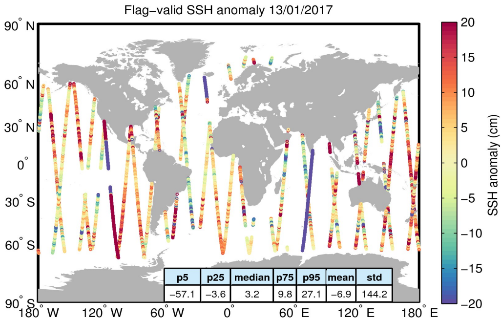
Figure 5. Geographical distribution of flag-valid 1-Hz SSH anomaly data over oceans and lakes for 13/01/2017. The statistical values shown in the table refer to the SSH anomaly in cm and are calculated over all measurements shown in the figure.
