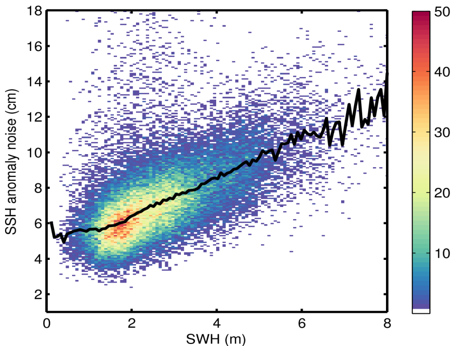
Figure 9. 2D histogram showing flag-valid SSH anomaly noise as a function of SWH for 13/01/2017. The black line denotes the median SSH anomaly noise as a function of SWH.
