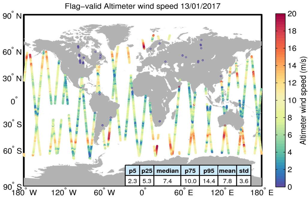
Figure 31. Geographical distribution of flag-valid wind data over oceans and lakes for 13/01/2017. The statistical values shown in the table refer to the wind in m/s and are calculated over all measurements shown in the figure.
