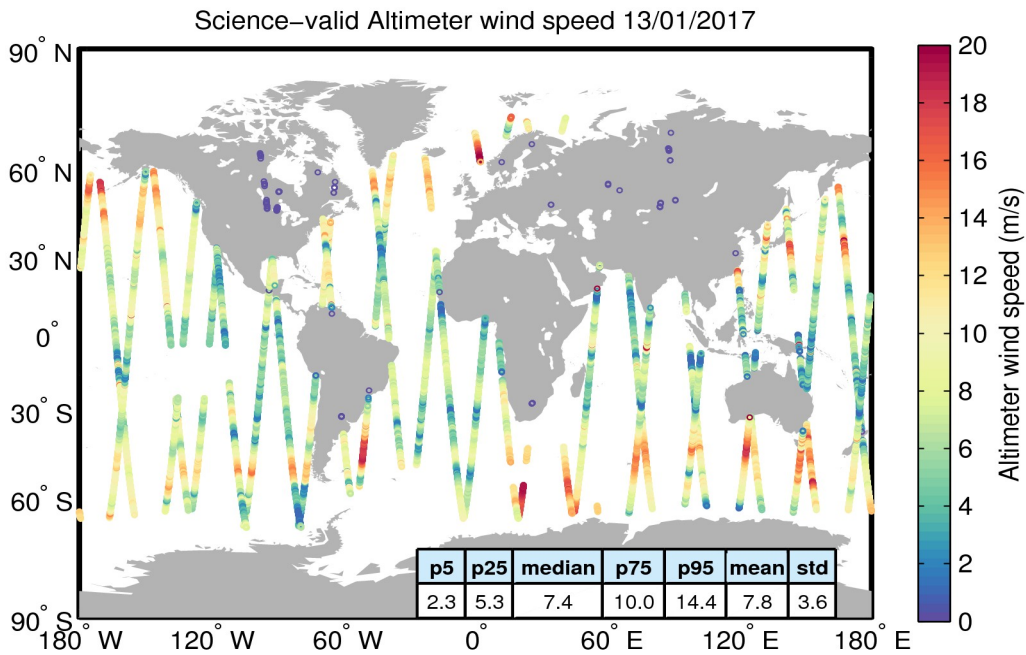
Figure 34. Geographical distribution of science-valid wind data over oceans and lakes for 13/01/2017. The statistical values shown in the table refer to the wind in m/s and are calculated over all measurements shown in the figure. Gray circles denote records that have been rejected based on the editing criteria described in Table 5.
