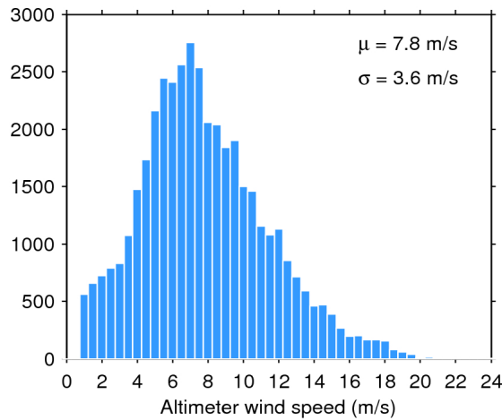
Figure 33. Histogram of flag-valid wind over oceans and lakes for 13/01/2017. The mean ( \mu ) and standard deviation ( \sigma ) are also shown. Note that values larger than 24 m/s are excluded from the histogram for the sake of readability but not from the computation of \mu and \sigma .
