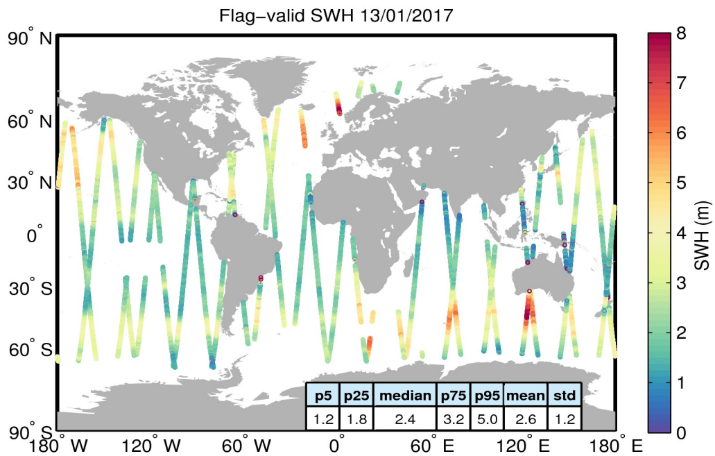
Figure 15. Geographical distribution of flag-valid SWH data over oceans and lakes for 13/01/2017. The statistical values shown in the table refer to the SWH in m and are calculated over all measurements shown in the figure.
