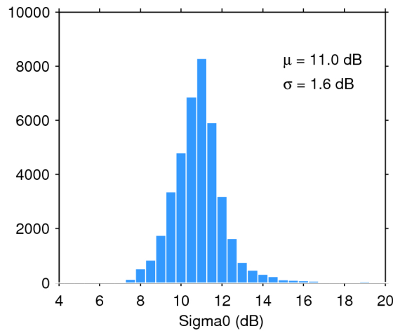
Figure 28. Histogram of science-valid sigma0 over oceans and lakes for 13/01/2017. The mean ( \mu ) and standard deviation ( \sigma ) are also shown. Note that values outside [4 20] dB are excluded from the histogram for the sake of readability but not from the computation of \mu and \sigma .
