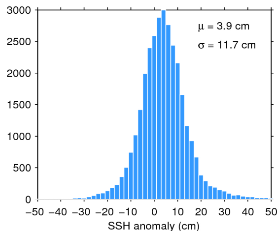
Figure 11. Histogram of science-valid SSH anomaly over oceans and lakes for 13/01/2017. The mean ( \mu ) and standard deviation ( \sigma ) are also shown. Note that values outside [-50 50] cm are excluded from the histogram for the sake of readability but not from the computation of \mu and \sigma .
