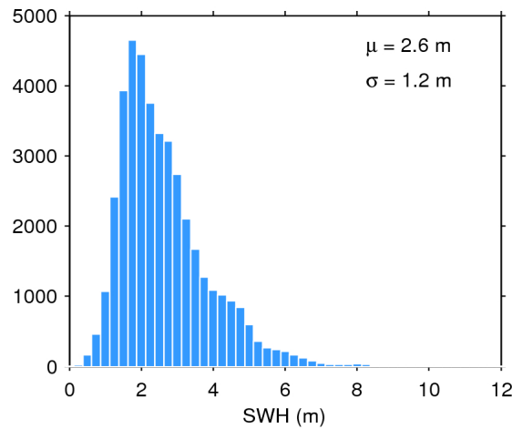
Figure 17. Histogram of flag-valid SWH over oceans and lakes for 13/01/2017. The mean ( \mu ) and standard deviation ( \sigma ) are also shown. Note that values larger than 12 m are excluded from the histogram for the sake of readability but not from the computation of \mu and \sigma .
