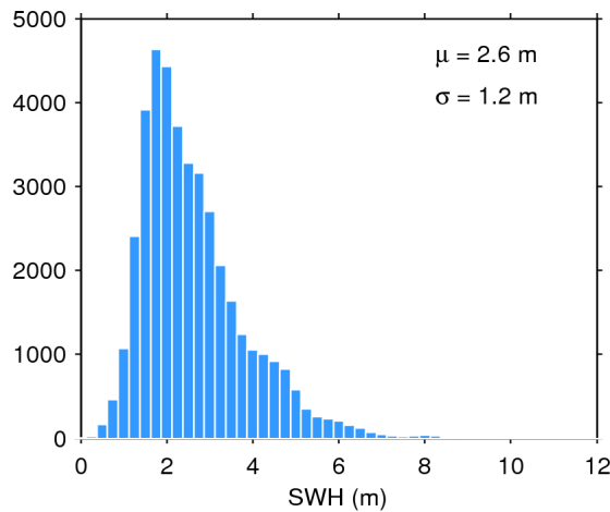
Figure 20. Histogram of science-valid SWH over oceans and lakes for 13/01/2017. The mean ( \mu ) and standard deviation ( \sigma ) are also shown. Note that values larger than 12 m are excluded from the histogram for the sake of readability but not from the computation of \mu and \sigma .
