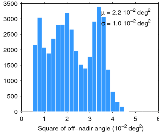
Figure 39. Histogram of flag-valid mispointing over oceans and lakes for 13/01/2017. The mean ( \mu ) and standard deviation ( \sigma ) are also shown. Note that values larger than 6 \cdot 10^{-2} \text{ deg}^2 are excluded from the histogram for the sake of readability but not from the computation of \mu and \sigma .
