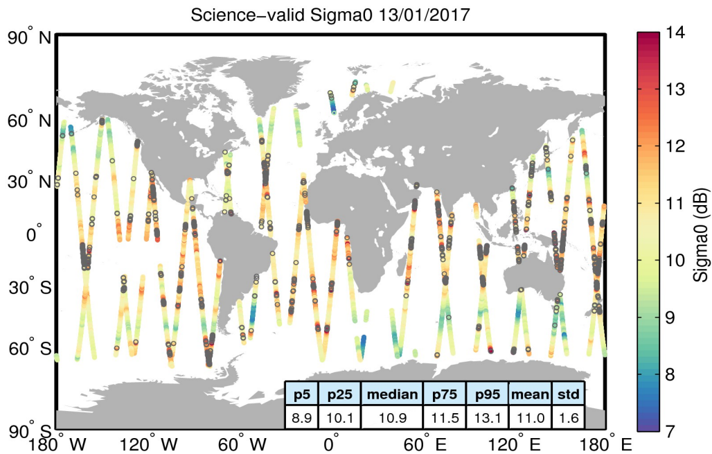
Figure 27. Geographical distribution of science-valid sigma0 data over oceans and lakes for 13/01/2017. The statistical values shown in the table refer to the sigma0 in dB and are calculated over all measurements shown in the figure. Gray circles denote records that have been rejected based on the editing criteria described in Table 4.
