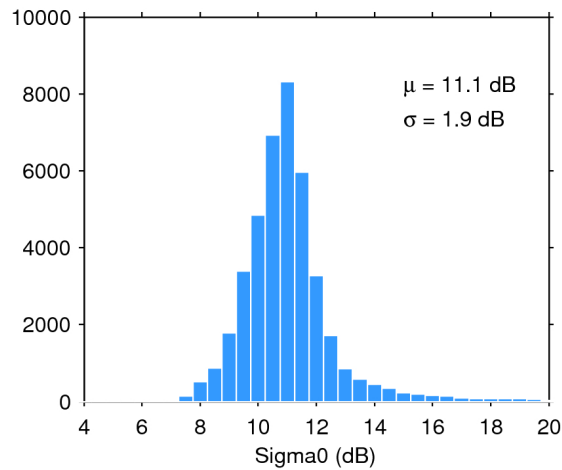
Figure 25. Histogram of flag-valid sigma0 over oceans and lakes for 13/01/2017. The mean ( \mu ) and standard deviation ( \sigma ) are also shown. Note that values outside [4 20] dB are excluded from the histogram for the sake of readability but not from the computation of \mu and \sigma .
