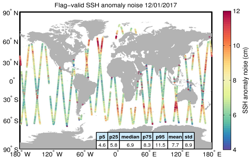
Figure 8. Geographical distribution of flag-valid 20-Hz SSH anomaly measurement noise over oceans and lakes for 12/01/2017. The statistical values shown in the table refer to the SSH anomaly noise and are calculated over all measurements shown in the figure.
