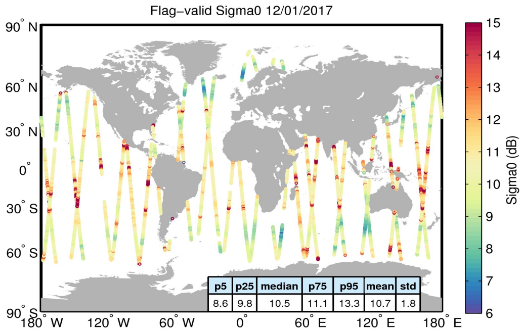
Figure 23. Geographical distribution of flag-valid sigma0 data over oceans and lakes for 12/01/2017. The statistical values shown in the table refer to the sigma0 in dB and are calculated over all measurements shown in the figure.
