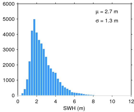
Figure 17. Histogram of flag-valid SWH over oceans and lakes for 12/01/2017. The mean ( \mu ) and standard deviation ( \sigma ) are also shown. Note that values larger than 12 m are excluded from the histogram for the sake of readability but not from the computation of \mu and \sigma .
