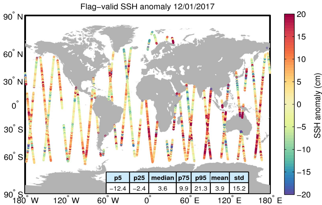
Figure 5. Geographical distribution of flag-valid 1-Hz SSH anomaly data over oceans and lakes for 12/01/2017. The statistical values shown in the table refer to the SSH anomaly in cm and are calculated over all measurements shown in the figure.
