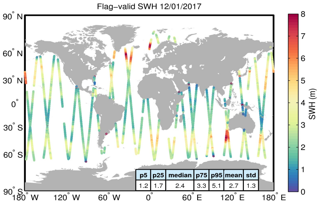
Figure 15. Geographical distribution of flag-valid SWH data over oceans and lakes for 12/01/2017. The statistical values shown in the table refer to the SWH in m and are calculated over all measurements shown in the figure.
