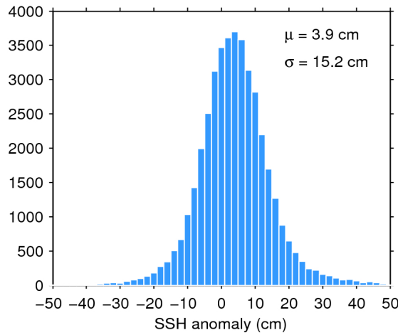
Figure 7. Histogram of flag-valid SSH anomaly over oceans and lakes for 12/01/2017. The mean ( \mu ) and standard deviation ( \sigma ) are also shown. Note that values outside [-50\ 50] cm are excluded from the histogram for the sake of readability but not from the computation of \mu and \sigma .
