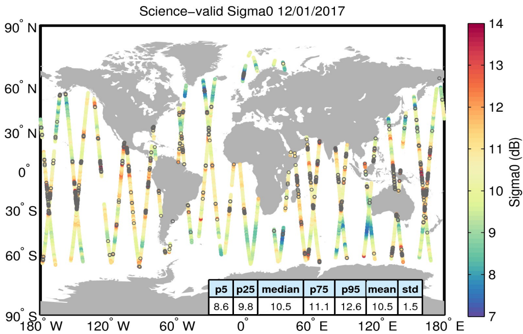
Figure 27. Geographical distribution of science-valid sigma0 data over oceans and lakes for 12/01/2017. The statistical values shown in the table refer to the sigma0 in dB and are calculated over all measurements shown in the figure. Gray circles denote records that have been rejected based on the editing criteria described in Table 4.
