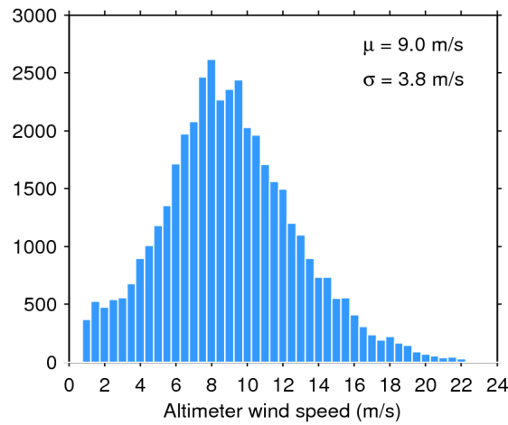
Figure 33. Histogram of flag-valid wind over oceans and lakes for 12/01/2017. The mean ( \mu ) and standard deviation ( \sigma ) are also shown. Note that values larger than 24 m/s are excluded from the histogram for the sake of readability but not from the computation of \mu and \sigma .
