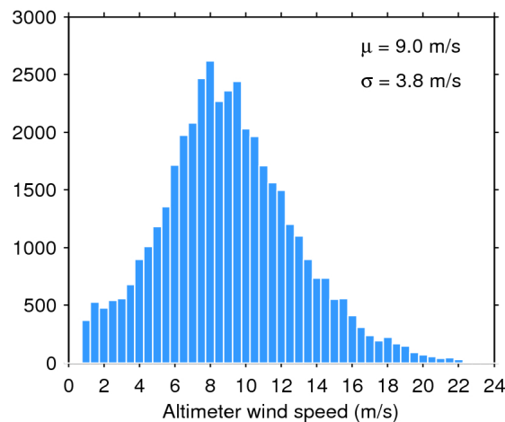
Figure 35. Histogram of science-valid wind over oceans and lakes for 12/01/2017. The mean ( \mu ) and standard deviation ( \sigma ) are also shown. Note that values larger than 24 m/s are excluded from the histogram for the sake of readability but not from the computation of \mu and \sigma .
