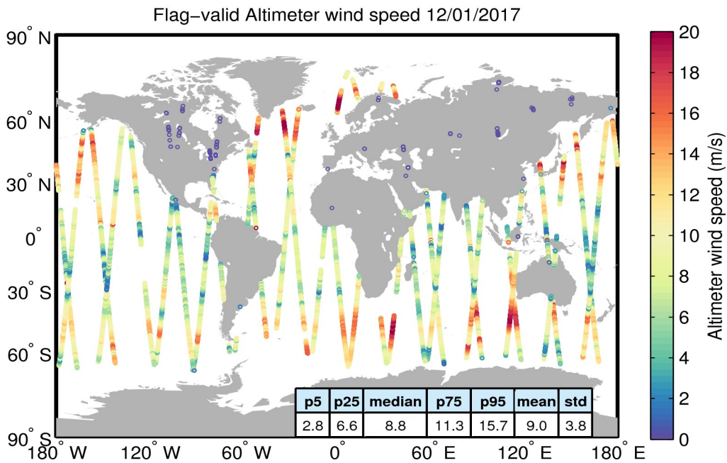
Figure 31. Geographical distribution of flag-valid wind data over oceans and lakes for 12/01/2017. The statistical values shown in the table refer to the wind in m/s and are calculated over all measurements shown in the figure.
