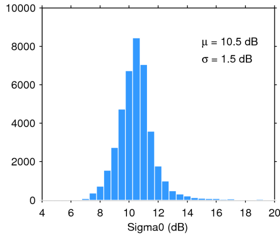
Figure 28. Histogram of science-valid sigma0 over oceans and lakes for 12/01/2017. The mean ( \mu ) and standard deviation ( \sigma ) are also shown. Note that values outside [4 20] dB are excluded from the histogram for the sake of readability but not from the computation of \mu and \sigma .
