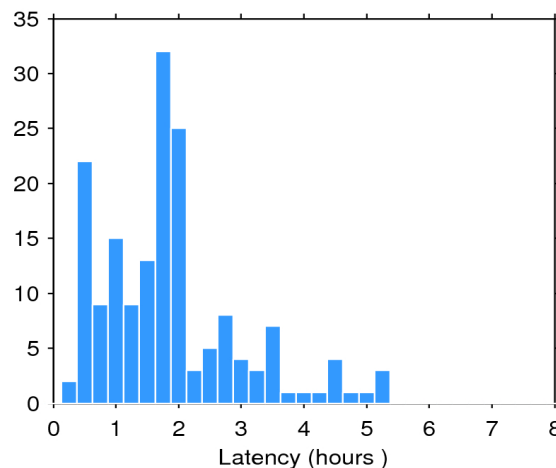
Figure 2. Histogram of the data latency for 12/01/2017. The y-axis denotes the number of files that are made available with a delay of x-hours with respect to the mean time of the records stored in the file.
