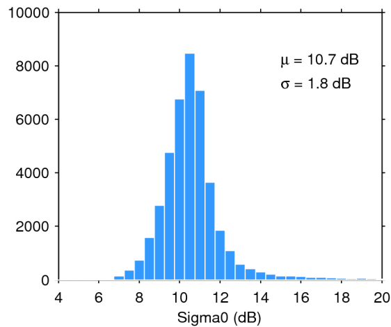
Figure 25. Histogram of flag-valid sigma0 over oceans and lakes for 12/01/2017. The mean ( \mu ) and standard deviation ( \sigma ) are also shown. Note that values outside [4 20] dB are excluded from the histogram for the sake of readability but not from the computation of \mu and \sigma .
