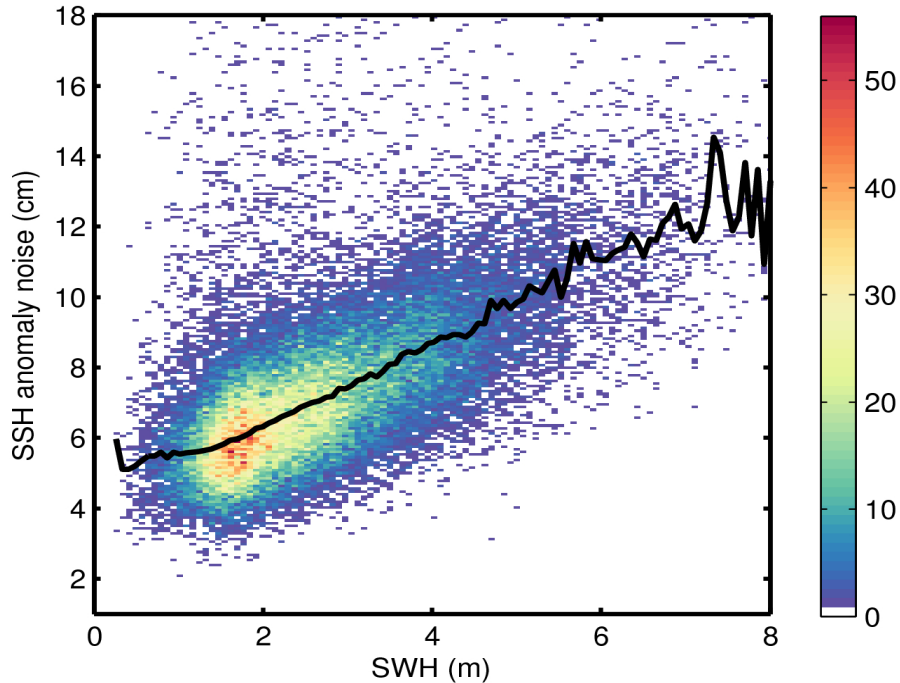
Figure 9. 2D histogram showing flag-valid SSH anomaly noise as a function of SWH for 12/01/2017. The black line denotes the median SSH anomaly noise as a function of SWH.
