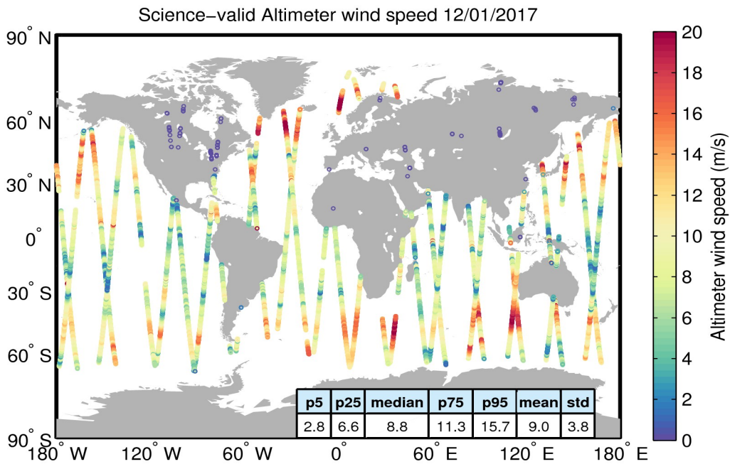
Figure 34. Geographical distribution of science-valid wind data over oceans and lakes for 12/01/2017. The statistical values shown in the table refer to the wind in m/s and are calculated over all measurements shown in the figure. Gray circles denote records that have been rejected based on the editing criteria described in Table 5.
