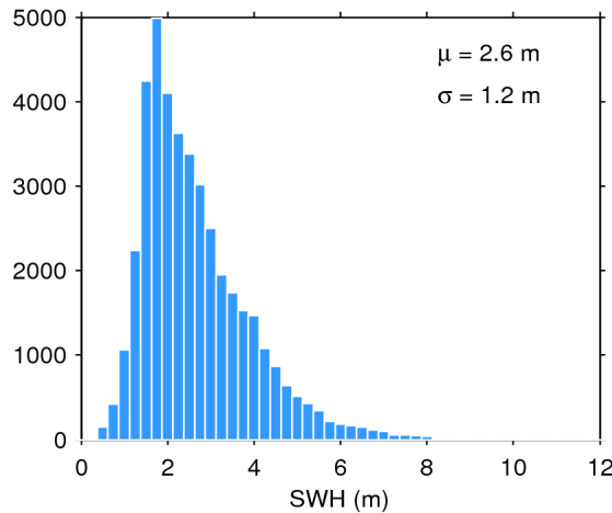
Figure 20. Histogram of science-valid SWH over oceans and lakes for 12/01/2017. The mean ( \mu ) and standard deviation ( \sigma ) are also shown. Note that values larger than 12 m are excluded from the histogram for the sake of readability but not from the computation of \mu and \sigma .
