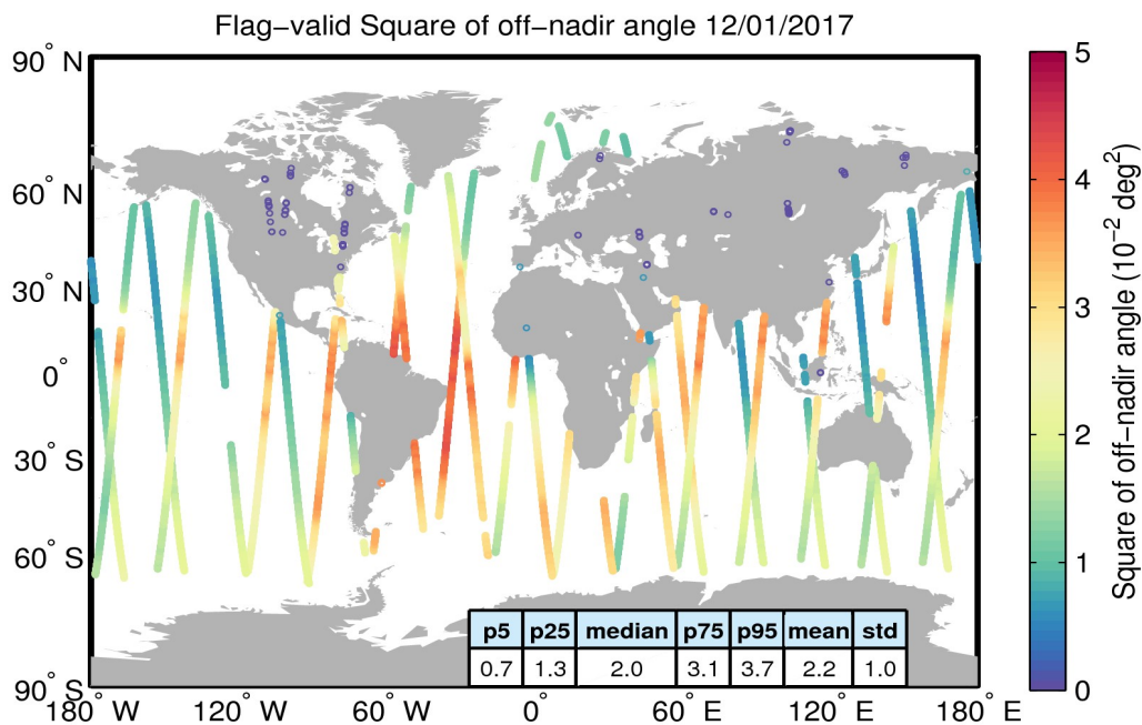
Figure 37. Geographical distribution of flag-valid mispointing data over oceans and lakes for 12/01/2017. The statistical values shown in the table refer to the mispointing in 10^{-2} deg 2 and are calculated over all measurements shown in the figure.
