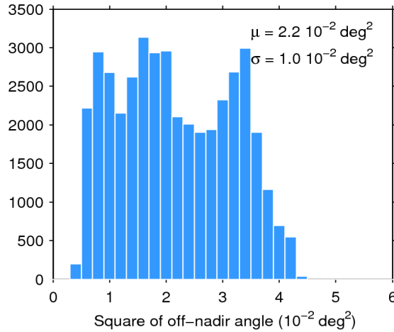
Figure 39. Histogram of flag-valid mispointing over oceans and lakes for 12/01/2017. The mean ( \mu ) and standard deviation ( \sigma ) are also shown. Note that values larger than 6 \cdot 10^{-2} \text{ deg}^2 are excluded from the histogram for the sake of readability but not from the computation of \mu and \sigma .
