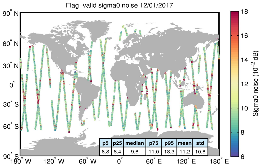
Figure 26. Geographical distribution of flag-valid 20-Hz sigma0 measurement noise over oceans and lakes for 12/01/2017. The statistical values shown in the table refer to the sigma0 noise and are calculated over all measurements shown in the figure.
