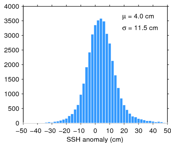
Figure 11. Histogram of science-valid SSH anomaly over oceans and lakes for 12/01/2017. The mean ( \mu ) and standard deviation ( \sigma ) are also shown. Note that values outside [-50 50] cm are excluded from the histogram for the sake of readability but not from the computation of \mu and \sigma .
