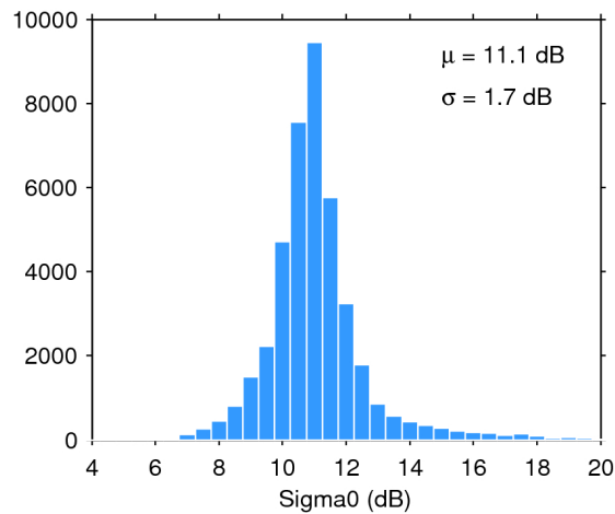
Figure 25. Histogram of flag-valid sigma0 over oceans and lakes for 11/01/2017. The mean ( \mu ) and standard deviation ( \sigma ) are also shown. Note that values outside [4 20] dB are excluded from the histogram for the sake of readability but not from the computation of \mu and \sigma .
