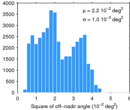
Figure 39. Histogram of flag-valid mispointing over oceans and lakes for 11/01/2017. The mean ( \mu ) and standard deviation ( \sigma ) are also shown. Note that values larger than 6 \cdot 10^{-2} \text{ deg}^2 are excluded from the histogram for the sake of readability but not from the computation of \mu and \sigma .
