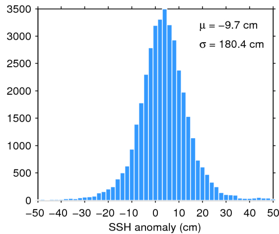
Figure 7. Histogram of flag-valid SSH anomaly over oceans and lakes for 11/01/2017. The mean ( \mu ) and standard deviation ( \sigma ) are also shown. Note that values outside [-50 50] cm are excluded from the histogram for the sake of readability but not from the computation of \mu and \sigma .
