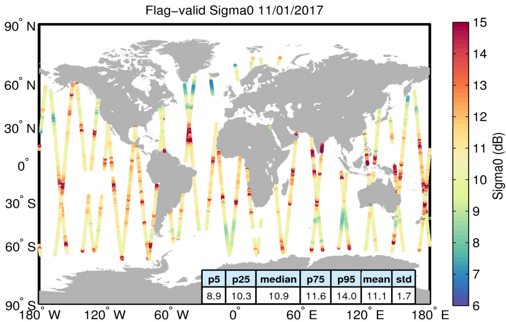
Figure 23. Geographical distribution of flag-valid sigma0 data over oceans and lakes for 11/01/2017. The statistical values shown in the table refer to the sigma0 in dB and are calculated over all measurements shown in the figure.
