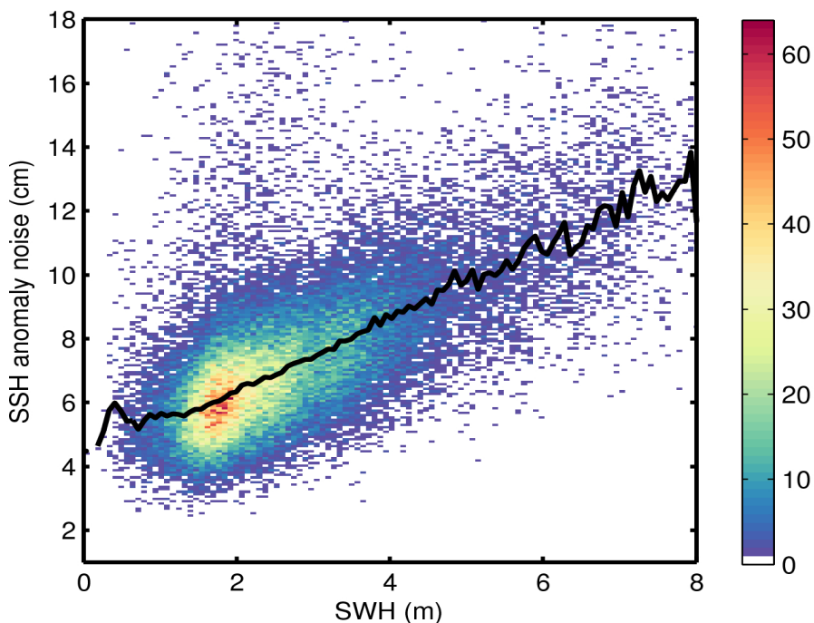
Figure 9. 2D histogram showing flag-valid SSH anomaly noise as a function of SWH for 11/01/2017. The black line denotes the median SSH anomaly noise as a function of SWH.
