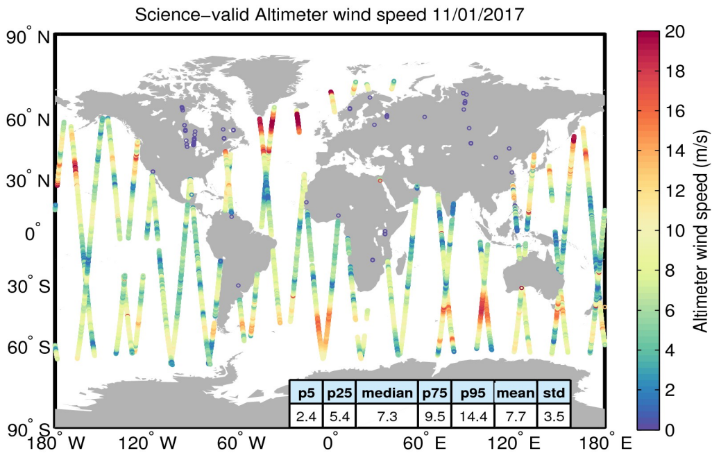
Figure 34. Geographical distribution of science-valid wind data over oceans and lakes for 11/01/2017. The statistical values shown in the table refer to the wind in m/s and are calculated over all measurements shown in the figure. Gray circles denote records that have been rejected based on the editing criteria described in Table 5.
