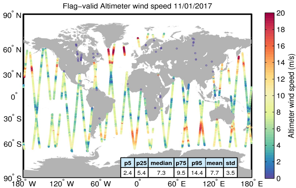
Figure 31. Geographical distribution of flag-valid wind data over oceans and lakes for 11/01/2017. The statistical values shown in the table refer to the wind in m/s and are calculated over all measurements shown in the figure.
