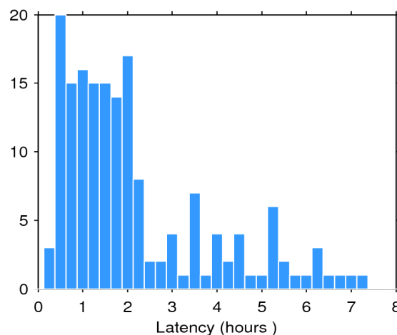
Figure 2. Histogram of the data latency for 11/01/2017. The y-axis denotes the number of files that are made available with a delay of x-hours with respect to the mean time of the records stored in the file.
