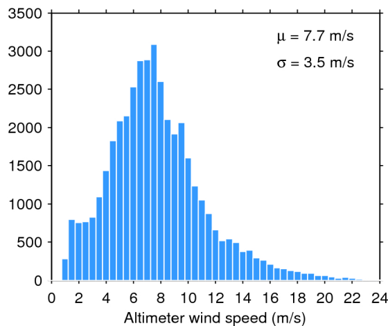
Figure 35. Histogram of science-valid wind over oceans and lakes for 11/01/2017. The mean ( \mu ) and standard deviation ( \sigma ) are also shown. Note that values larger than 24 m/s are excluded from the histogram for the sake of readability but not from the computation of \mu and \sigma .
