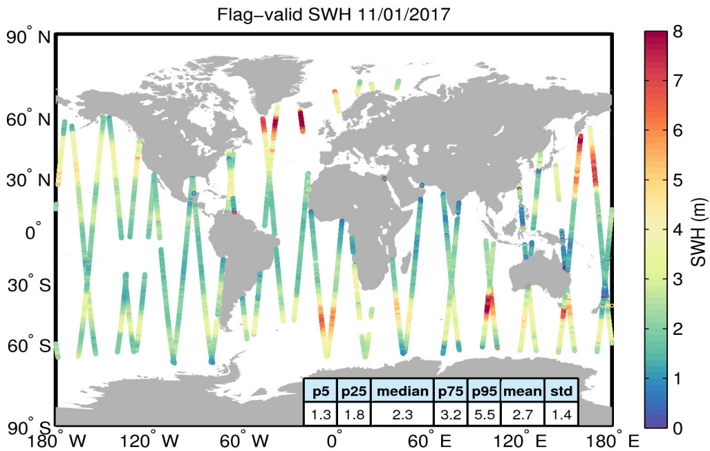
Figure 15. Geographical distribution of flag-valid SWH data over oceans and lakes for 11/01/2017. The statistical values shown in the table refer to the SWH in m and are calculated over all measurements shown in the figure.
