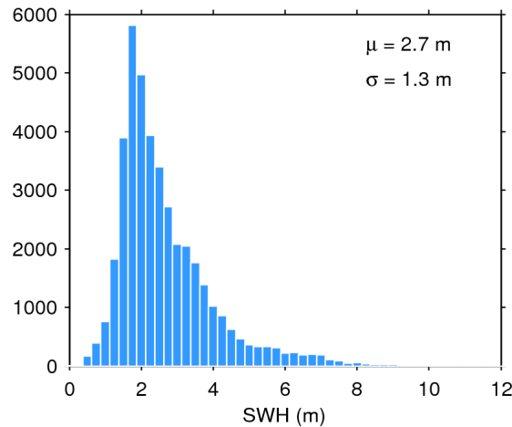
Figure 20. Histogram of science-valid SWH over oceans and lakes for 11/01/2017. The mean ( \mu ) and standard deviation ( \sigma ) are also shown. Note that values larger than 12 m are excluded from the histogram for the sake of readability but not from the computation of \mu and \sigma .
