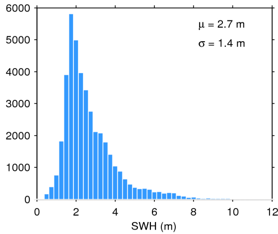
Figure 17. Histogram of flag-valid SWH over oceans and lakes for 11/01/2017. The mean ( \mu ) and standard deviation ( \sigma ) are also shown. Note that values larger than 12 m are excluded from the histogram for the sake of readability but not from the computation of \mu and \sigma .
