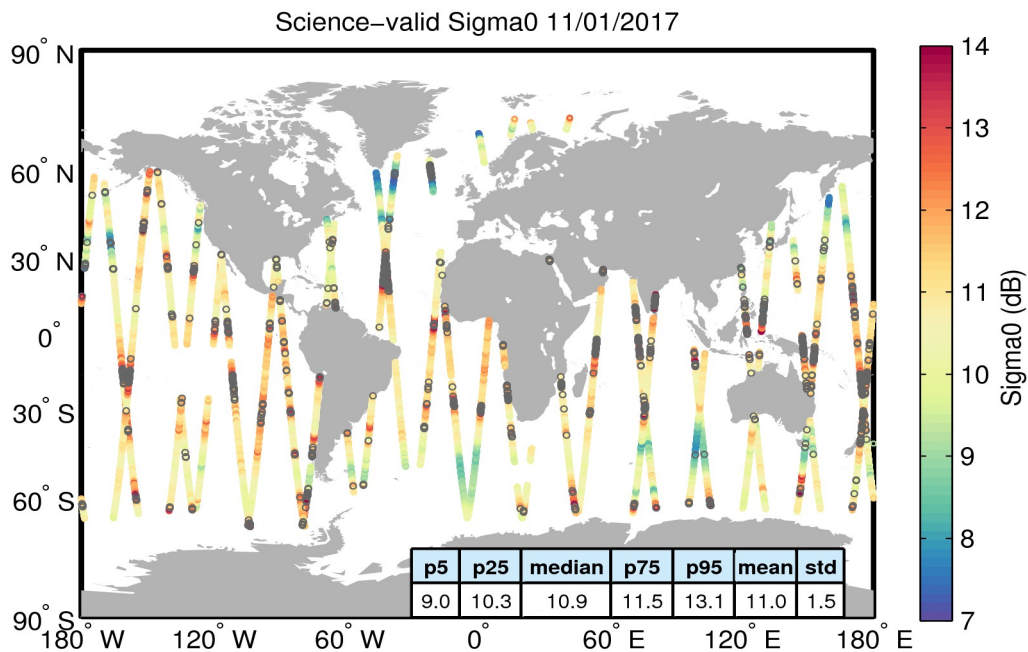
Figure 27. Geographical distribution of science-valid sigma0 data over oceans and lakes for 11/01/2017. The statistical values shown in the table refer to the sigma0 in dB and are calculated over all measurements shown in the figure. Gray circles denote records that have been rejected based on the editing criteria described in Table 4.
