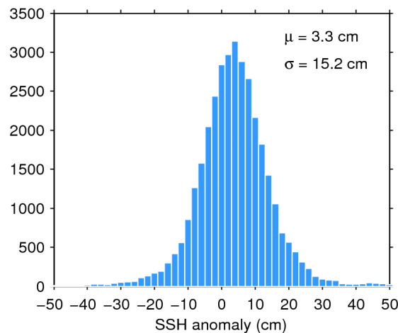
Figure 11. Histogram of science-valid SSH anomaly over oceans and lakes for 11/01/2017. The mean ( \mu ) and standard deviation ( \sigma ) are also shown. Note that values outside [-50 50] cm are excluded from the histogram for the sake of readability but not from the computation of \mu and \sigma .
