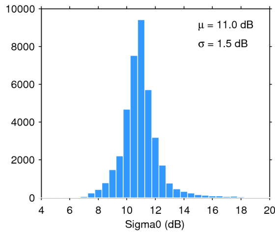
Figure 28. Histogram of science-valid sigma0 over oceans and lakes for 11/01/2017. The mean ( \mu ) and standard deviation ( \sigma ) are also shown. Note that values outside [4 20] dB are excluded from the histogram for the sake of readability but not from the computation of \mu and \sigma .
