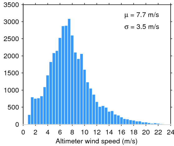
Figure 33. Histogram of flag-valid wind over oceans and lakes for 11/01/2017. The mean ( \mu ) and standard deviation ( \sigma ) are also shown. Note that values larger than 24 m/s are excluded from the histogram for the sake of readability but not from the computation of \mu and \sigma .
