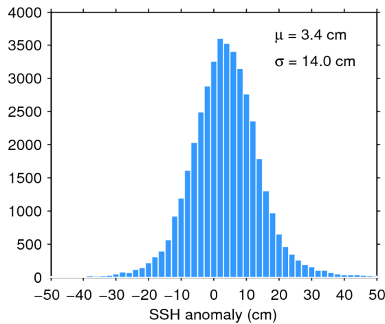
Figure 7. Histogram of flag-valid SSH anomaly over oceans and lakes for 10/01/2017. The mean ( \mu ) and standard deviation ( \sigma ) are also shown. Note that values outside [-50 50] cm are excluded from the histogram for the sake of readability but not from the computation of \mu and \sigma .
