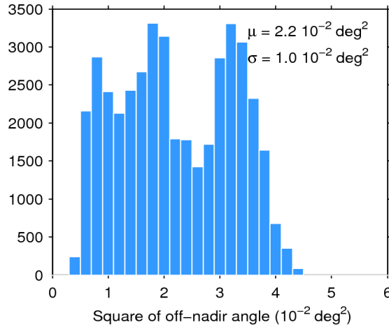
Figure 39. Histogram of flag-valid mispointing over oceans and lakes for 10/01/2017. The mean ( \mu ) and standard deviation ( \sigma ) are also shown. Note that values larger than 6 \cdot 10^{-2} \text{ deg}^2 are excluded from the histogram for the sake of readability but not from the computation of \mu and \sigma .
