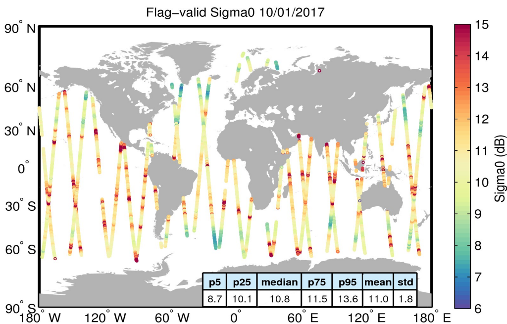
Figure 23. Geographical distribution of flag-valid sigma0 data over oceans and lakes for 10/01/2017. The statistical values shown in the table refer to the sigma0 in dB and are calculated over all measurements shown in the figure.
