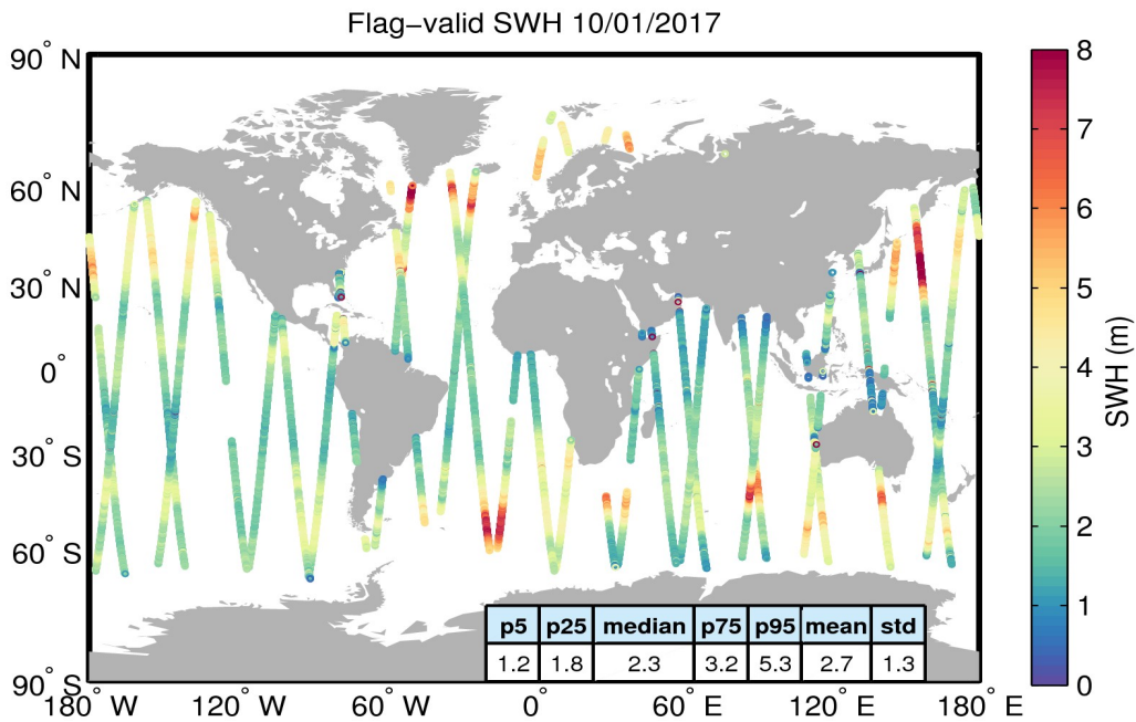
Figure 15. Geographical distribution of flag-valid SWH data over oceans and lakes for 10/01/2017. The statistical values shown in the table refer to the SWH in m and are calculated over all measurements shown in the figure.
