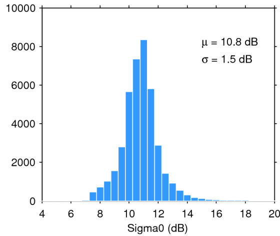
Figure 28. Histogram of science-valid sigma0 over oceans and lakes for 10/01/2017. The mean ( \mu ) and standard deviation ( \sigma ) are also shown. Note that values outside [4 20] dB are excluded from the histogram for the sake of readability but not from the computation of \mu and \sigma .
