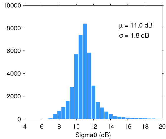
Figure 25. Histogram of flag-valid sigma0 over oceans and lakes for 10/01/2017. The mean ( \mu ) and standard deviation ( \sigma ) are also shown. Note that values outside [4 20] dB are excluded from the histogram for the sake of readability but not from the computation of \mu and \sigma .
