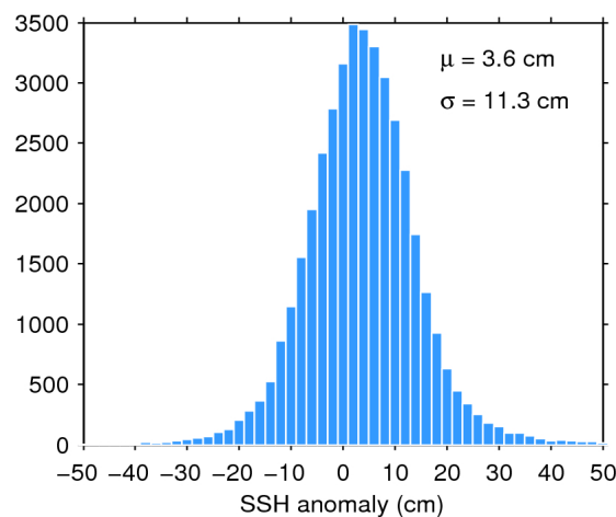
Figure 11. Histogram of science-valid SSH anomaly over oceans and lakes for 10/01/2017. The mean ( \mu ) and standard deviation ( \sigma ) are also shown. Note that values outside [-50 50] cm are excluded from the histogram for the sake of readability but not from the computation of \mu and \sigma .
