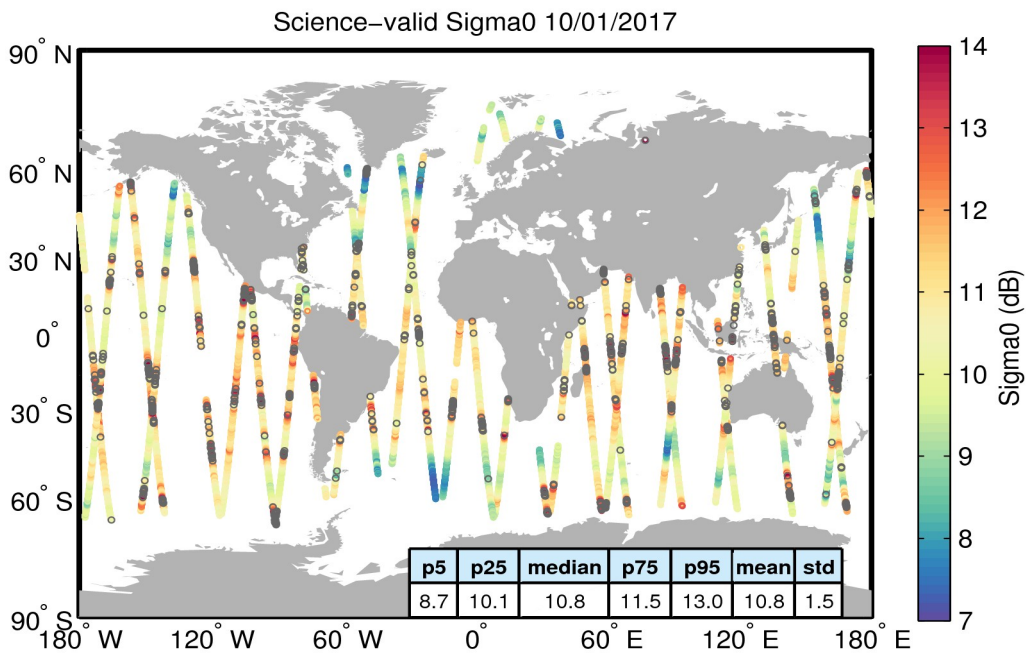
Figure 27. Geographical distribution of science-valid sigma0 data over oceans and lakes for 10/01/2017. The statistical values shown in the table refer to the sigma0 in dB and are calculated over all measurements shown in the figure. Gray circles denote records that have been rejected based on the editing criteria described in Table 4.
