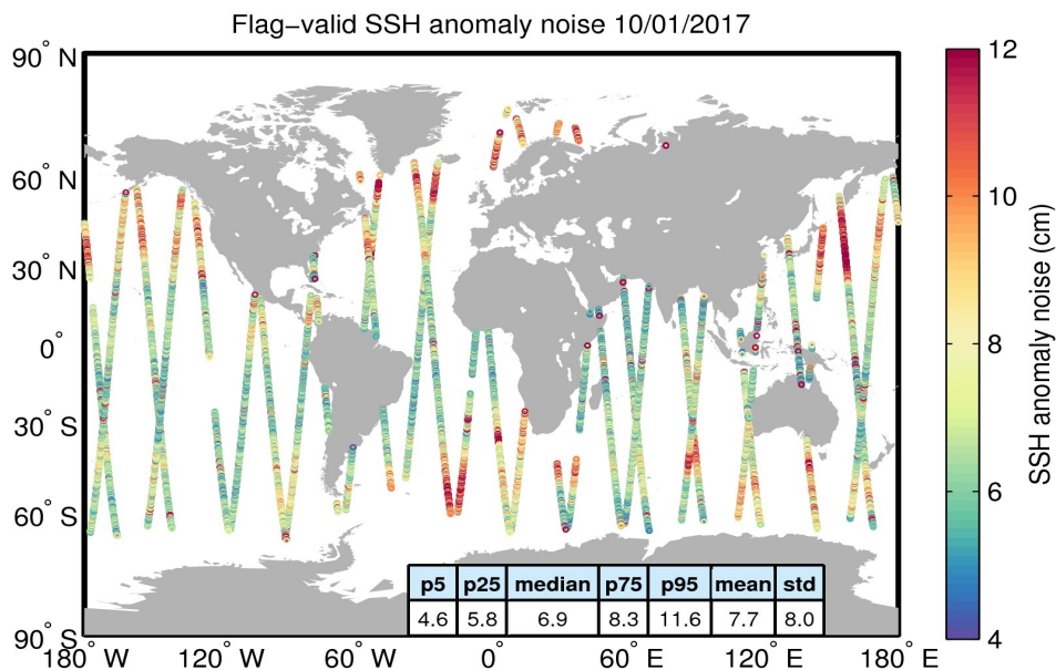
Figure 8. Geographical distribution of flag-valid 20-Hz SSH anomaly measurement noise over oceans and lakes for 10/01/2017. The statistical values shown in the table refer to the SSH anomaly noise and are calculated over all measurements shown in the figure.
