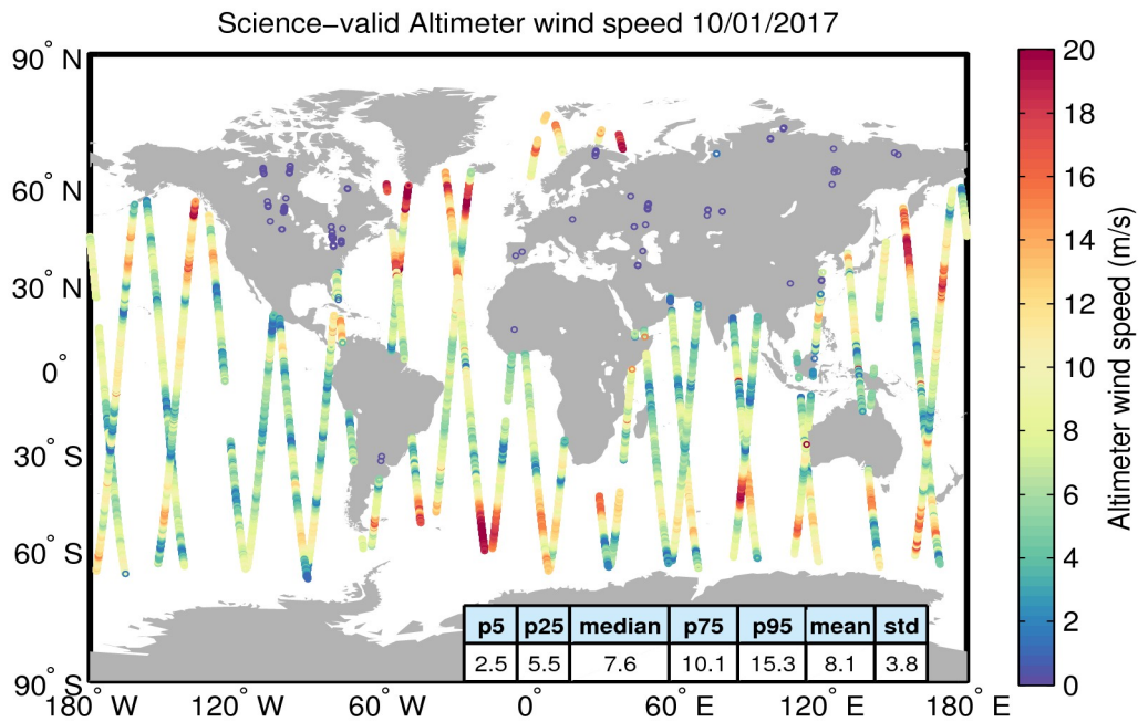
Figure 34. Geographical distribution of science-valid wind data over oceans and lakes for 10/01/2017. The statistical values shown in the table refer to the wind in m/s and are calculated over all measurements shown in the figure. Gray circles denote records that have been rejected based on the editing criteria described in Table 5.
