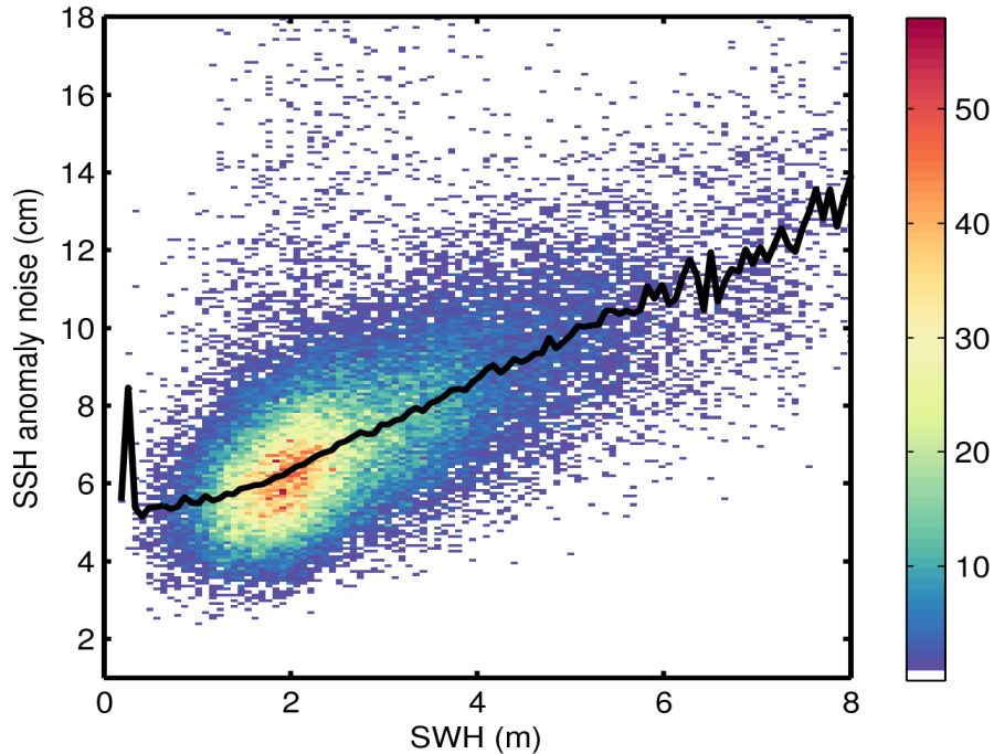
Figure 9. 2D histogram showing flag-valid SSH anomaly noise as a function of SWH for 10/01/2017. The black line denotes the median SSH anomaly noise as a function of SWH.
