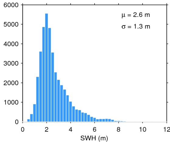
Figure 20. Histogram of science-valid SWH over oceans and lakes for 10/01/2017. The mean ( \mu ) and standard deviation ( \sigma ) are also shown. Note that values larger than 12 m are excluded from the histogram for the sake of readability but not from the computation of \mu and \sigma .
