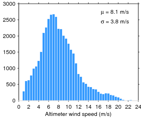
Figure 33. Histogram of flag-valid wind over oceans and lakes for 10/01/2017. The mean ( \mu ) and standard deviation ( \sigma ) are also shown. Note that values larger than 24 m/s are excluded from the histogram for the sake of readability but not from the computation of \mu and \sigma .
