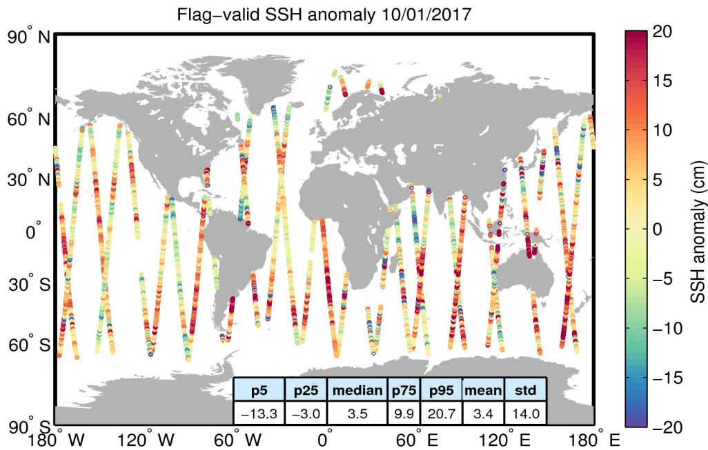
Figure 5. Geographical distribution of flag-valid 1-Hz SSH anomaly data over oceans and lakes for 10/01/2017. The statistical values shown in the table refer to the SSH anomaly in cm and are calculated over all measurements shown in the figure.
