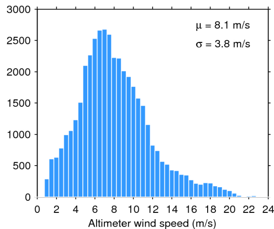
Figure 35. Histogram of science-valid wind over oceans and lakes for 10/01/2017. The mean ( \mu ) and standard deviation ( \sigma ) are also shown. Note that values larger than 24 m/s are excluded from the histogram for the sake of readability but not from the computation of \mu and \sigma .
