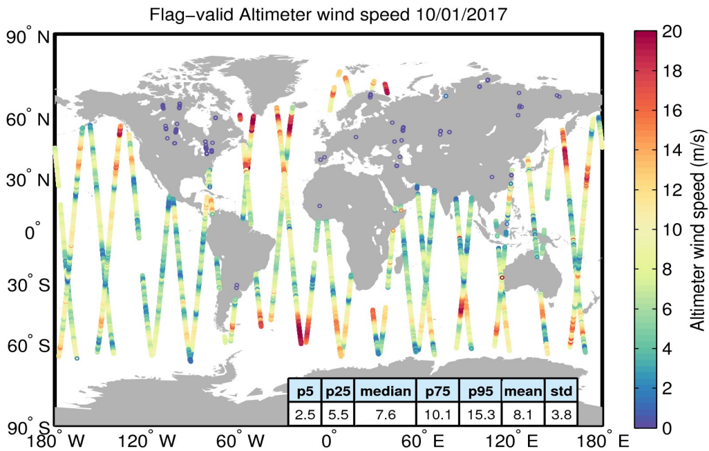
Figure 31. Geographical distribution of flag-valid wind data over oceans and lakes for 10/01/2017. The statistical values shown in the table refer to the wind in m/s and are calculated over all measurements shown in the figure.
