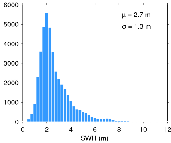
Figure 17. Histogram of flag-valid SWH over oceans and lakes for 10/01/2017. The mean ( \mu ) and standard deviation ( \sigma ) are also shown. Note that values larger than 12 m are excluded from the histogram for the sake of readability but not from the computation of \mu and \sigma .
