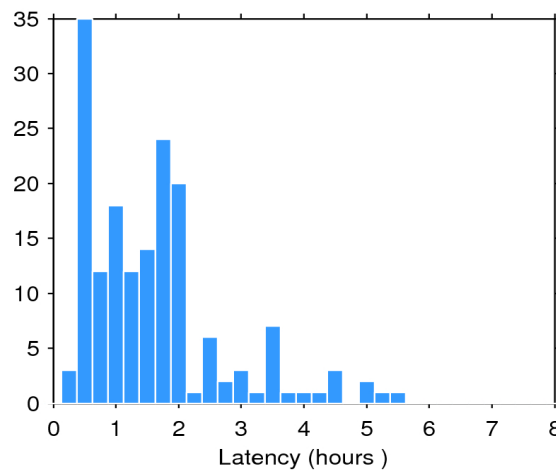
Figure 2. Histogram of the data latency for 10/01/2017. The y-axis denotes the number of files that are made available with a delay of x-hours with respect to the mean time of the records stored in the file.
