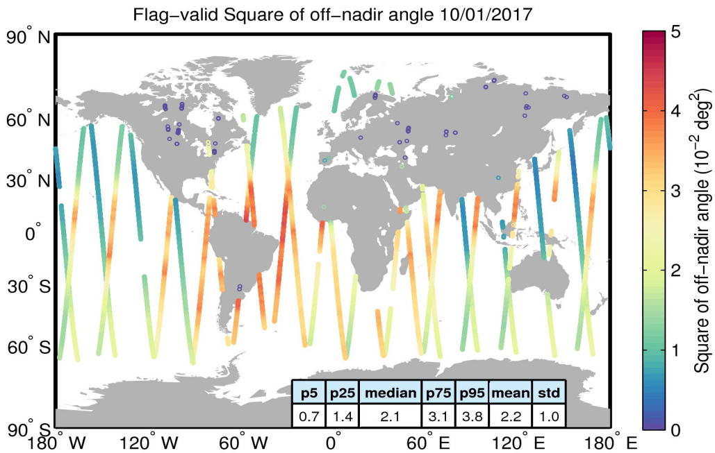
Figure 37. Geographical distribution of flag-valid mispointing data over oceans and lakes for 10/01/2017. The statistical values shown in the table refer to the mispointing in 10^{-2} deg 2 and are calculated over all measurements shown in the figure.
