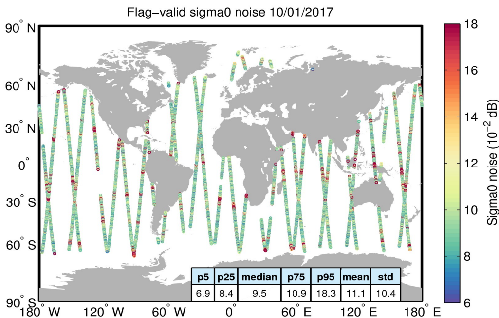
Figure 26. Geographical distribution of flag-valid 20-Hz sigma0 measurement noise over oceans and lakes for 10/01/2017. The statistical values shown in the table refer to the sigma0 noise and are calculated over all measurements shown in the figure.
