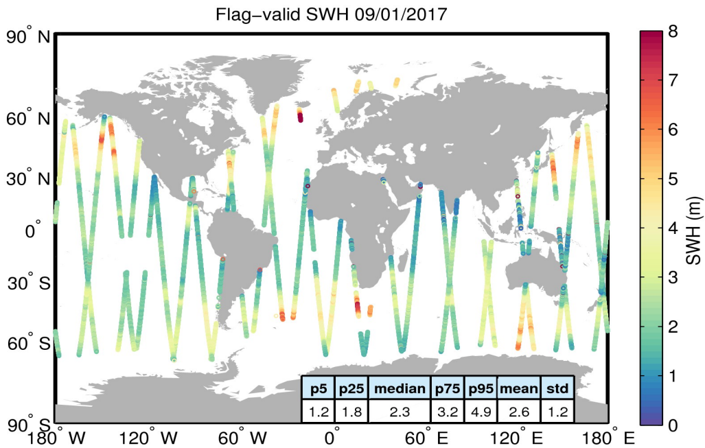
Figure 15. Geographical distribution of flag-valid SWH data over oceans and lakes for 09/01/2017. The statistical values shown in the table refer to the SWH in m and are calculated over all measurements shown in the figure.
