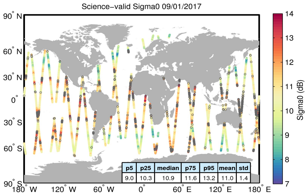
Figure 27. Geographical distribution of science-valid sigma0 data over oceans and lakes for 09/01/2017. The statistical values shown in the table refer to the sigma0 in dB and are calculated over all measurements shown in the figure. Gray circles denote records that have been rejected based on the editing criteria described in Table 4.
