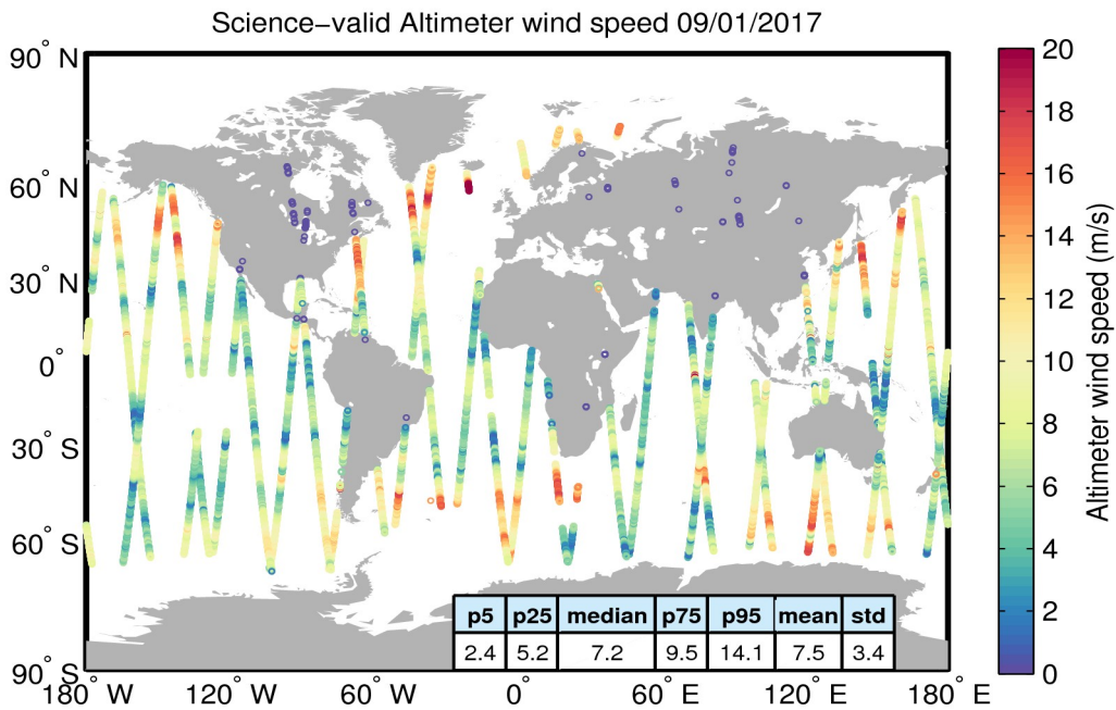
Figure 34. Geographical distribution of science-valid wind data over oceans and lakes for 09/01/2017. The statistical values shown in the table refer to the wind in m/s and are calculated over all measurements shown in the figure. Gray circles denote records that have been rejected based on the editing criteria described in Table 5.
