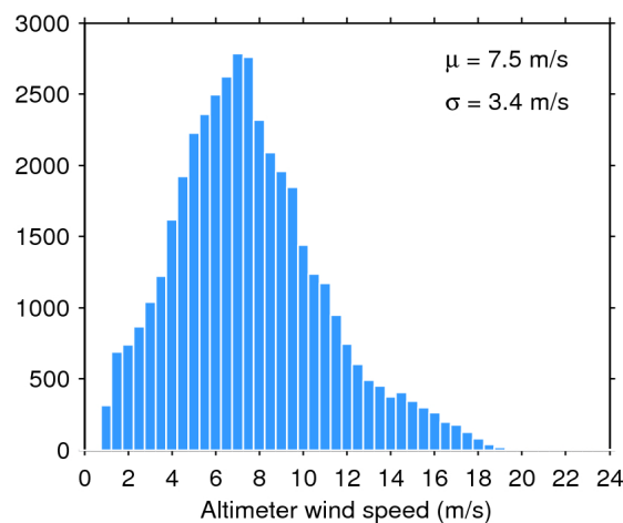
Figure 35. Histogram of science-valid wind over oceans and lakes for 09/01/2017. The mean ( \mu ) and standard deviation ( \sigma ) are also shown. Note that values larger than 24 m/s are excluded from the histogram for the sake of readability but not from the computation of \mu and \sigma .
