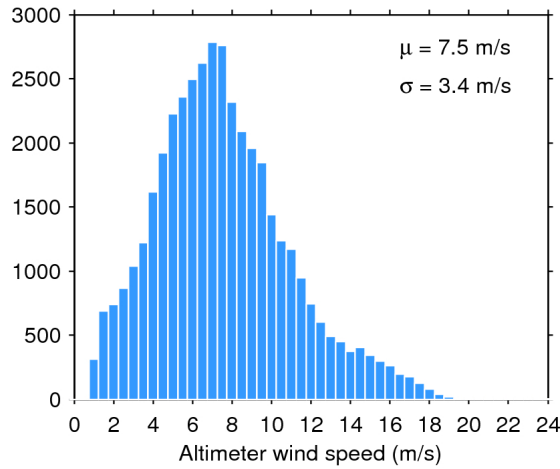
Figure 33. Histogram of flag-valid wind over oceans and lakes for 09/01/2017. The mean ( \mu ) and standard deviation ( \sigma ) are also shown. Note that values larger than 24 m/s are excluded from the histogram for the sake of readability but not from the computation of \mu and \sigma .
