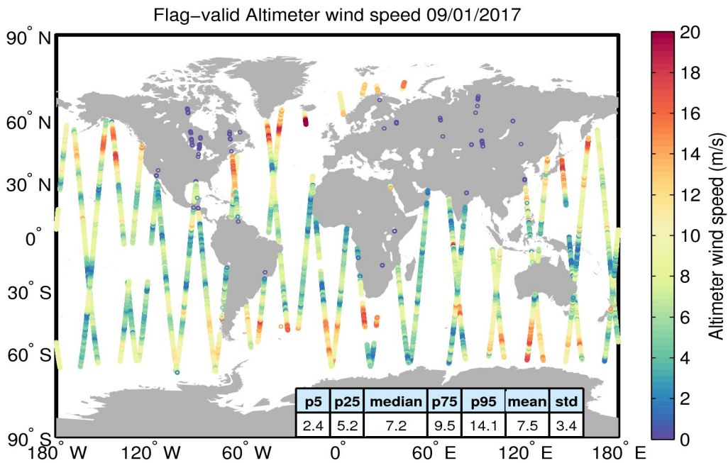
Figure 31. Geographical distribution of flag-valid wind data over oceans and lakes for 09/01/2017. The statistical values shown in the table refer to the wind in m/s and are calculated over all measurements shown in the figure.
