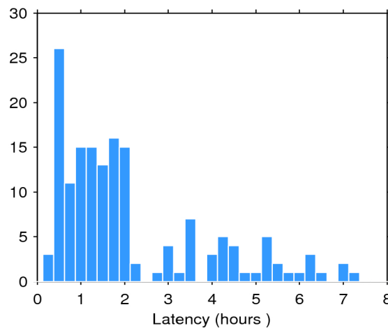
Figure 2. Histogram of the data latency for 09/01/2017. The y-axis denotes the number of files that are made available with a delay of x-hours with respect to the mean time of the records stored in the file.
