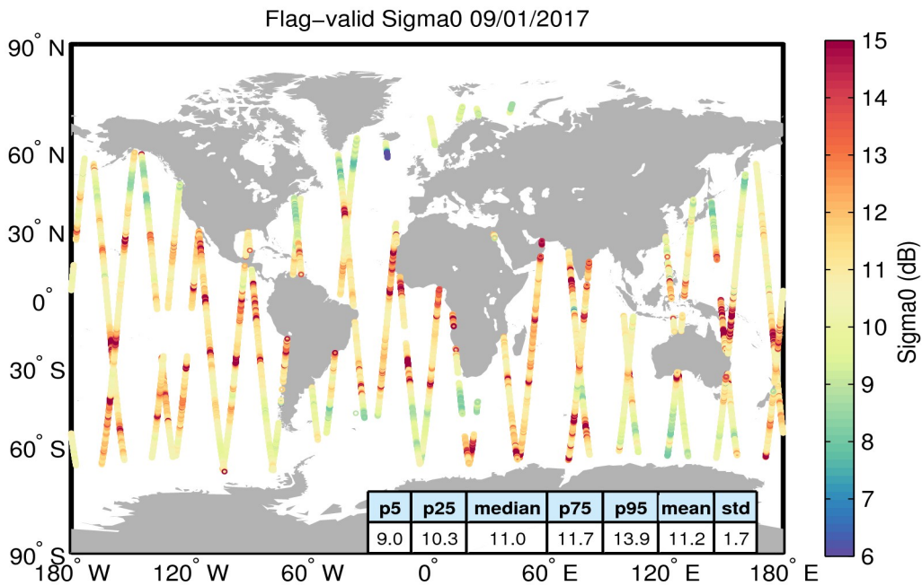
Figure 23. Geographical distribution of flag-valid sigma0 data over oceans and lakes for 09/01/2017. The statistical values shown in the table refer to the sigma0 in dB and are calculated over all measurements shown in the figure.
