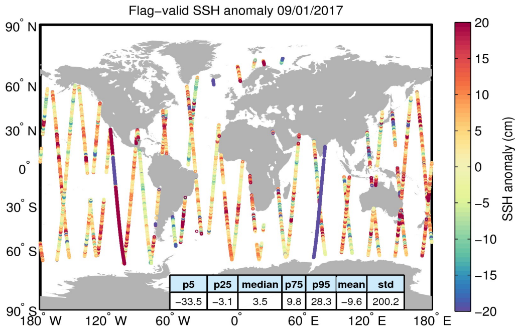
Figure 5. Geographical distribution of flag-valid 1-Hz SSH anomaly data over oceans and lakes for 09/01/2017. The statistical values shown in the table refer to the SSH anomaly in cm and are calculated over all measurements shown in the figure.
