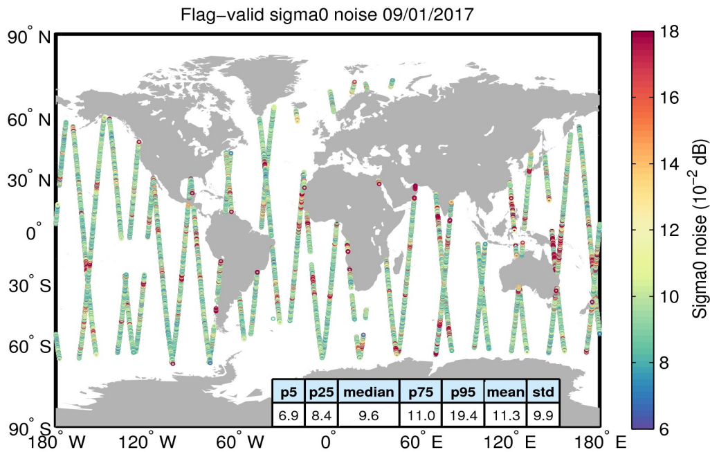
Figure 26. Geographical distribution of flag-valid 20-Hz sigma0 measurement noise over oceans and lakes for 09/01/2017. The statistical values shown in the table refer to the sigma0 noise and are calculated over all measurements shown in the figure.
