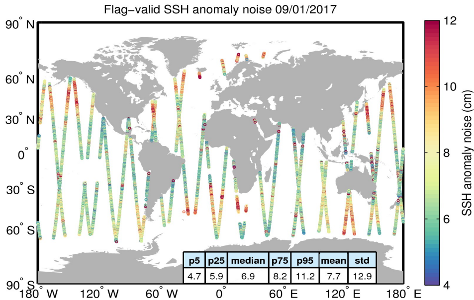
Figure 8. Geographical distribution of flag-valid 20-Hz SSH anomaly measurement noise over oceans and lakes for 09/01/2017. The statistical values shown in the table refer to the SSH anomaly noise and are calculated over all measurements shown in the figure.
