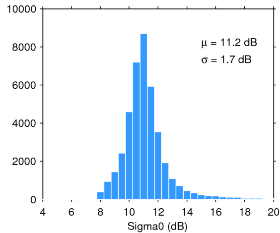
Figure 25. Histogram of flag-valid sigma0 over oceans and lakes for 09/01/2017. The mean ( \mu ) and standard deviation ( \sigma ) are also shown. Note that values outside [4 20] dB are excluded from the histogram for the sake of readability but not from the computation of \mu and \sigma .
