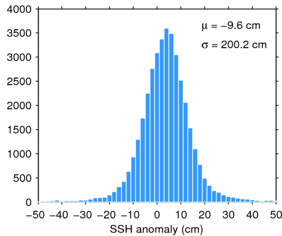
Figure 7. Histogram of flag-valid SSH anomaly over oceans and lakes for 09/01/2017. The mean ( \mu ) and standard deviation ( \sigma ) are also shown. Note that values outside [-50 50] cm are excluded from the histogram for the sake of readability but not from the computation of \mu and \sigma .
