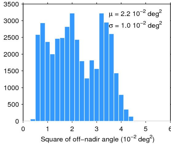
Figure 39. Histogram of flag-valid mispointing over oceans and lakes for 09/01/2017. The mean ( \mu ) and standard deviation ( \sigma ) are also shown. Note that values larger than 6 \cdot 10^{-2} \text{ deg}^2 are excluded from the histogram for the sake of readability but not from the computation of \mu and \sigma .
