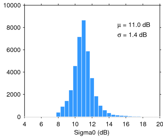
Figure 28. Histogram of science-valid sigma0 over oceans and lakes for 09/01/2017. The mean ( \mu ) and standard deviation ( \sigma ) are also shown. Note that values outside [4 20] dB are excluded from the histogram for the sake of readability but not from the computation of \mu and \sigma .
