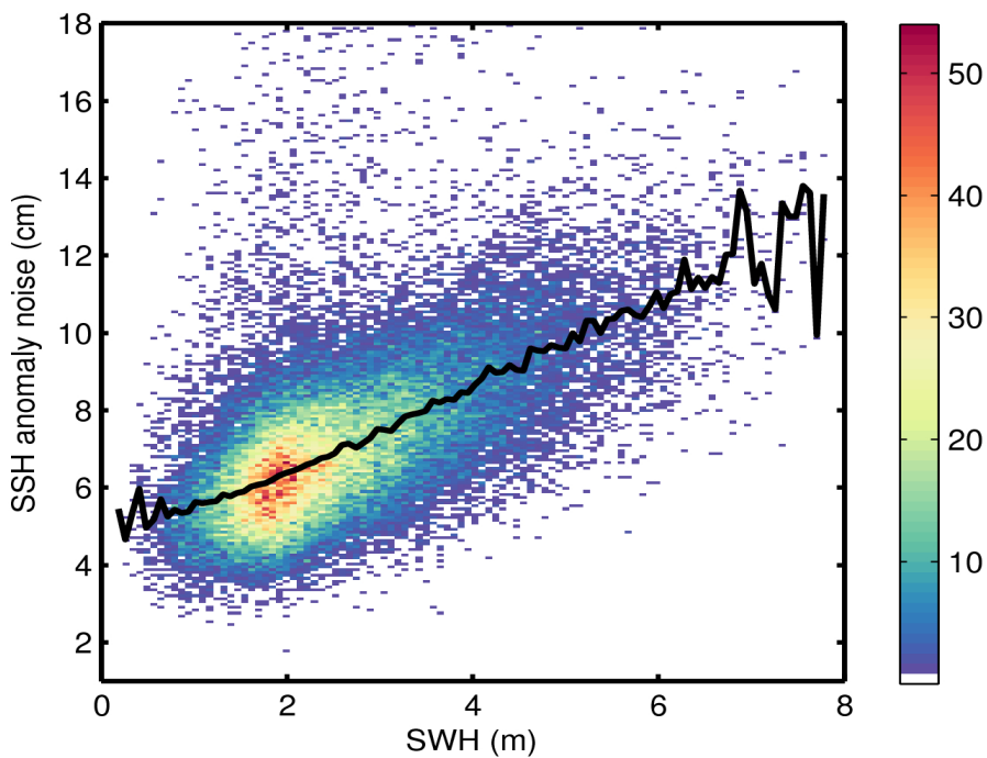
Figure 9. 2D histogram showing flag-valid SSH anomaly noise as a function of SWH for 09/01/2017. The black line denotes the median SSH anomaly noise as a function of SWH.
