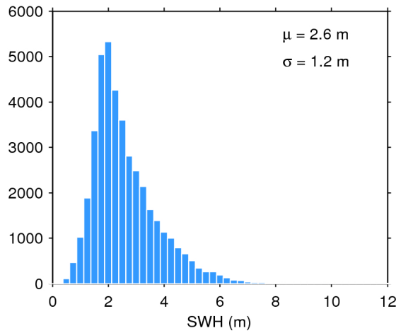
Figure 17. Histogram of flag-valid SWH over oceans and lakes for 09/01/2017. The mean ( \mu ) and standard deviation ( \sigma ) are also shown. Note that values larger than 12 m are excluded from the histogram for the sake of readability but not from the computation of \mu and \sigma .
