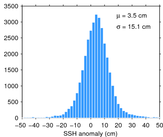
Figure 11. Histogram of science-valid SSH anomaly over oceans and lakes for 09/01/2017. The mean ( \mu ) and standard deviation ( \sigma ) are also shown. Note that values outside [-50 50] cm are excluded from the histogram for the sake of readability but not from the computation of \mu and \sigma .
