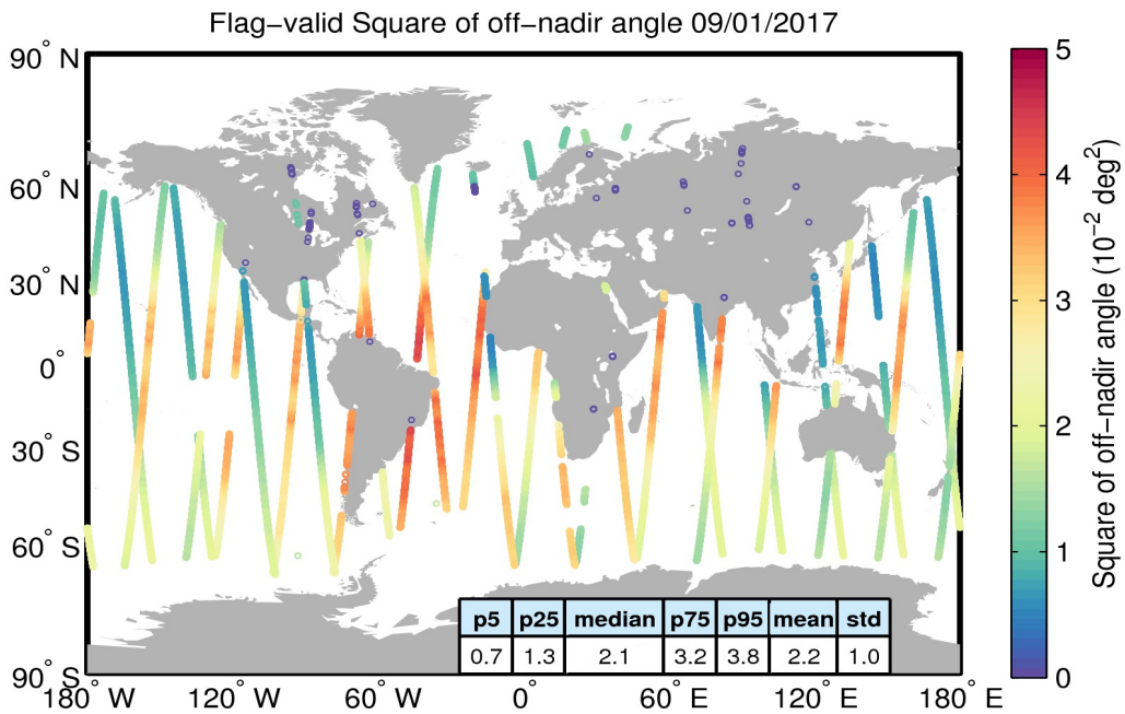
Figure 37. Geographical distribution of flag-valid mispointing data over oceans and lakes for 09/01/2017. The statistical values shown in the table refer to the mispointing in 10^{-2} deg 2 and are calculated over all measurements shown in the figure.
