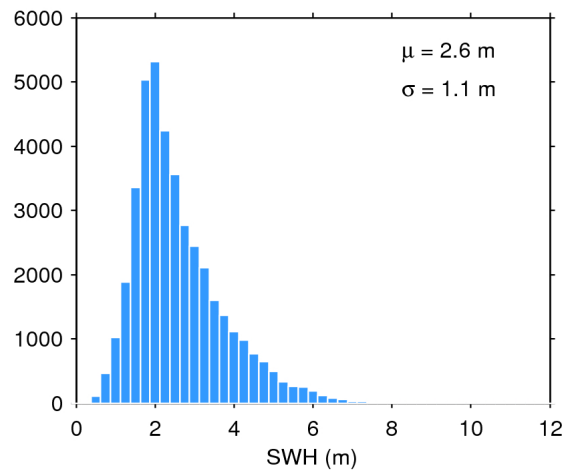
Figure 20. Histogram of science-valid SWH over oceans and lakes for 09/01/2017. The mean ( \mu ) and standard deviation ( \sigma ) are also shown. Note that values larger than 12 m are excluded from the histogram for the sake of readability but not from the computation of \mu and \sigma .
