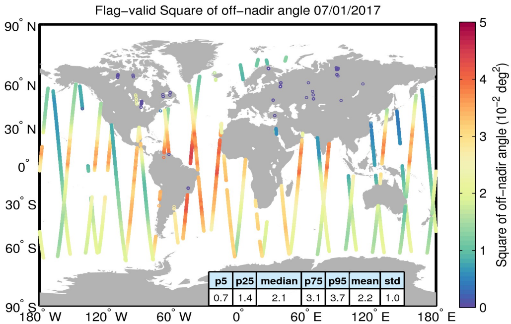
Figure 37. Geographical distribution of flag-valid mispointing data over oceans and lakes for 07/01/2017. The statistical values shown in the table refer to the mispointing in 10^{-2} deg 2 and are calculated over all measurements shown in the figure.
