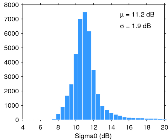
Figure 25. Histogram of flag-valid sigma0 over oceans and lakes for 07/01/2017. The mean ( \mu ) and standard deviation ( \sigma ) are also shown. Note that values outside [4 20] dB are excluded from the histogram for the sake of readability but not from the computation of \mu and \sigma .
