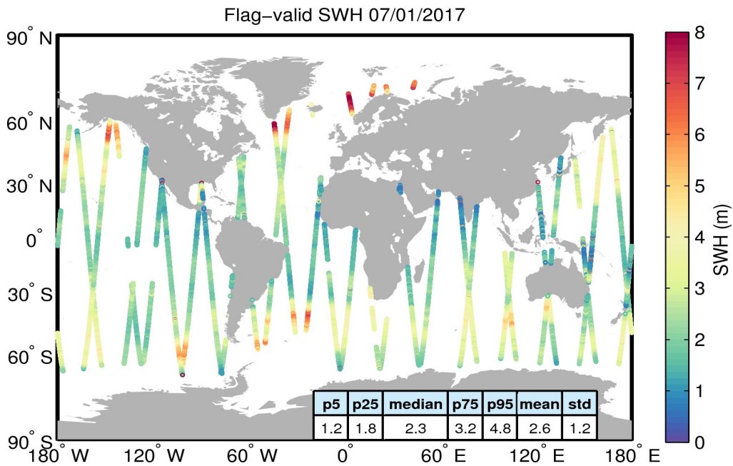
Figure 15. Geographical distribution of flag-valid SWH data over oceans and lakes for 07/01/2017. The statistical values shown in the table refer to the SWH in m and are calculated over all measurements shown in the figure.
