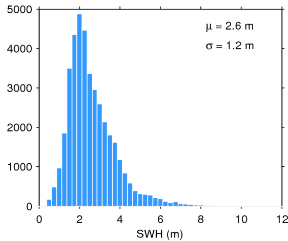
Figure 17. Histogram of flag-valid SWH over oceans and lakes for 07/01/2017. The mean ( \mu ) and standard deviation ( \sigma ) are also shown. Note that values larger than 12 m are excluded from the histogram for the sake of readability but not from the computation of \mu and \sigma .
