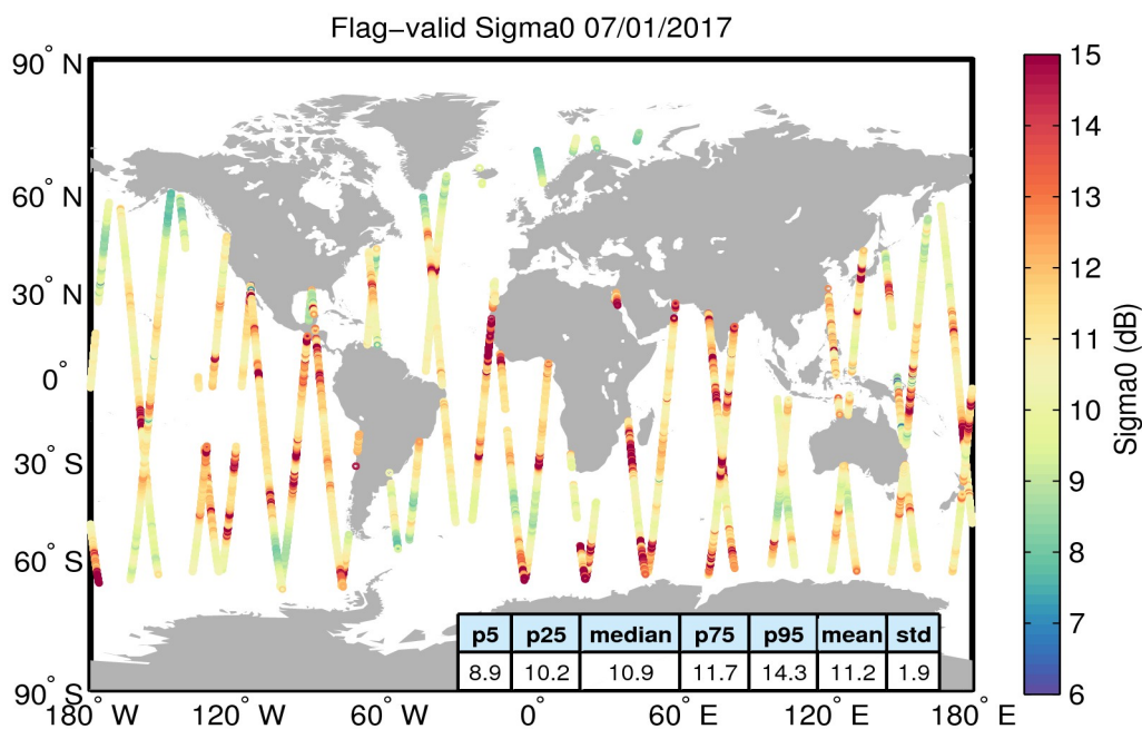
Figure 23. Geographical distribution of flag-valid sigma0 data over oceans and lakes for 07/01/2017. The statistical values shown in the table refer to the sigma0 in dB and are calculated over all measurements shown in the figure.
