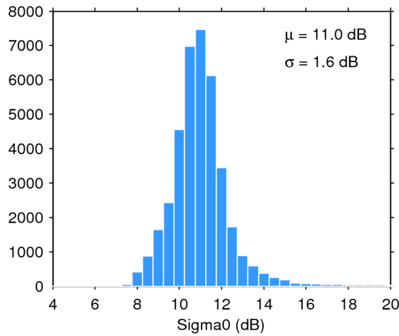
Figure 28. Histogram of science-valid sigma0 over oceans and lakes for 07/01/2017. The mean ( \mu ) and standard deviation ( \sigma ) are also shown. Note that values outside [4 20] dB are excluded from the histogram for the sake of readability but not from the computation of \mu and \sigma .
