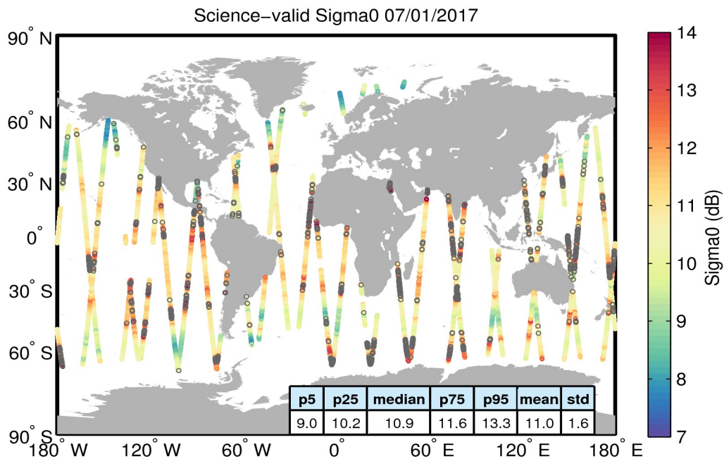
Figure 27. Geographical distribution of science-valid sigma0 data over oceans and lakes for 07/01/2017. The statistical values shown in the table refer to the sigma0 in dB and are calculated over all measurements shown in the figure. Gray circles denote records that have been rejected based on the editing criteria described in Table 4.
