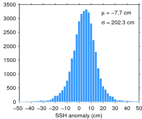
Figure 7. Histogram of flag-valid SSH anomaly over oceans and lakes for 07/01/2017. The mean ( \mu ) and standard deviation ( \sigma ) are also shown. Note that values outside [-50 50] cm are excluded from the histogram for the sake of readability but not from the computation of \mu and \sigma .
