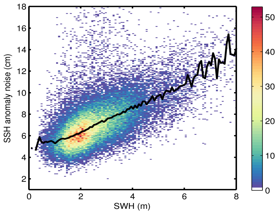
Figure 9. 2D histogram showing flag-valid SSH anomaly noise as a function of SWH for 07/01/2017. The black line denotes the median SSH anomaly noise as a function of SWH.
