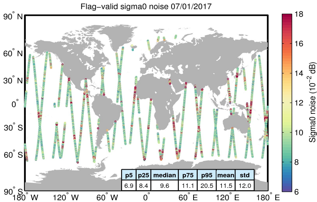
Figure 26. Geographical distribution of flag-valid 20-Hz sigma0 measurement noise over oceans and lakes for 07/01/2017. The statistical values shown in the table refer to the sigma0 noise and are calculated over all measurements shown in the figure.
