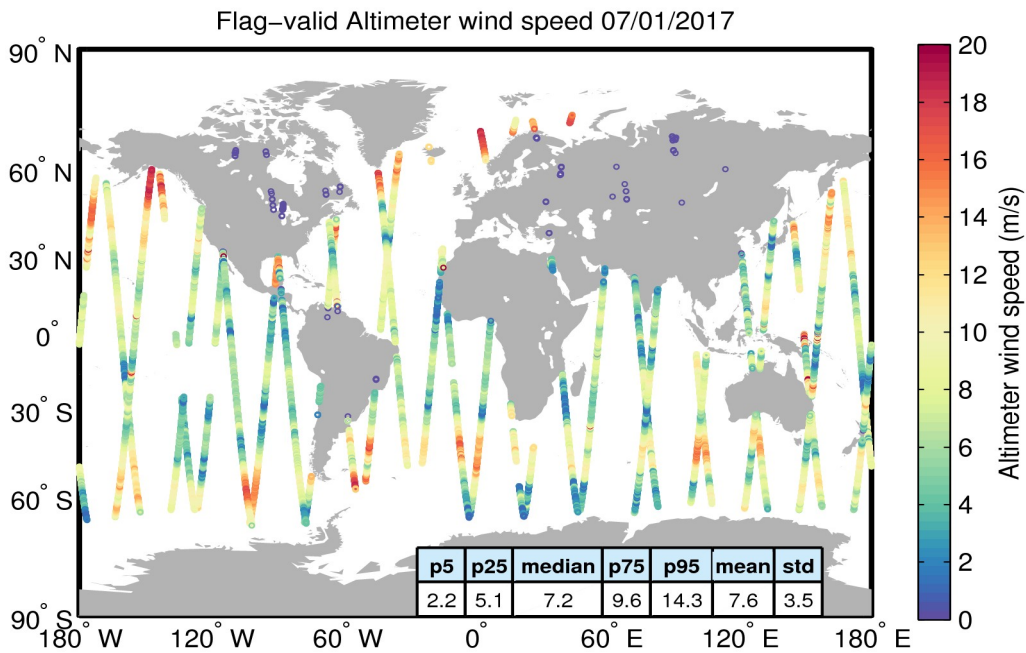
Figure 31. Geographical distribution of flag-valid wind data over oceans and lakes for 07/01/2017. The statistical values shown in the table refer to the wind in m/s and are calculated over all measurements shown in the figure.
