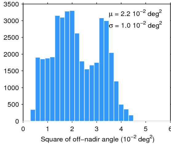
Figure 39. Histogram of flag-valid mispointing over oceans and lakes for 07/01/2017. The mean ( \mu ) and standard deviation ( \sigma ) are also shown. Note that values larger than 6 \cdot 10^{-2} \text{ deg}^2 are excluded from the histogram for the sake of readability but not from the computation of \mu and \sigma .
