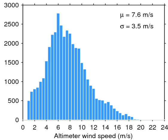
Figure 33. Histogram of flag-valid wind over oceans and lakes for 07/01/2017. The mean ( \mu ) and standard deviation ( \sigma ) are also shown. Note that values larger than 24 m/s are excluded from the histogram for the sake of readability but not from the computation of \mu and \sigma .
