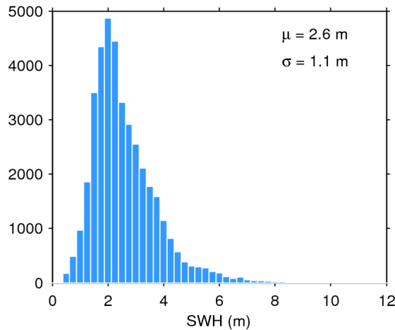
Figure 20. Histogram of science-valid SWH over oceans and lakes for 07/01/2017. The mean ( \mu ) and standard deviation ( \sigma ) are also shown. Note that values larger than 12 m are excluded from the histogram for the sake of readability but not from the computation of \mu and \sigma .
