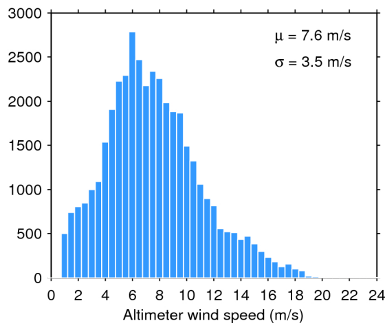
Figure 35. Histogram of science-valid wind over oceans and lakes for 07/01/2017. The mean ( \mu ) and standard deviation ( \sigma ) are also shown. Note that values larger than 24 m/s are excluded from the histogram for the sake of readability but not from the computation of \mu and \sigma .
