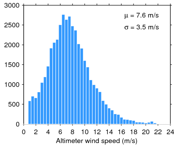
Figure 33. Histogram of flag-valid wind over oceans and lakes for 06/01/2017. The mean ( \mu ) and standard deviation ( \sigma ) are also shown. Note that values larger than 24 m/s are excluded from the histogram for the sake of readability but not from the computation of \mu and \sigma .
