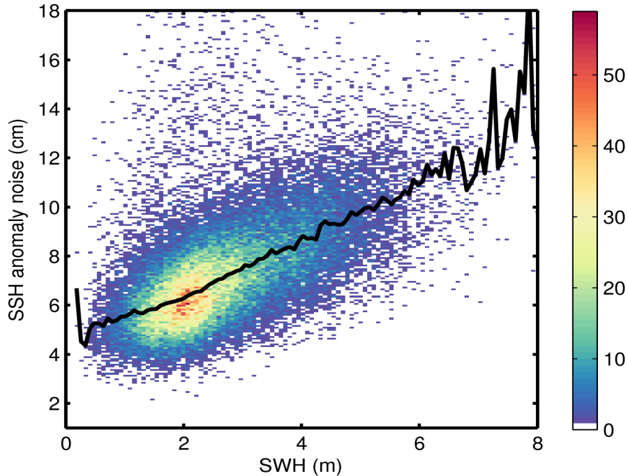
Figure 9. 2D histogram showing flag-valid SSH anomaly noise as a function of SWH for 06/01/2017. The black line denotes the median SSH anomaly noise as a function of SWH.
