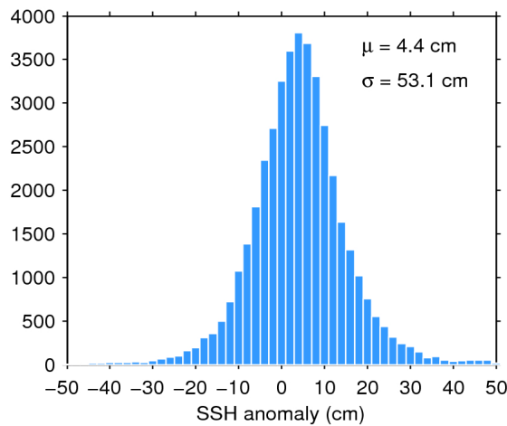
Figure 7. Histogram of flag-valid SSH anomaly over oceans and lakes for 06/01/2017. The mean ( \mu ) and standard deviation ( \sigma ) are also shown. Note that values outside [-50 50] cm are excluded from the histogram for the sake of readability but not from the computation of \mu and \sigma .
