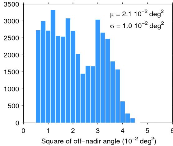
Figure 39. Histogram of flag-valid mispointing over oceans and lakes for 06/01/2017. The mean ( \mu ) and standard deviation ( \sigma ) are also shown. Note that values larger than 6 \cdot 10^{-2} \text{ deg}^2 are excluded from the histogram for the sake of readability but not from the computation of \mu and \sigma .
