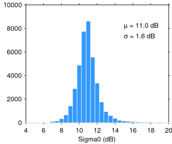
Figure 28. Histogram of science-valid sigma0 over oceans and lakes for 06/01/2017. The mean ( \mu ) and standard deviation ( \sigma ) are also shown. Note that values outside [4 20] dB are excluded from the histogram for the sake of readability but not from the computation of \mu and \sigma .
