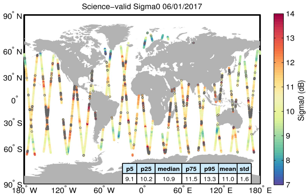
Figure 27. Geographical distribution of science-valid sigma0 data over oceans and lakes for 06/01/2017. The statistical values shown in the table refer to the sigma0 in dB and are calculated over all measurements shown in the figure. Gray circles denote records that have been rejected based on the editing criteria described in Table 4.
