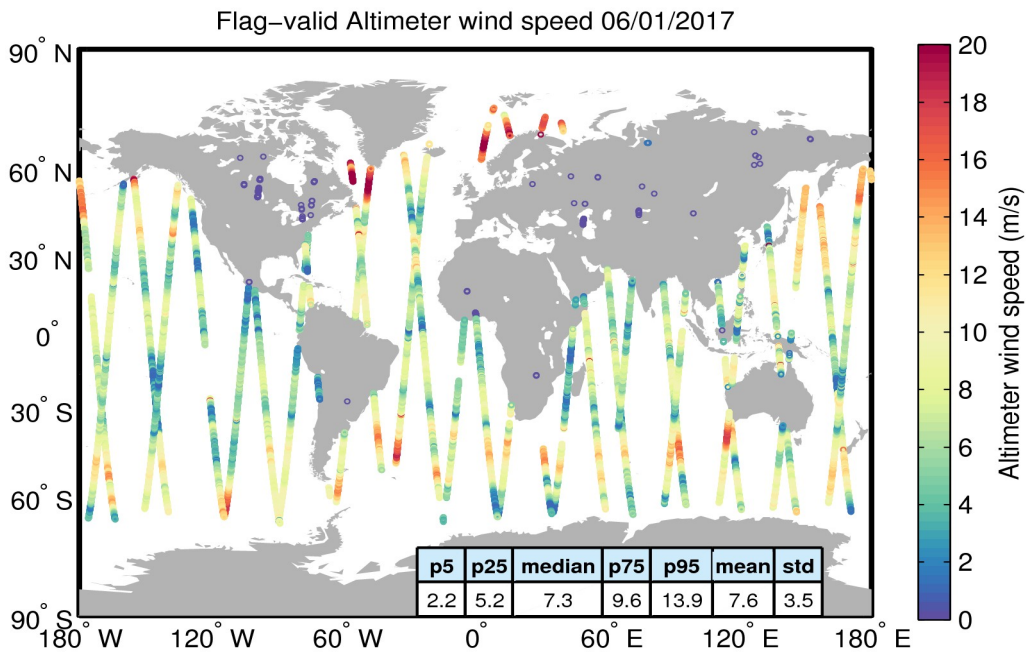
Figure 31. Geographical distribution of flag-valid wind data over oceans and lakes for 06/01/2017. The statistical values shown in the table refer to the wind in m/s and are calculated over all measurements shown in the figure.
