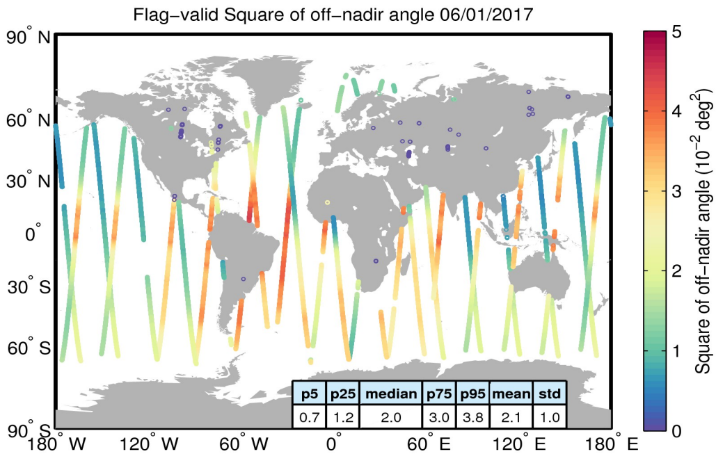
Figure 37. Geographical distribution of flag-valid mispointing data over oceans and lakes for 06/01/2017. The statistical values shown in the table refer to the mispointing in 10^{-2} deg 2 and are calculated over all measurements shown in the figure.
