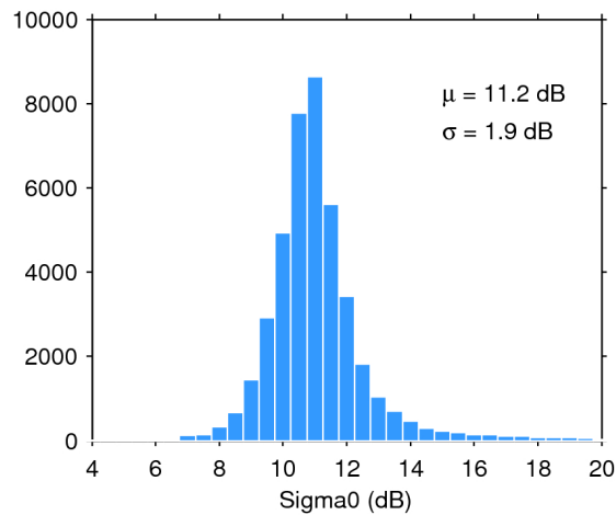
Figure 25. Histogram of flag-valid sigma0 over oceans and lakes for 06/01/2017. The mean ( \mu ) and standard deviation ( \sigma ) are also shown. Note that values outside [4 20] dB are excluded from the histogram for the sake of readability but not from the computation of \mu and \sigma .
