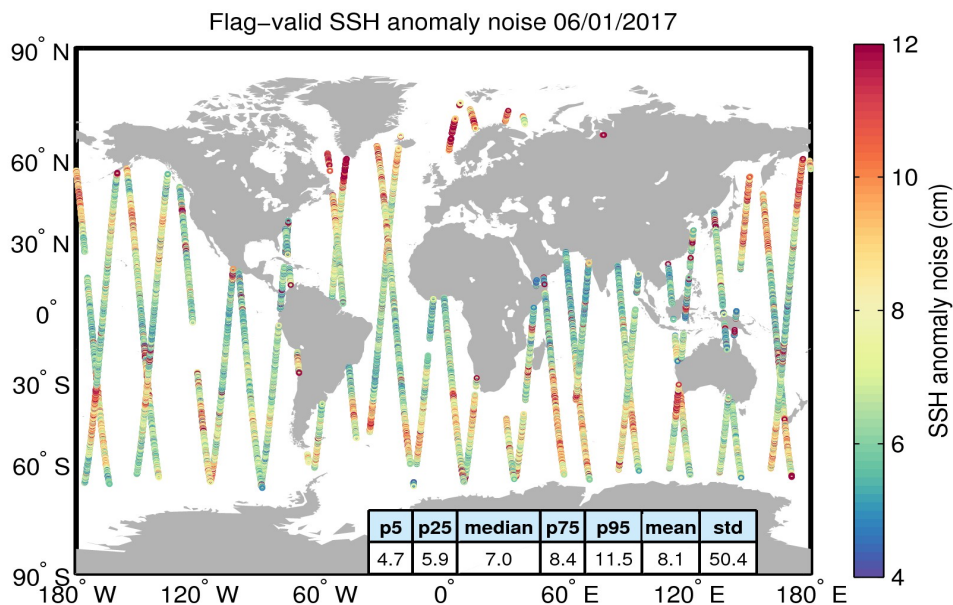
Figure 8. Geographical distribution of flag-valid 20-Hz SSH anomaly measurement noise over oceans and lakes for 06/01/2017. The statistical values shown in the table refer to the SSH anomaly noise and are calculated over all measurements shown in the figure.
