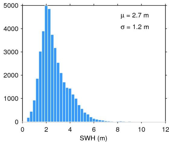
Figure 20. Histogram of science-valid SWH over oceans and lakes for 06/01/2017. The mean ( \mu ) and standard deviation ( \sigma ) are also shown. Note that values larger than 12 m are excluded from the histogram for the sake of readability but not from the computation of \mu and \sigma .
