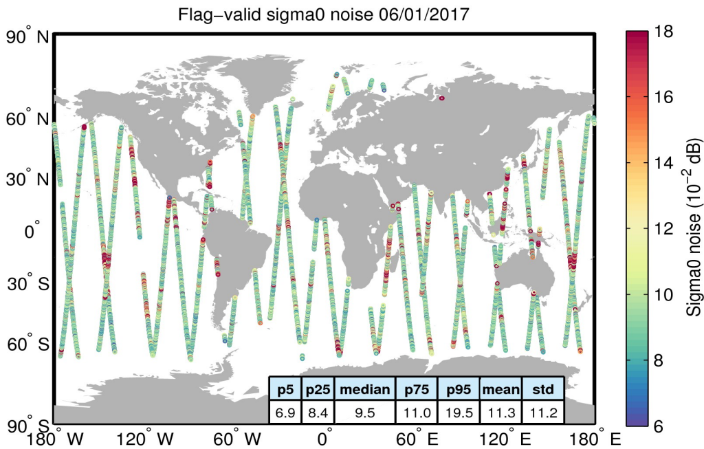
Figure 26. Geographical distribution of flag-valid 20-Hz sigma0 measurement noise over oceans and lakes for 06/01/2017. The statistical values shown in the table refer to the sigma0 noise and are calculated over all measurements shown in the figure.
