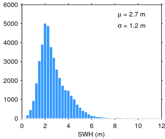
Figure 17. Histogram of flag-valid SWH over oceans and lakes for 06/01/2017. The mean ( \mu ) and standard deviation ( \sigma ) are also shown. Note that values larger than 12 m are excluded from the histogram for the sake of readability but not from the computation of \mu and \sigma .
