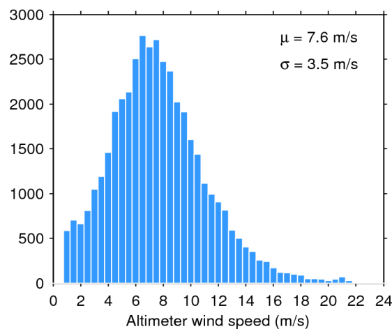
Figure 35. Histogram of science-valid wind over oceans and lakes for 06/01/2017. The mean ( \mu ) and standard deviation ( \sigma ) are also shown. Note that values larger than 24 m/s are excluded from the histogram for the sake of readability but not from the computation of \mu and \sigma .
