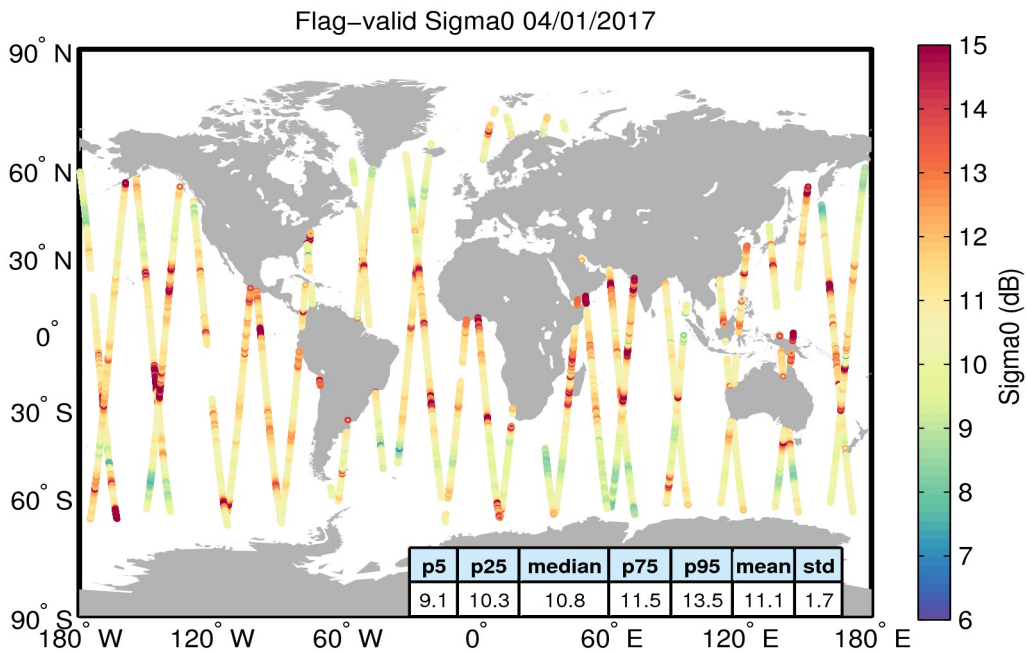
Figure 23. Geographical distribution of flag-valid sigma0 data over oceans and lakes for 04/01/2017. The statistical values shown in the table refer to the sigma0 in dB and are calculated over all measurements shown in the figure.
