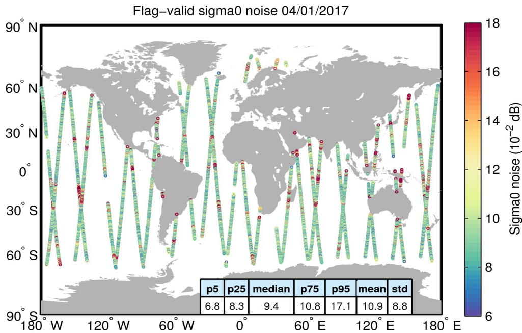
Figure 26. Geographical distribution of flag-valid 20-Hz sigma0 measurement noise over oceans and lakes for 04/01/2017. The statistical values shown in the table refer to the sigma0 noise and are calculated over all measurements shown in the figure.
