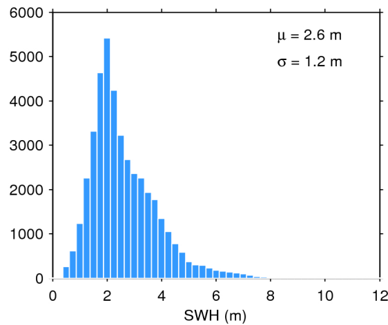
Figure 17. Histogram of flag-valid SWH over oceans and lakes for 04/01/2017. The mean ( \mu ) and standard deviation ( \sigma ) are also shown. Note that values larger than 12 m are excluded from the histogram for the sake of readability but not from the computation of \mu and \sigma .
