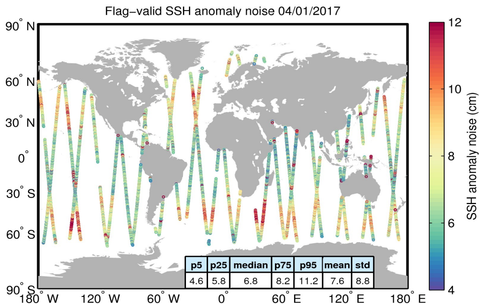
Figure 8. Geographical distribution of flag-valid 20-Hz SSH anomaly measurement noise over oceans and lakes for 04/01/2017. The statistical values shown in the table refer to the SSH anomaly noise and are calculated over all measurements shown in the figure.
