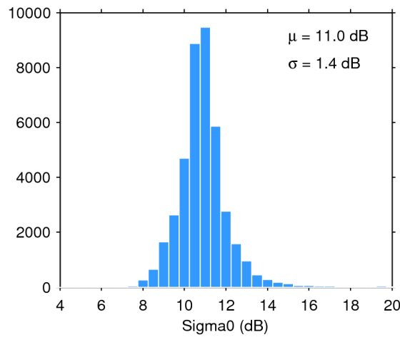
Figure 28. Histogram of science-valid sigma0 over oceans and lakes for 04/01/2017. The mean ( \mu ) and standard deviation ( \sigma ) are also shown. Note that values outside [4 20] dB are excluded from the histogram for the sake of readability but not from the computation of \mu and \sigma .
