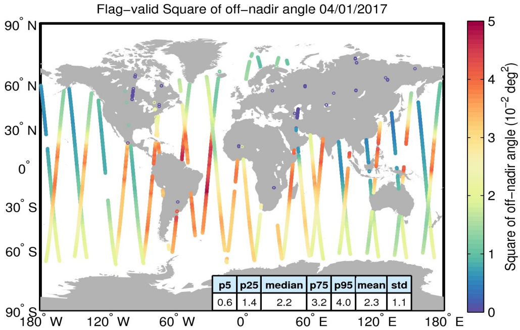
Figure 37. Geographical distribution of flag-valid mispointing data over oceans and lakes for 04/01/2017. The statistical values shown in the table refer to the mispointing in 10^{-2} deg 2 and are calculated over all measurements shown in the figure.
