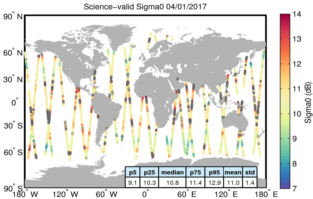
Figure 27. Geographical distribution of science-valid sigma0 data over oceans and lakes for 04/01/2017. The statistical values shown in the table refer to the sigma0 in dB and are calculated over all measurements shown in the figure. Gray circles denote records that have been rejected based on the editing criteria described in Table 4.
