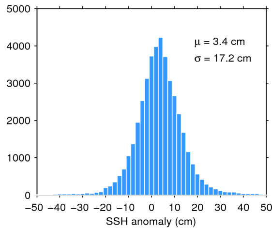
Figure 7. Histogram of flag-valid SSH anomaly over oceans and lakes for 04/01/2017. The mean ( \mu ) and standard deviation ( \sigma ) are also shown. Note that values outside [-50 50] cm are excluded from the histogram for the sake of readability but not from the computation of \mu and \sigma .
