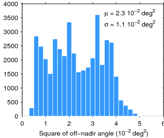
Figure 39. Histogram of flag-valid mispointing over oceans and lakes for 04/01/2017. The mean ( \mu ) and standard deviation ( \sigma ) are also shown. Note that values larger than 6 \cdot 10^{-2} \text{ deg}^2 are excluded from the histogram for the sake of readability but not from the computation of \mu and \sigma .
