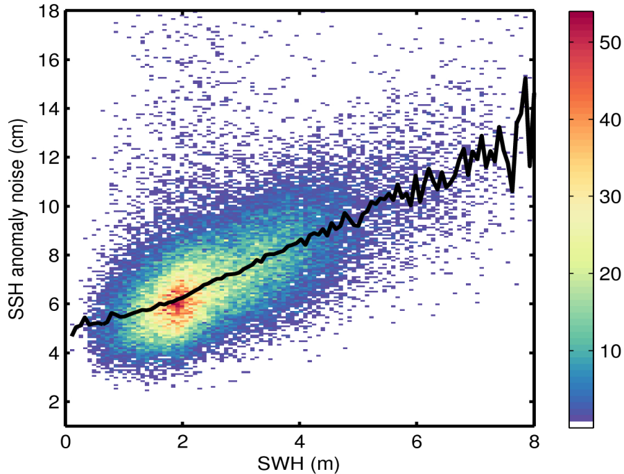
Figure 9. 2D histogram showing flag-valid SSH anomaly noise as a function of SWH for 04/01/2017. The black line denotes the median SSH anomaly noise as a function of SWH.
