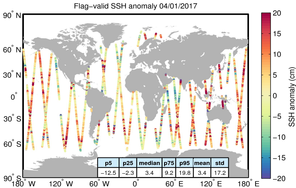
Figure 5. Geographical distribution of flag-valid 1-Hz SSH anomaly data over oceans and lakes for 04/01/2017. The statistical values shown in the table refer to the SSH anomaly in cm and are calculated over all measurements shown in the figure.
