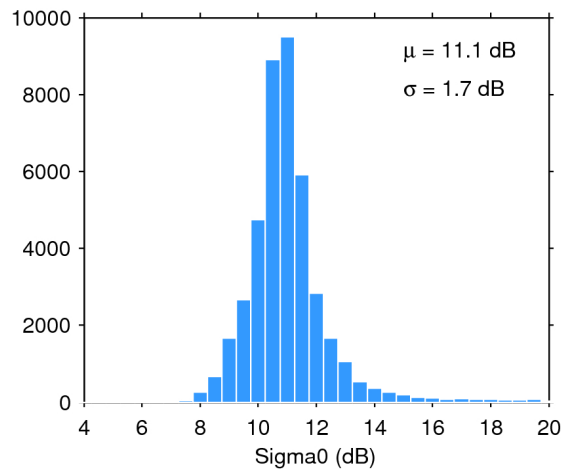
Figure 25. Histogram of flag-valid sigma0 over oceans and lakes for 04/01/2017. The mean ( \mu ) and standard deviation ( \sigma ) are also shown. Note that values outside [4 20] dB are excluded from the histogram for the sake of readability but not from the computation of \mu and \sigma .
