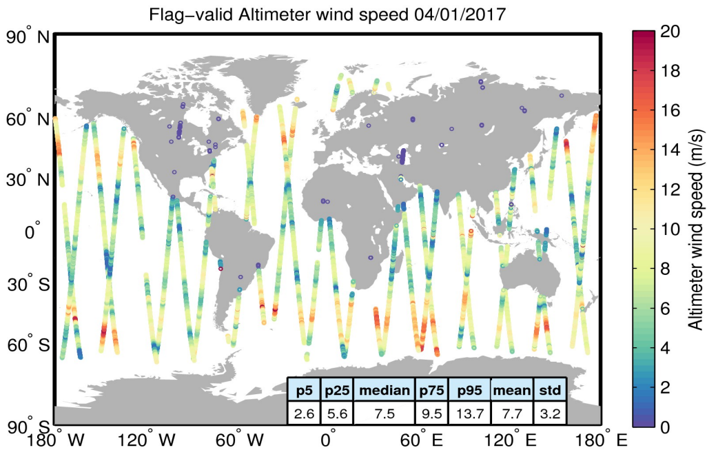
Figure 31. Geographical distribution of flag-valid wind data over oceans and lakes for 04/01/2017. The statistical values shown in the table refer to the wind in m/s and are calculated over all measurements shown in the figure.
