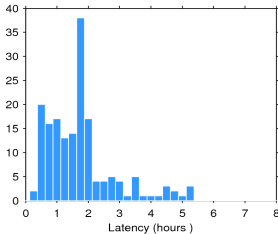
Figure 2. Histogram of the data latency for 04/01/2017. The y-axis denotes the number of files that are made available with a delay of x-hours with respect to the mean time of the records stored in the file.
