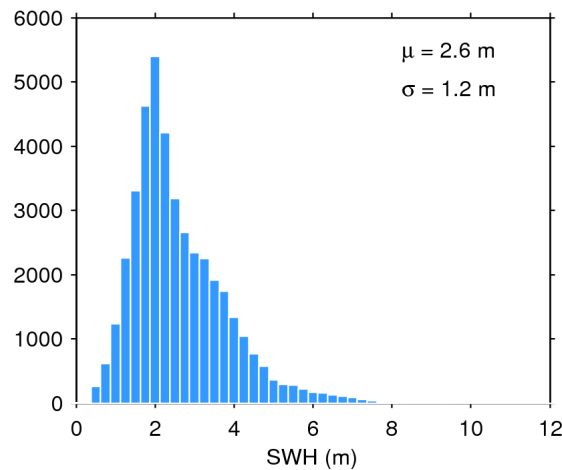
Figure 20. Histogram of science-valid SWH over oceans and lakes for 04/01/2017. The mean ( \mu ) and standard deviation ( \sigma ) are also shown. Note that values larger than 12 m are excluded from the histogram for the sake of readability but not from the computation of \mu and \sigma .
