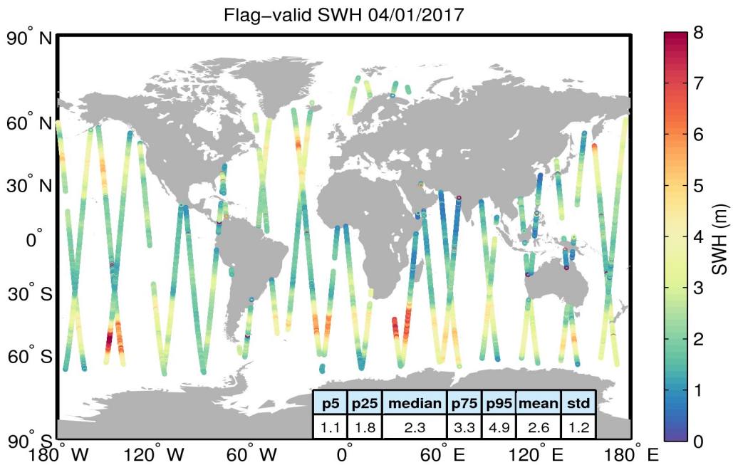
Figure 15. Geographical distribution of flag-valid SWH data over oceans and lakes for 04/01/2017. The statistical values shown in the table refer to the SWH in m and are calculated over all measurements shown in the figure.
