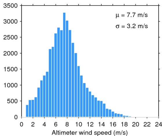
Figure 35. Histogram of science-valid wind over oceans and lakes for 04/01/2017. The mean ( \mu ) and standard deviation ( \sigma ) are also shown. Note that values larger than 24 m/s are excluded from the histogram for the sake of readability but not from the computation of \mu and \sigma .
