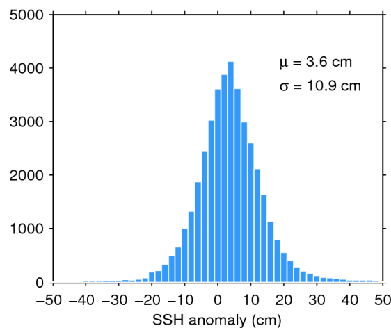
Figure 11. Histogram of science-valid SSH anomaly over oceans and lakes for 04/01/2017. The mean ( \mu ) and standard deviation ( \sigma ) are also shown. Note that values outside [-50 50] cm are excluded from the histogram for the sake of readability but not from the computation of \mu and \sigma .
