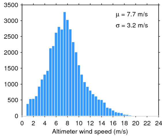
Figure 33. Histogram of flag-valid wind over oceans and lakes for 04/01/2017. The mean ( \mu ) and standard deviation ( \sigma ) are also shown. Note that values larger than 24 m/s are excluded from the histogram for the sake of readability but not from the computation of \mu and \sigma .
